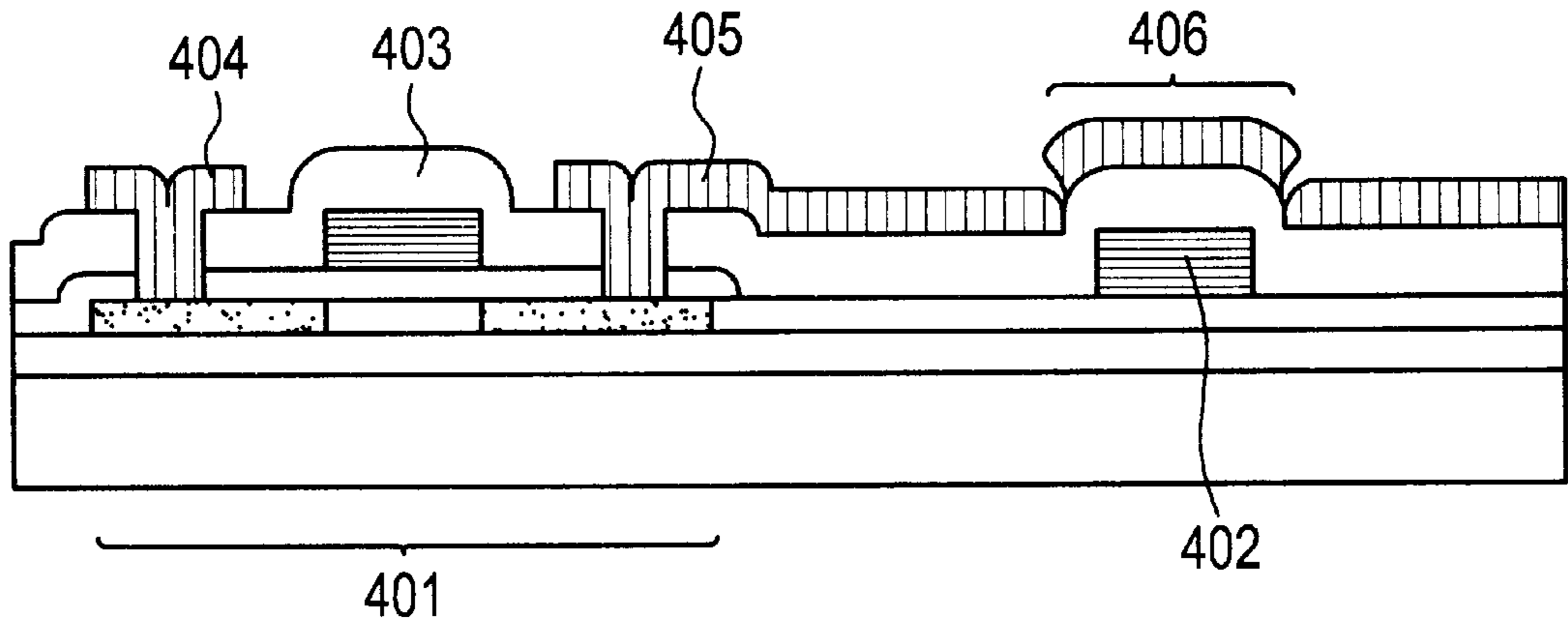
FIG. 4 PRIOR ART
