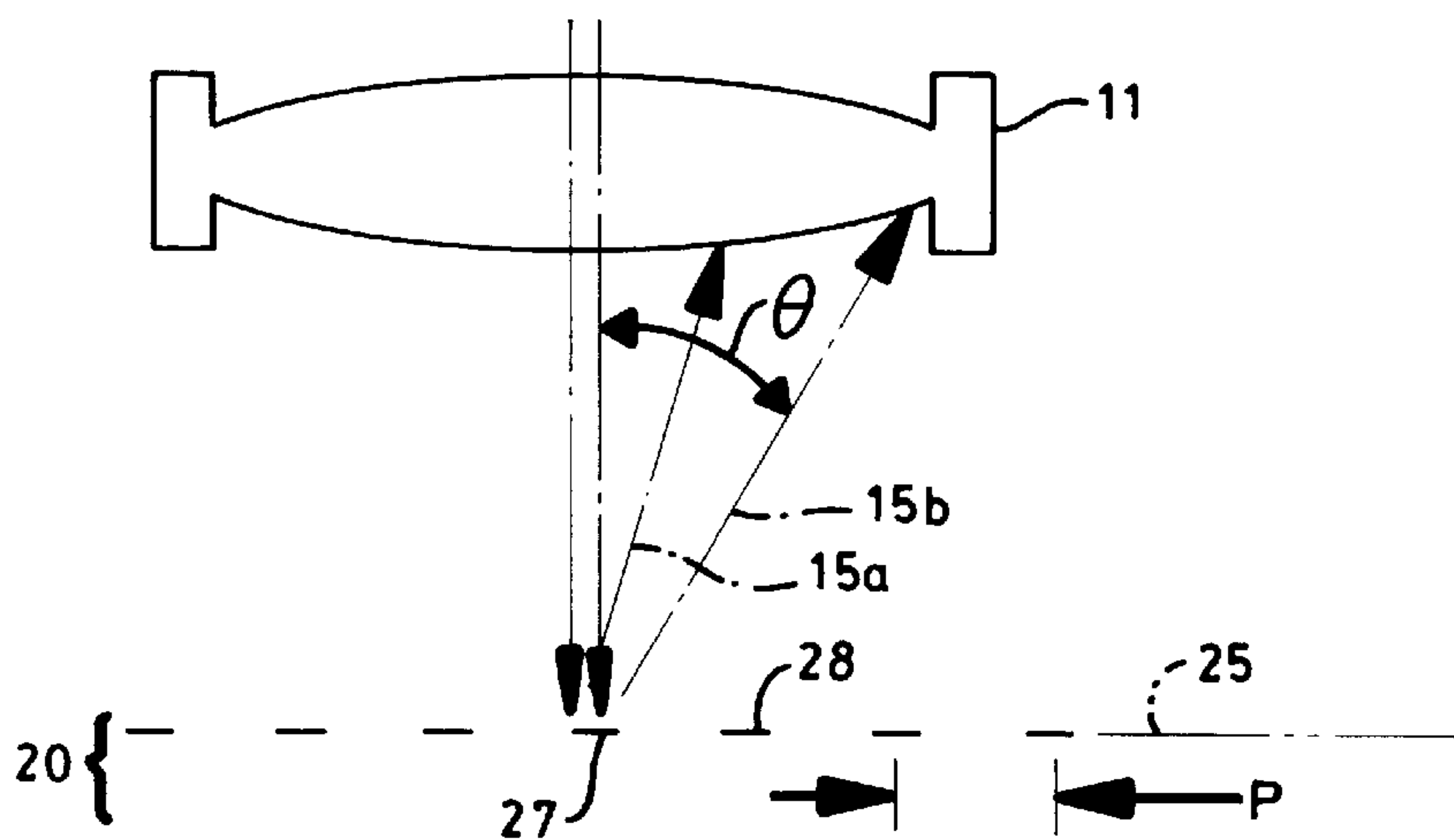
FIG. 3 (PRIOR ART)
