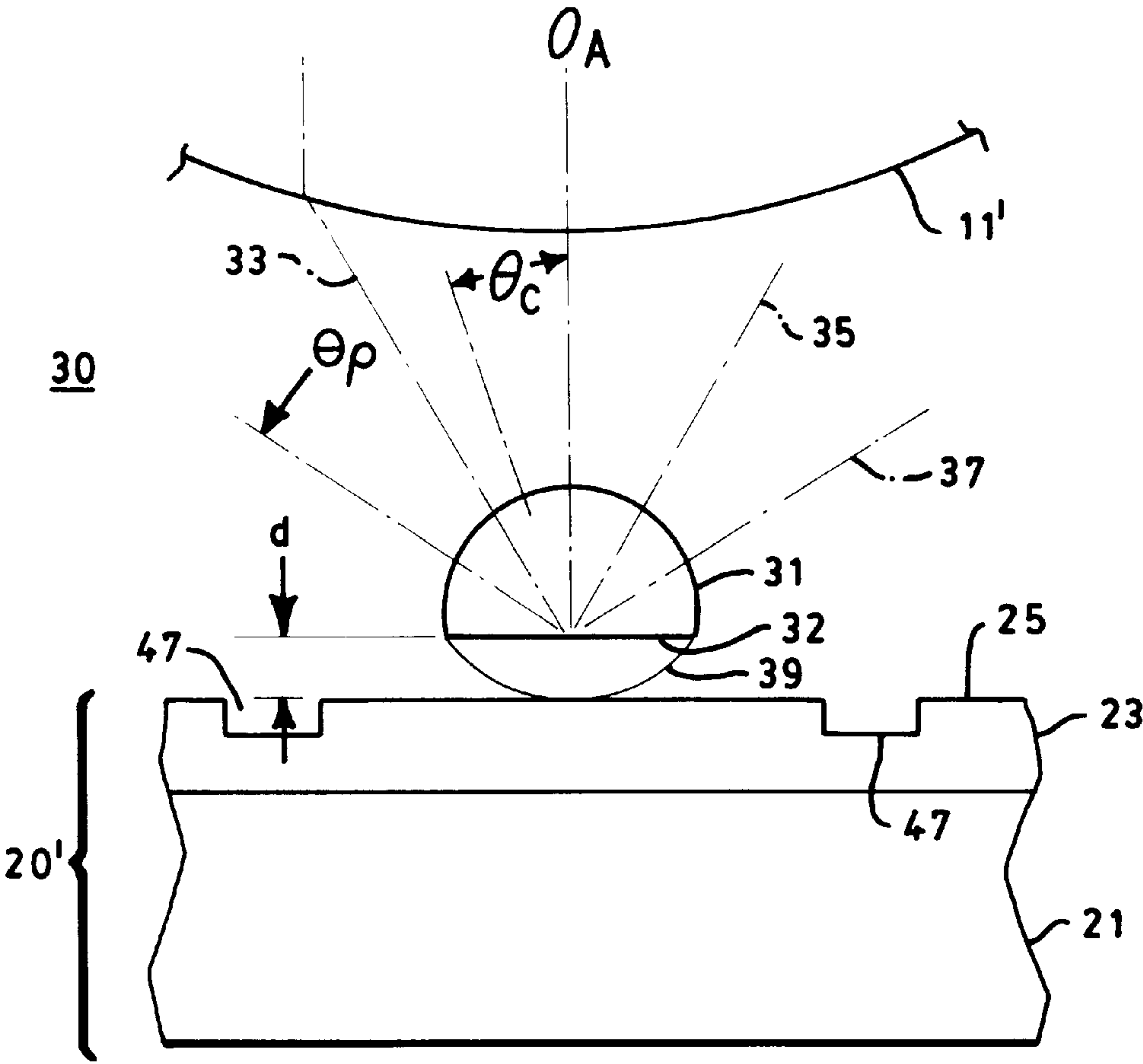
FIG. 9 (PRIOR ART)
