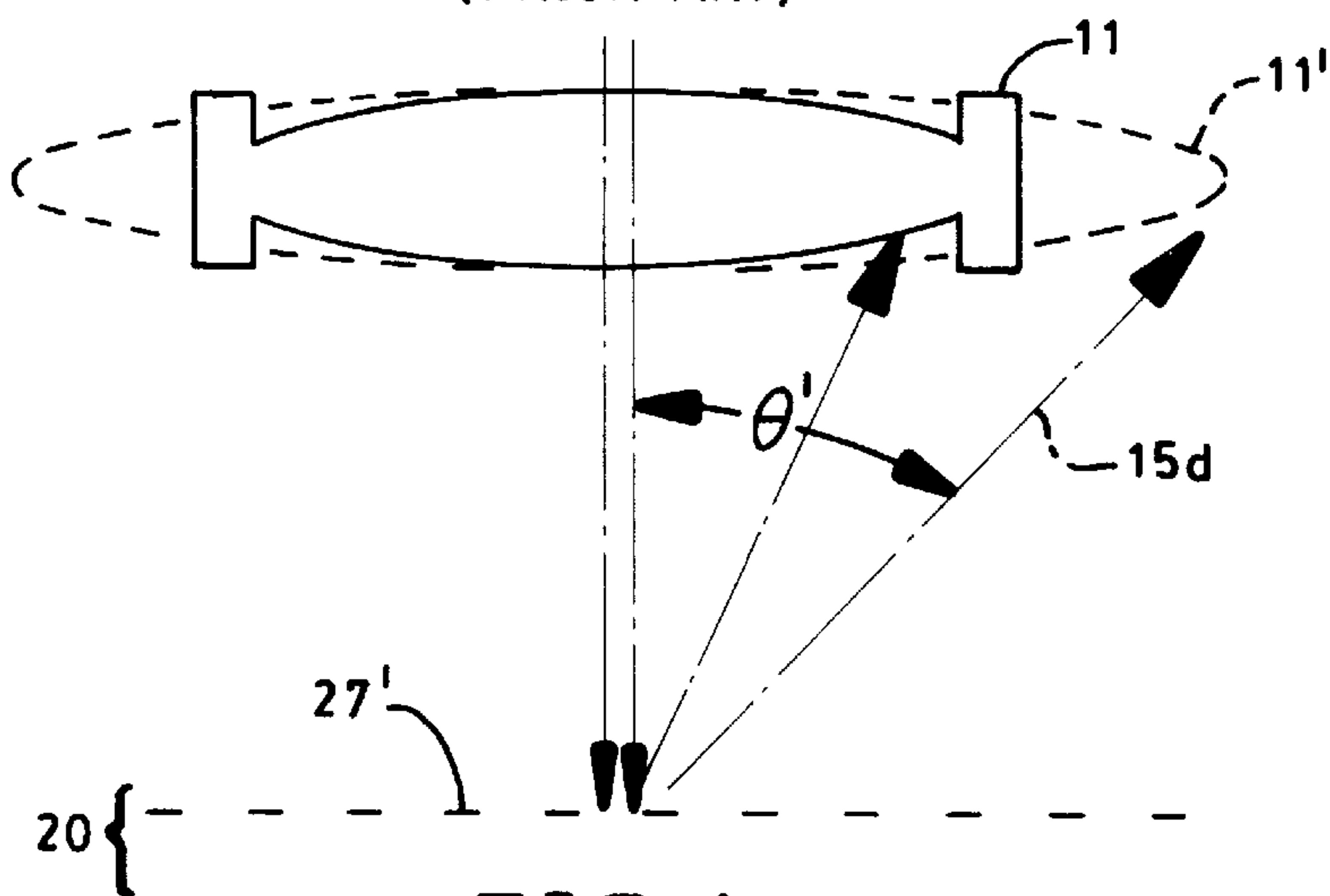
FIG. 4 (PRIOR ART)
