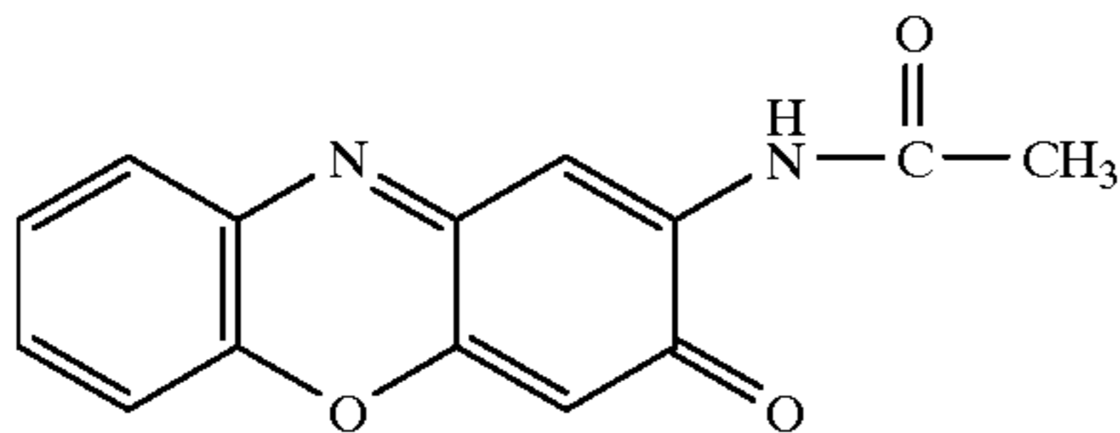
2-acetylamino- phenoxazin-3-one ("AAPOZ")
