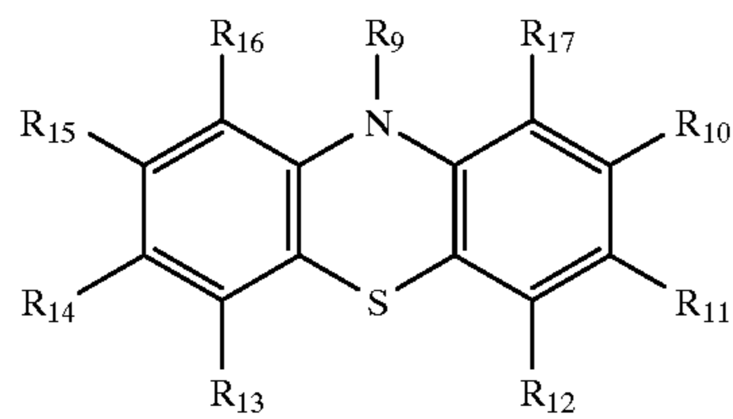
phenothiazines
