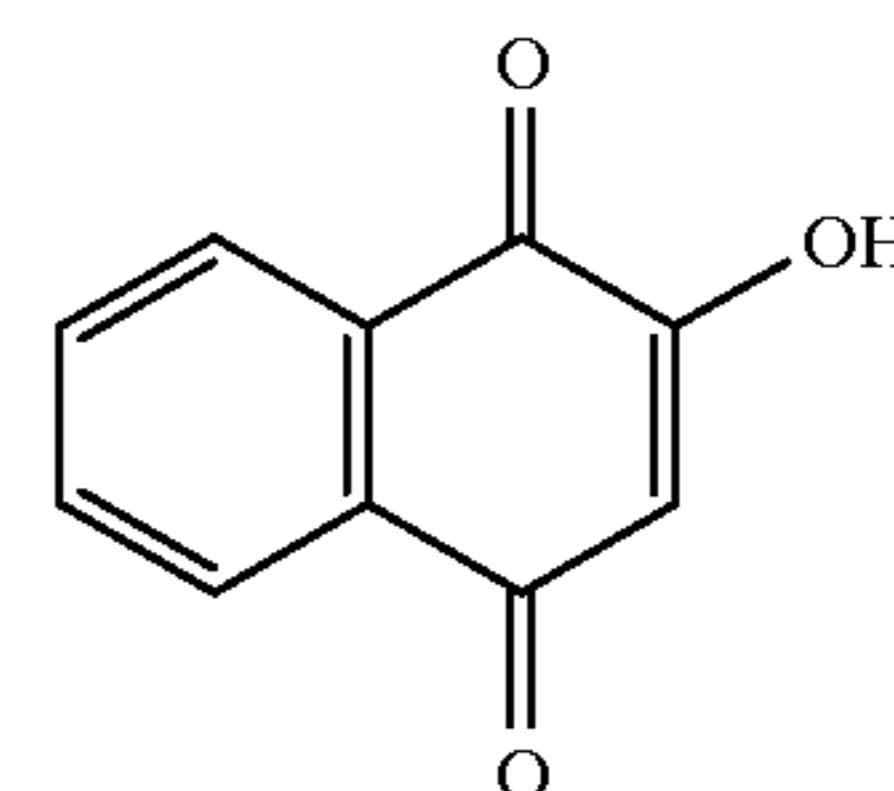
2-hydroxy-naphthoquinone
