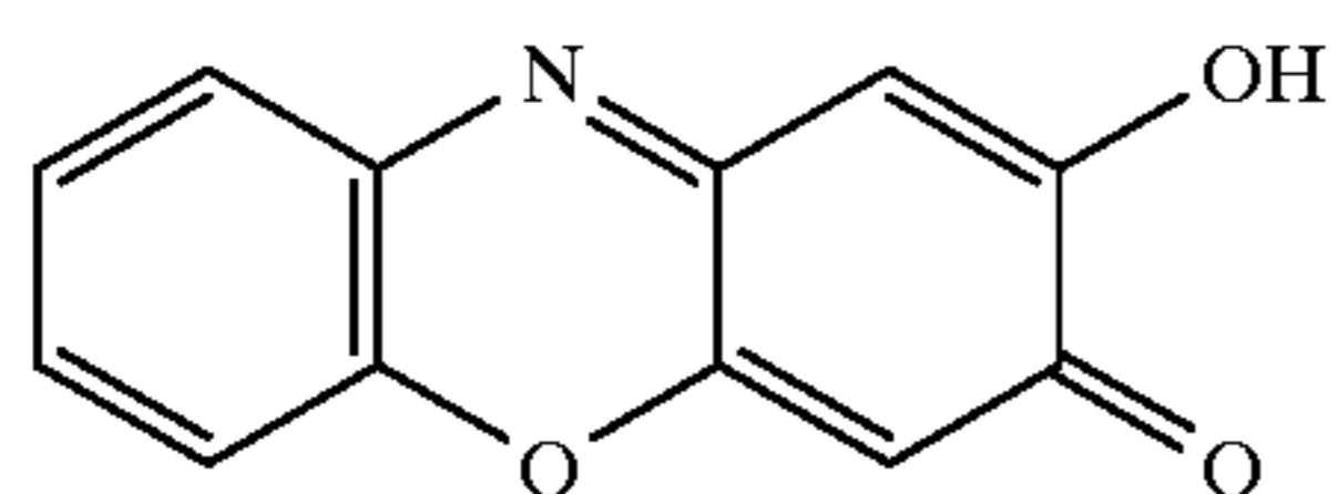
2-hydroxy-phenoxazin- 3-one ("HPOZ")
