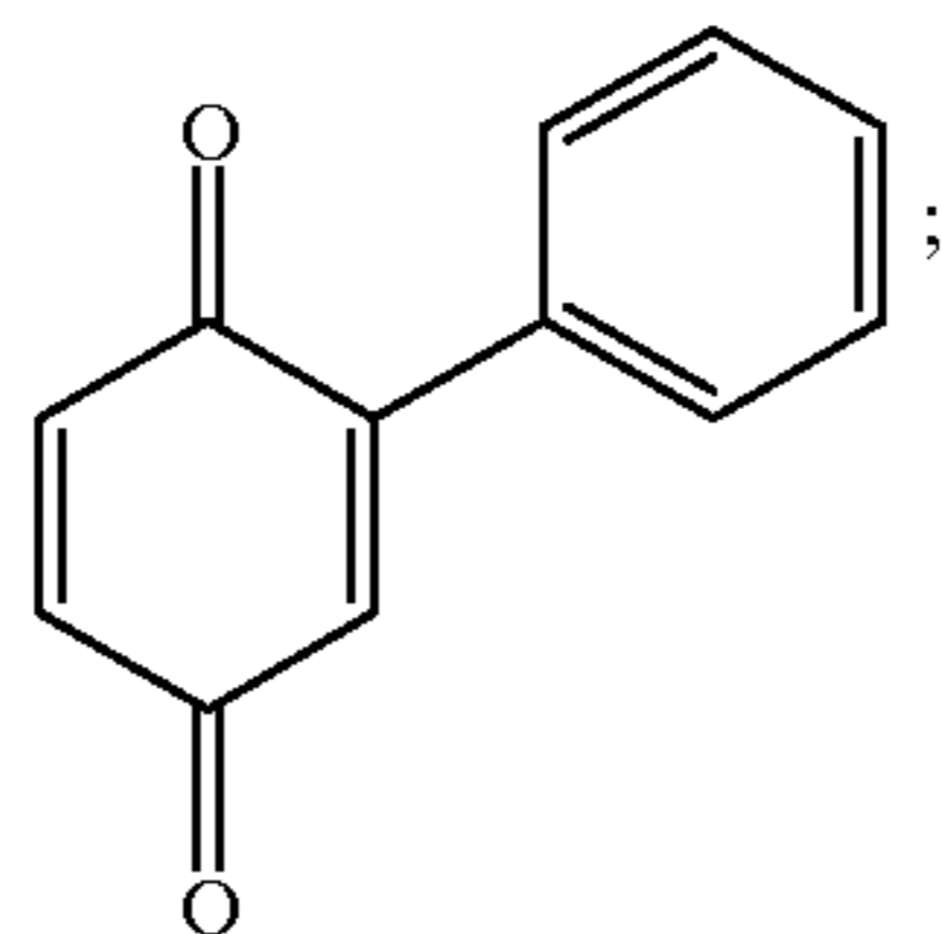
Phenyl-1,4-benzoquinone
