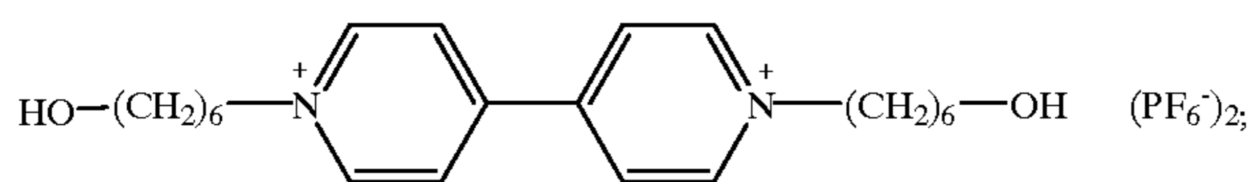
Hydroxyhexyl Viologen Hexafluorophosphate ("HHVPF 6 ")
