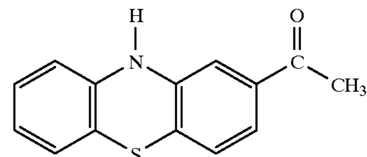
2-acetyl-phenothiazine ("APT")
