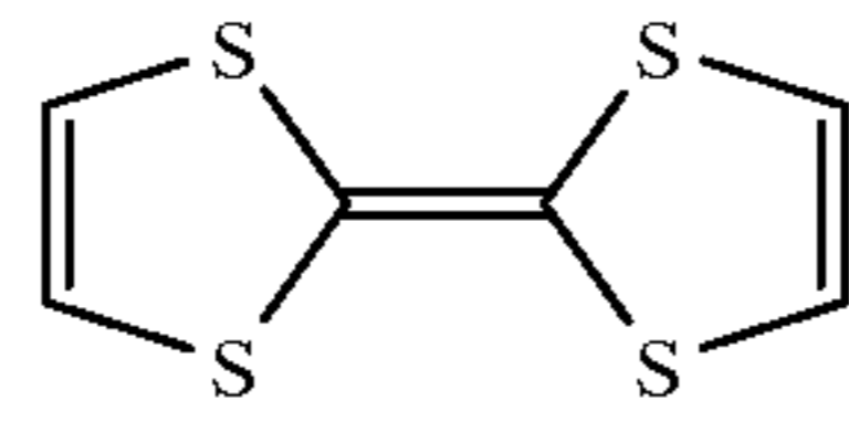
tetrathiafulvalene ("TTF")
