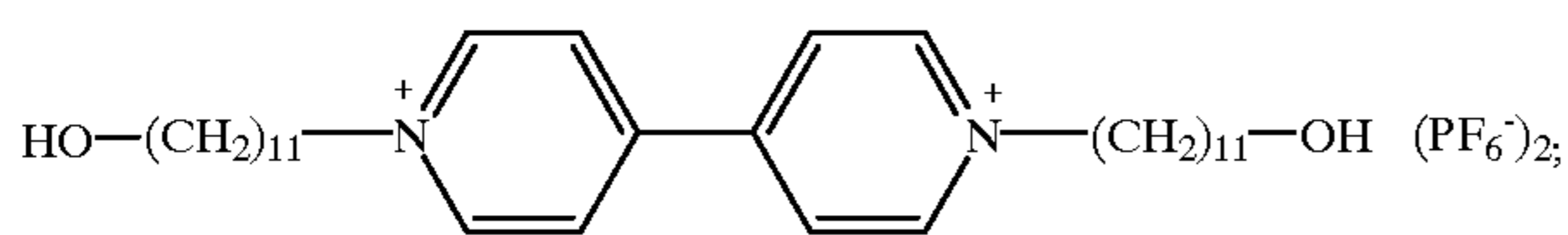
Hydroxyundecyl Viologen Hexafluorophosphate ("HUVPF 6 ")
