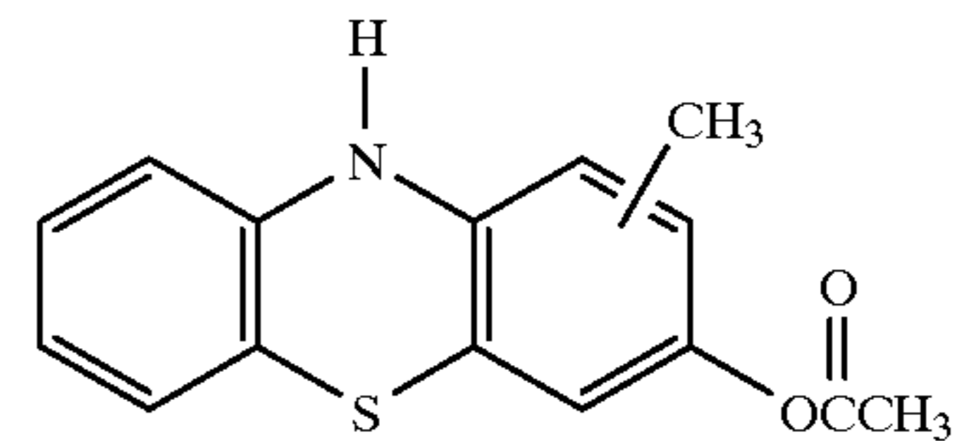
3-acetoxy-methyl-10H-phenothiazine ("AMPT")
