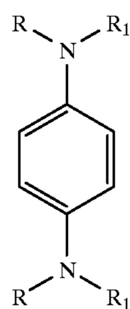
derivatives of 1,4-phenylenediamine
