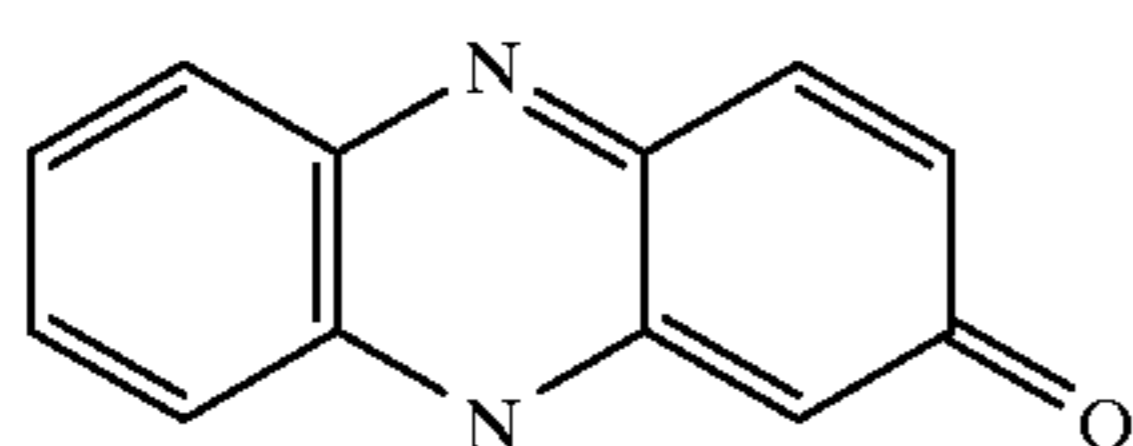
2-keto-N-ethyl- phenazine ("KEPA")
