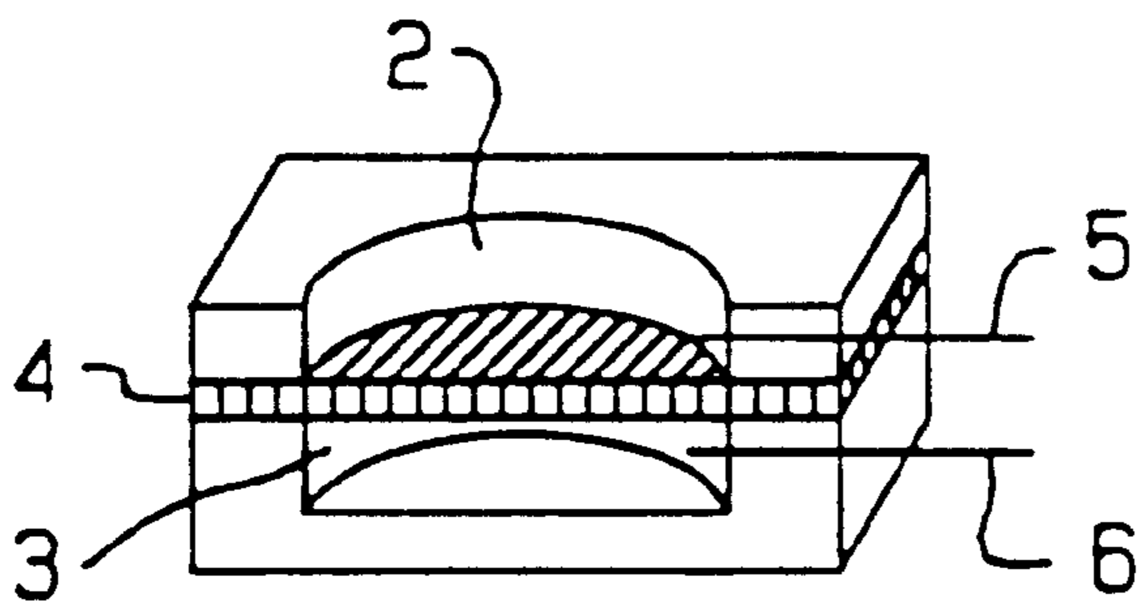
Sectional drawing of galvanic cell 1
