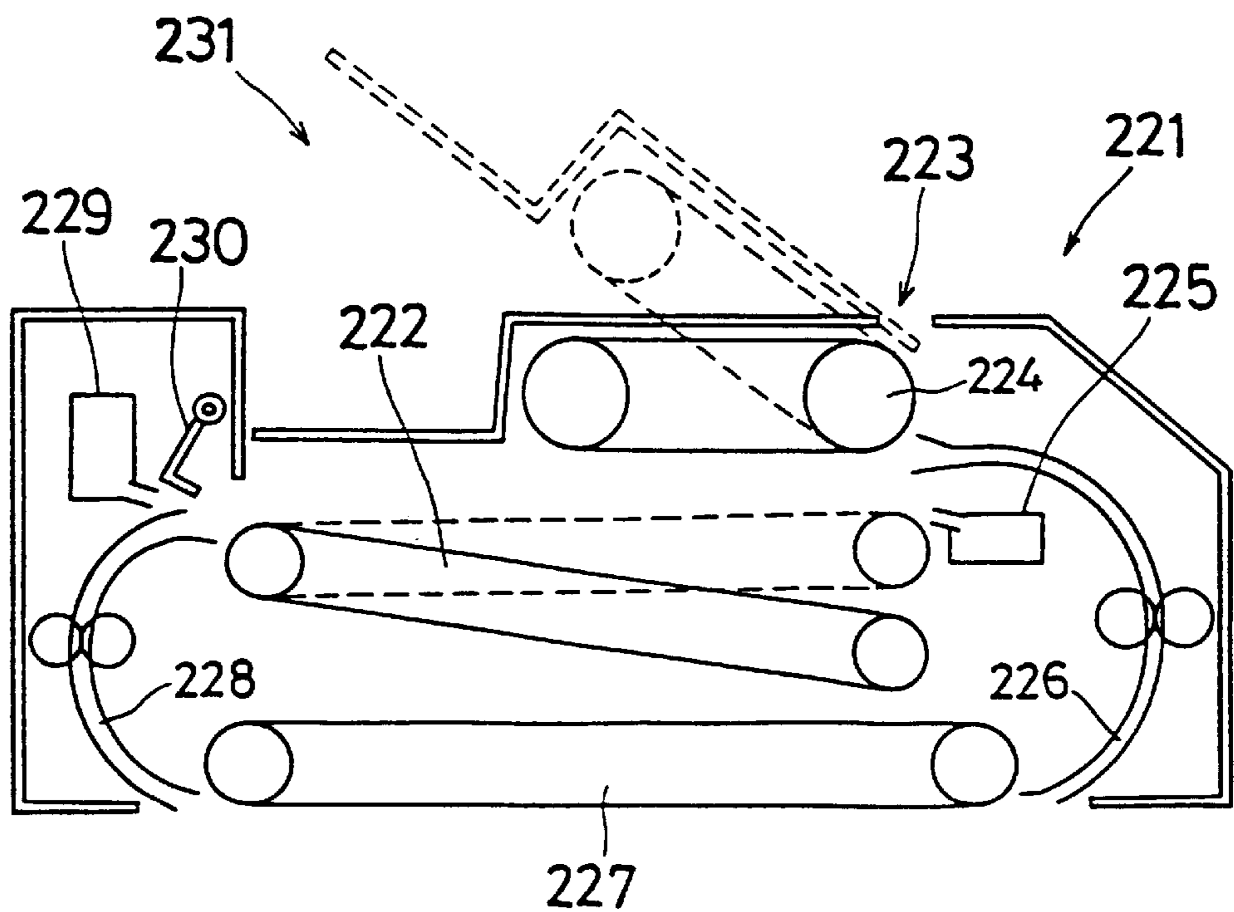
FIG. 59 PRIOR ART
