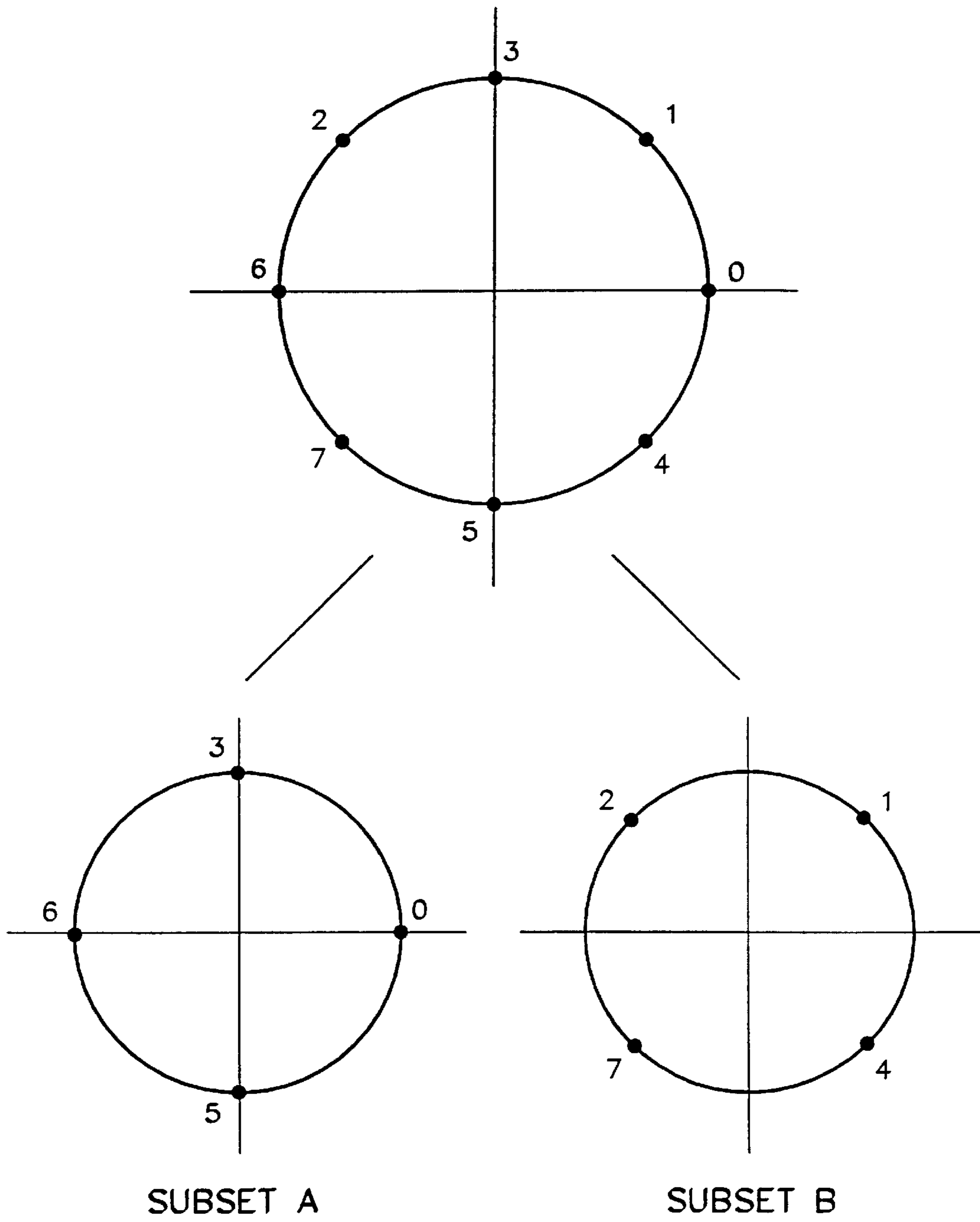
OUTPUT TABLE SET PARTITIONING FOR RAYLEIGH FADING
