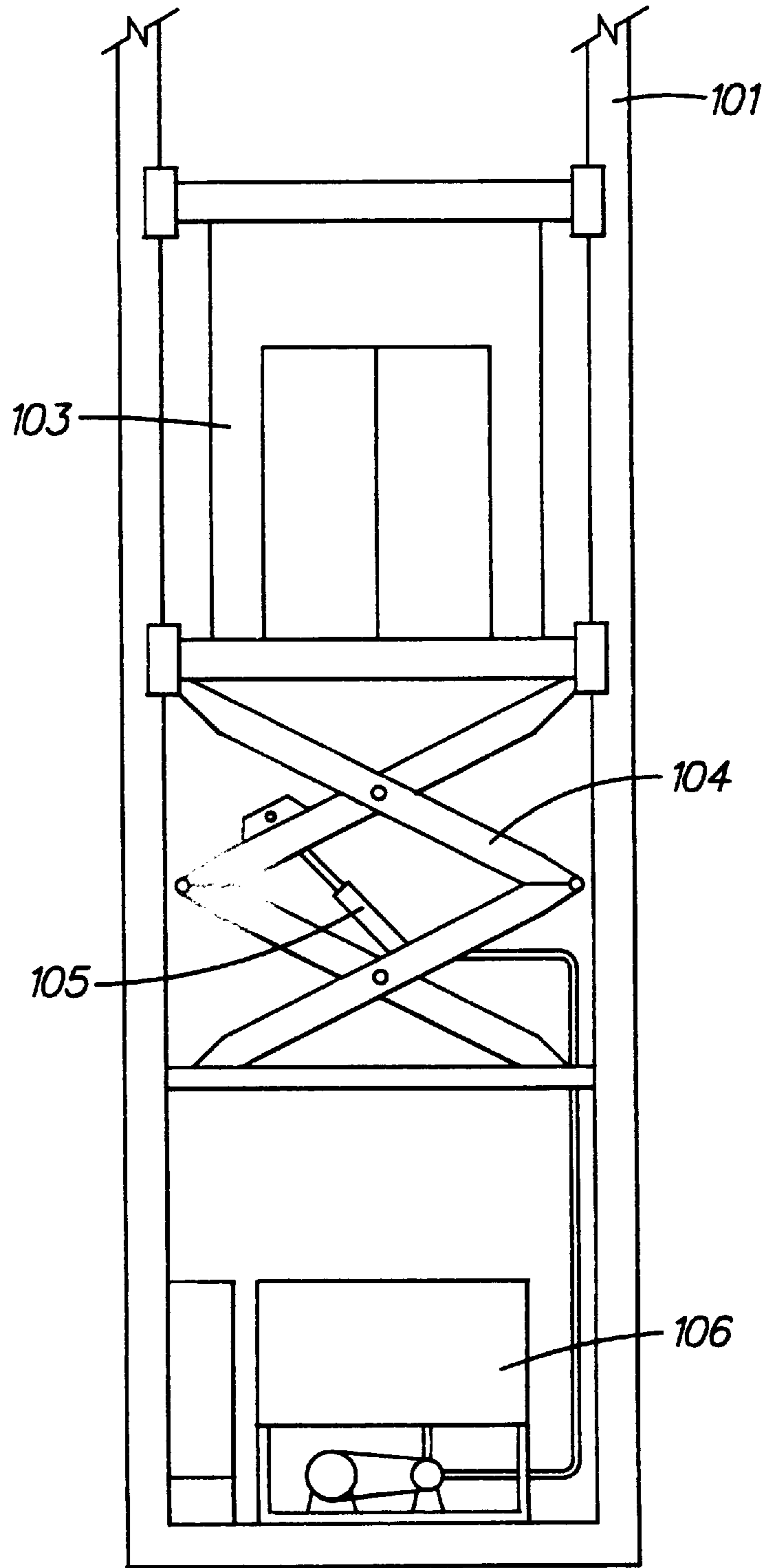
FIG. 9 PRIOR ART
