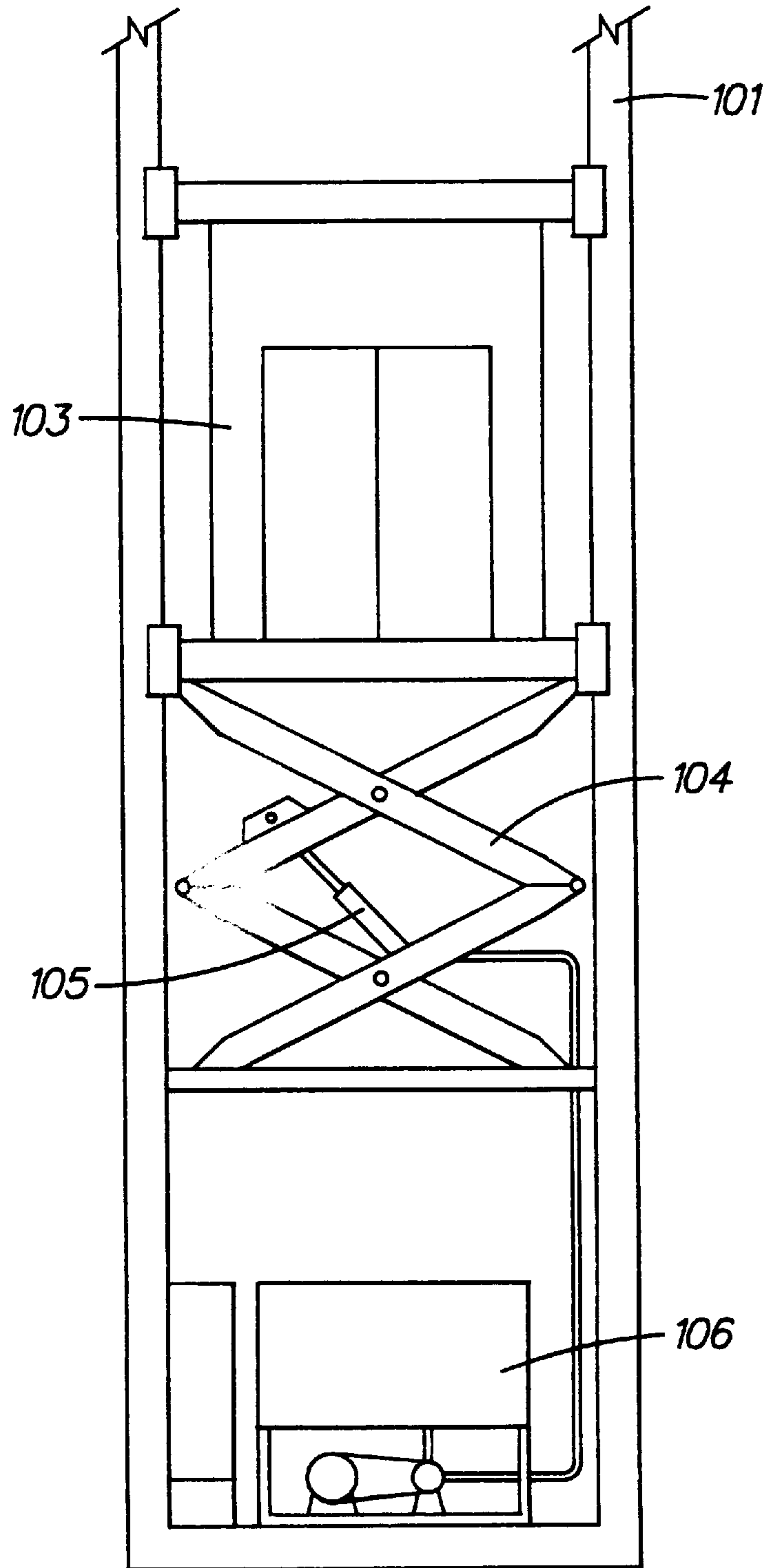
FIG. 9 PRIOR ART
