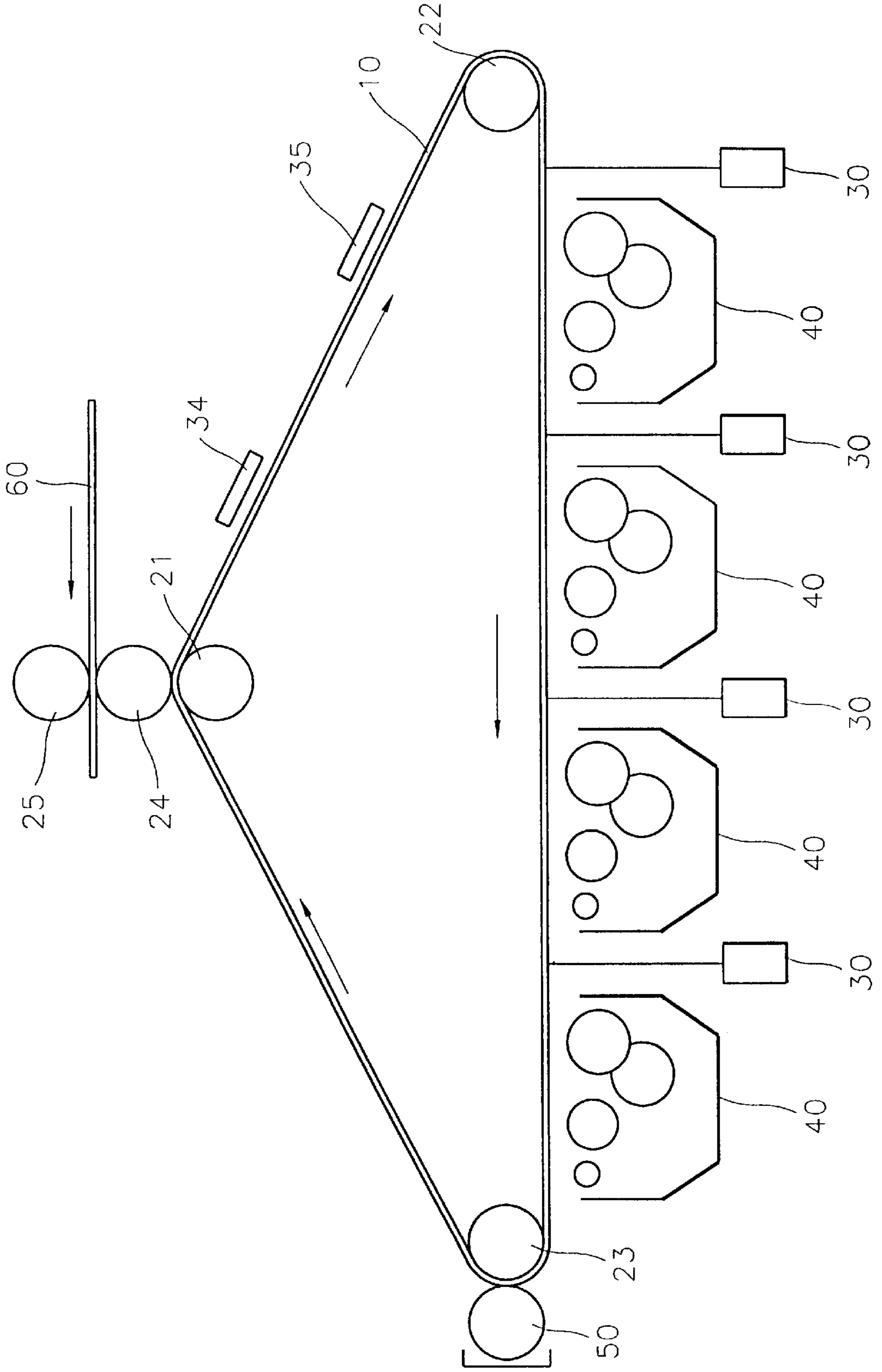
FIG. 1 (PRIOR ART)
