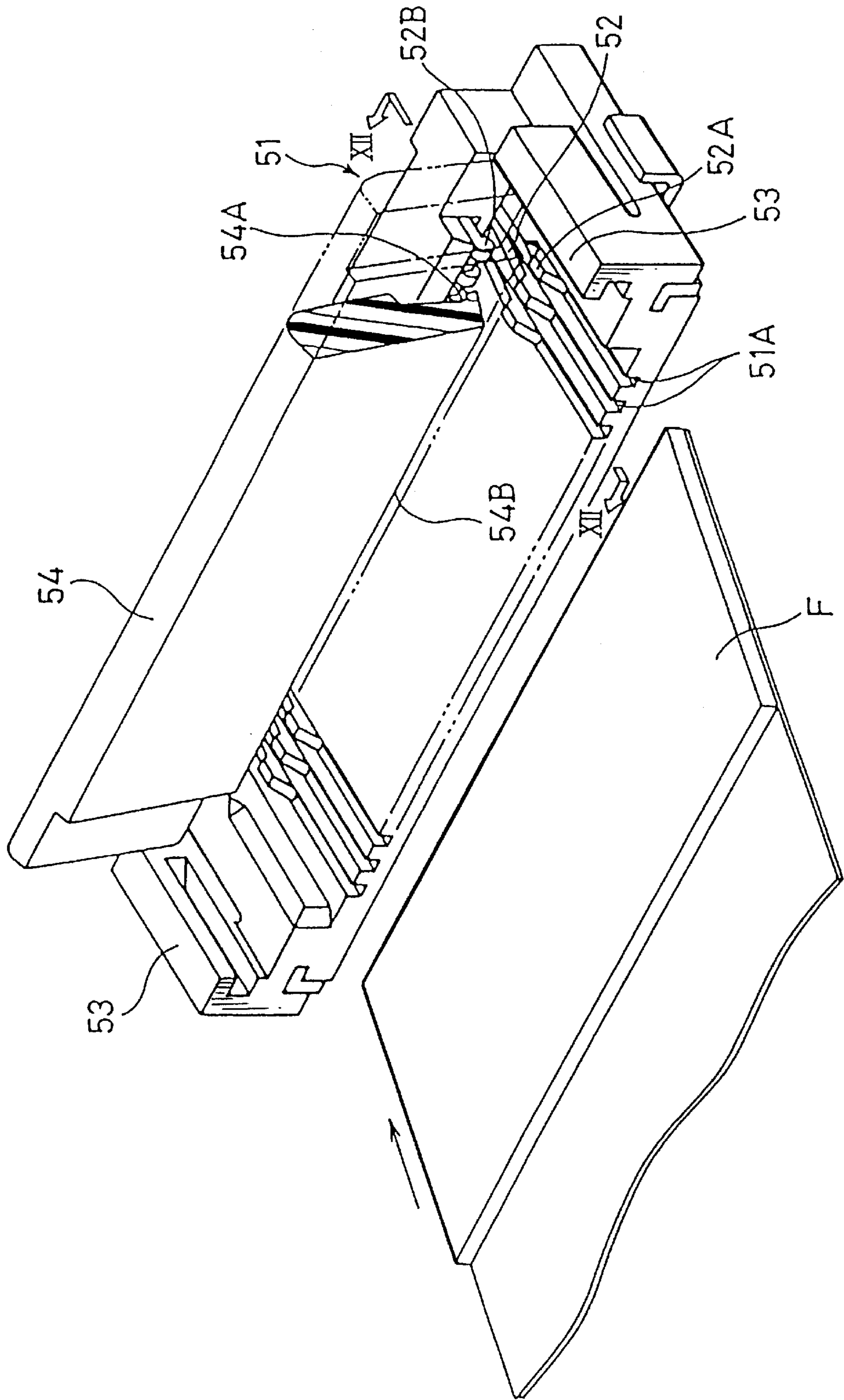
FIG. 11 PRIOR ART
