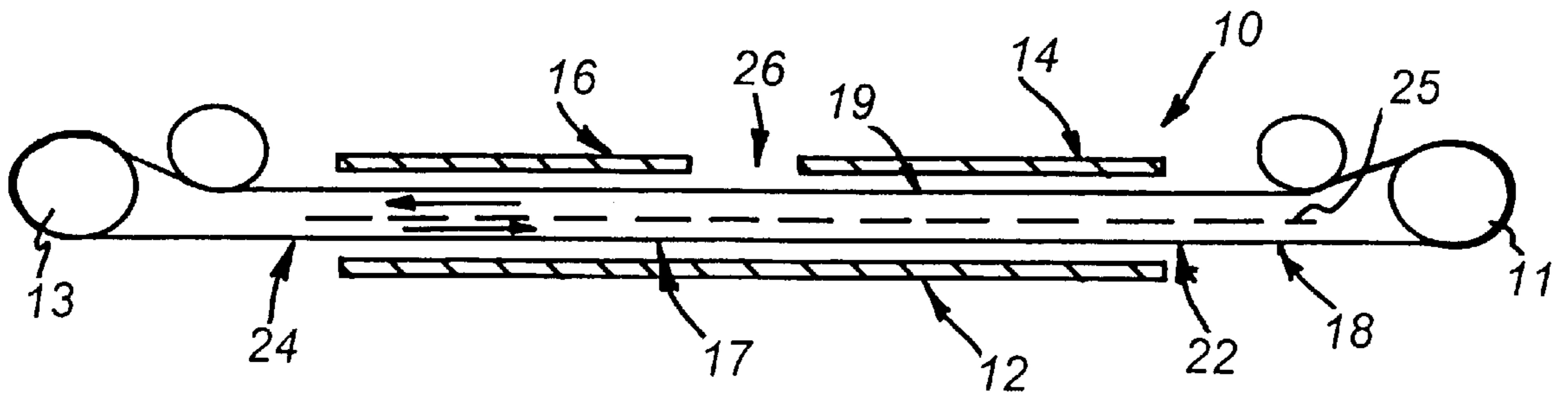
Fig. 1 (PRIOR ART)
