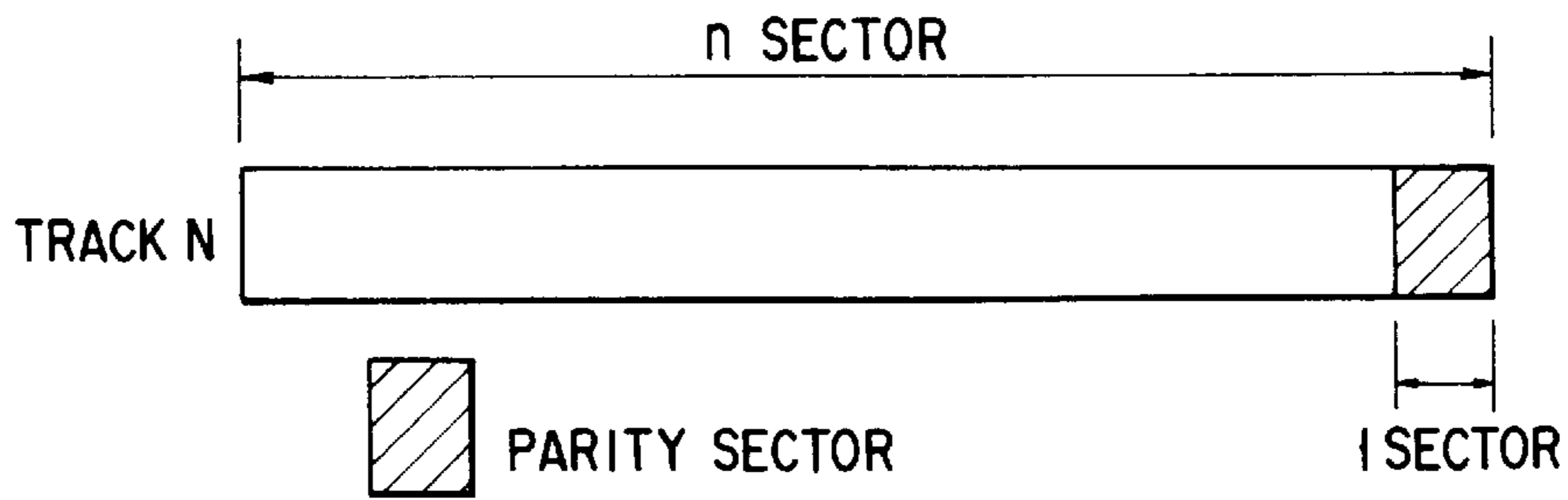
FIG. 2 (PRIOR ART)
