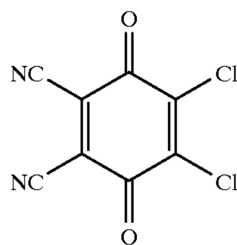
2,3-dichloro-5,6-dicyano-p-benzoquinone
