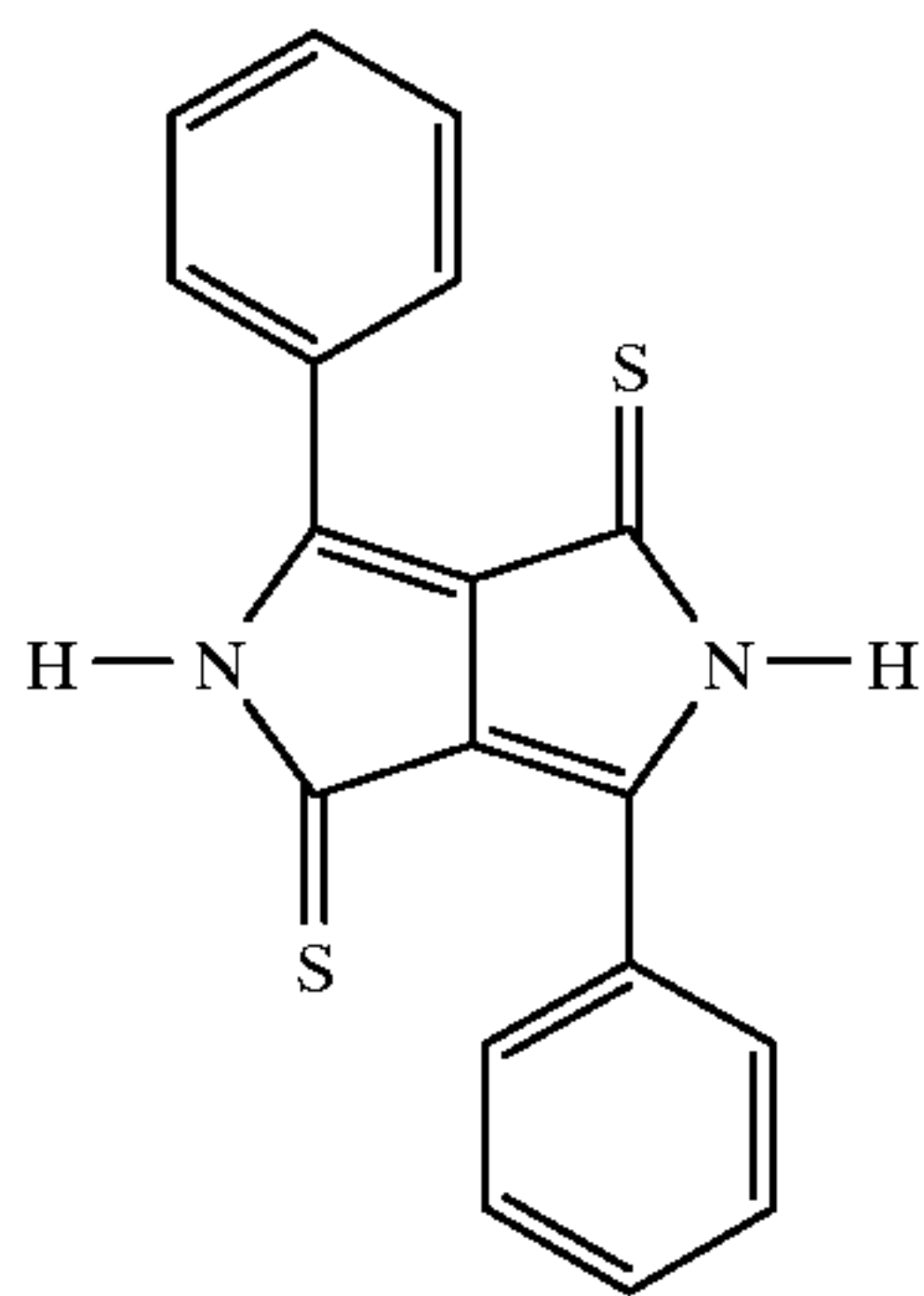
Pyrrolopyrrole Pigment
