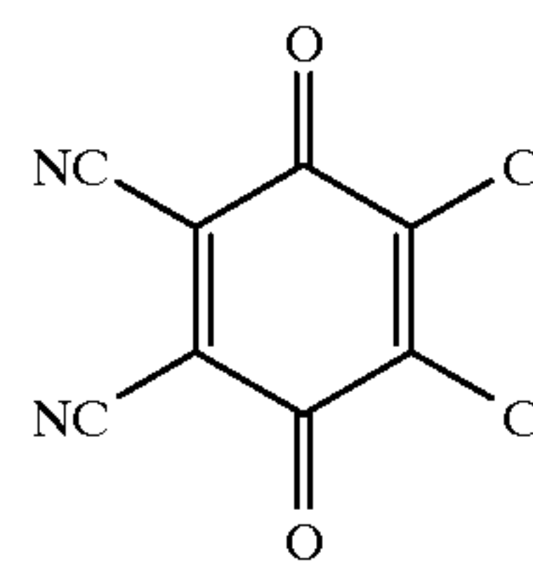
2,3-dichloro-5,6-dicyano-p-benzoquinone
