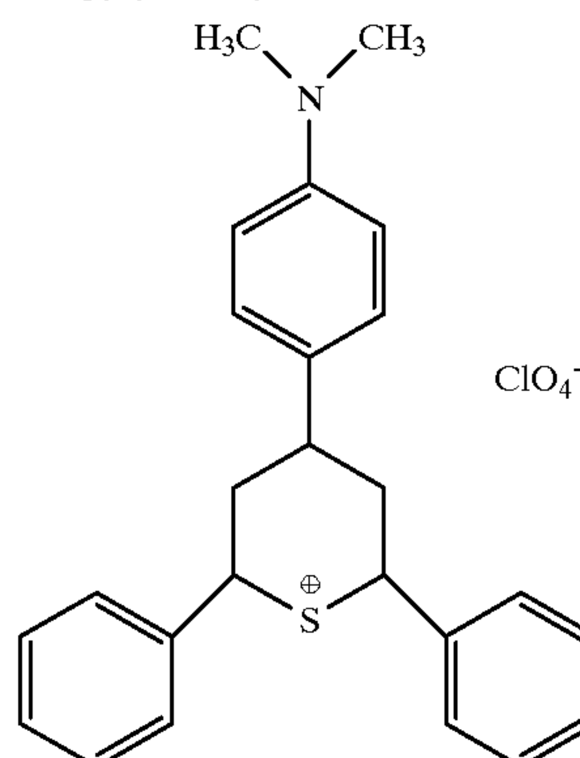
② Thiapyrylium dye
