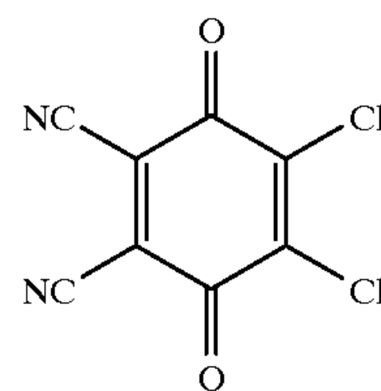
2,3-dichloro-5,6-dicyano-p-benzoquinone
