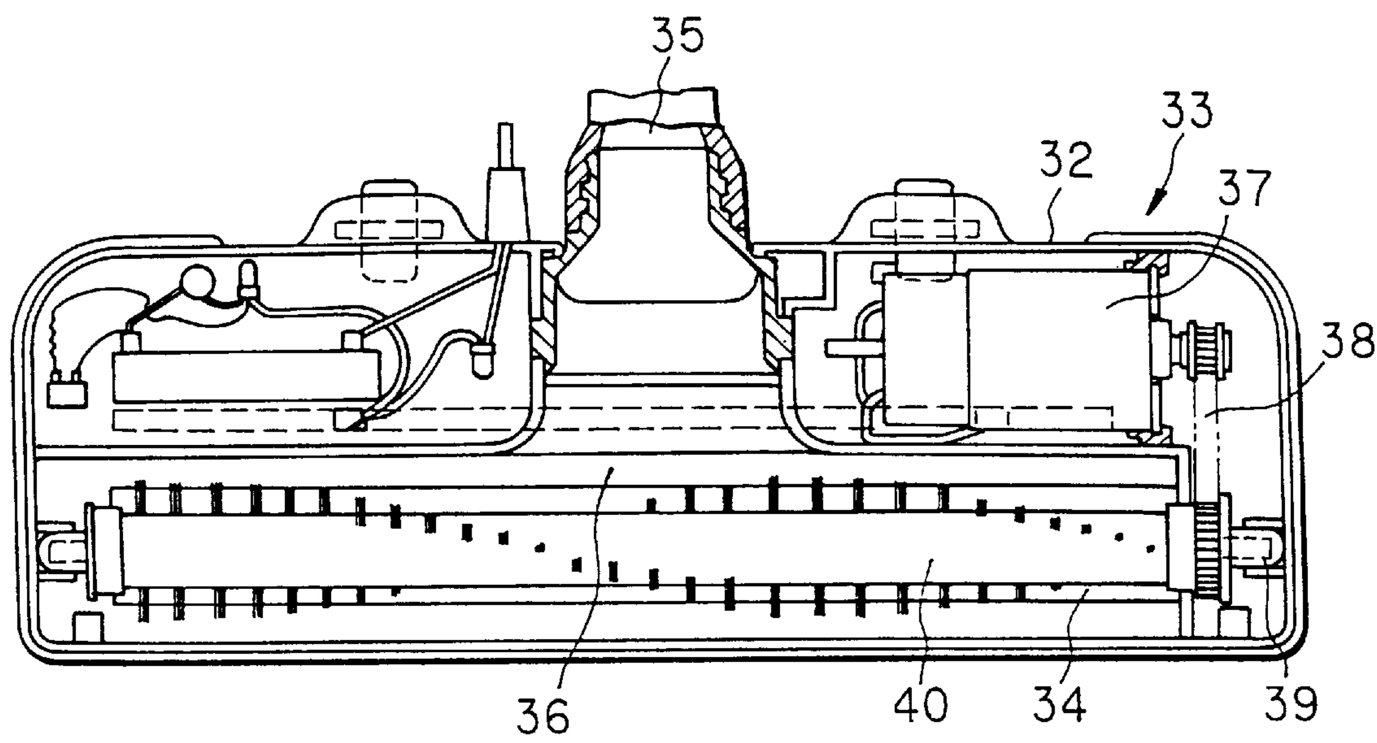
FIG. 1 PRIOR ART
