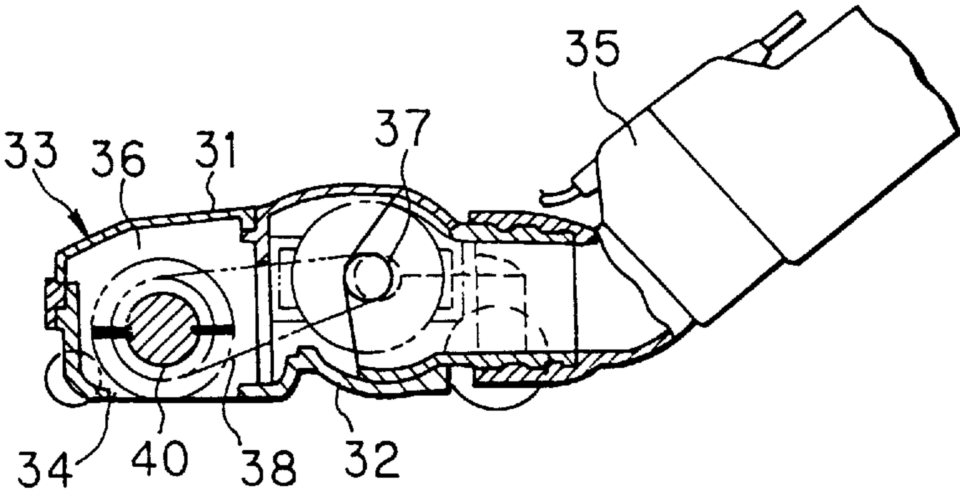
FIG. 2 PRIOR ART
