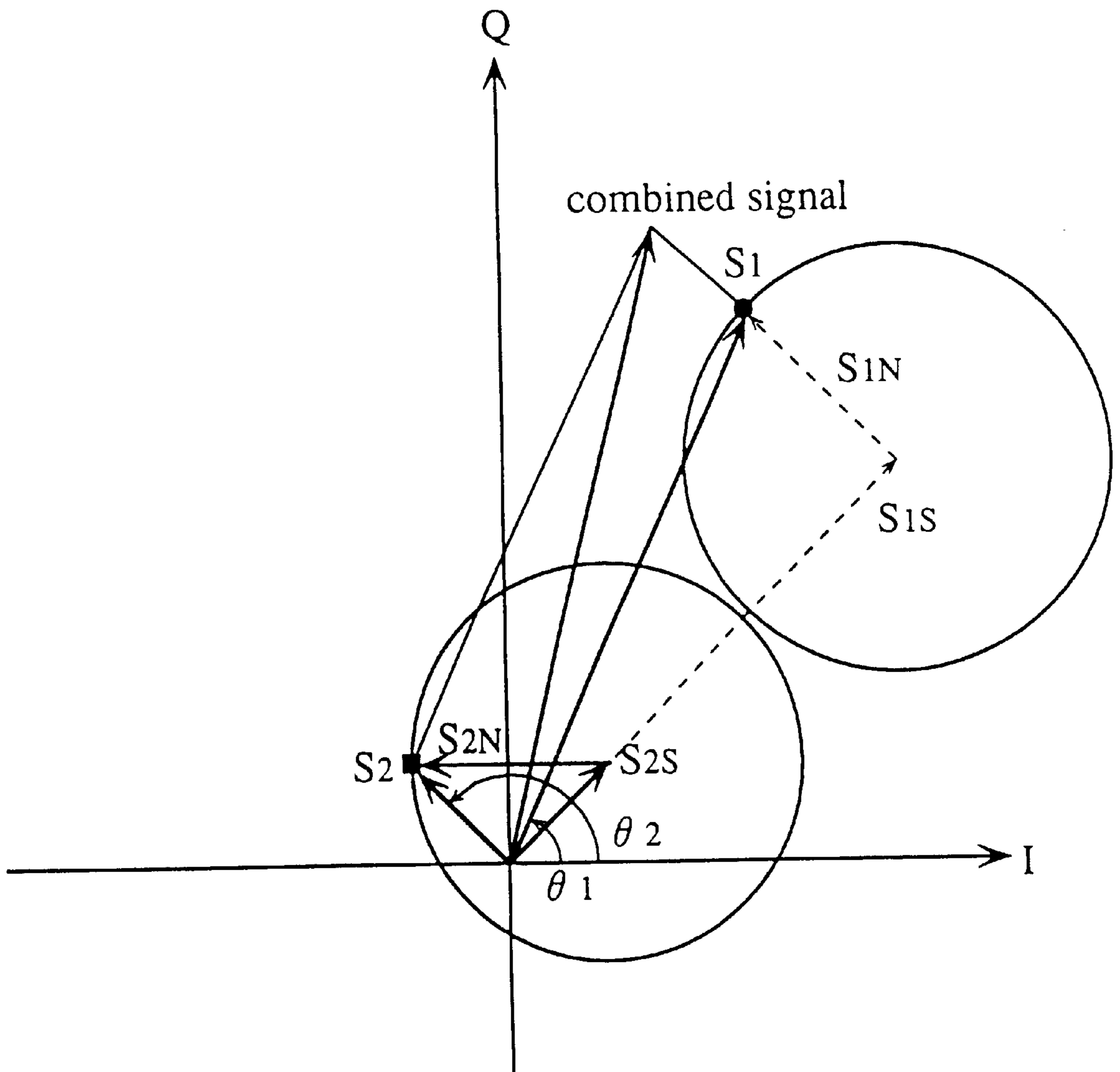
Fig. 2 ( PRIOR ART )
