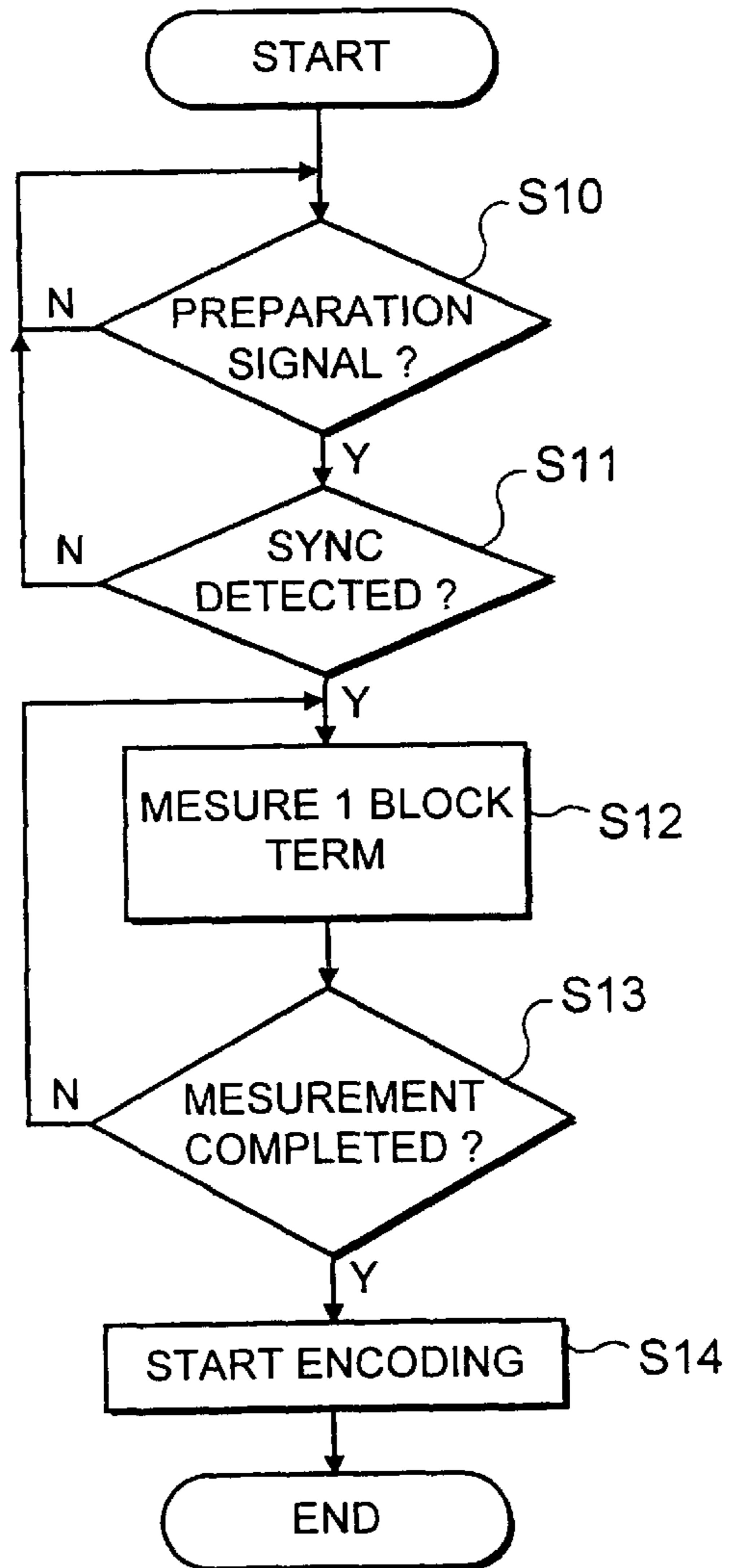
OPERATION AT 8 - 16 ENCODER
