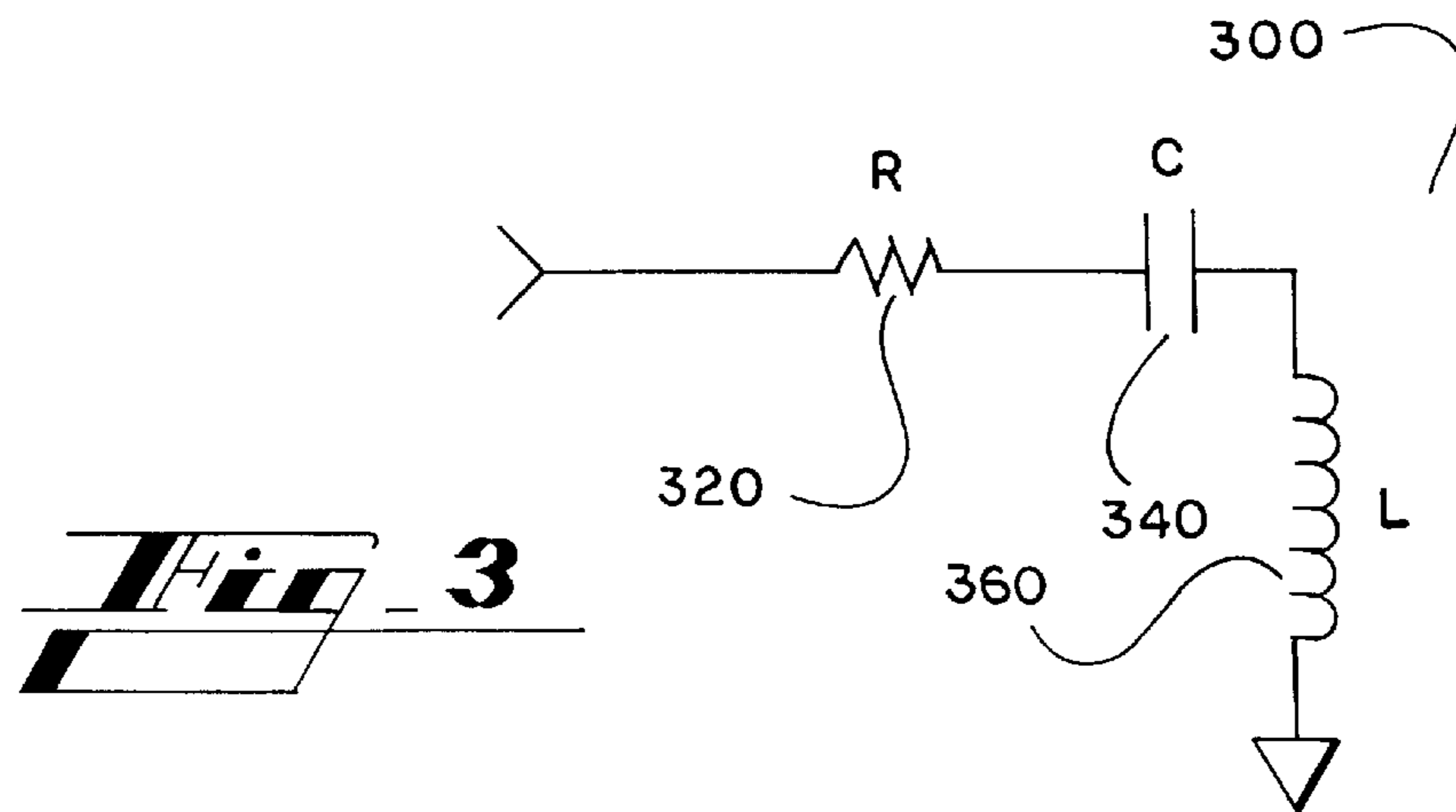
TRANSDUCER EQUIVALENT CIRCUIT
