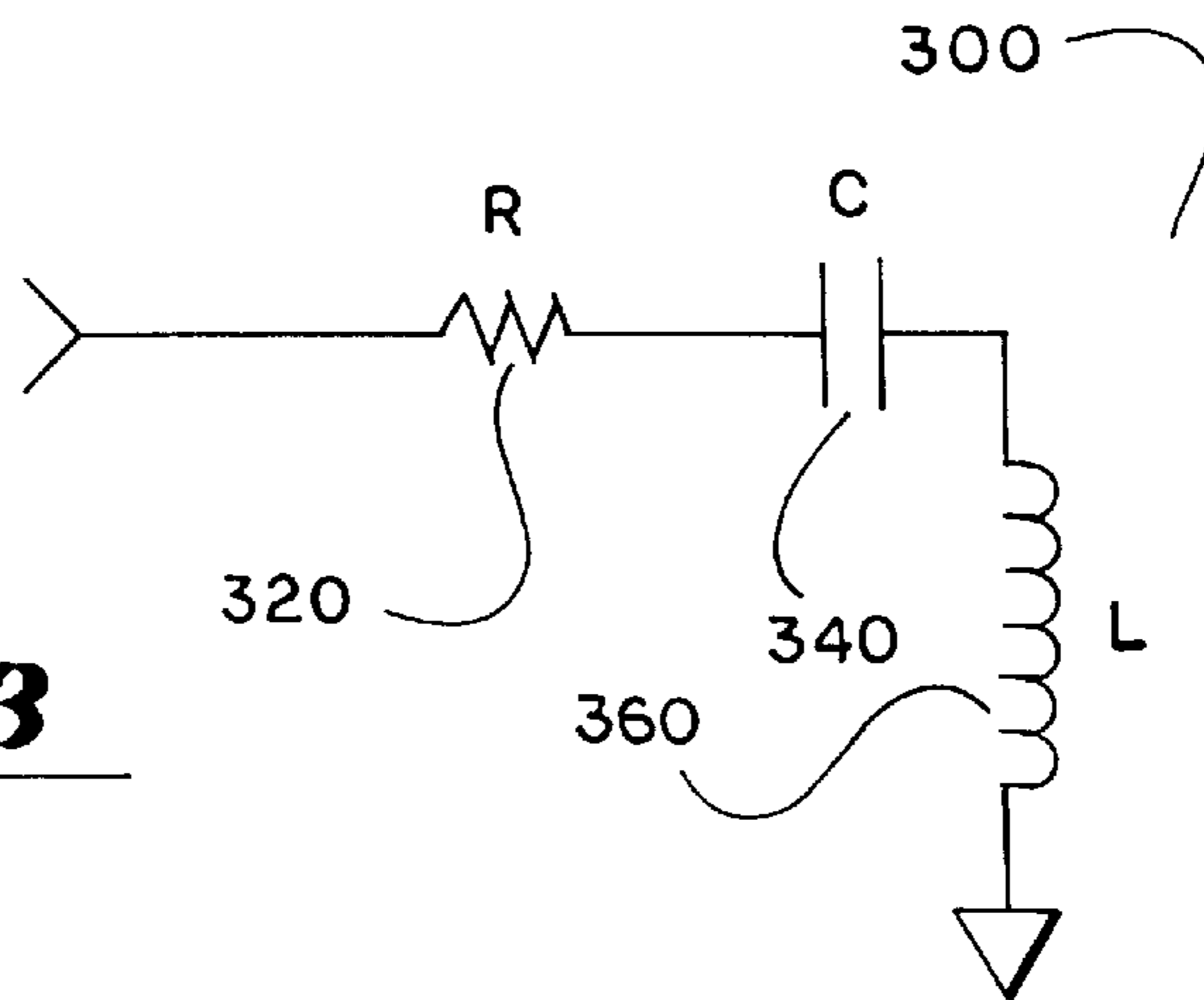
TRANSDUCER EQUIVALENT CIRCUIT
