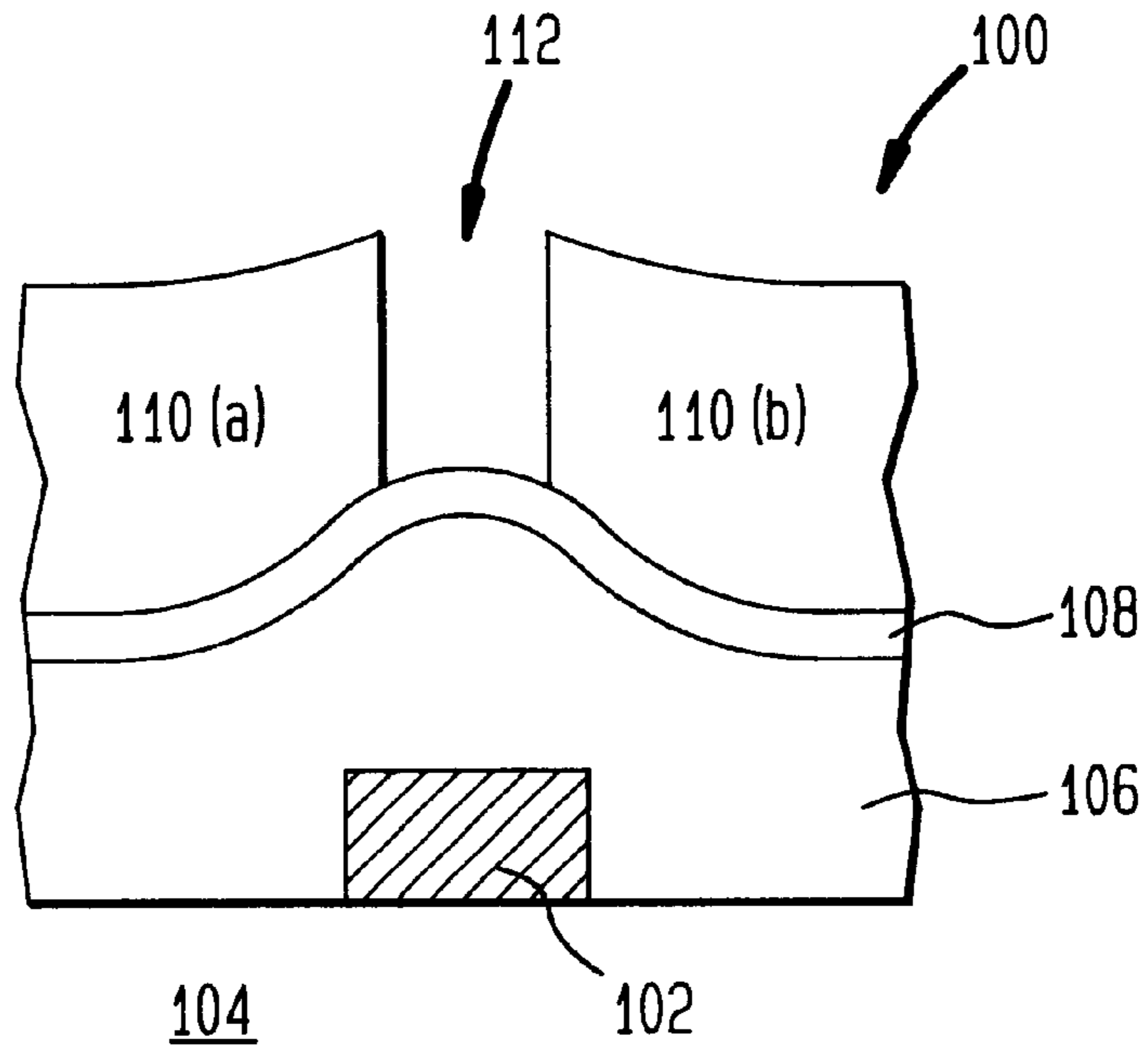
FIG. 1 (PRIOR ART)
