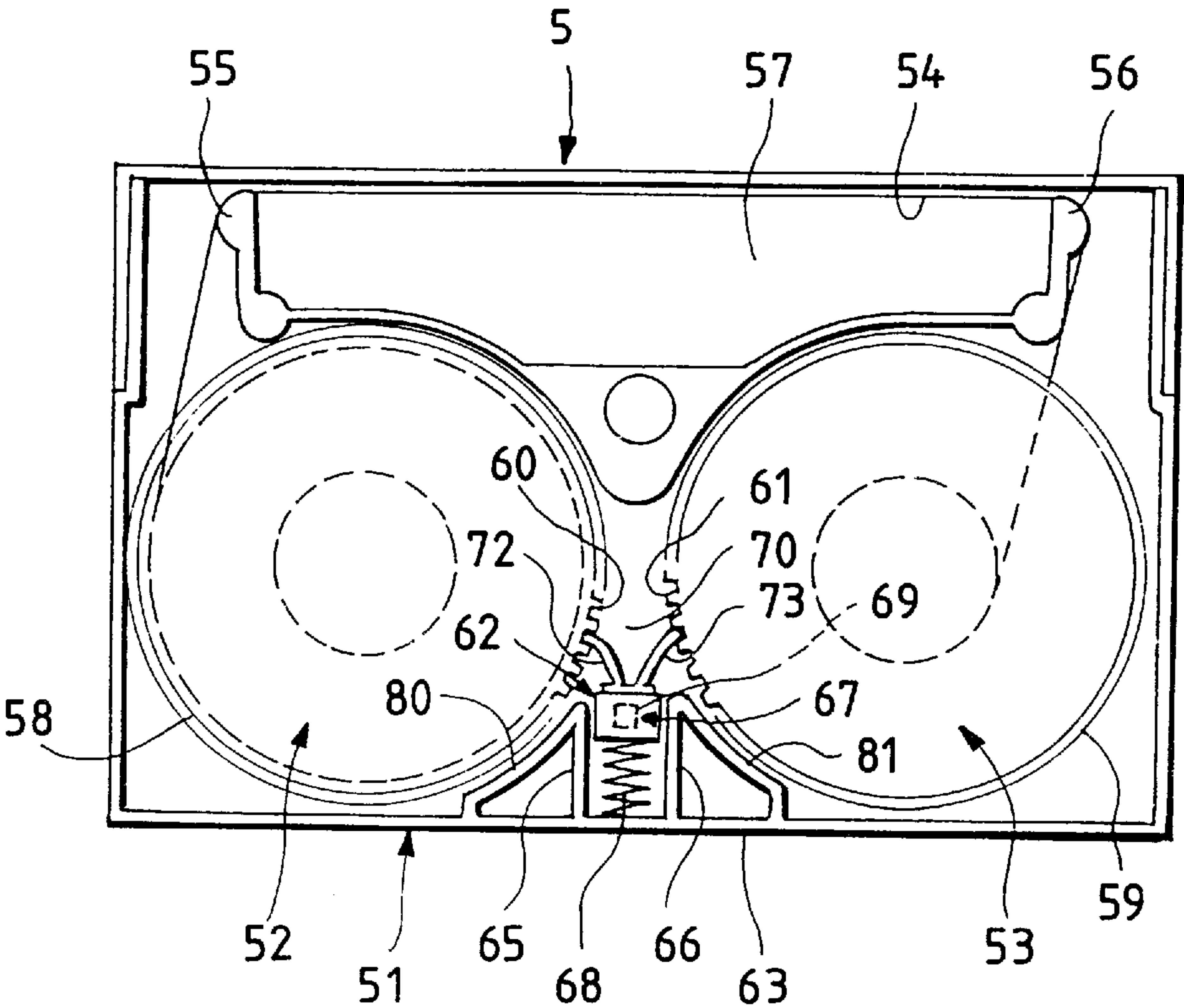
FIG. 1 PRIOR ART
