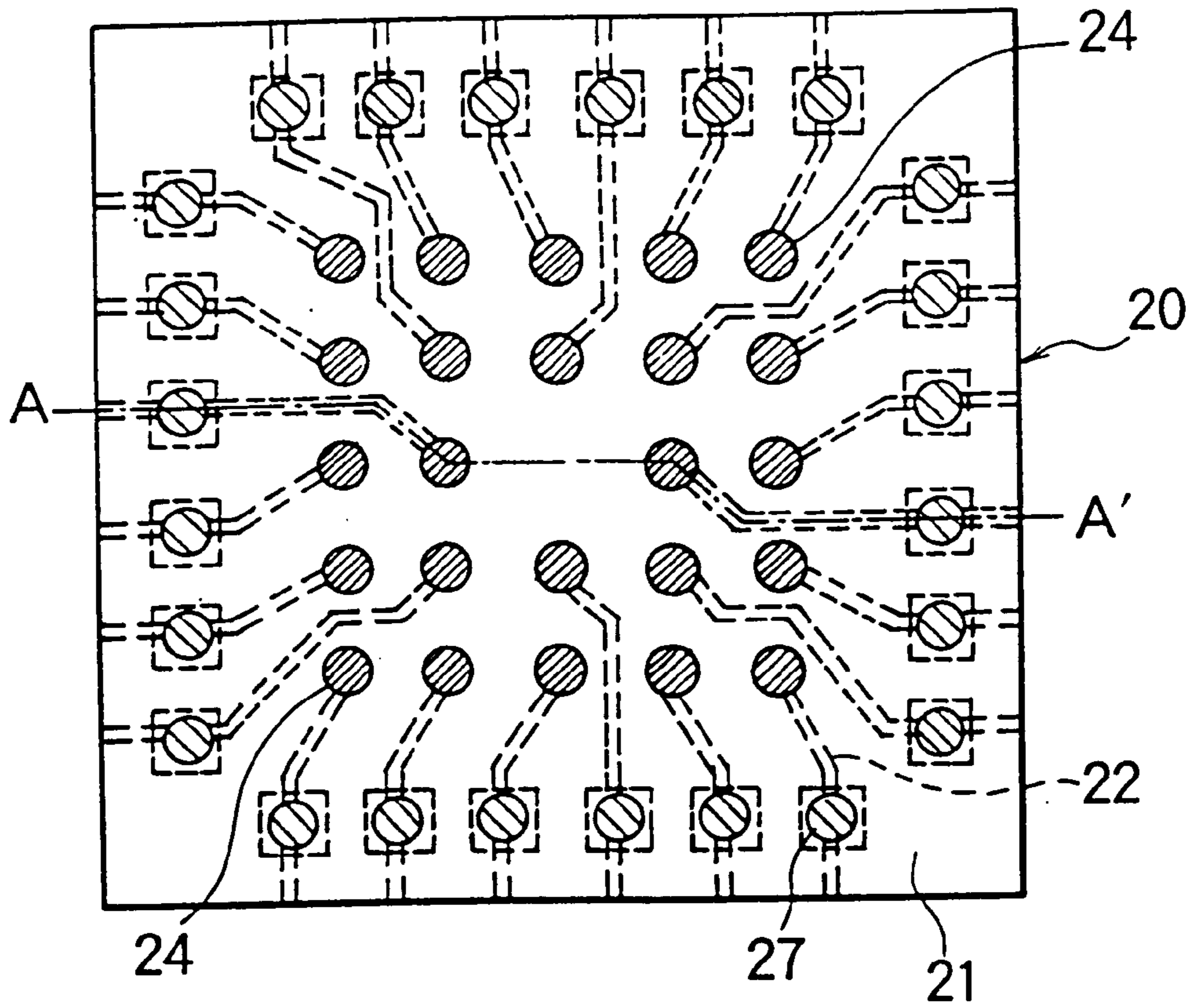
FIG. 1 PRIOR ART
