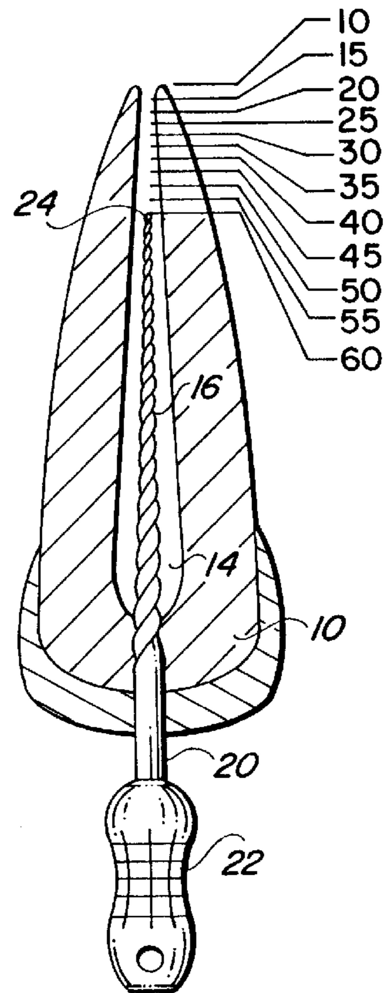
FIG. 2 (PRIOR ART)
