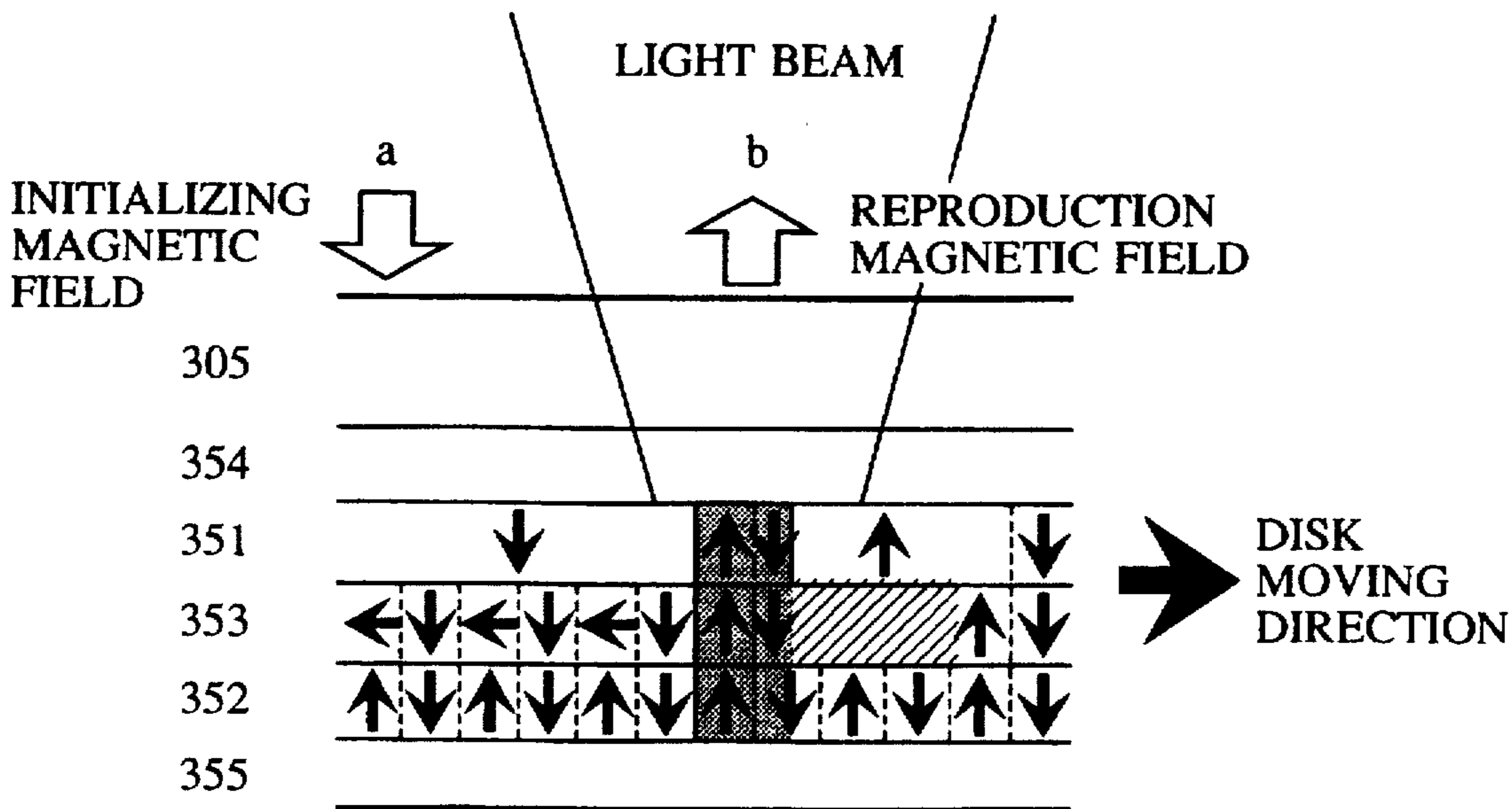
FIG. 15(b) CONVENTIONAL ART
