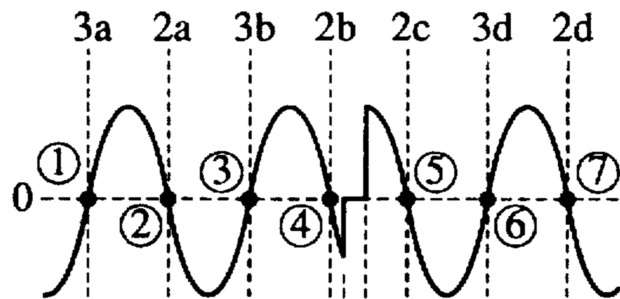
FIG. 6(b)(1) TRACKING ERROR SIGNAL (a)
