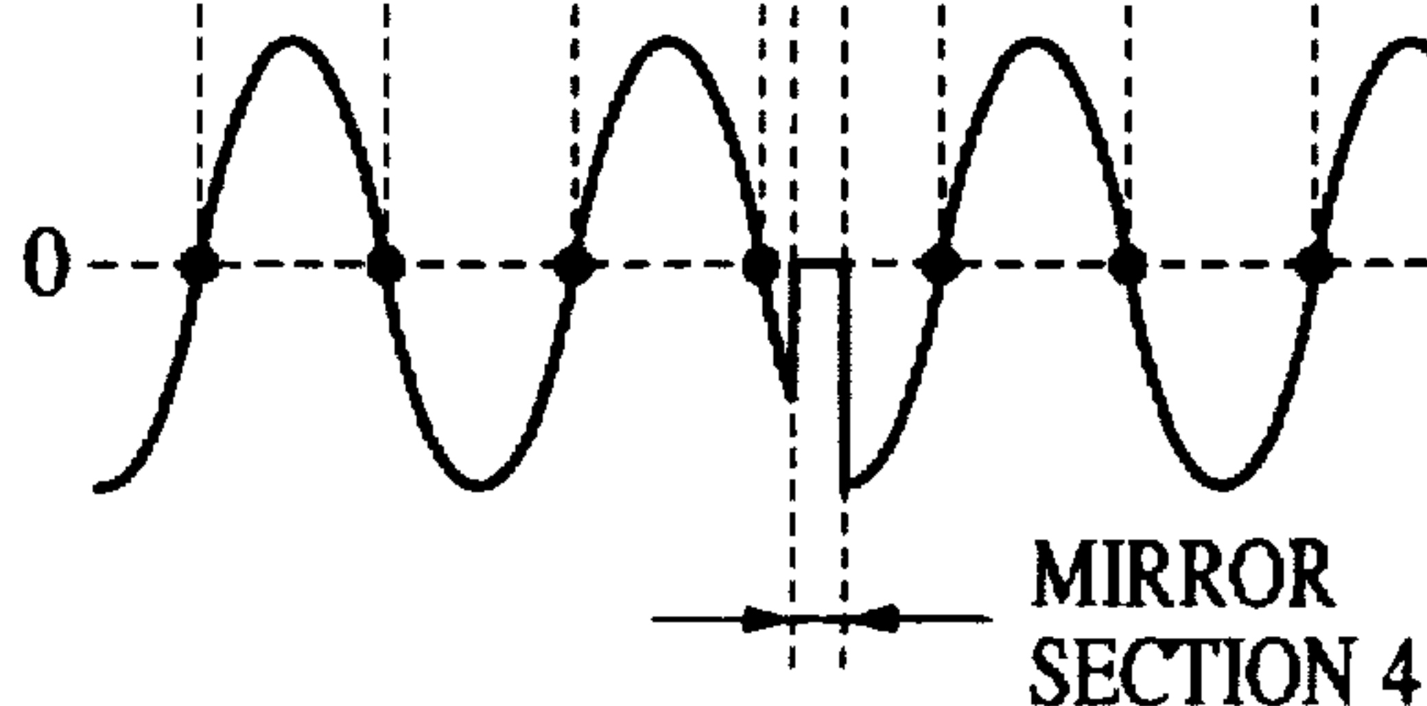
FIG. 6(b)(6) TRACKING ERROR SIGNAL (f)
