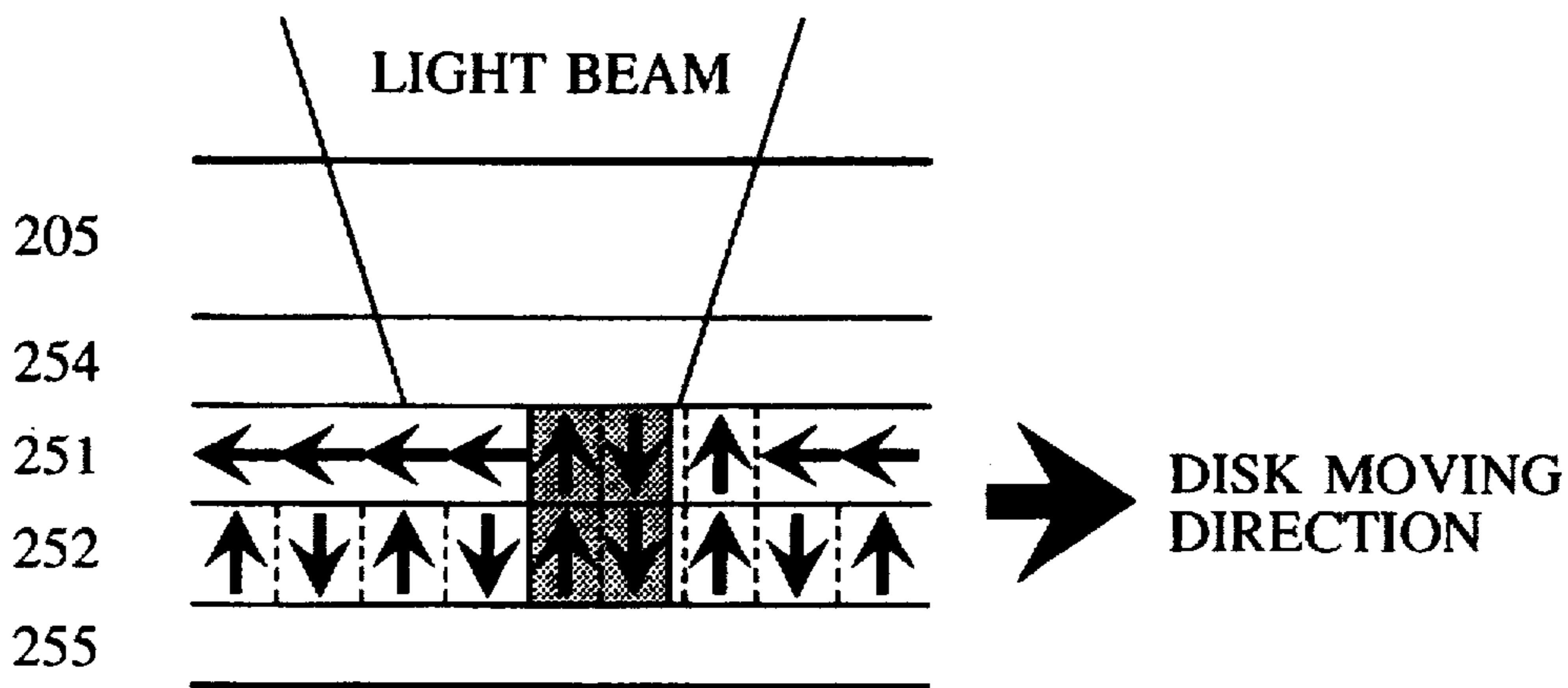
FIG. 14(a) CONVENTIONAL ART
