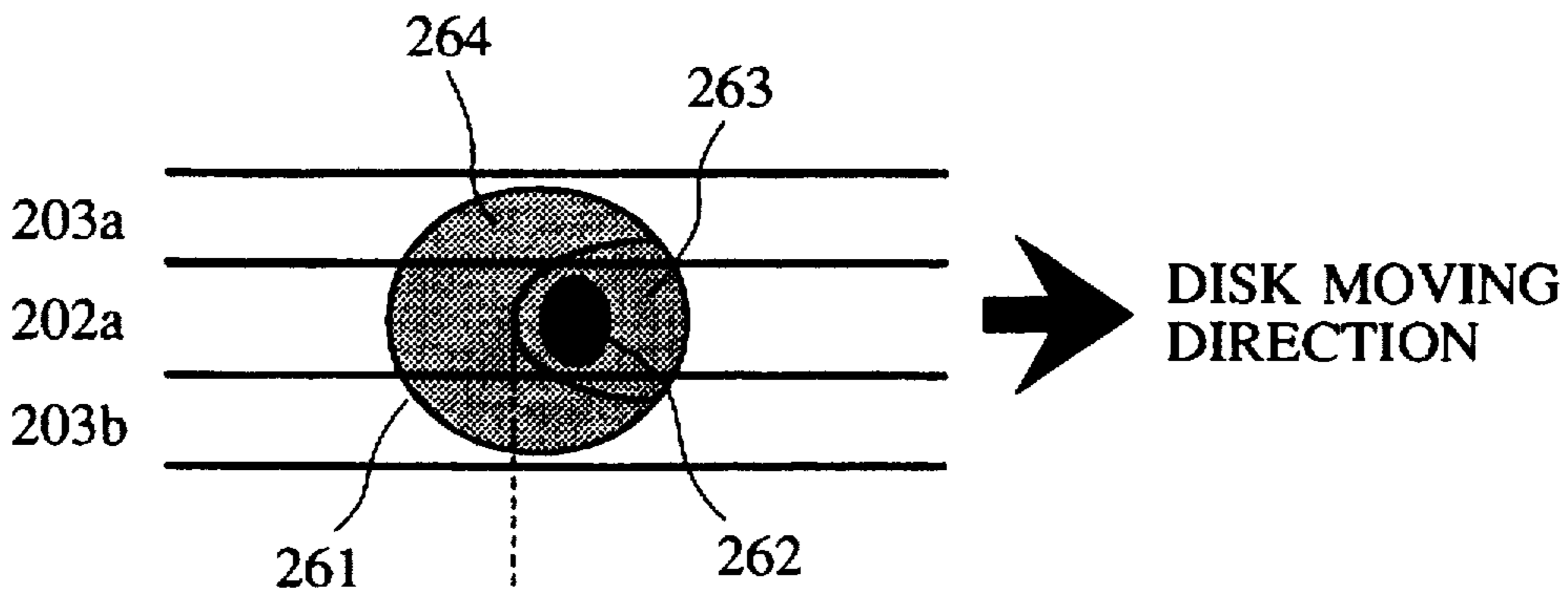
FIG. 14(b) CONVENTIONAL ART
