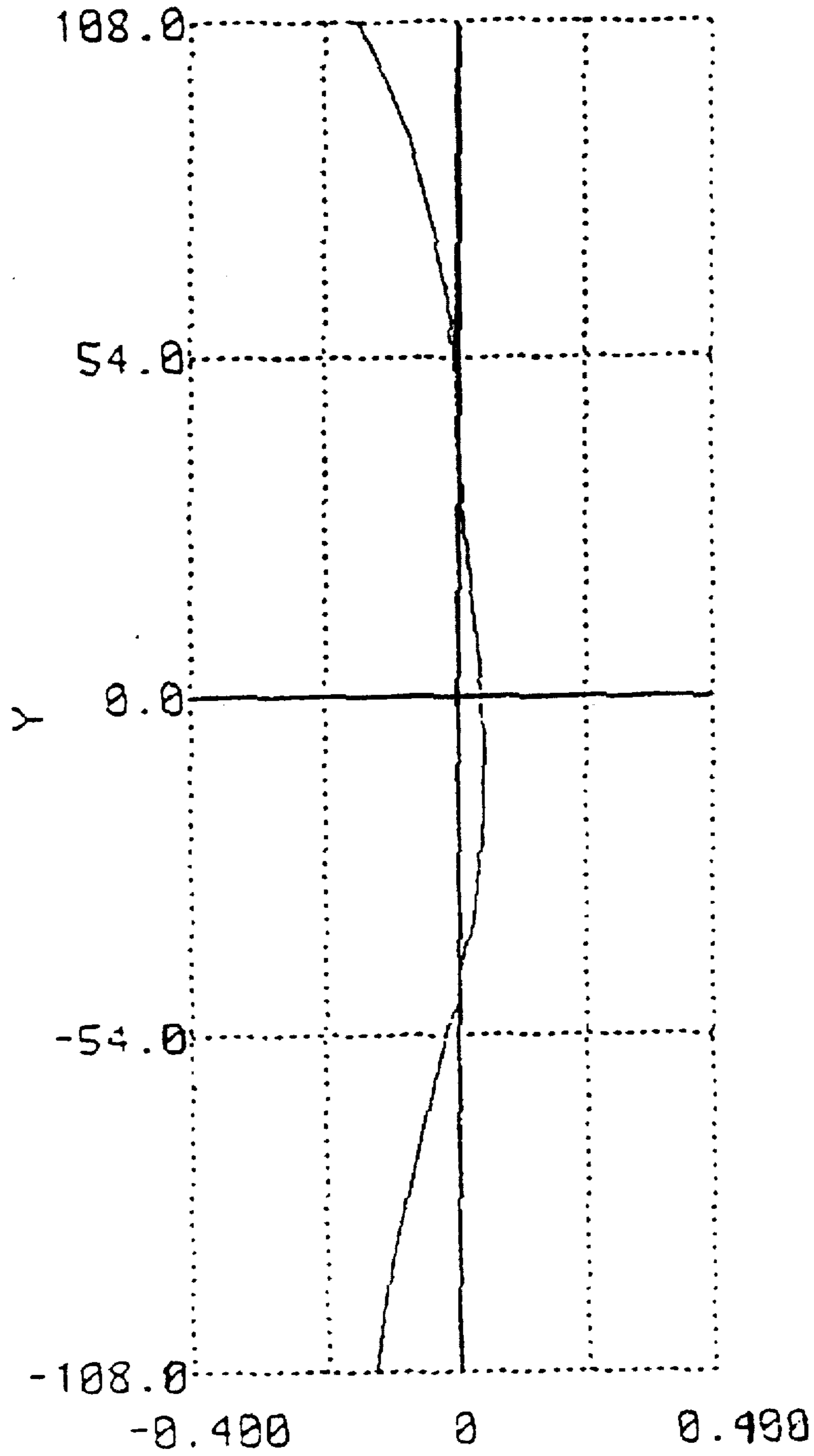
f\theta characteristic.
