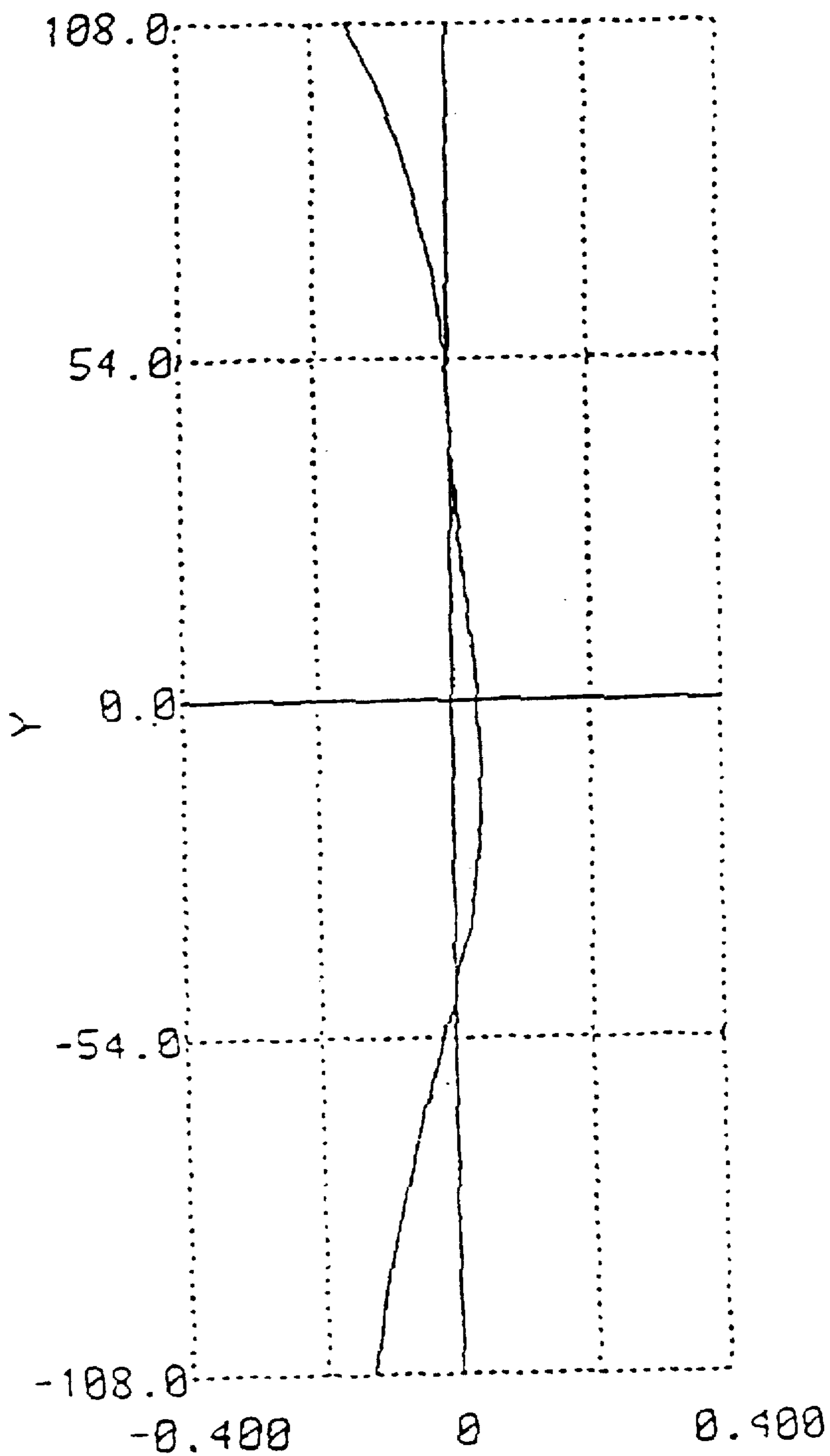
f\theta characteristic
