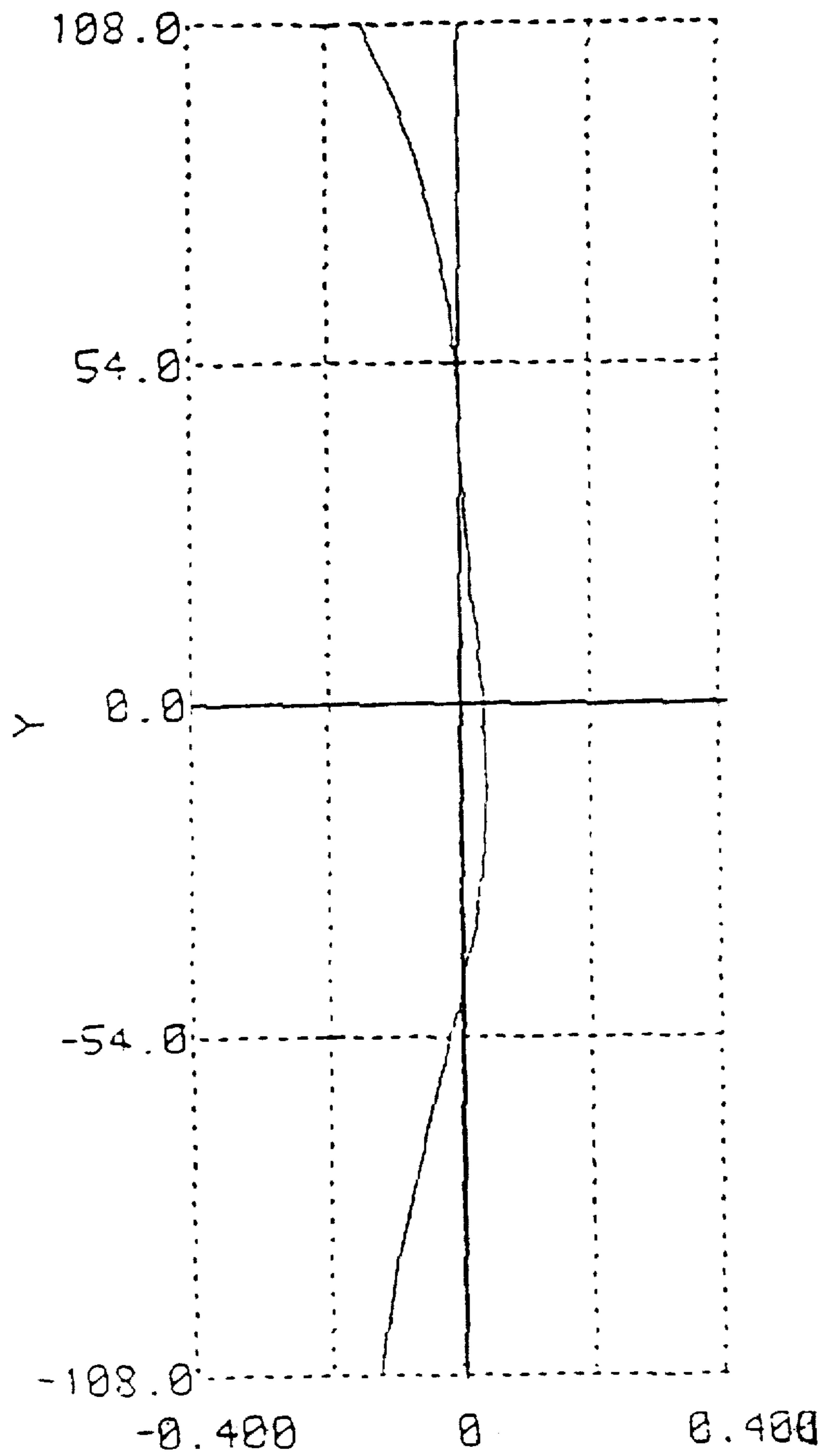
f\theta characteristic
