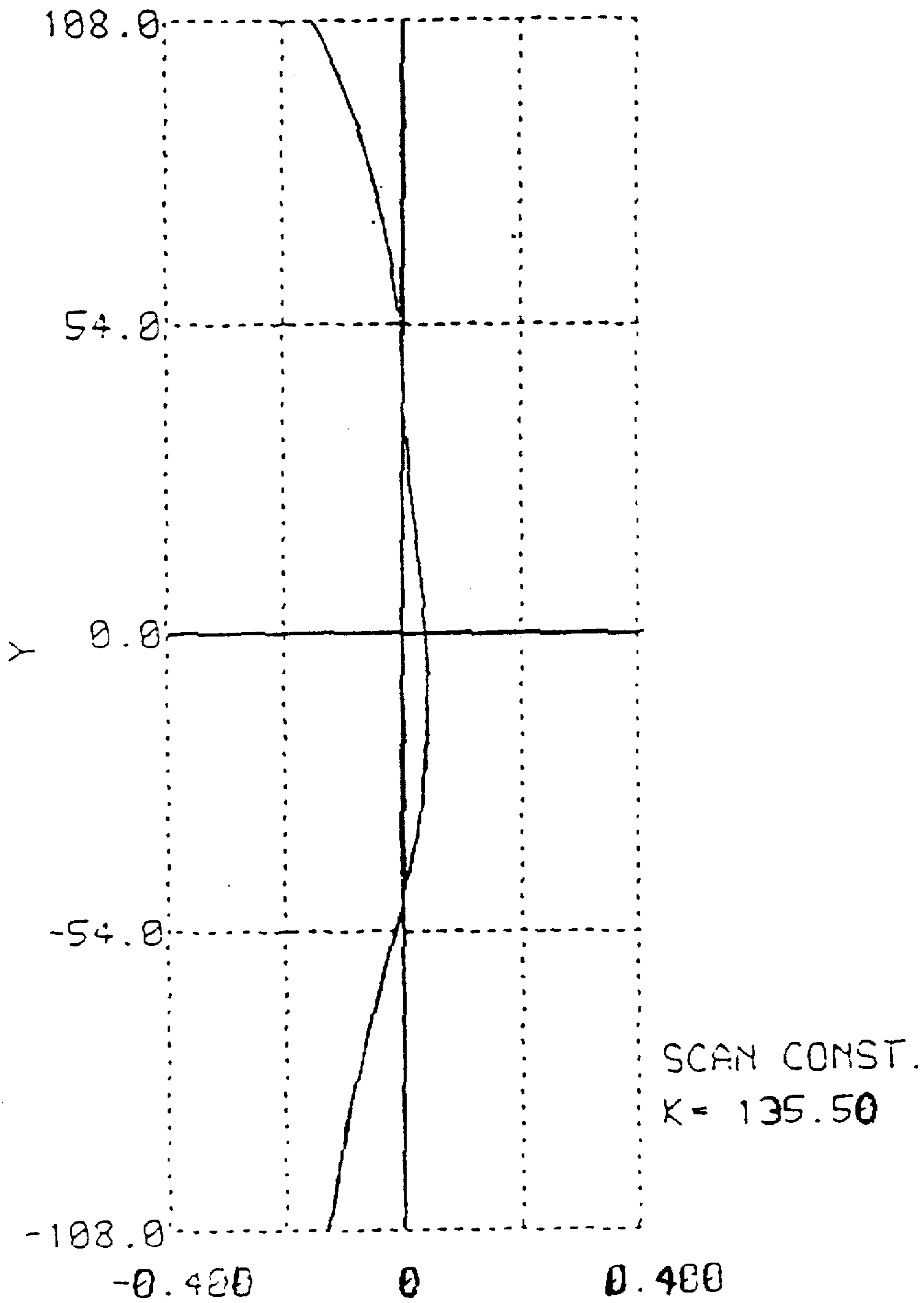
f\theta characteristic
