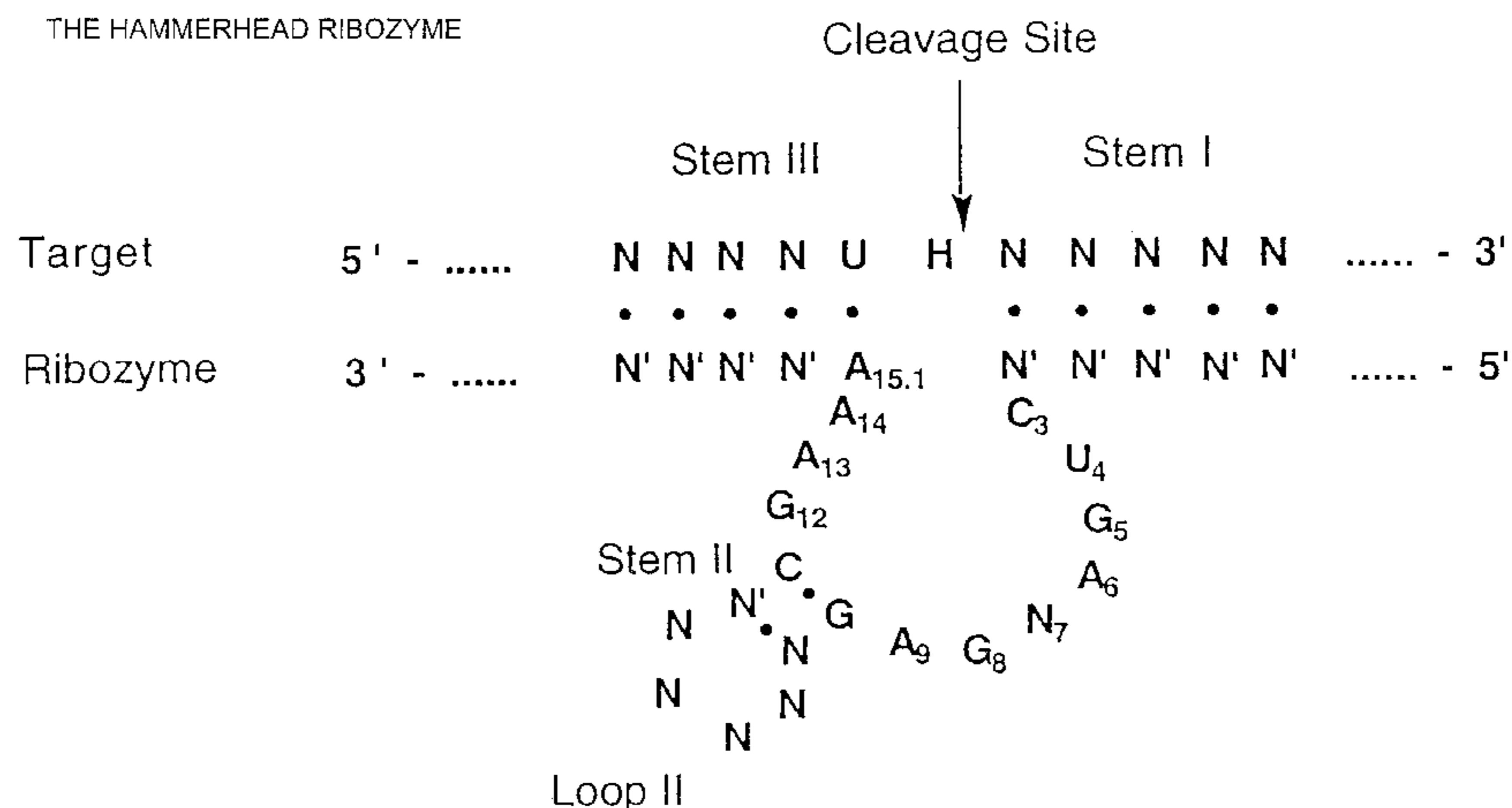
THE HAMMERHEAD RIBOZYME
