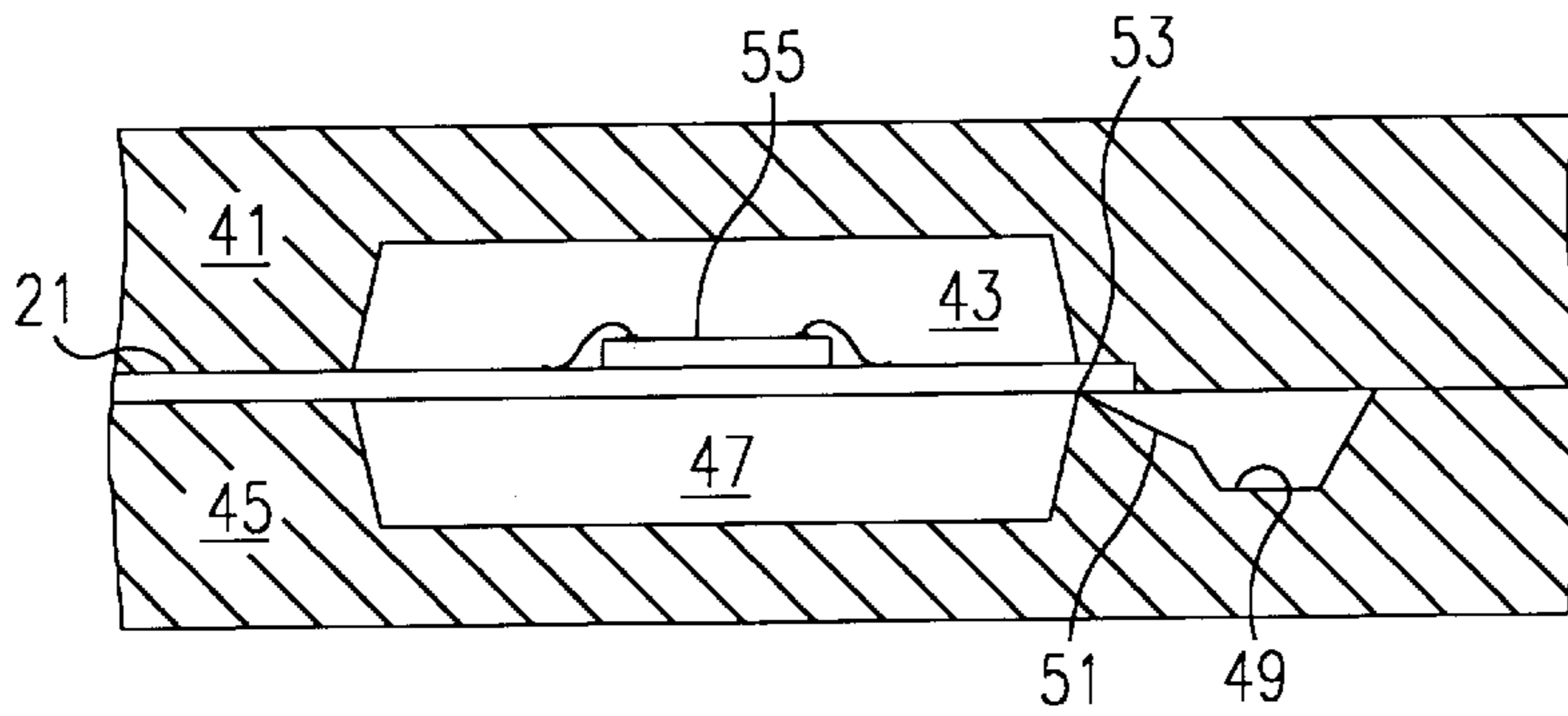
FIG. 2 (PRIOR ART)
