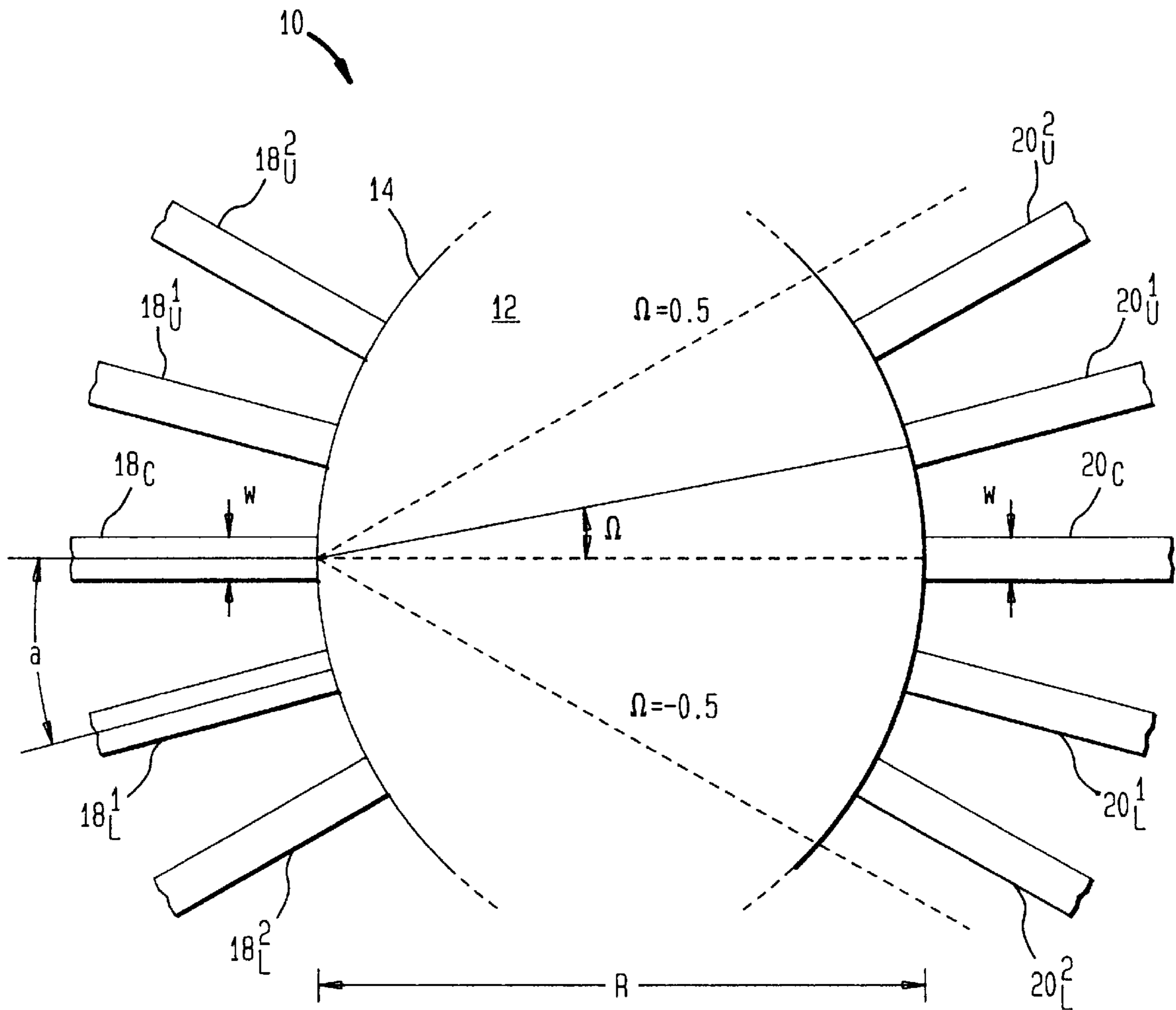
FIG. 1 (PRIOR ART)
