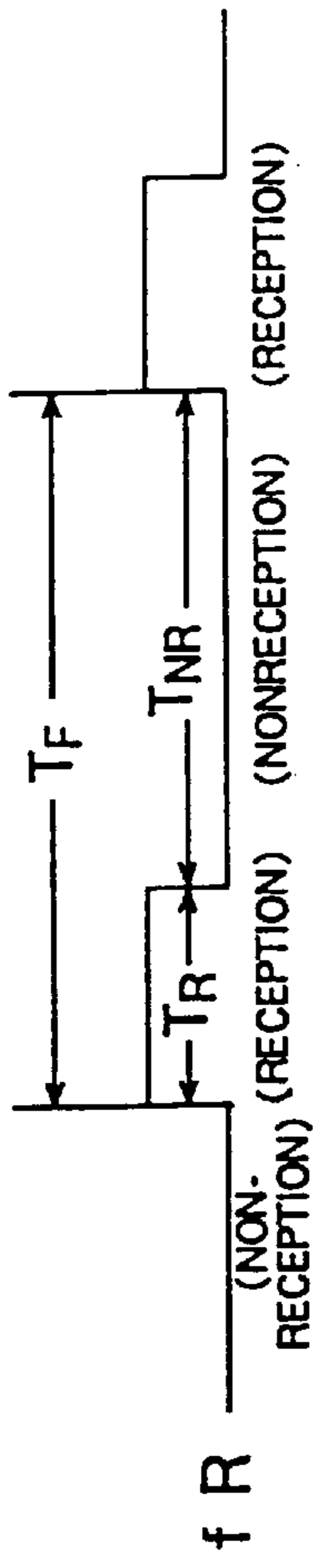
FIG. 4A RECEIVED CARRIER (INTERMITTENT RECEPTION)
