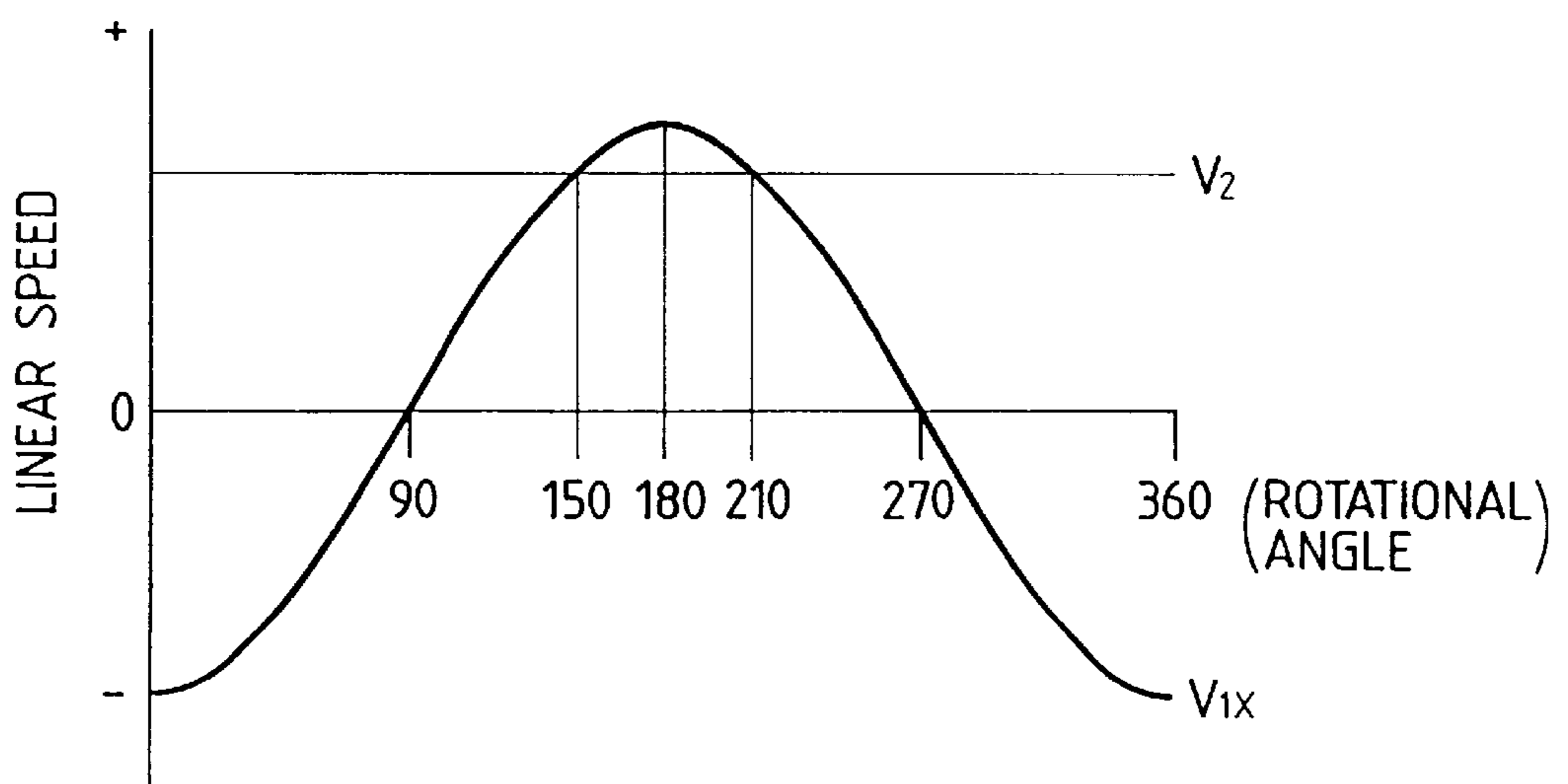
FIG. 23 PRIOR ART
