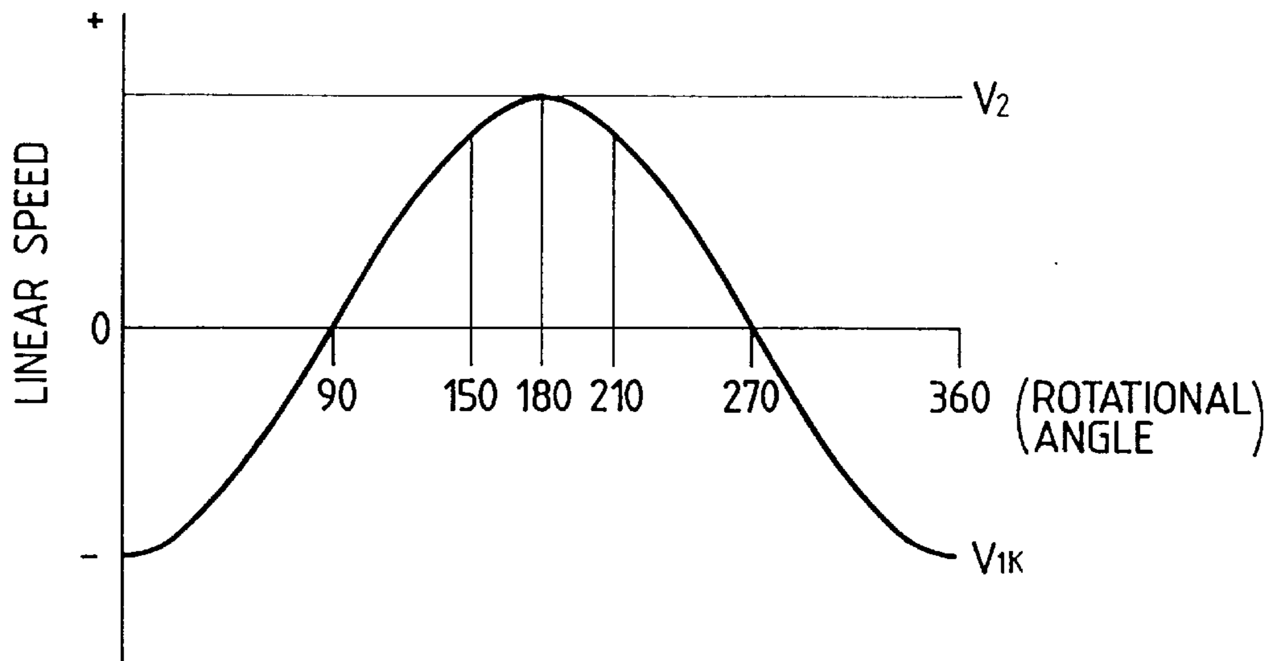
FIG. 22 PRIOR ART
