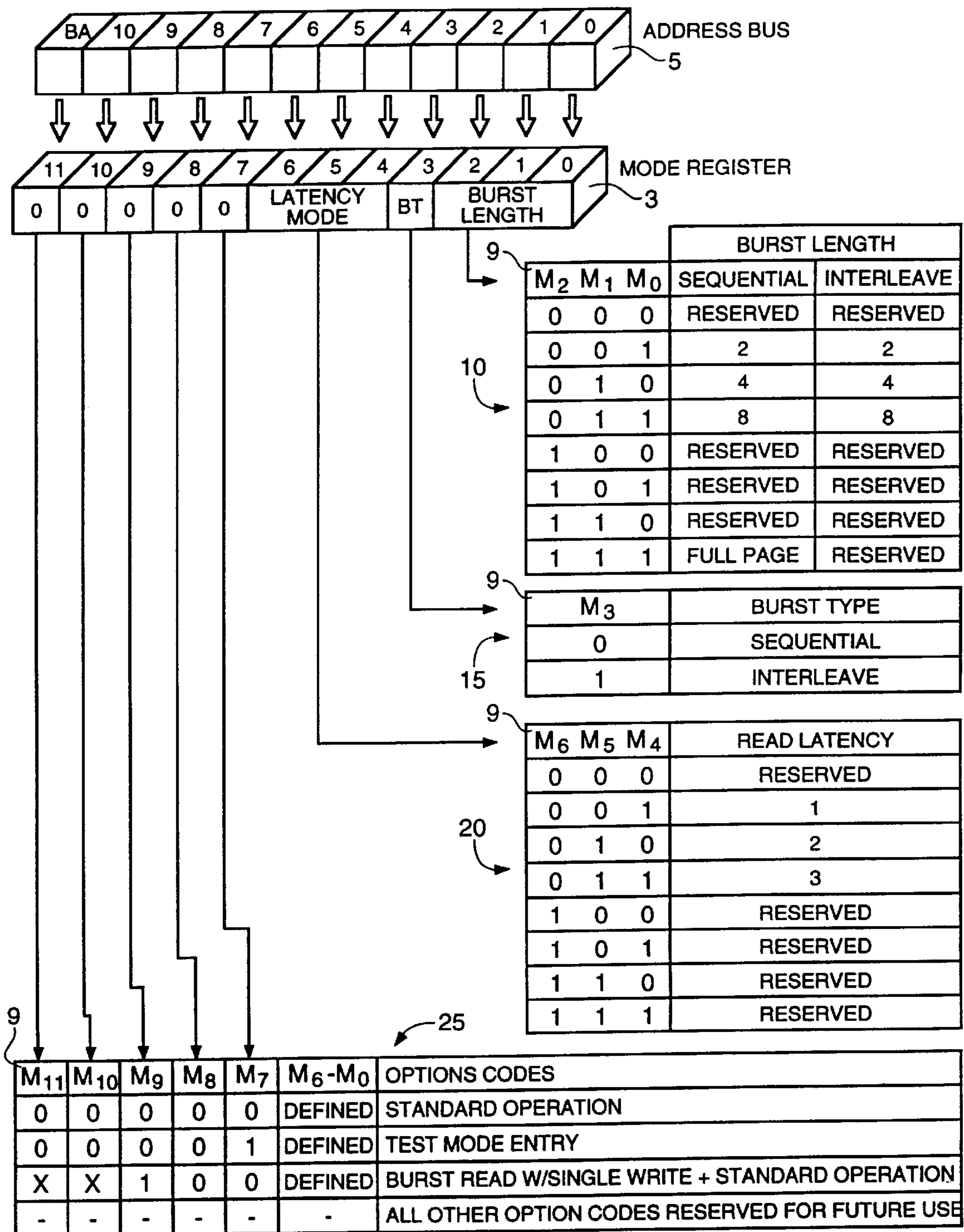
FIG. 2 (RELATED ART)
