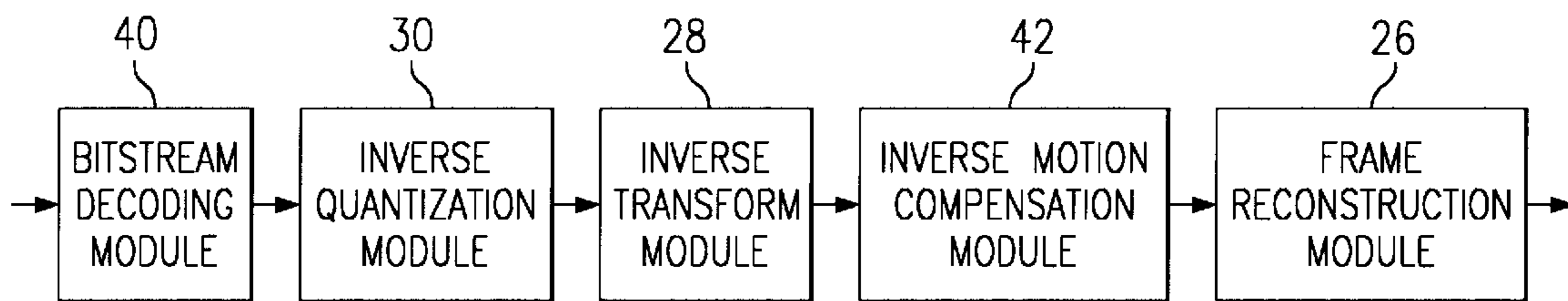
FIG. 2 (PRIOR ART)
