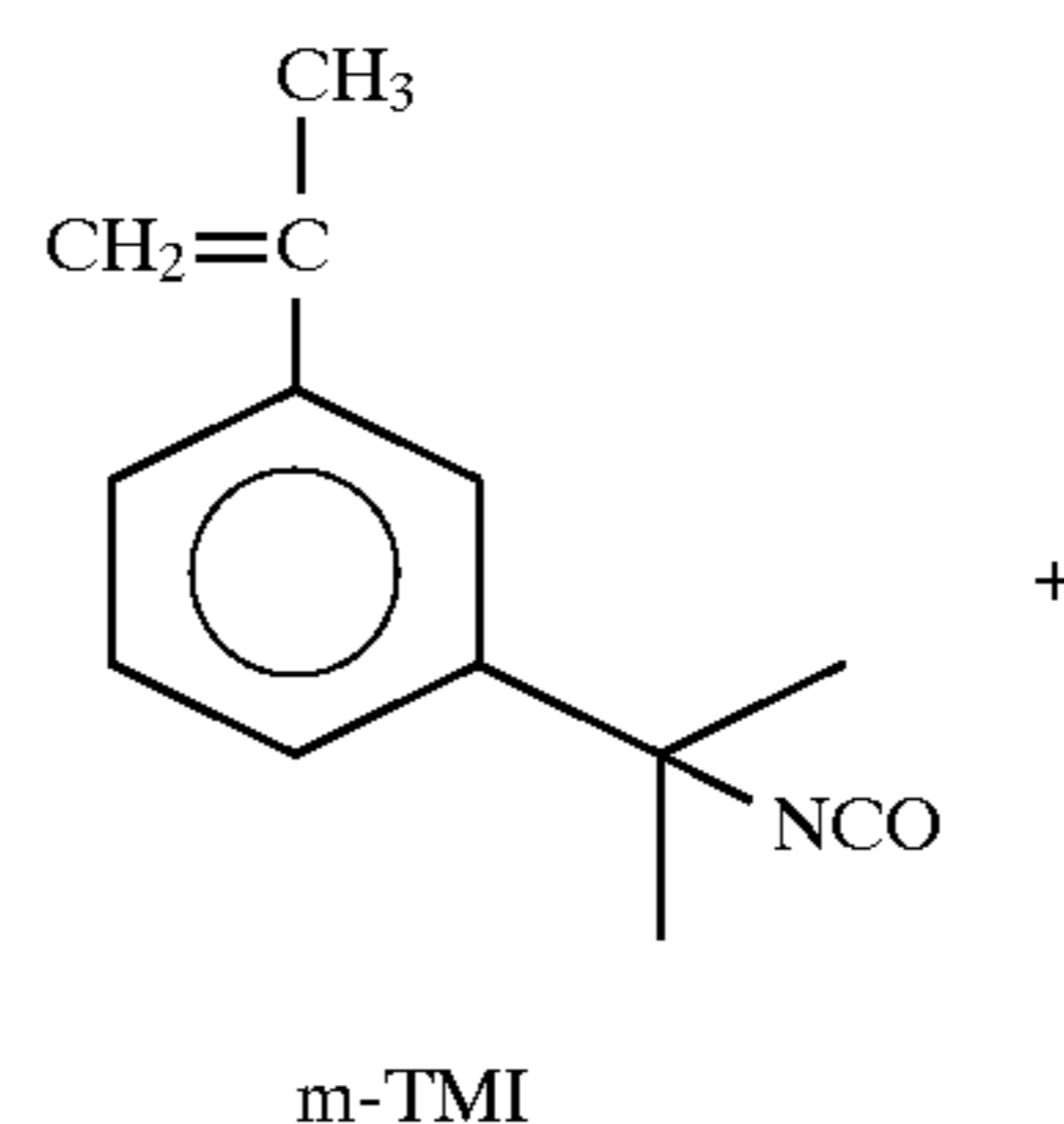
Scheme I: (Preparation of 3-isopropenyl- \alpha,\alpha -dimethyl benzyl amidoacetoacetate)
