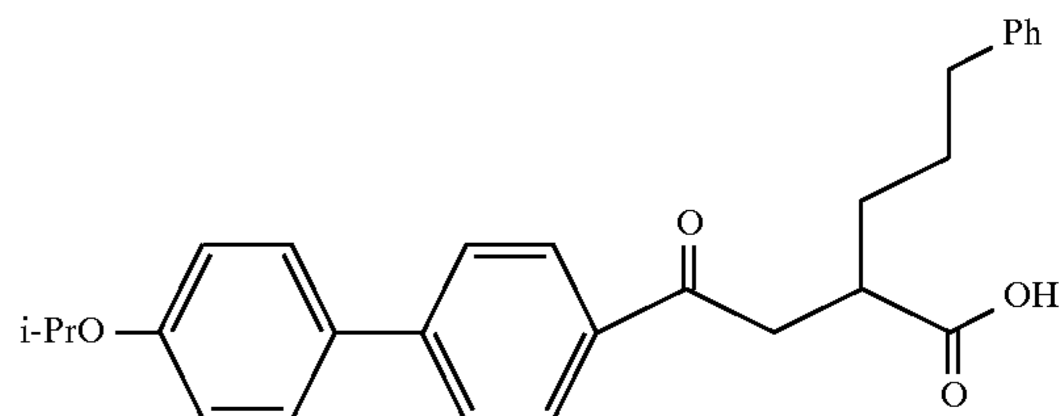
Example 85
