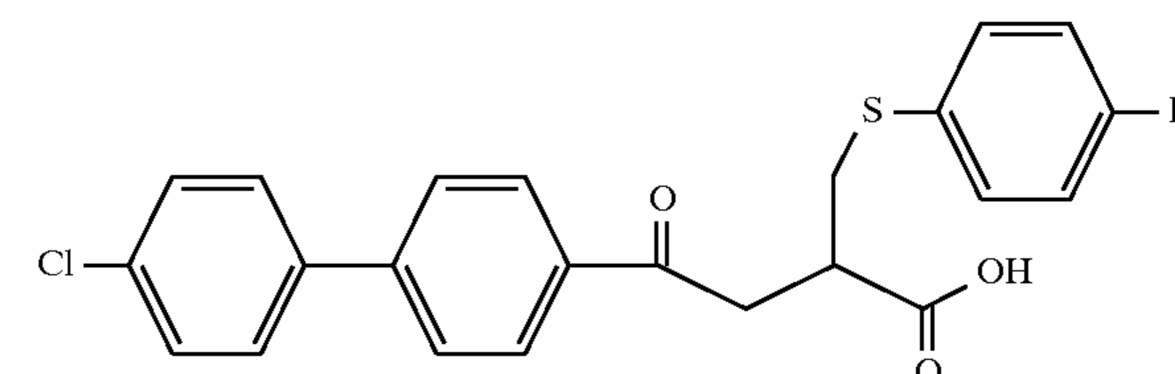
Example 138
