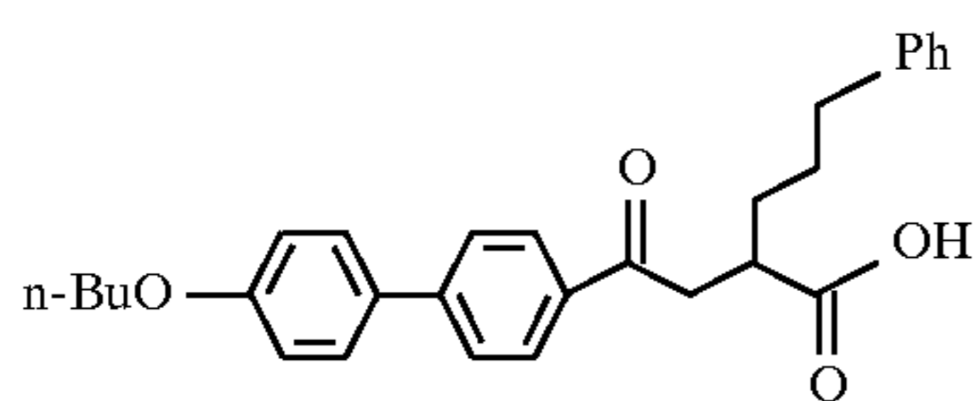
Example 83
