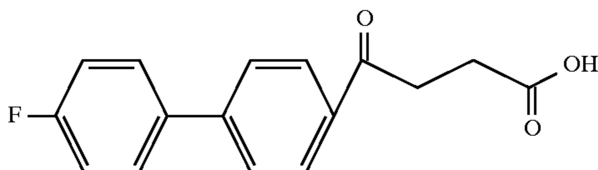
Example 8
