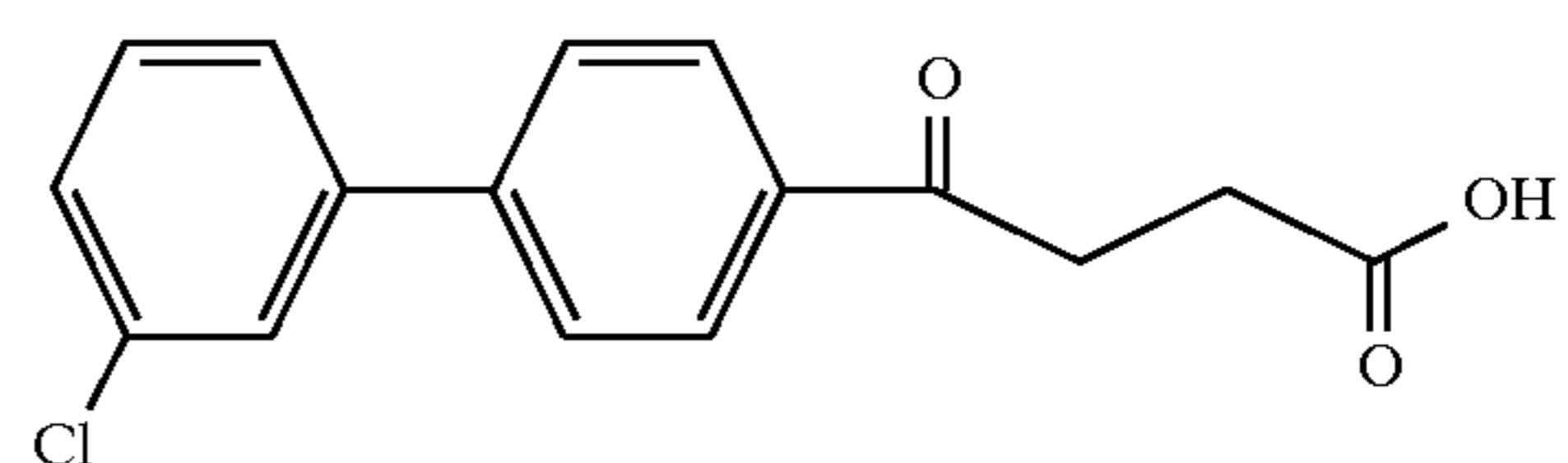
Example 12
