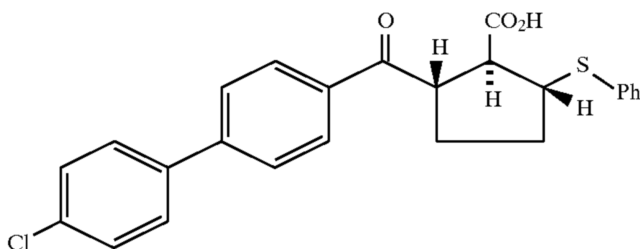
Example 209 (racemate)
