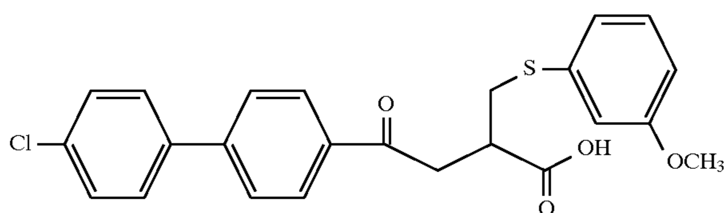
Example 164
