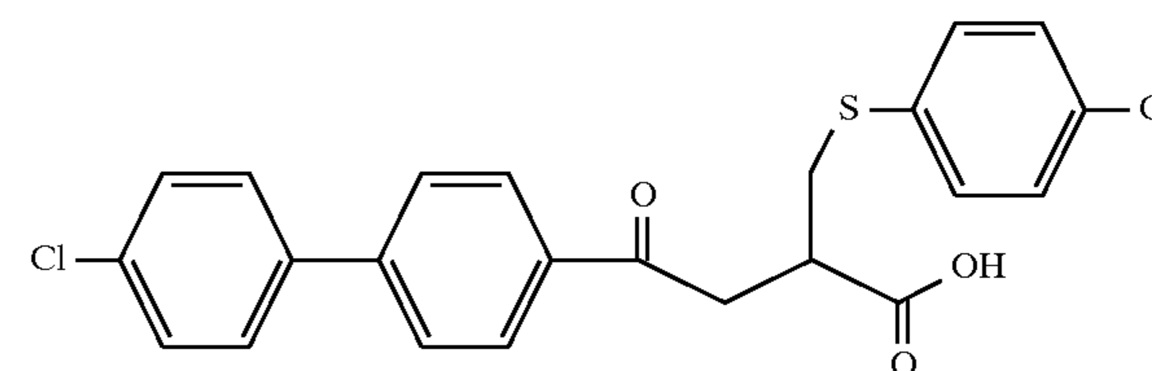
Example 139
