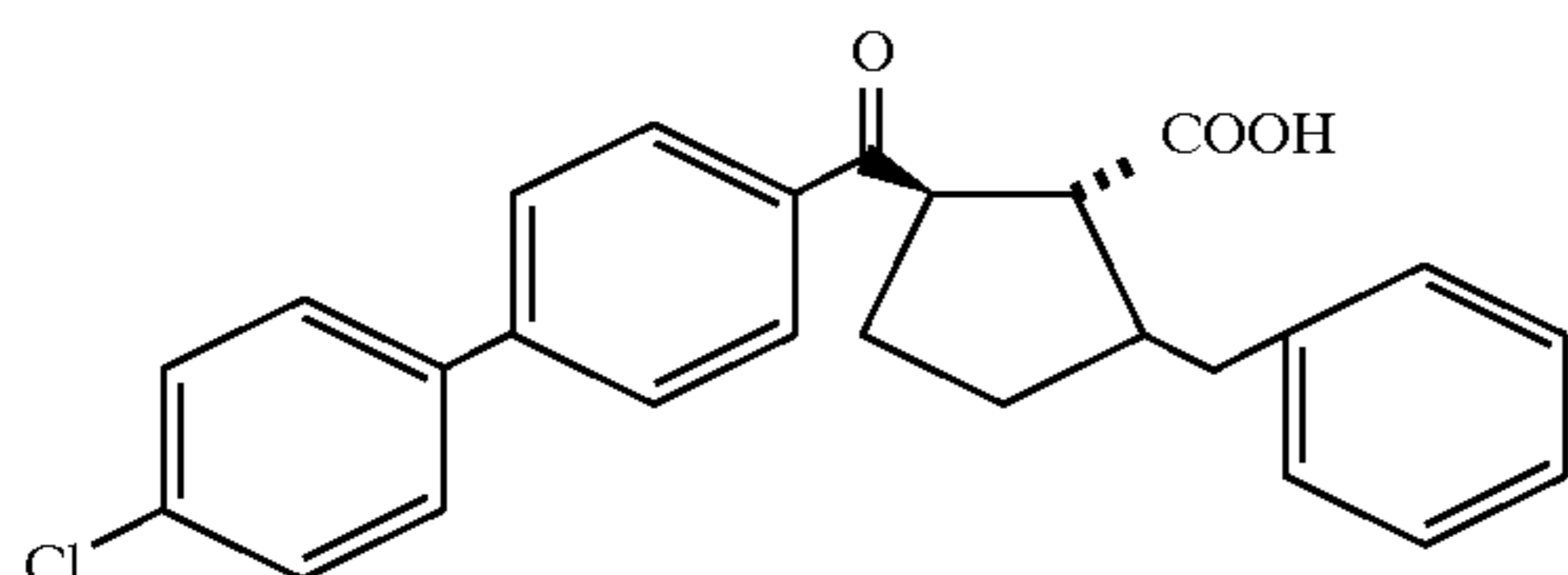
Example 227 (racemate)
