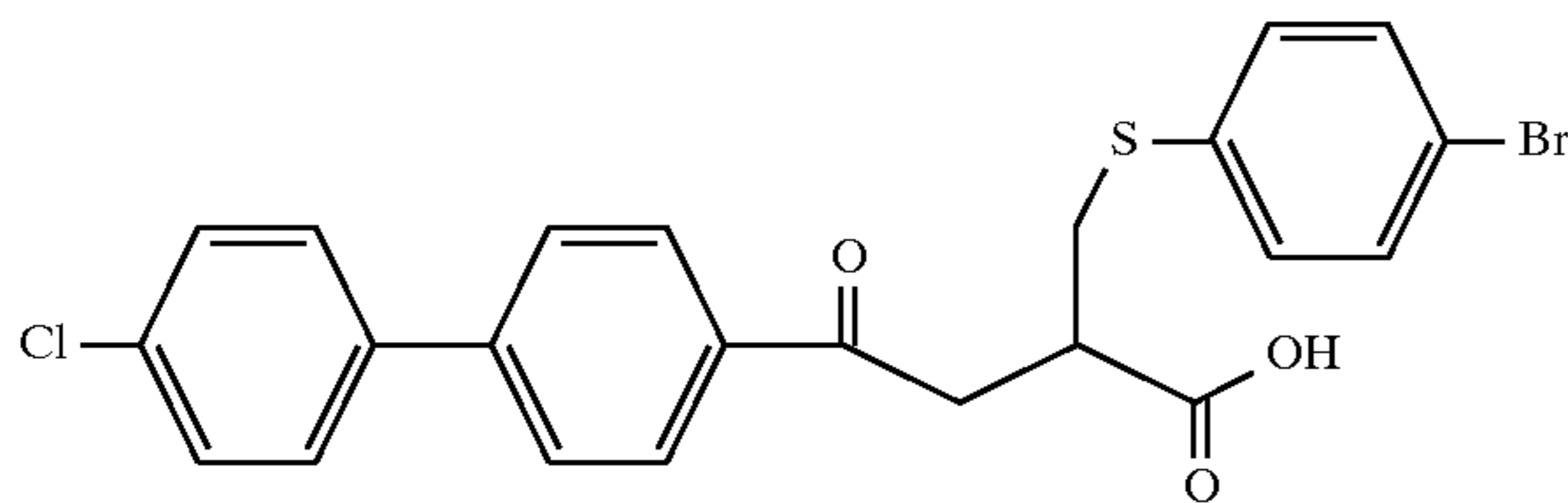
Example 140
