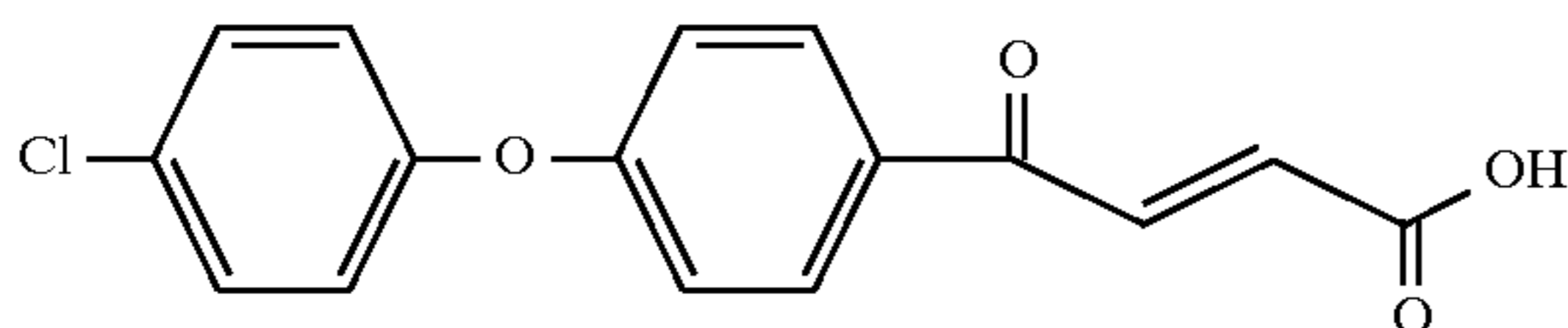
Example 35
