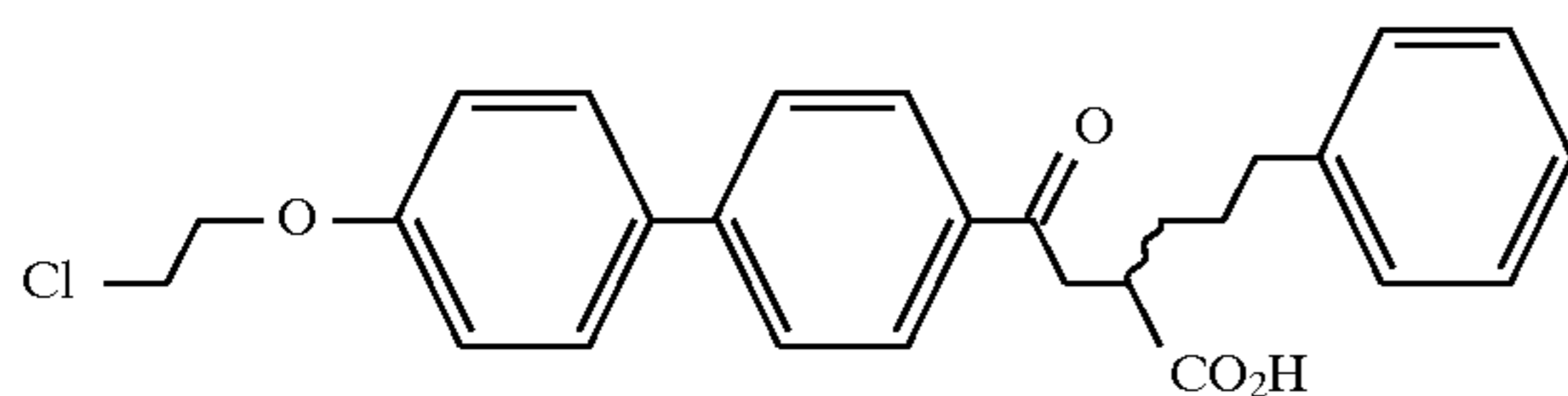
Example 52
