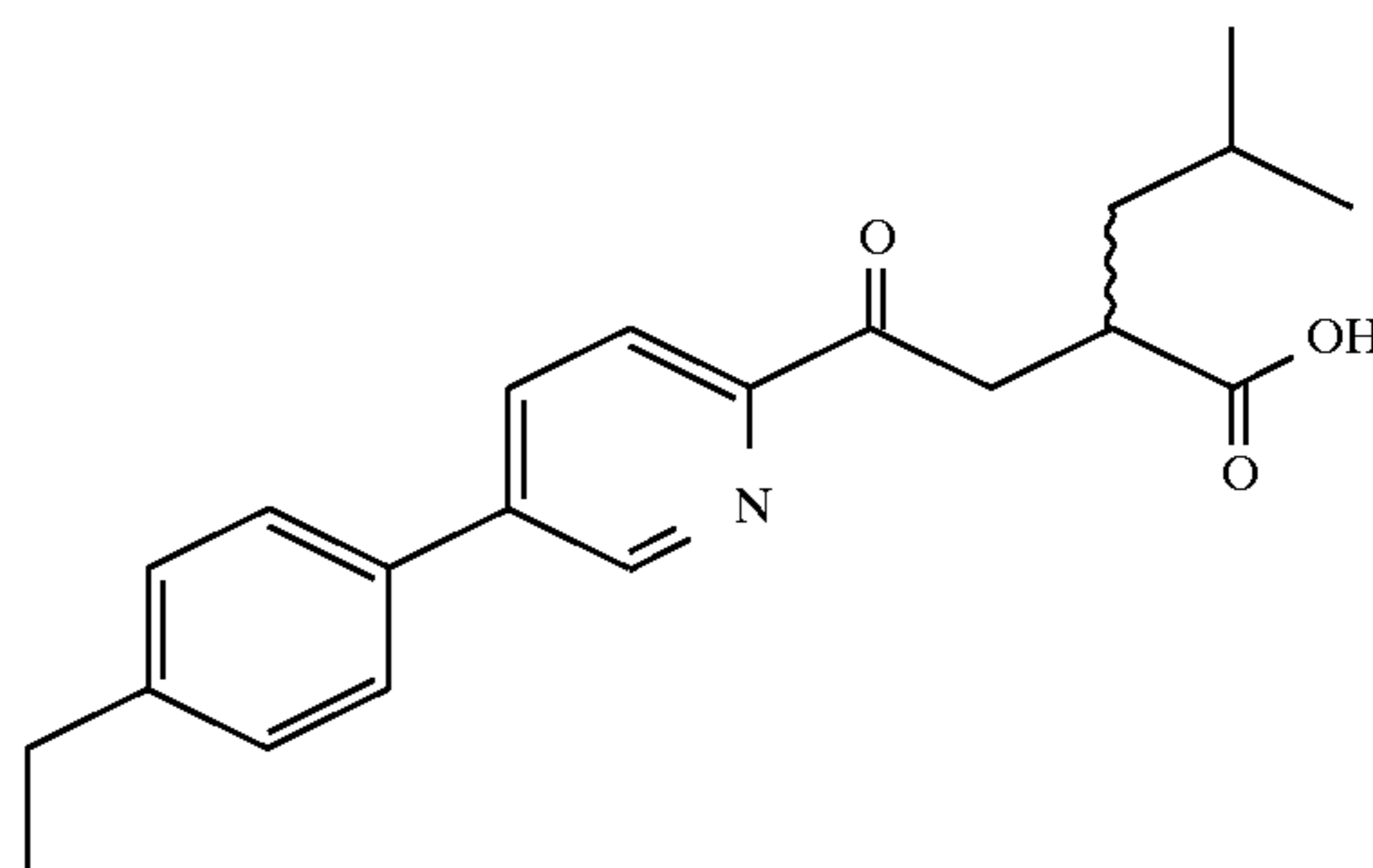
Example 61
