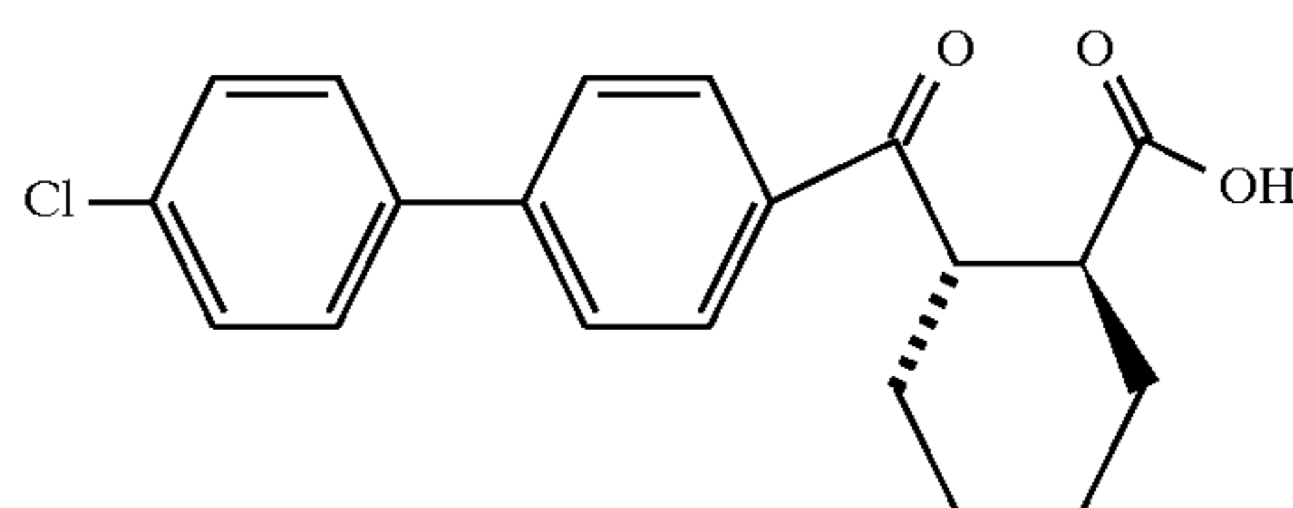
Example 200 (racemate)
