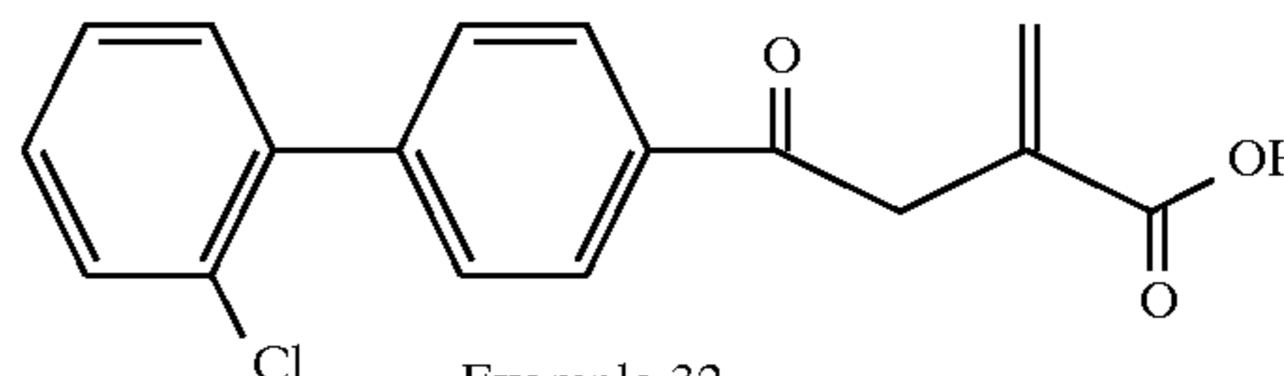
Example 32
