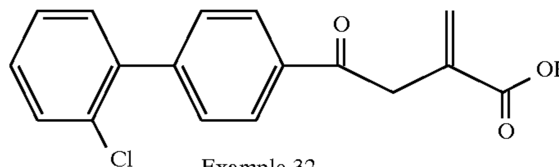
Example 32
