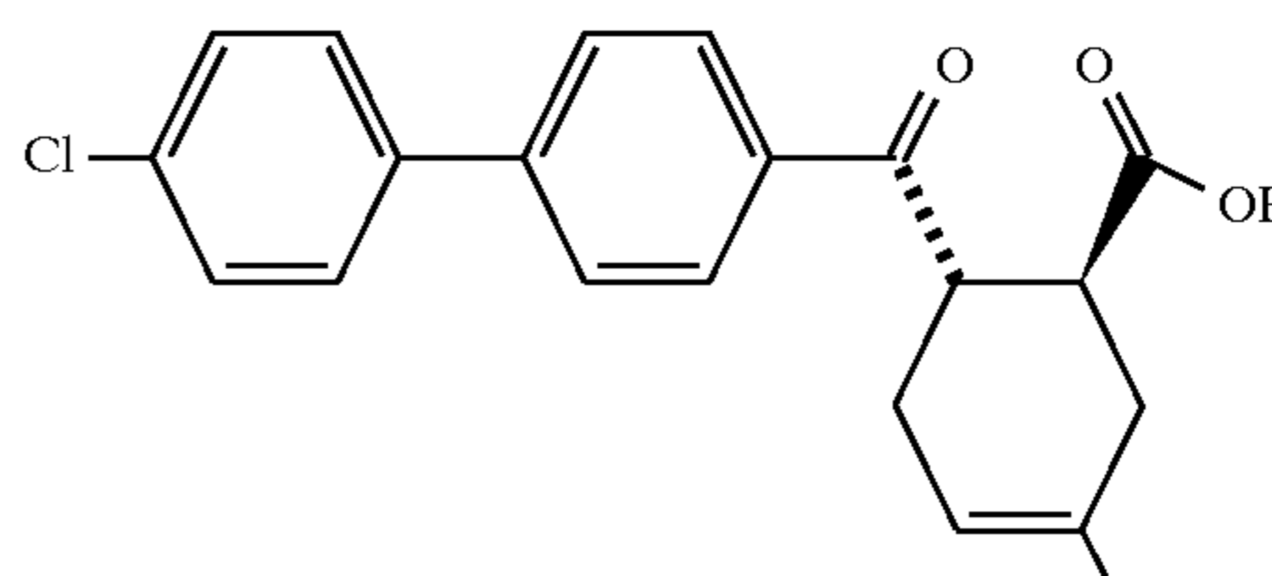
Example 230 (racemate)
