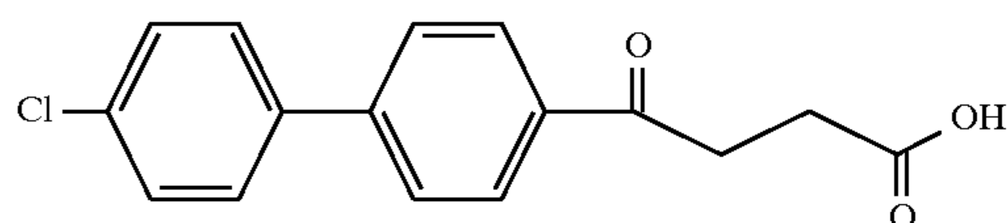
Example 6
