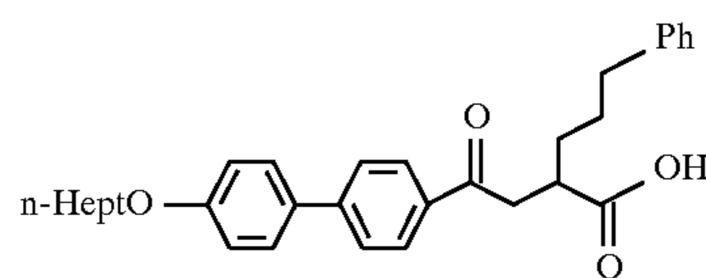
Example 86
