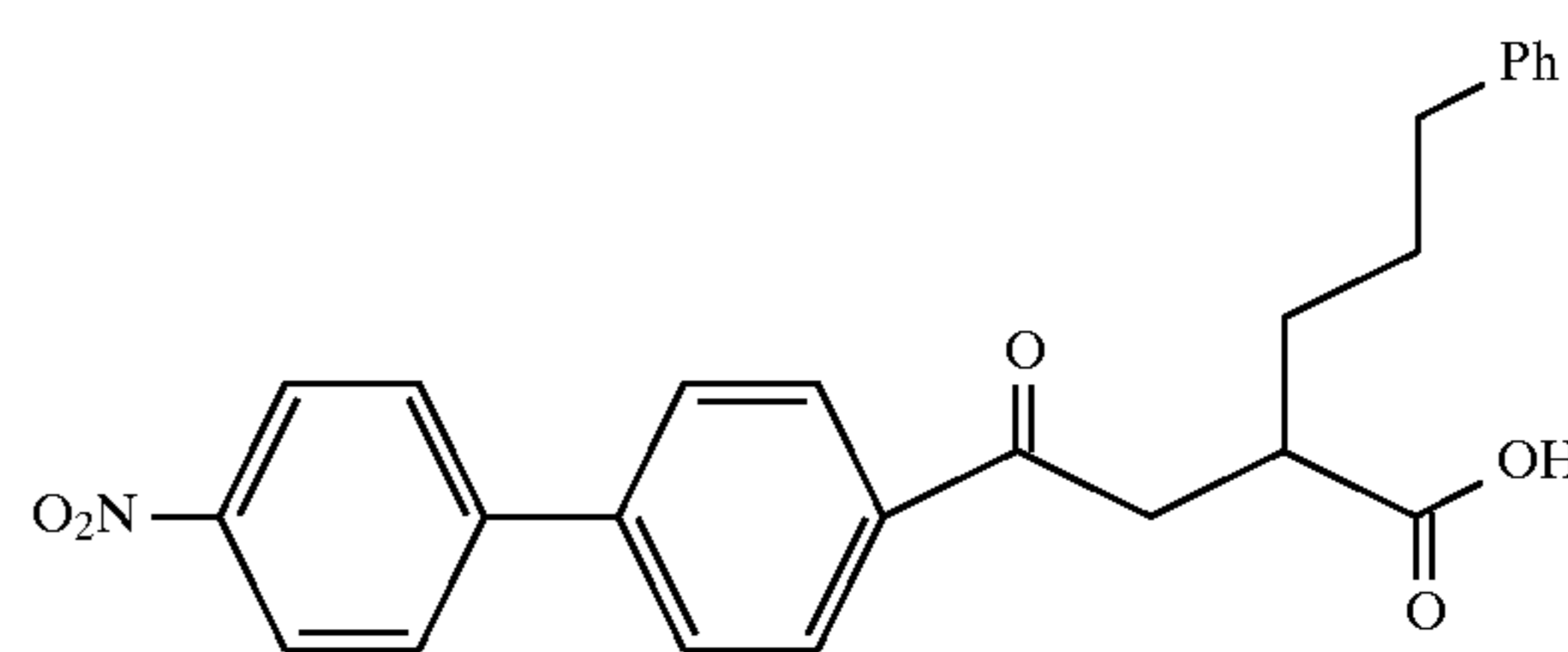
Example 63
