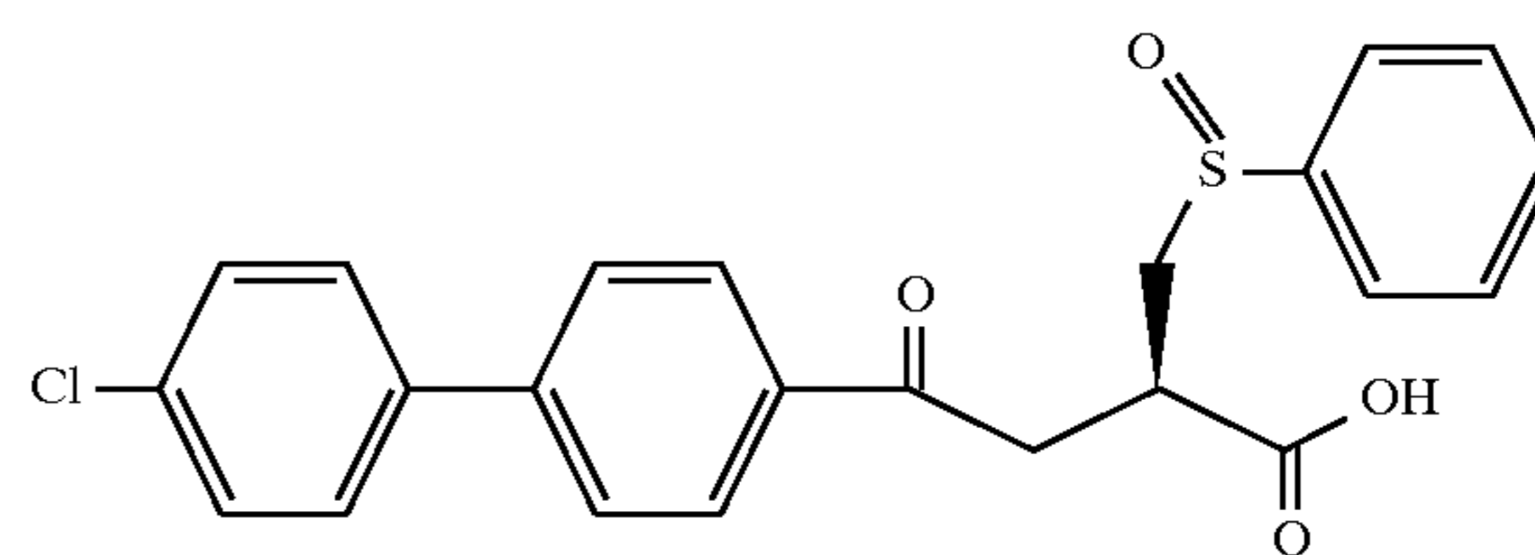
Example 126
