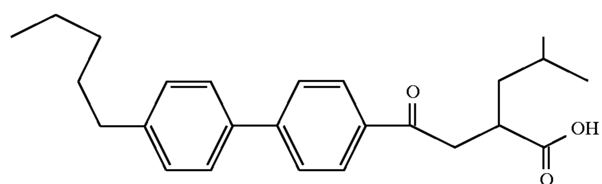
Example 23
