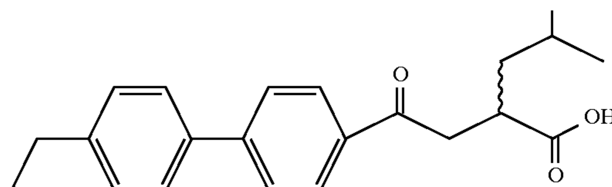
Example 16
