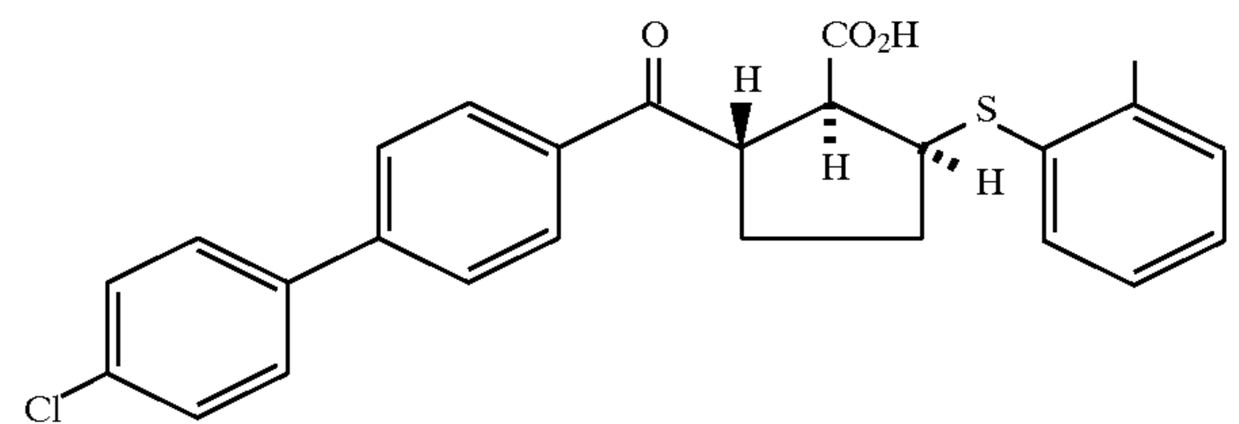
Example 218 (racemate)
