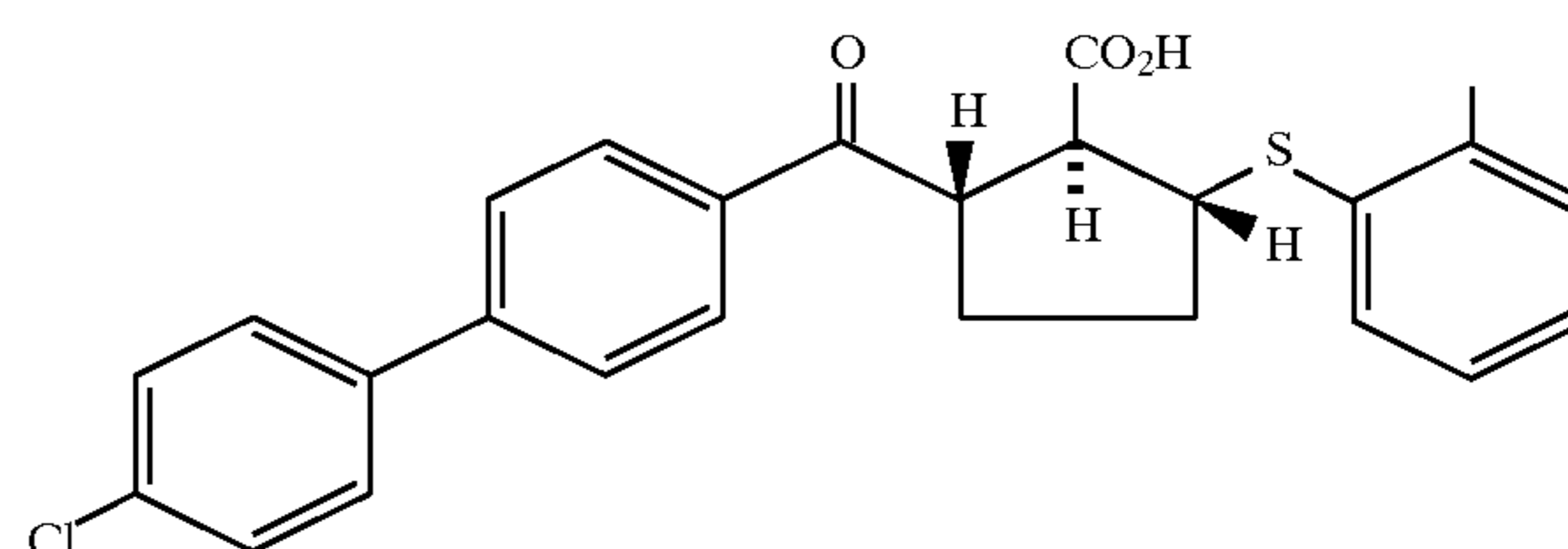
Example 219 (racemate)
