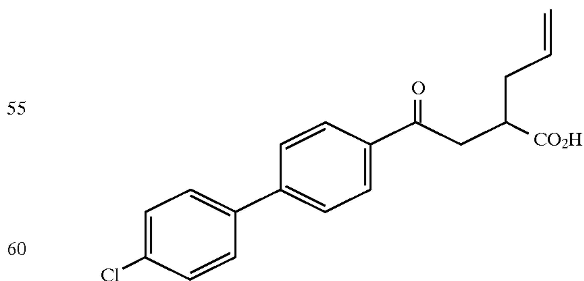
Example 94
