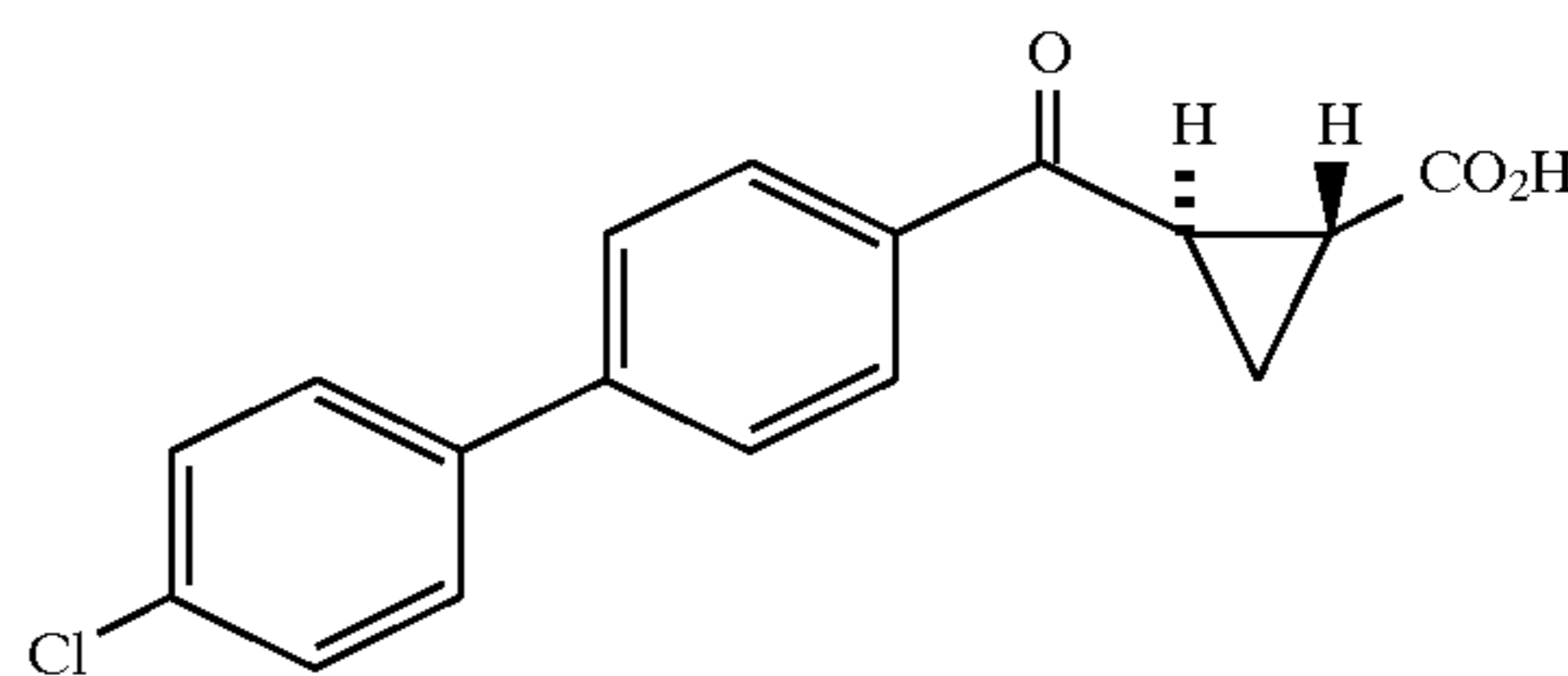
Example 208 (racemate)
