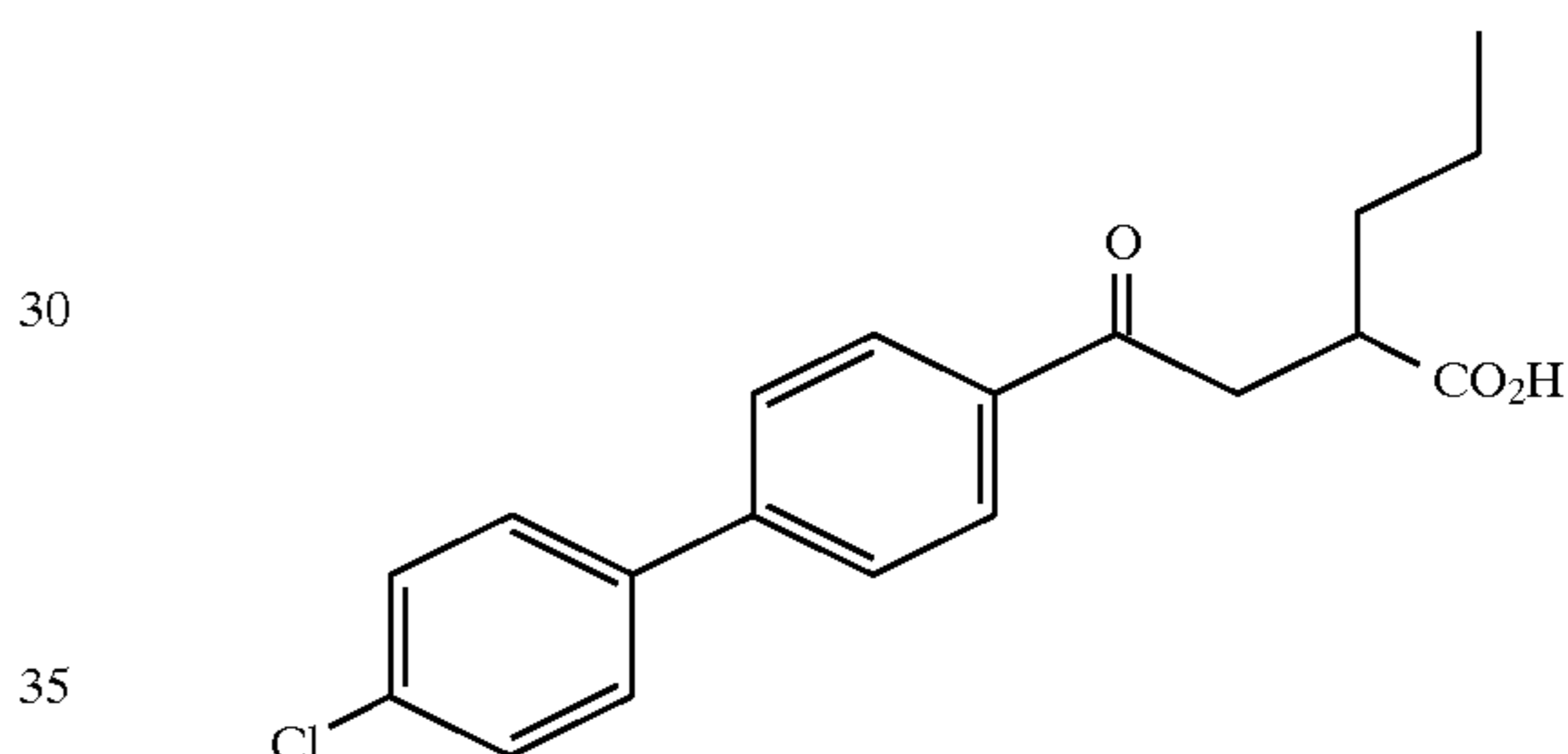
Example 93
