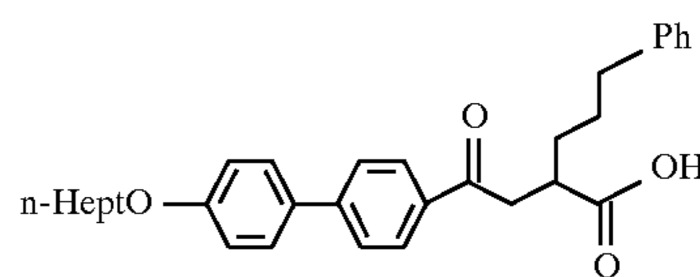
Example 86
