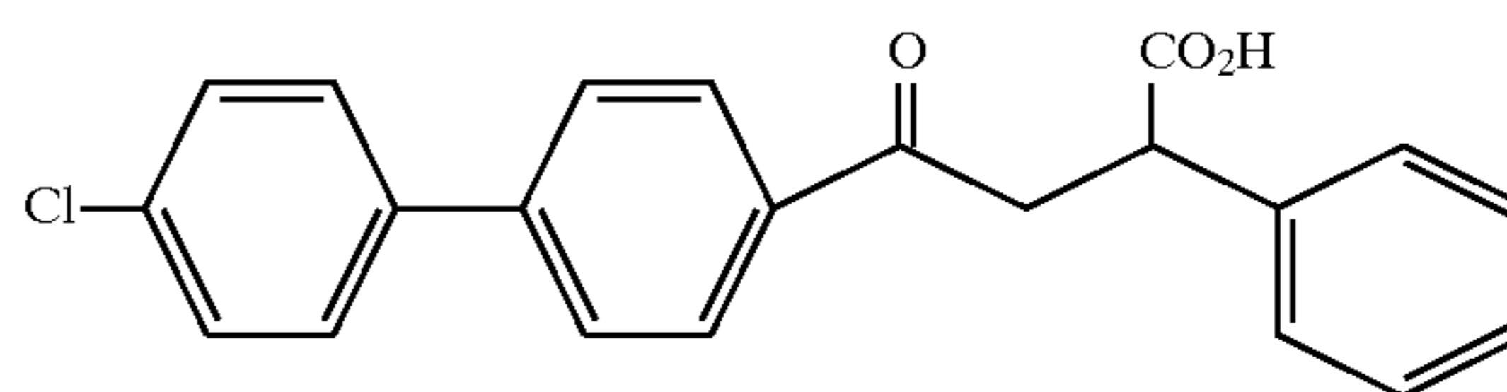
Example 104
