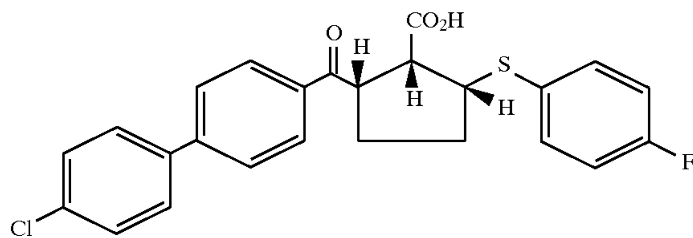
Example 214 (racemate)
