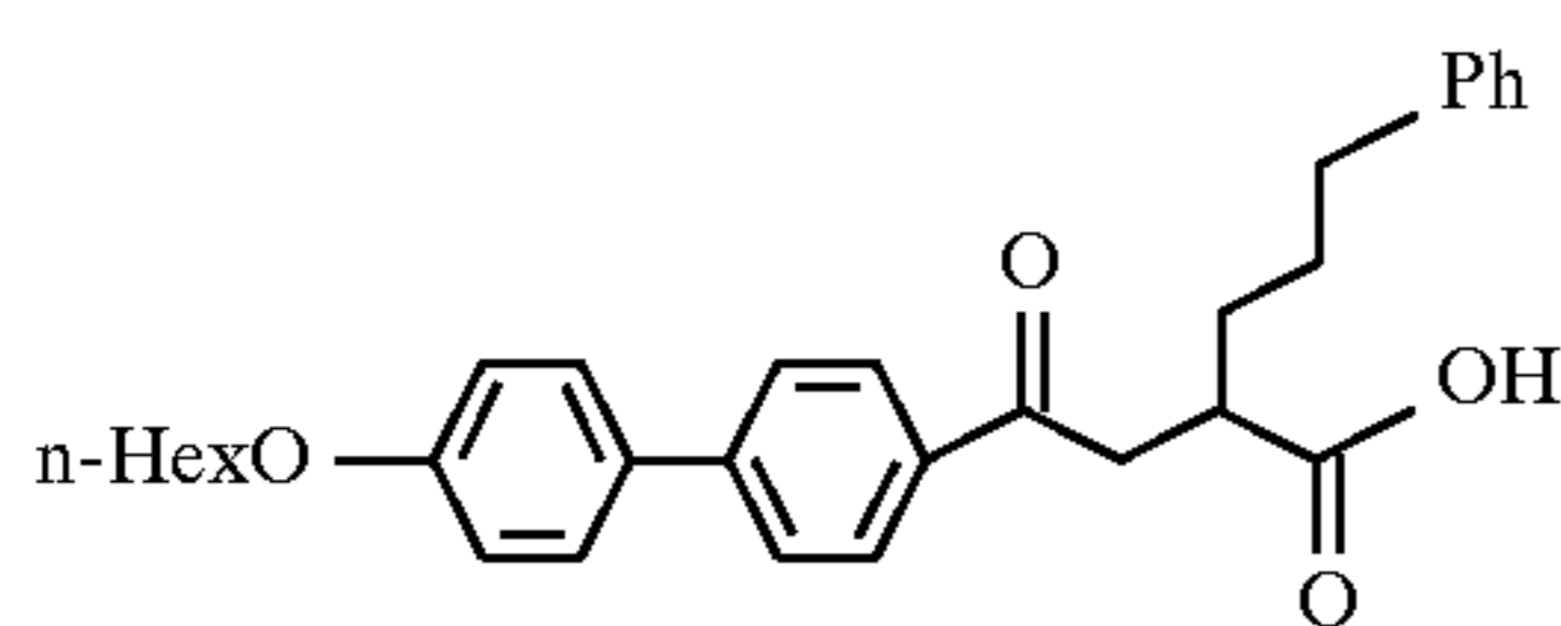
Example 82
