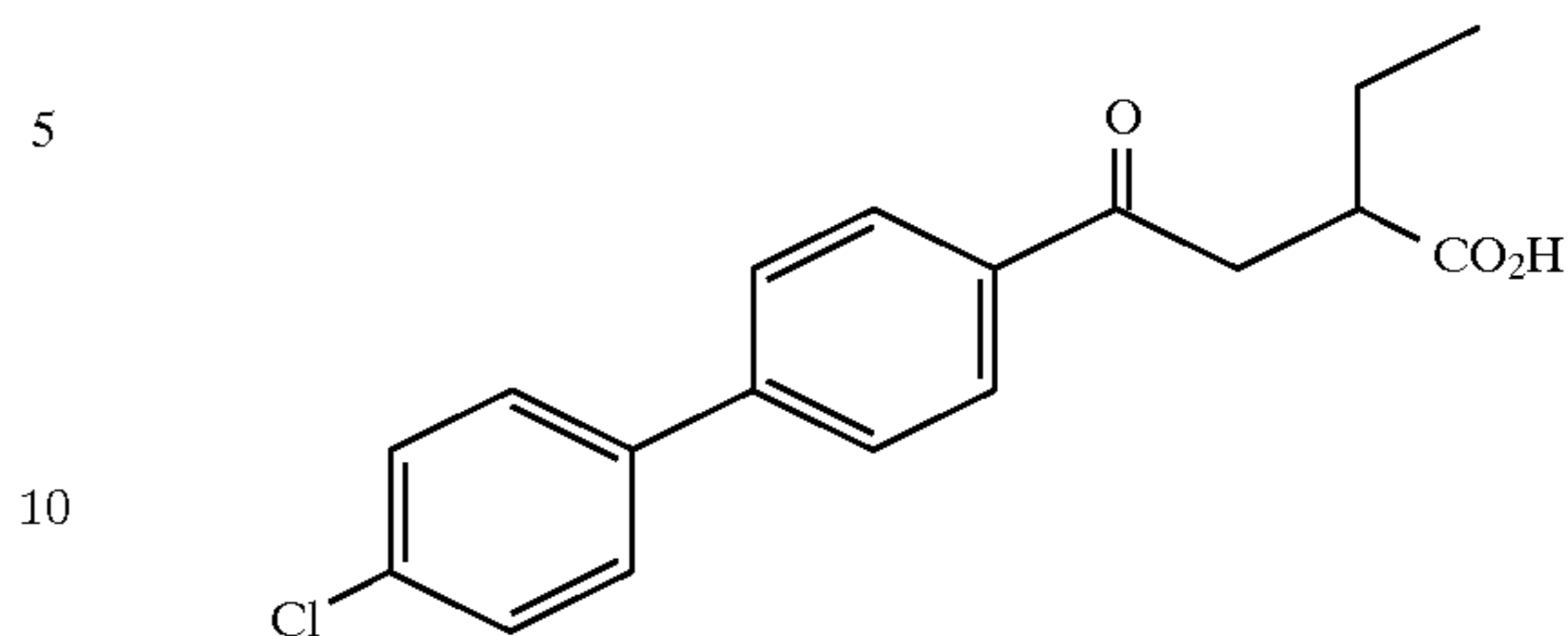
Example 92
