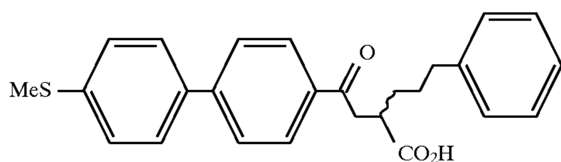
Example 51
