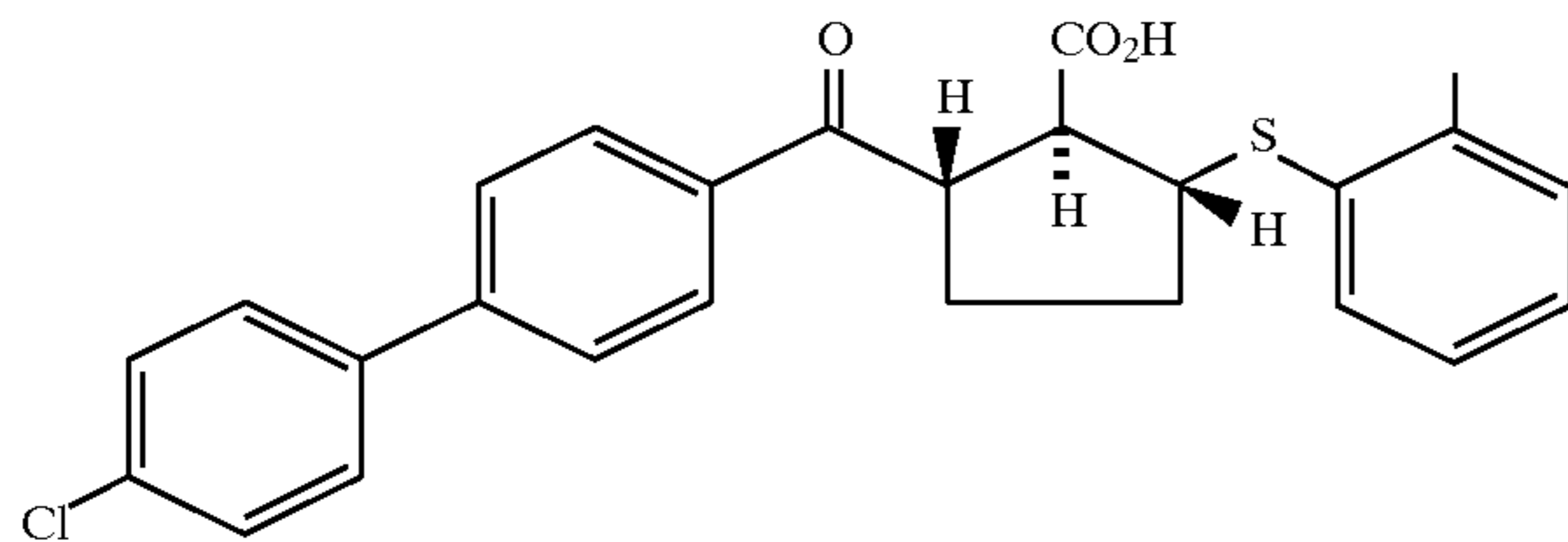
Example 216 (racemate)
