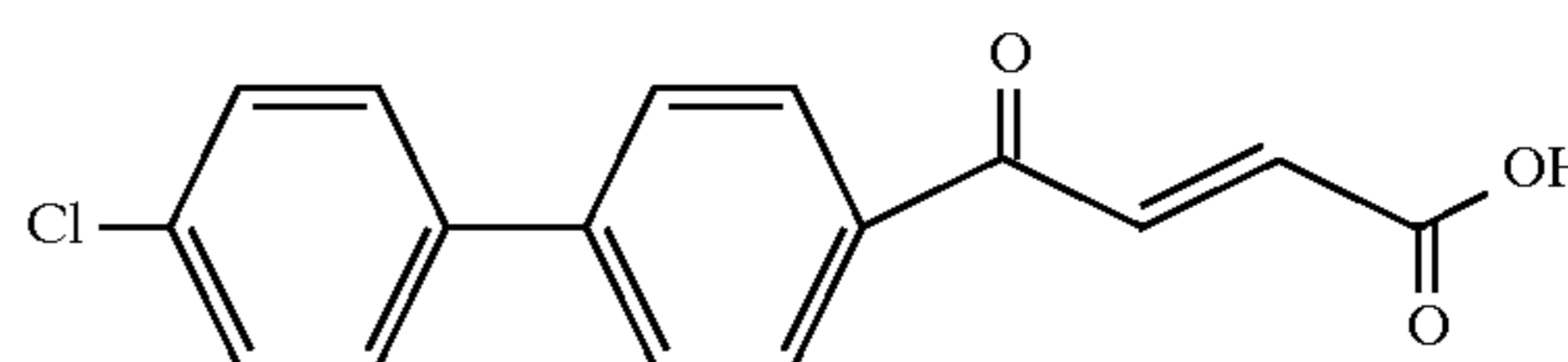
Example 34
