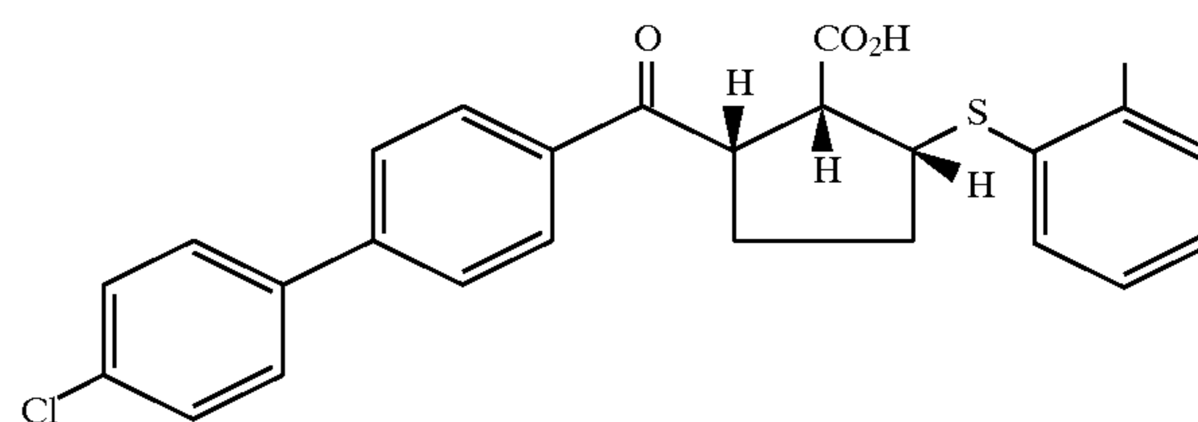
Example 217 (racemate)
