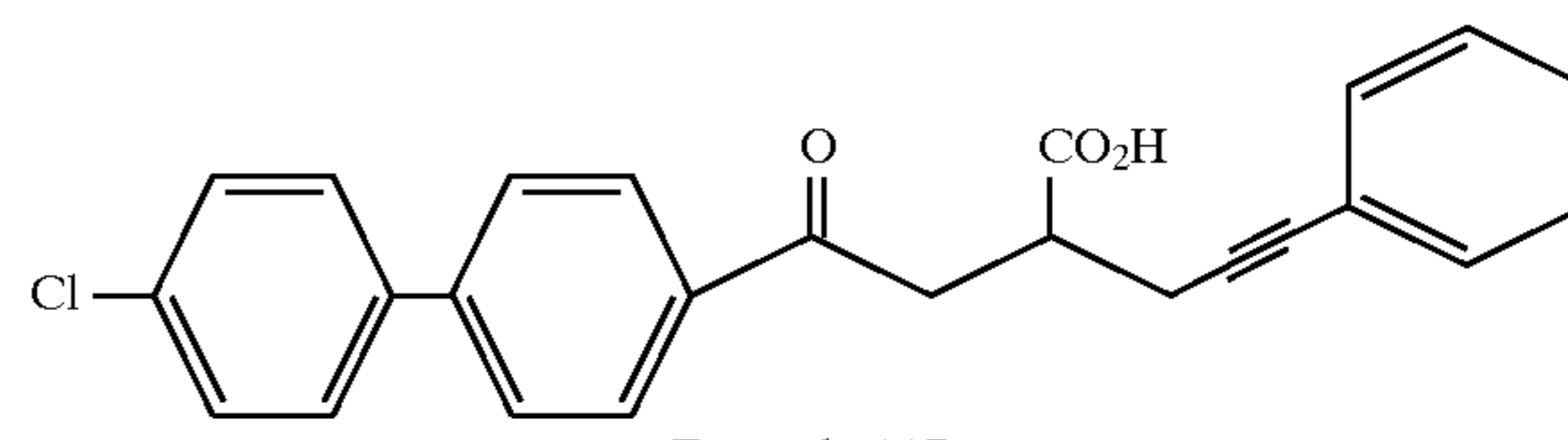
Example 117
