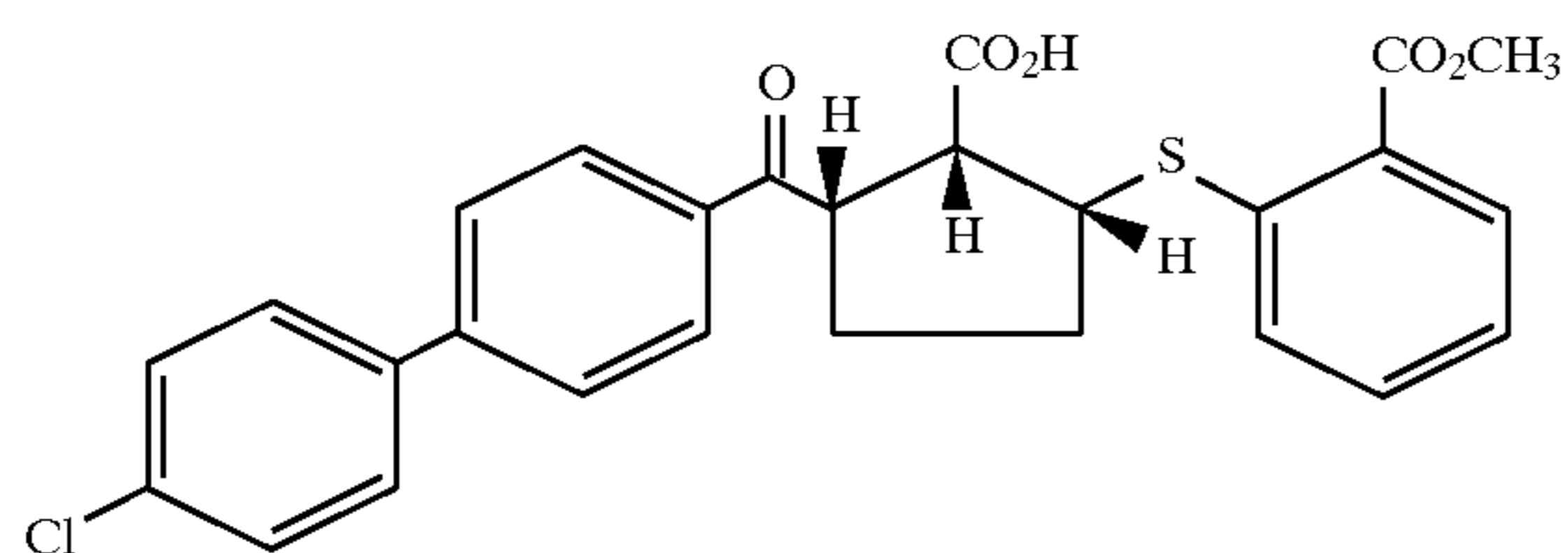
Example 220 (racemate)
