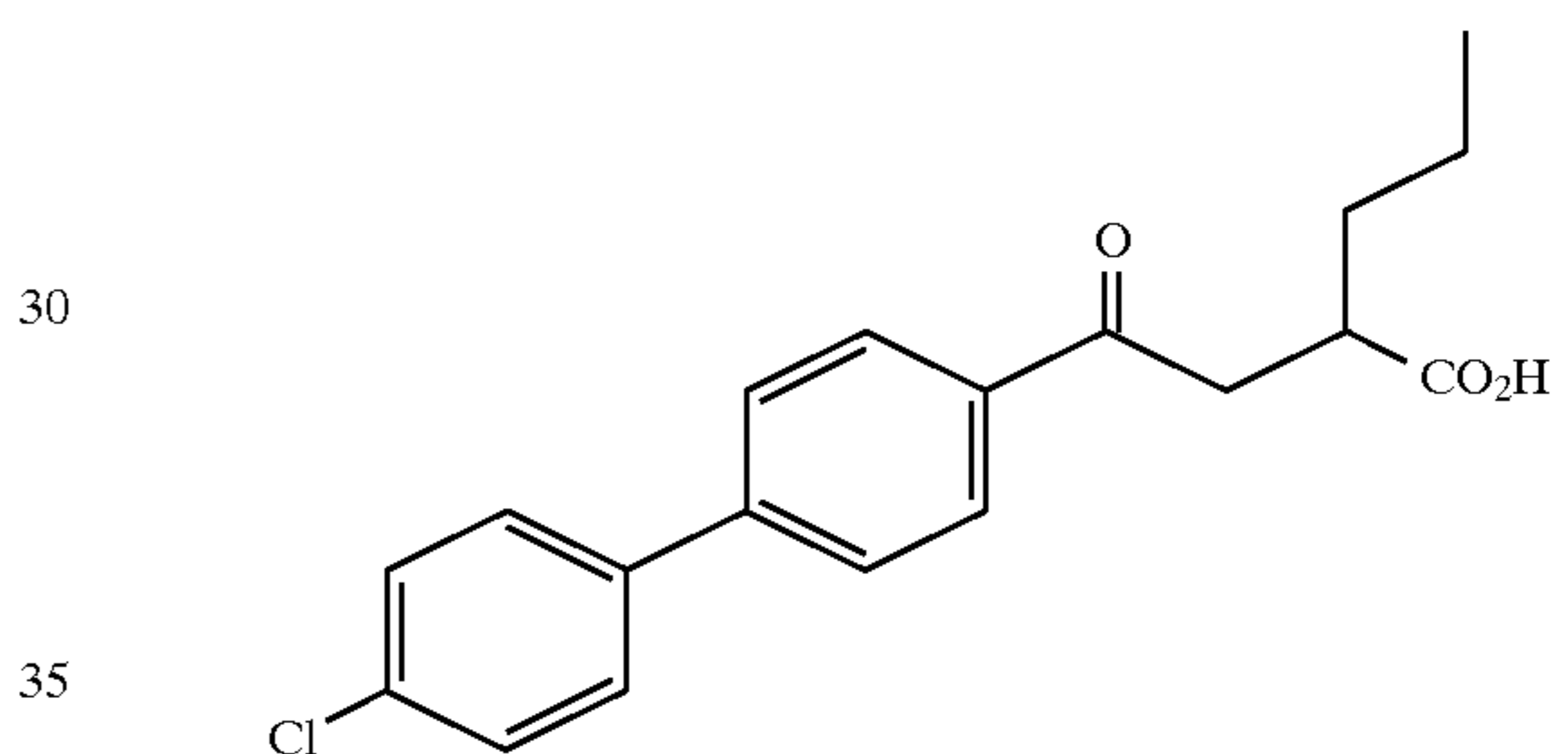
Example 93
