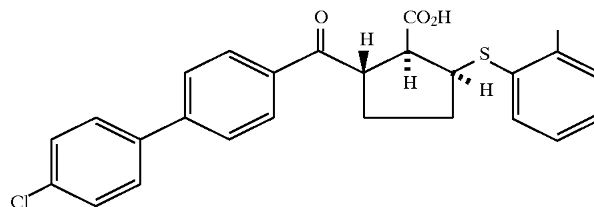
Example 218 (racemate)
