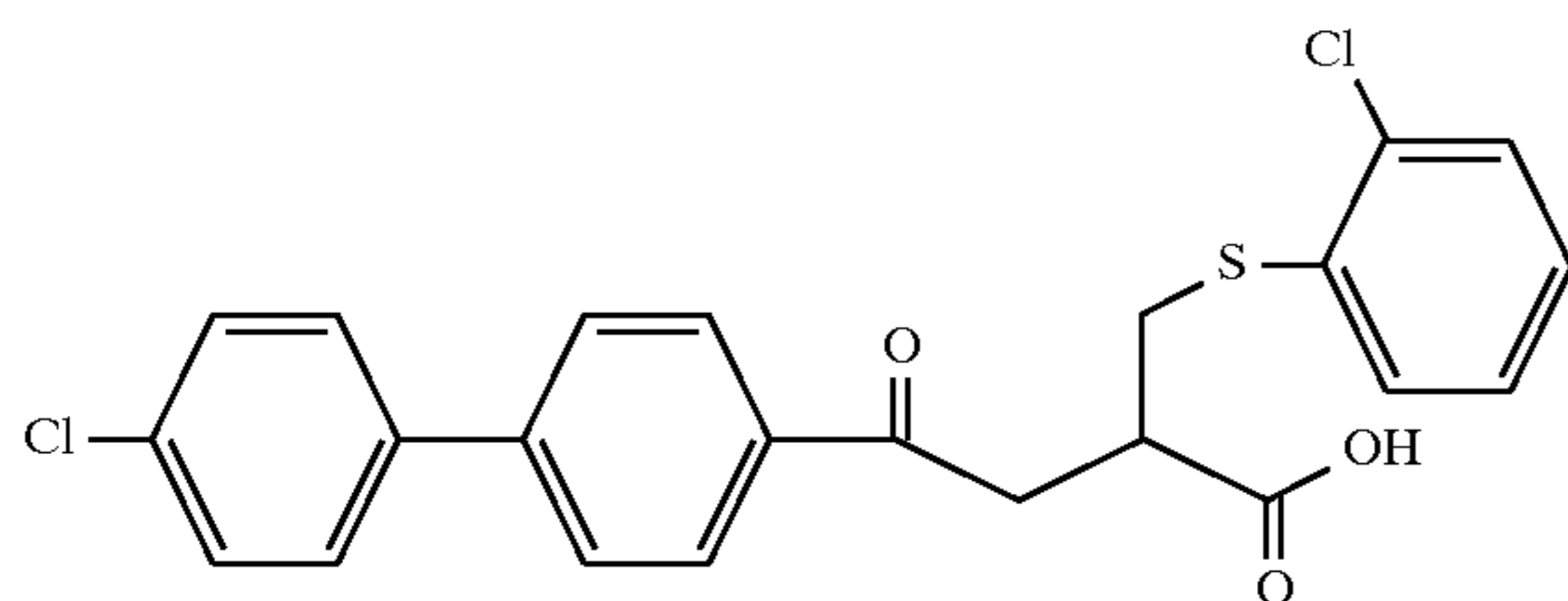
Example 160
