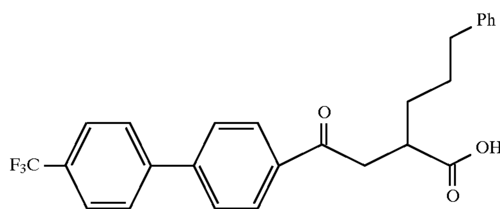
Example 62
