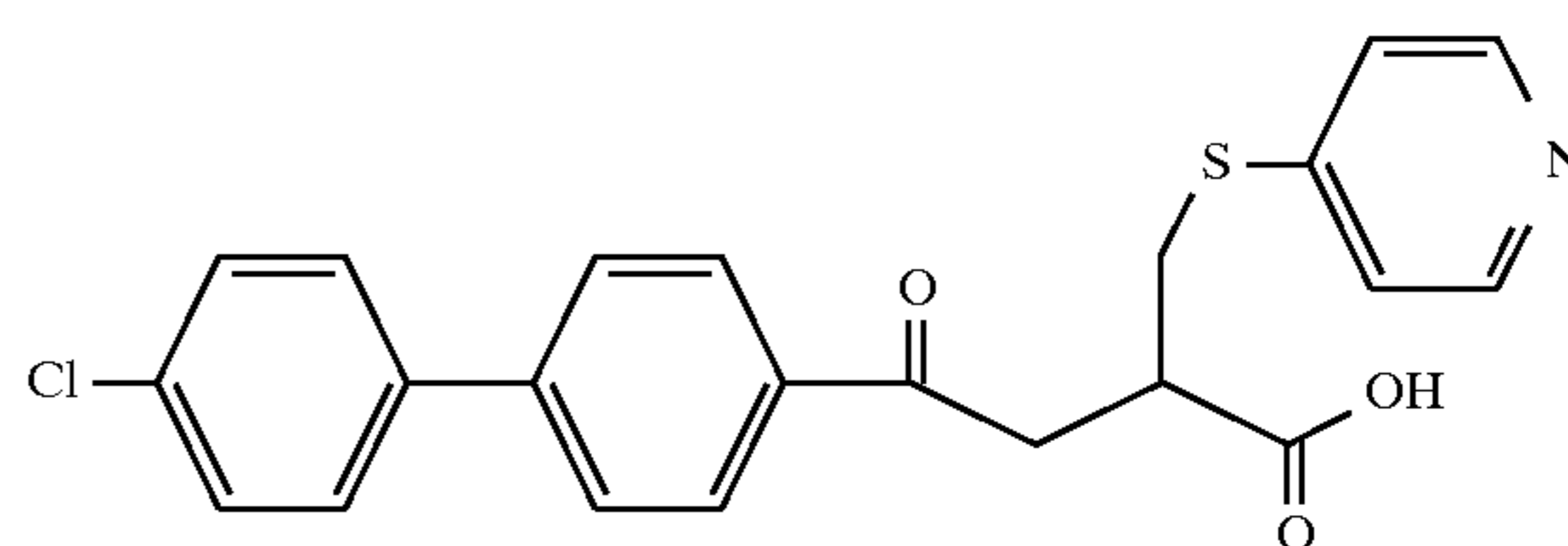
Example 152
