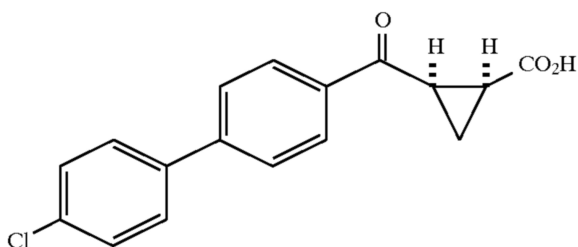
Example 207 (racemate)
