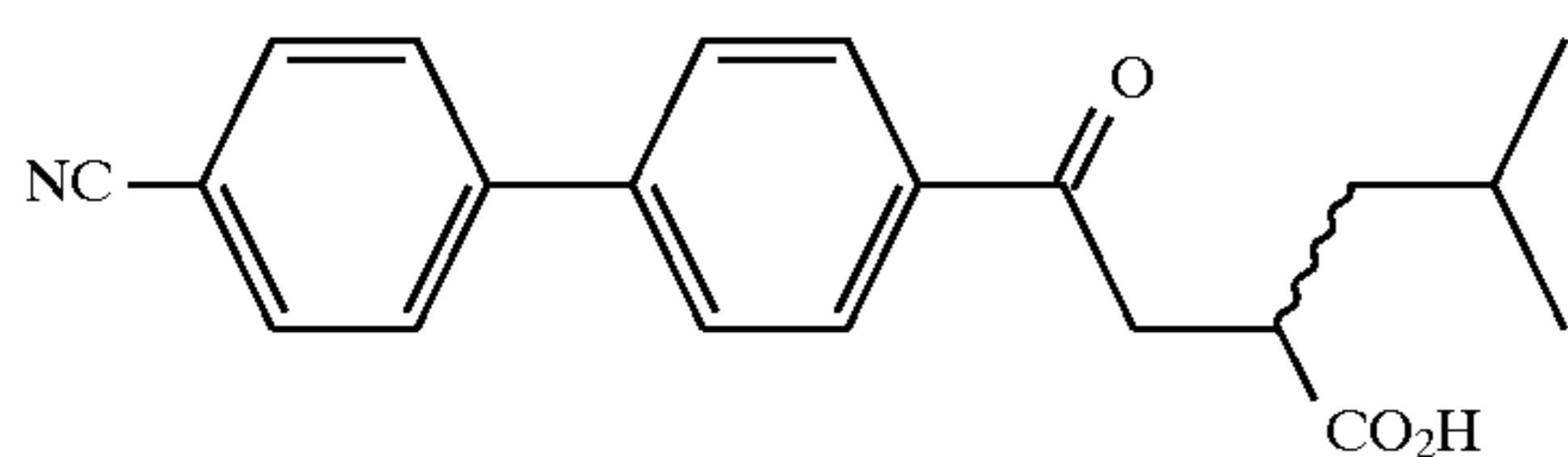
Example 46
