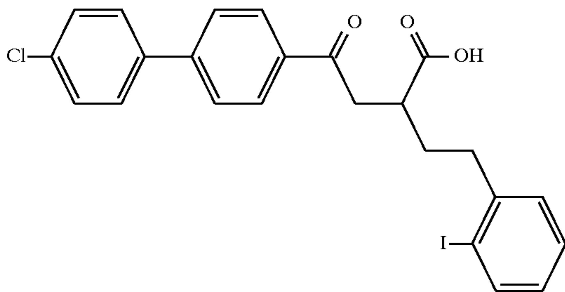
Example 102
