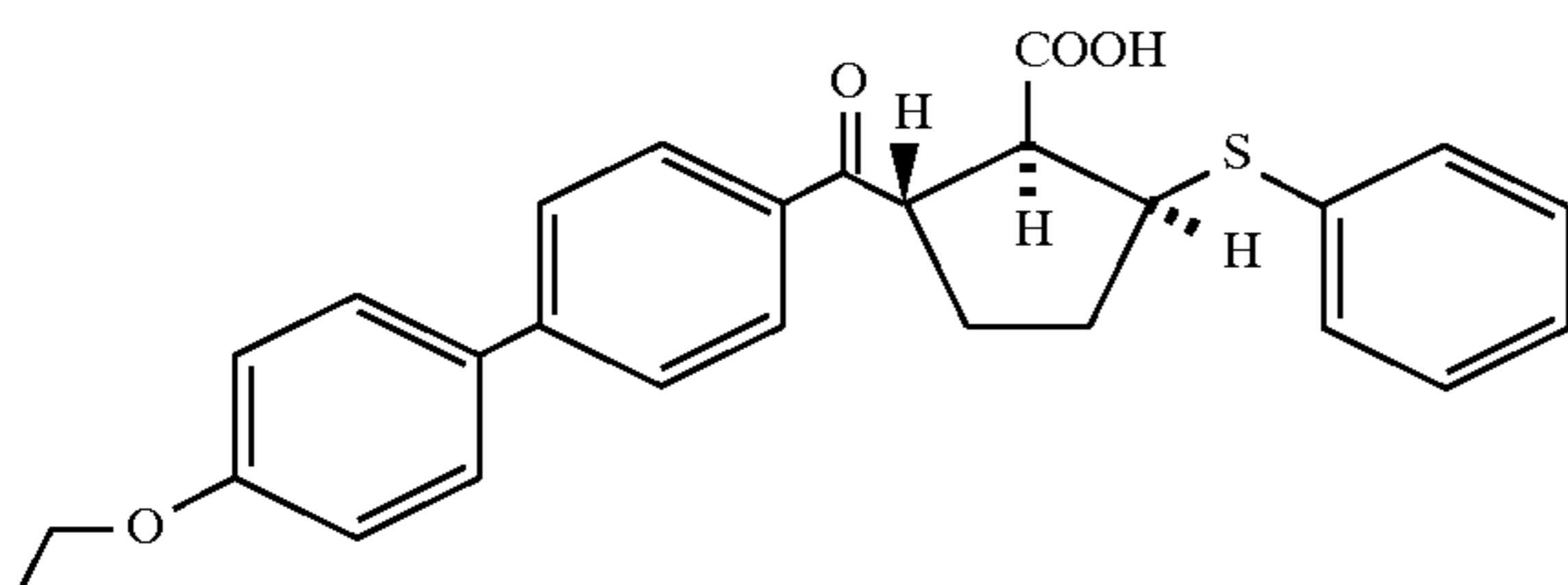
Example 225 (racemate)
