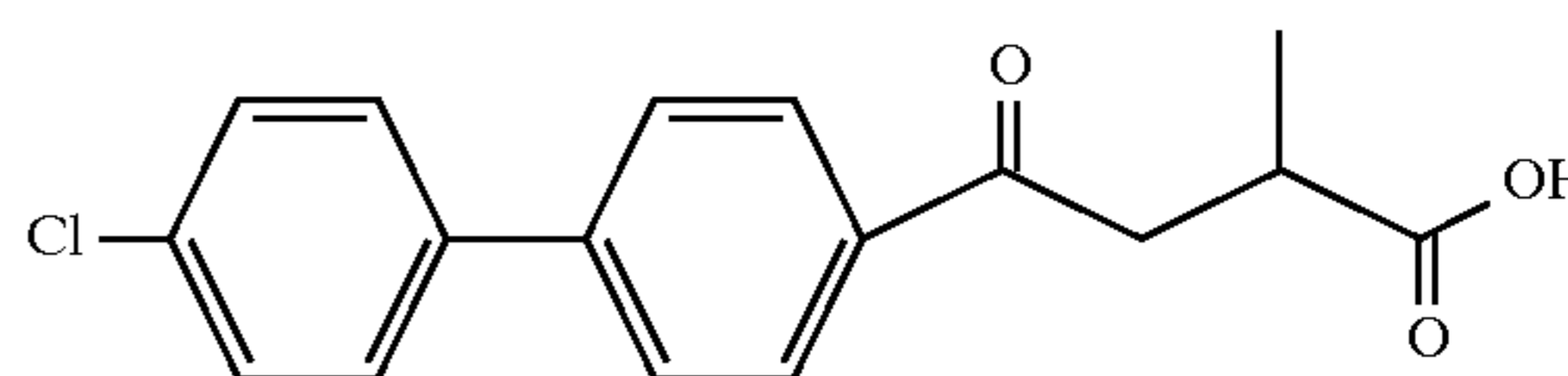
Example 33
