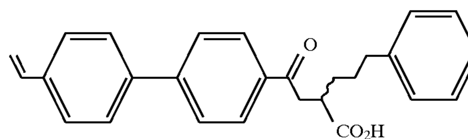
Example 55
