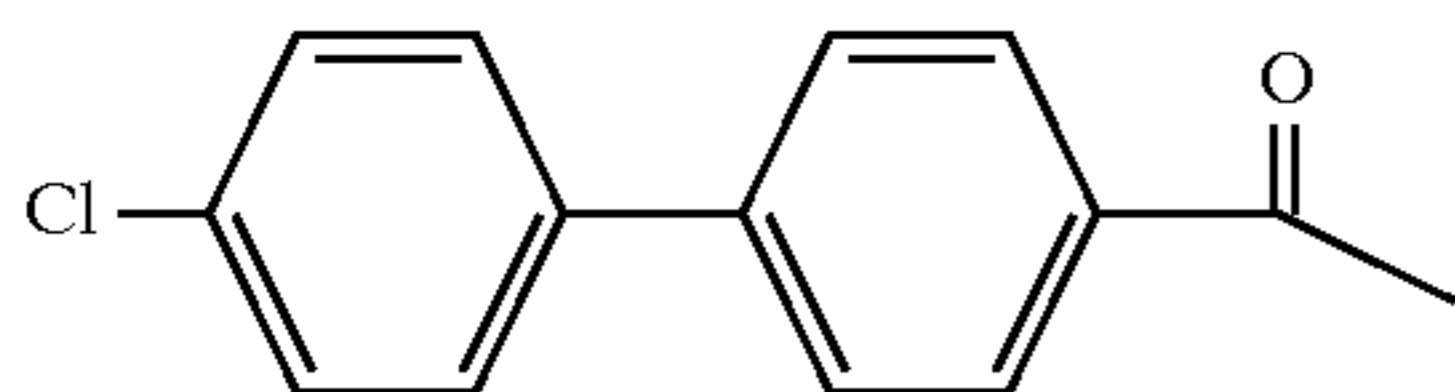
Example 37
