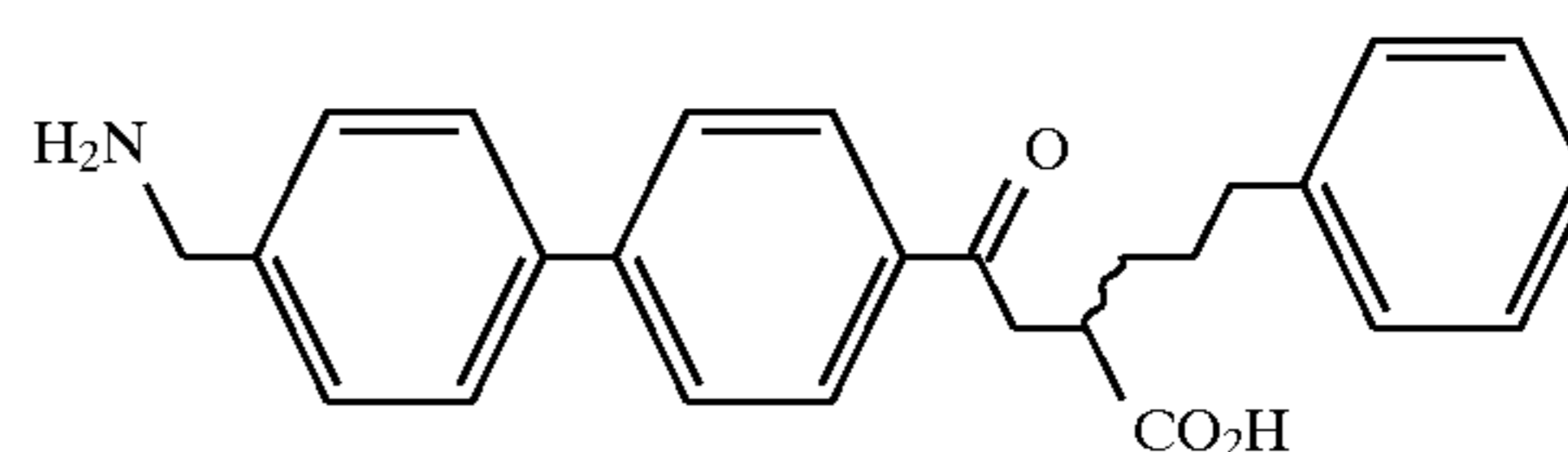
Example 59
