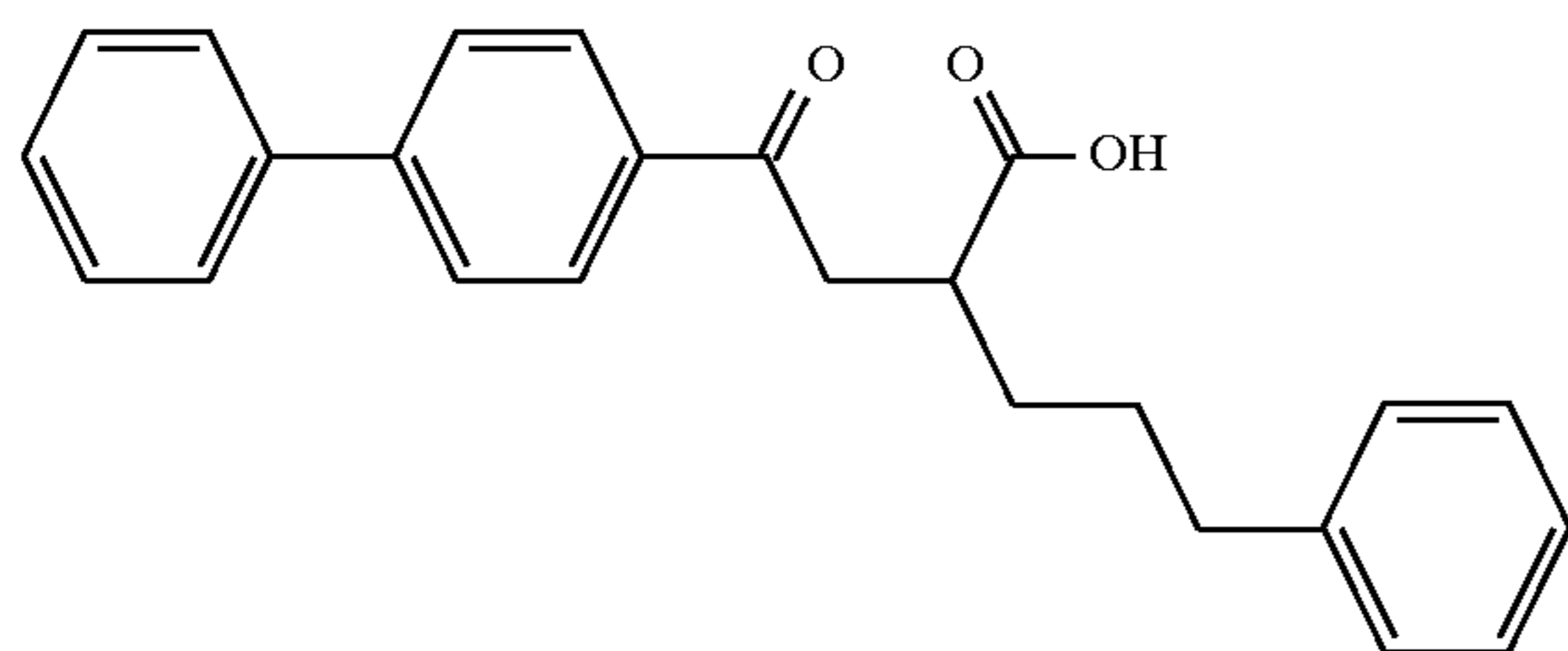
Example 91
