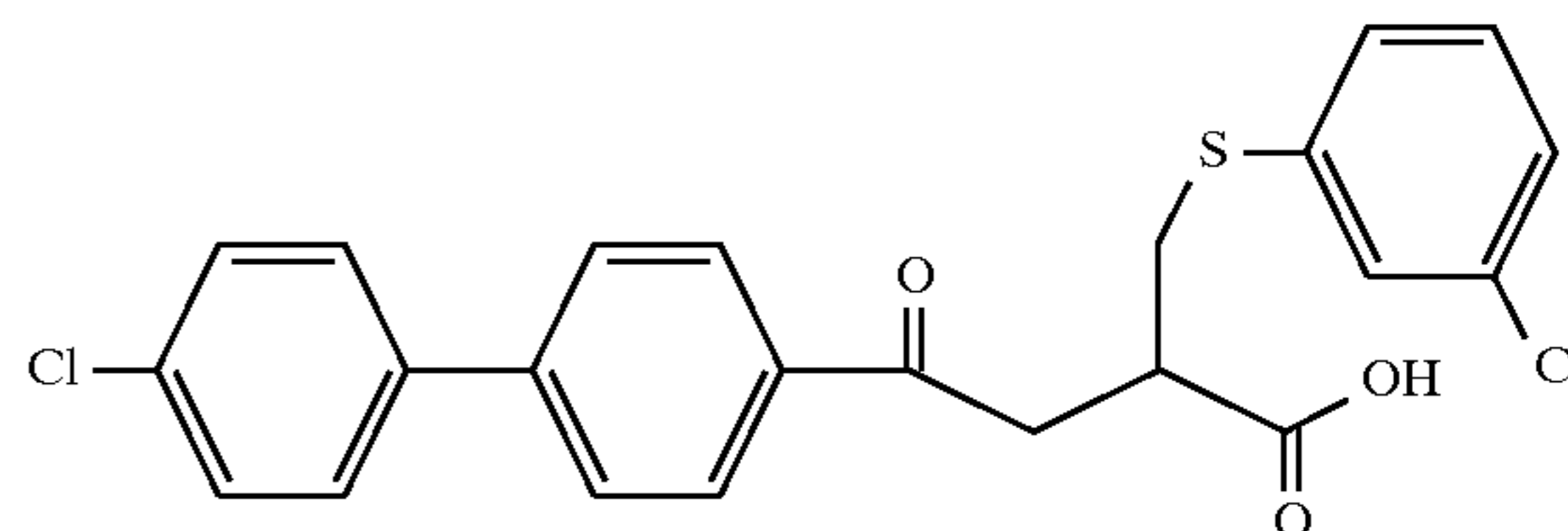
Example 172
