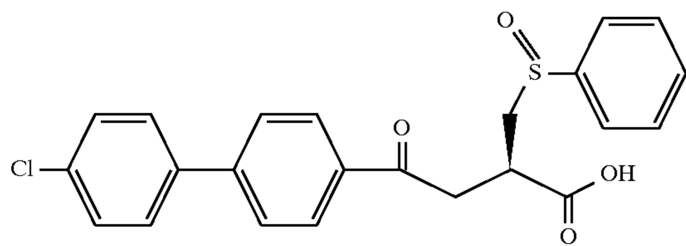
Example 125
