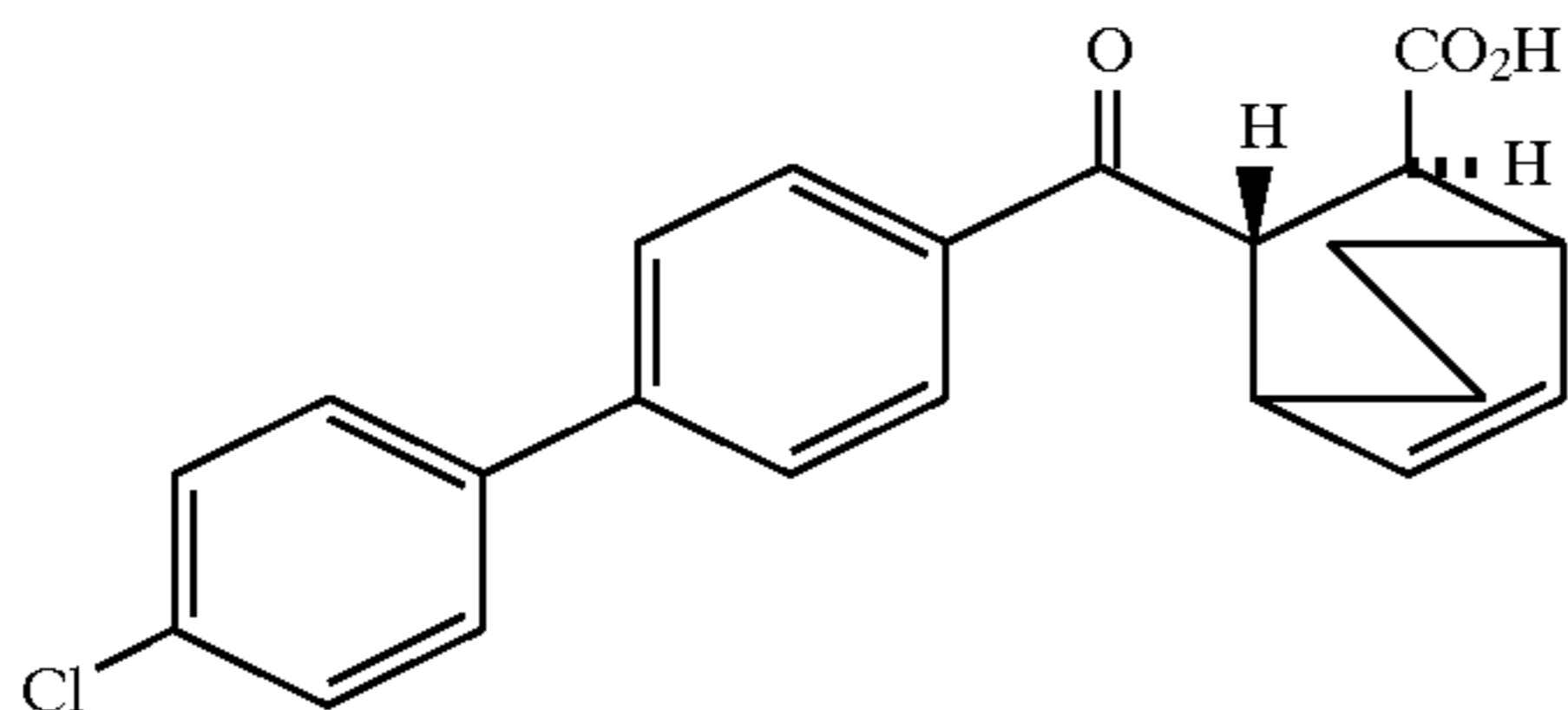
Example 231 (racemate)
