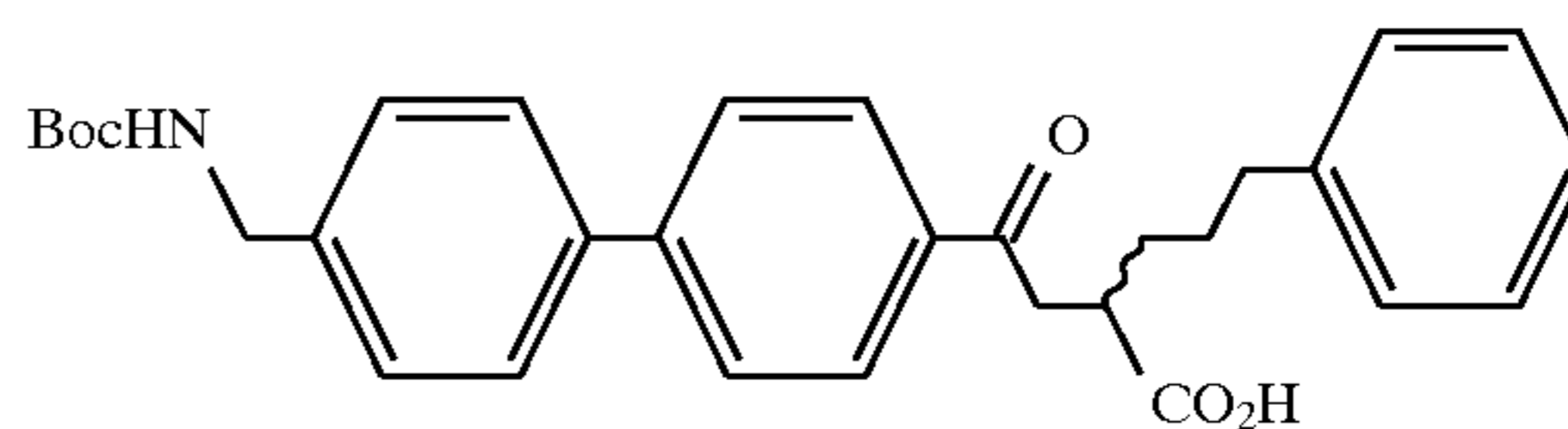
Example 49
