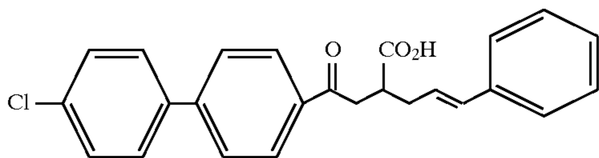
Example 111
