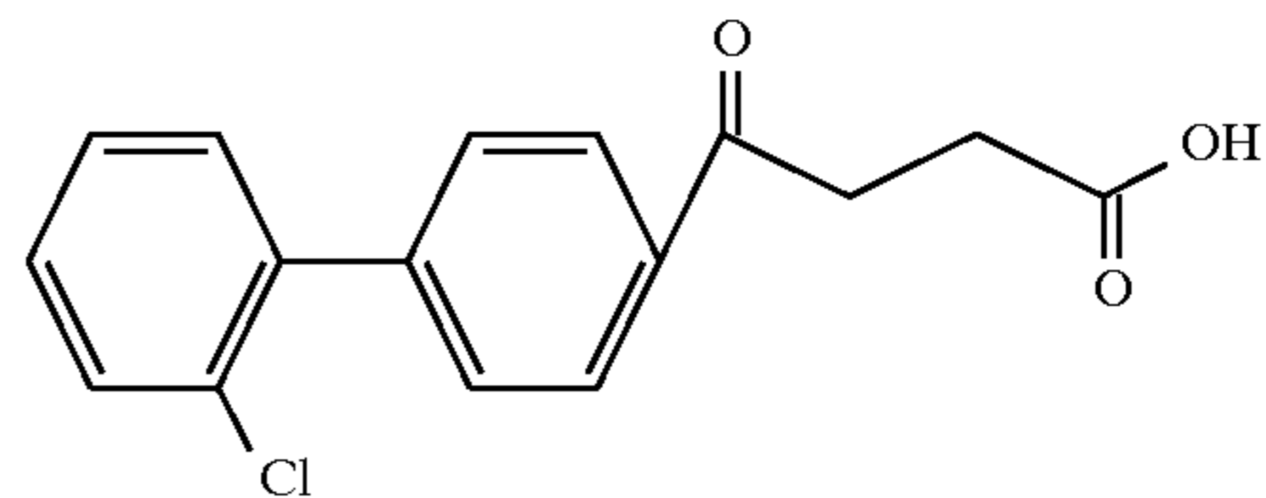
Example 10
