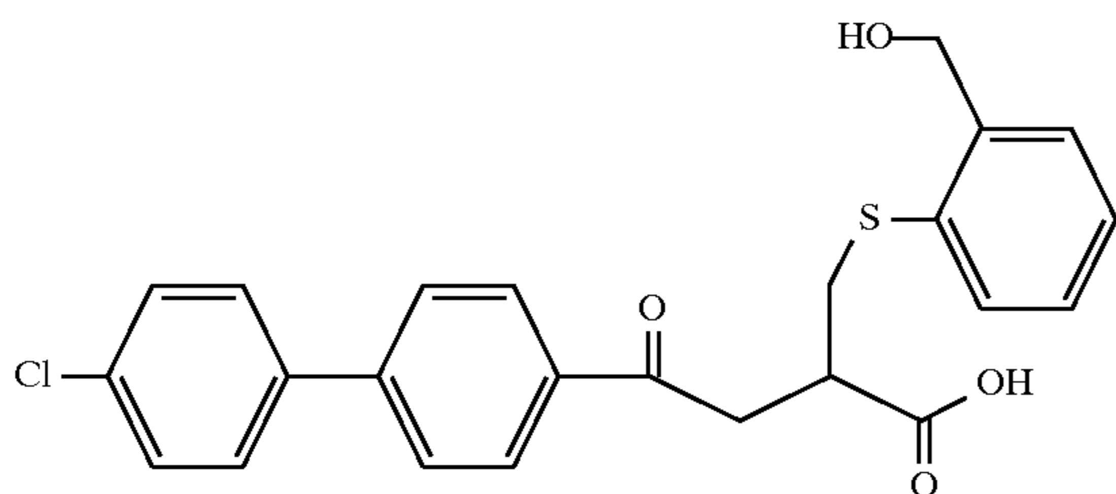
Example 147
