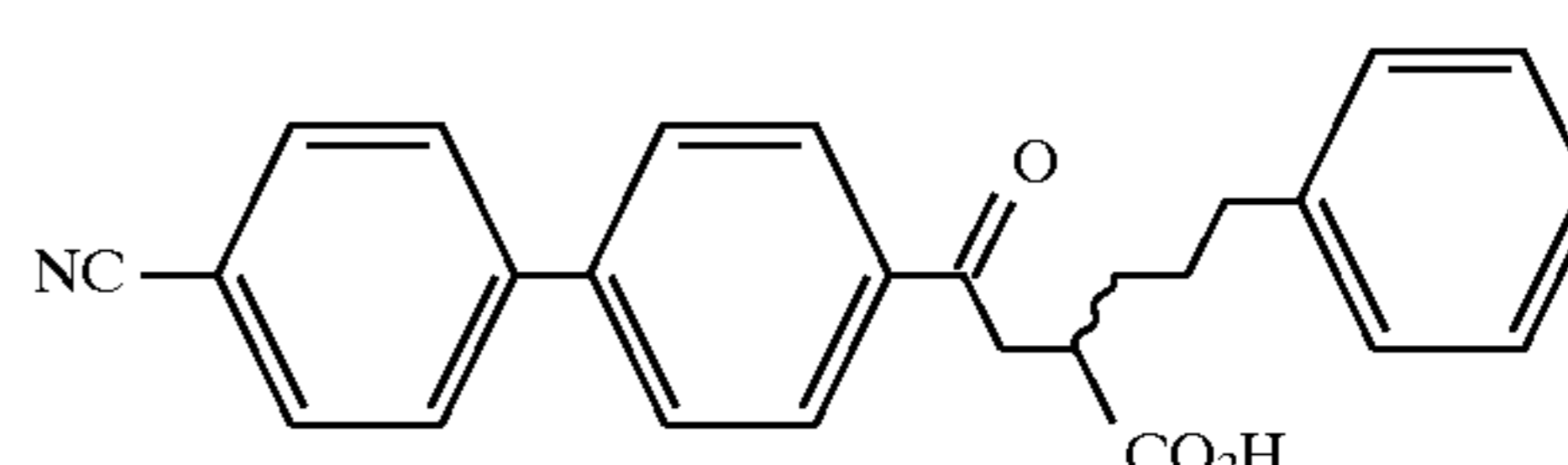
Example 56
