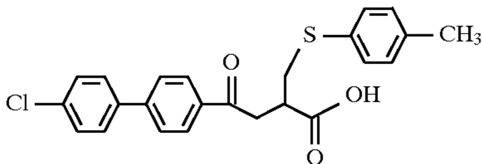
Example 141
