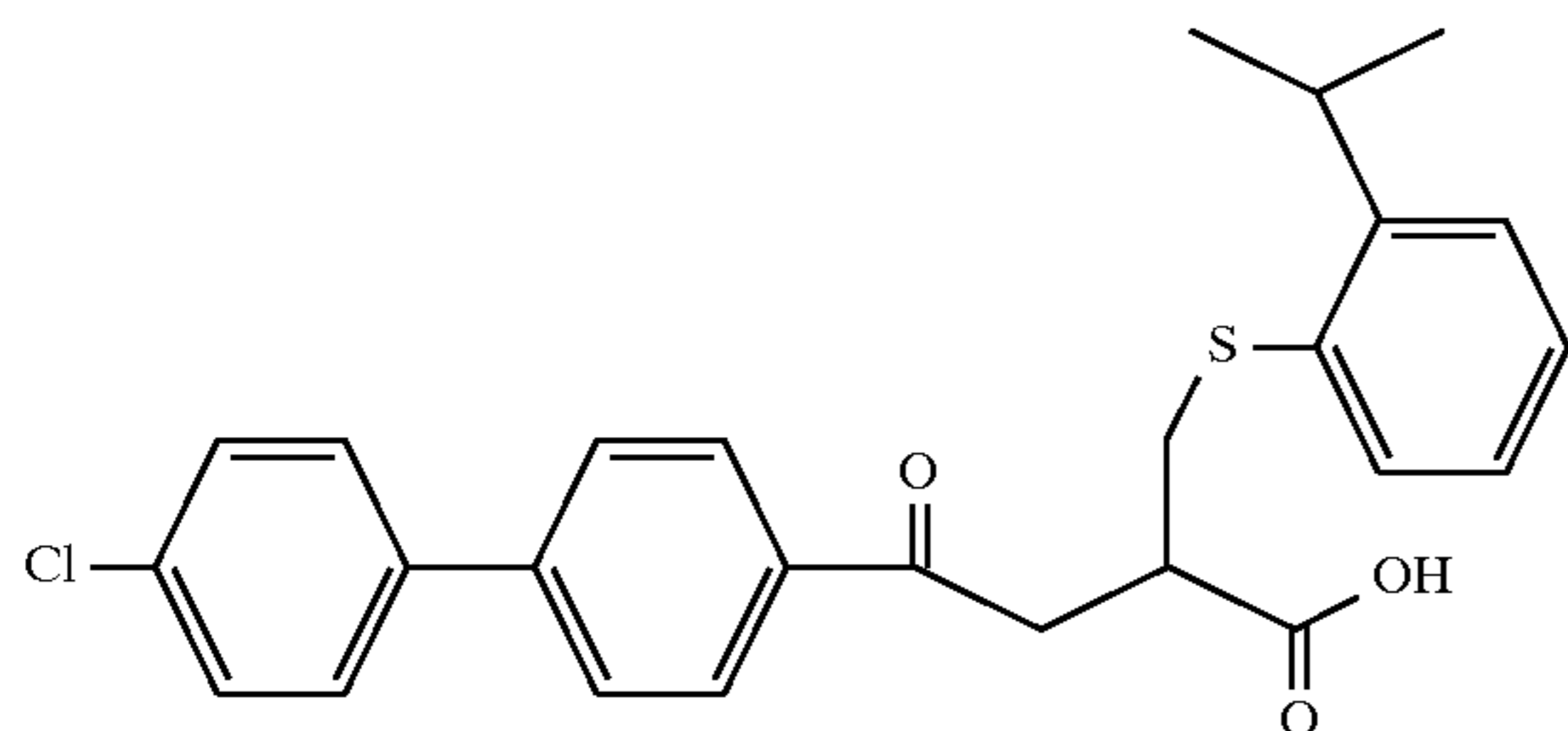
Example 151
