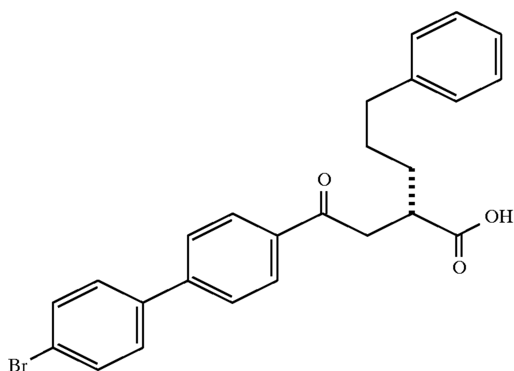
Example 90
