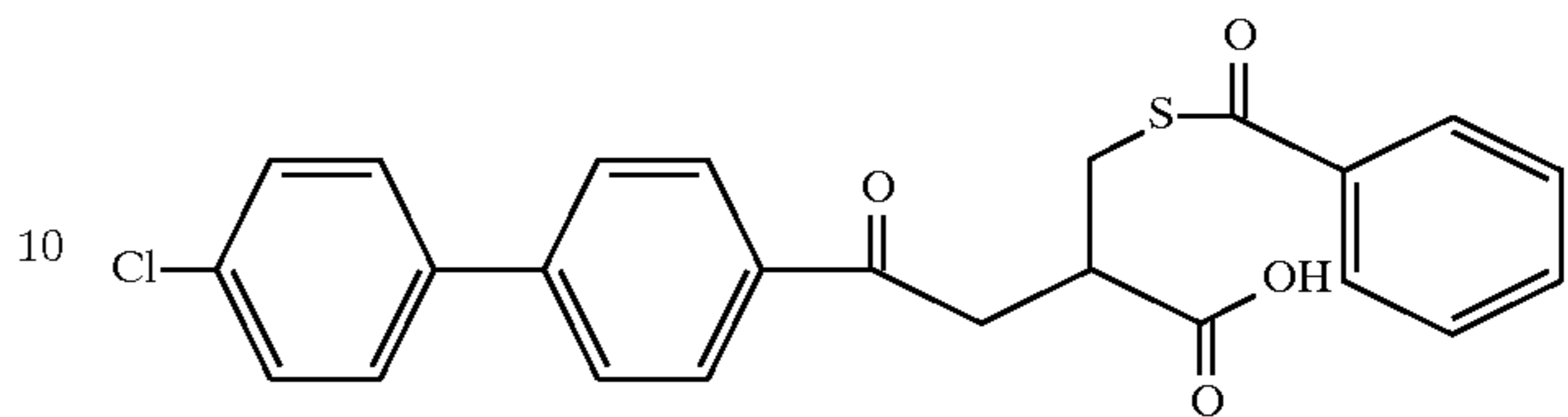
Example 132
