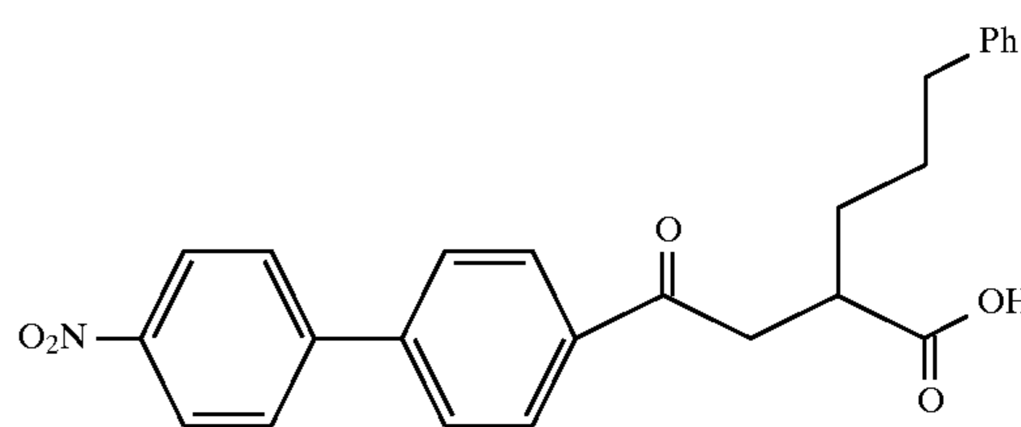
Example 63
