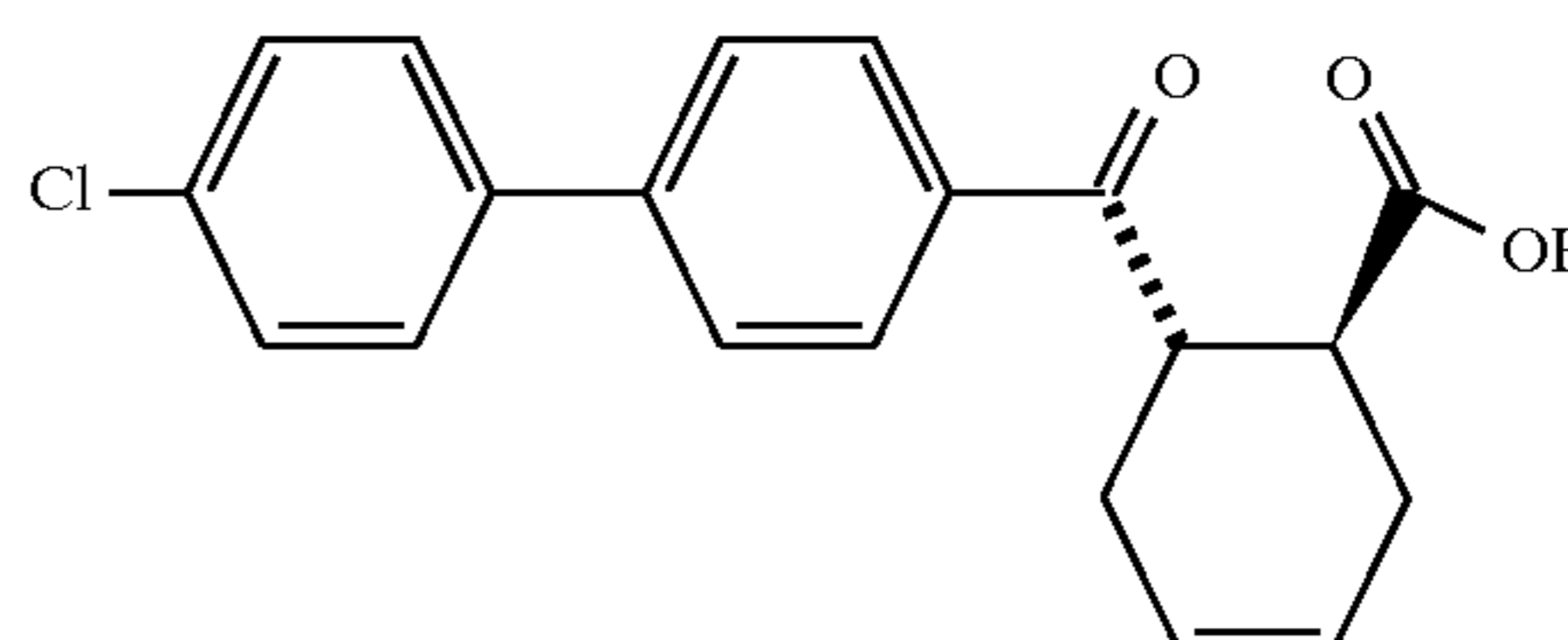
Example 229 (racemate)
