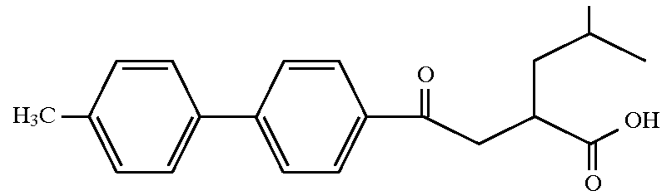
Example 21
