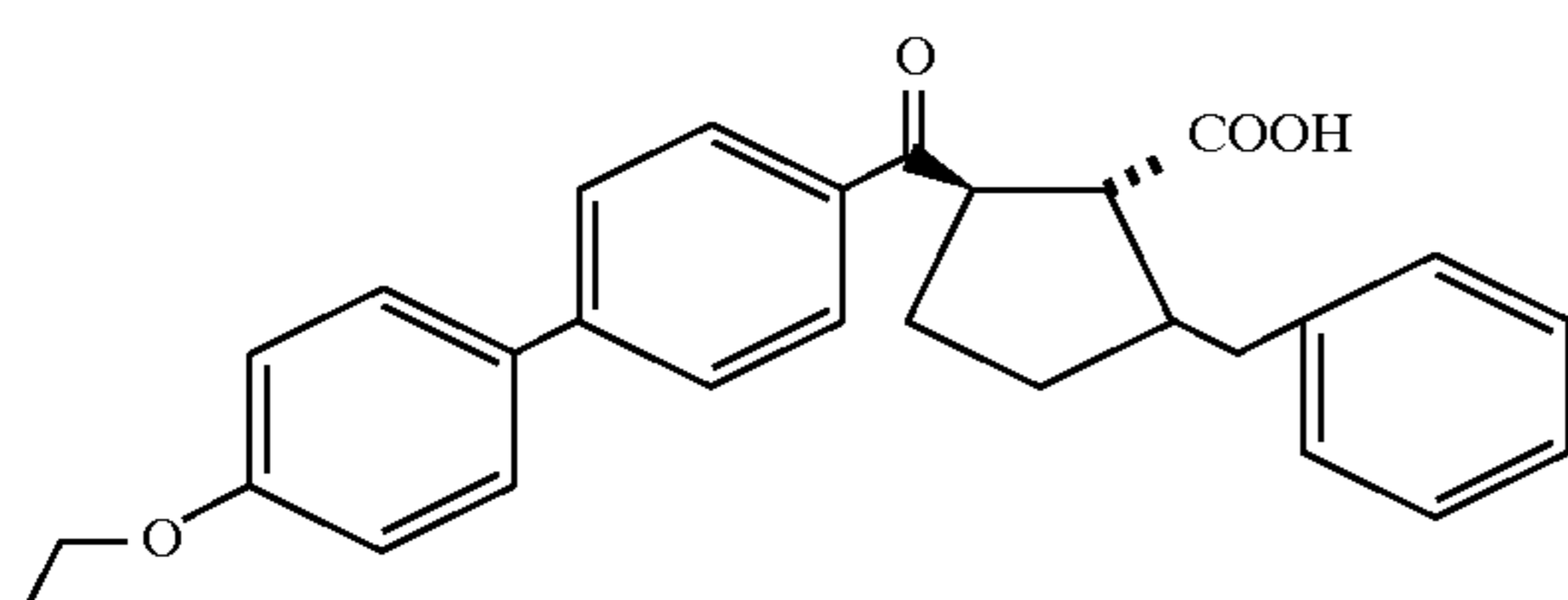
Example 226 (racemate)
