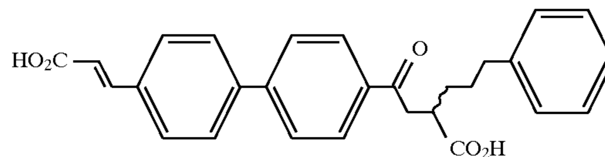
Example 43
