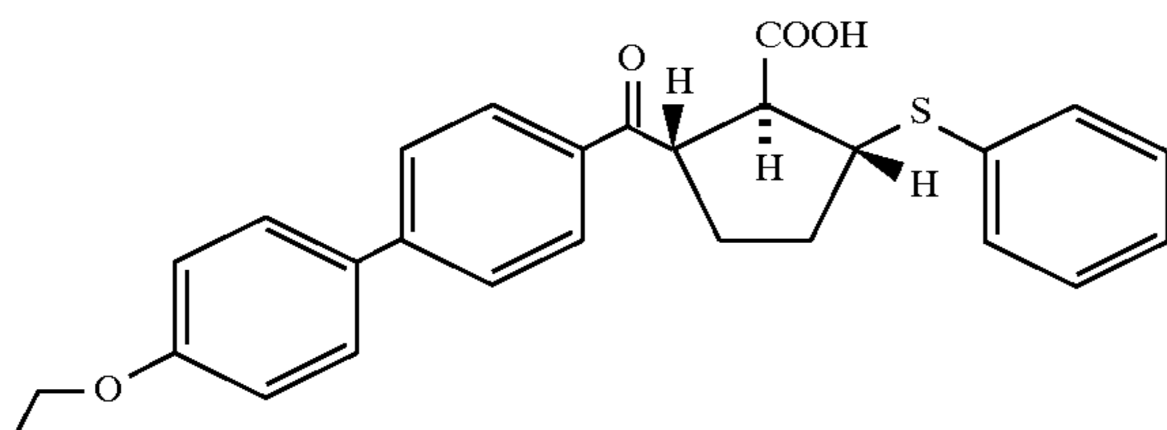
Example 224 (racemate)
