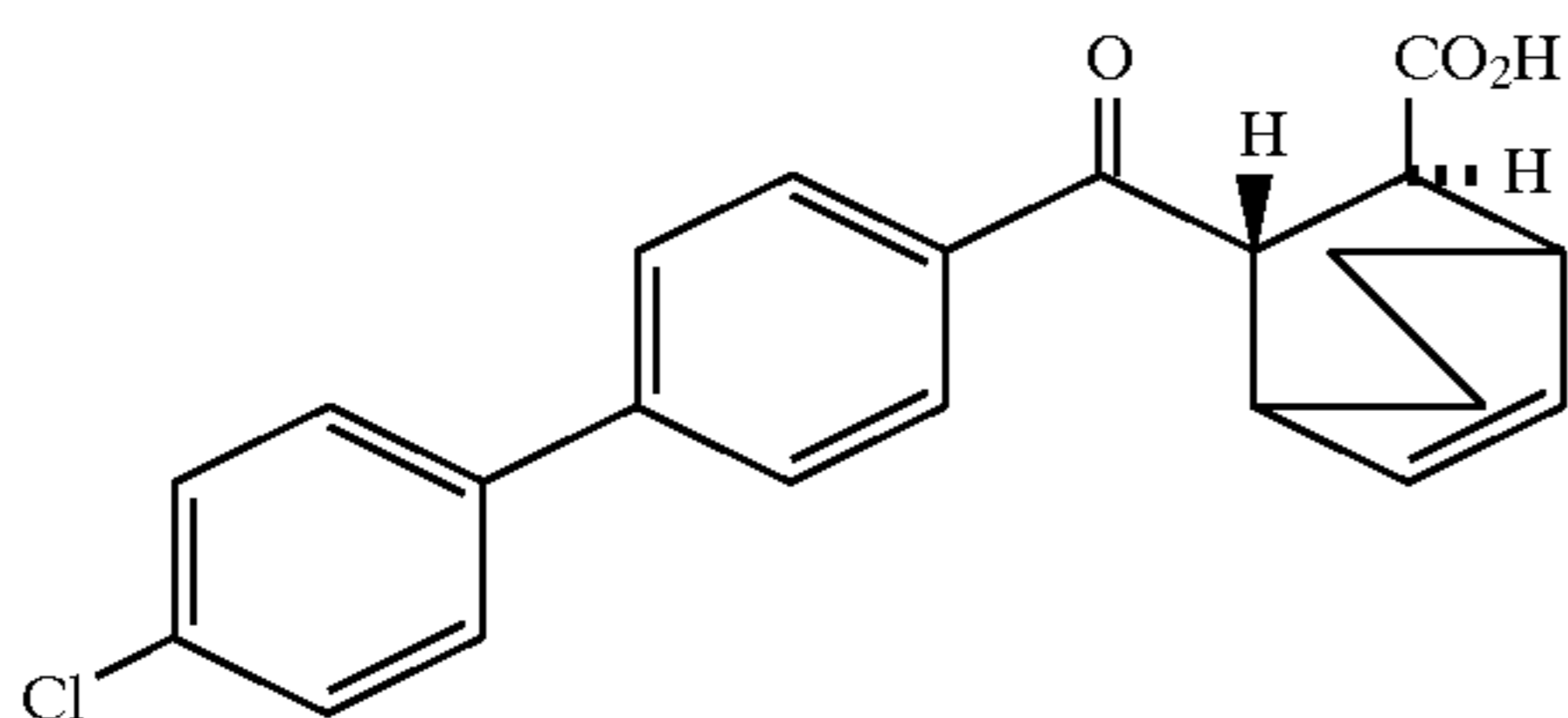
Example 231 (racemate)
