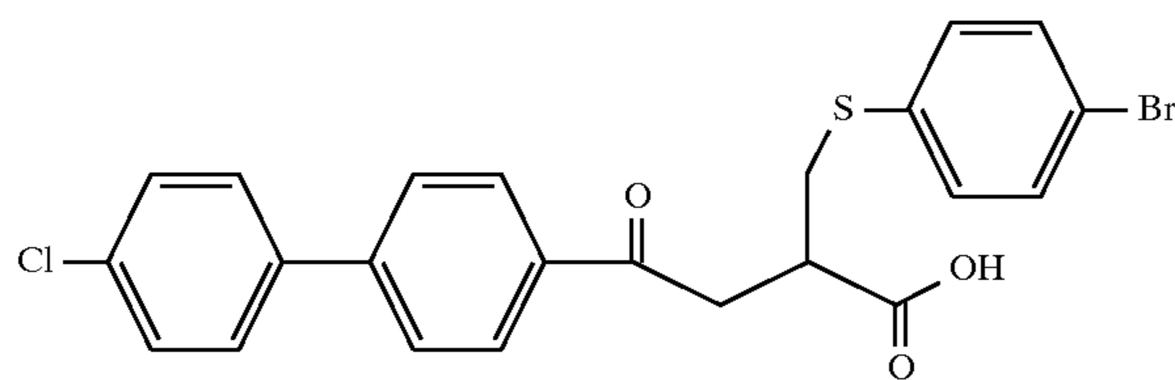
Example 140
