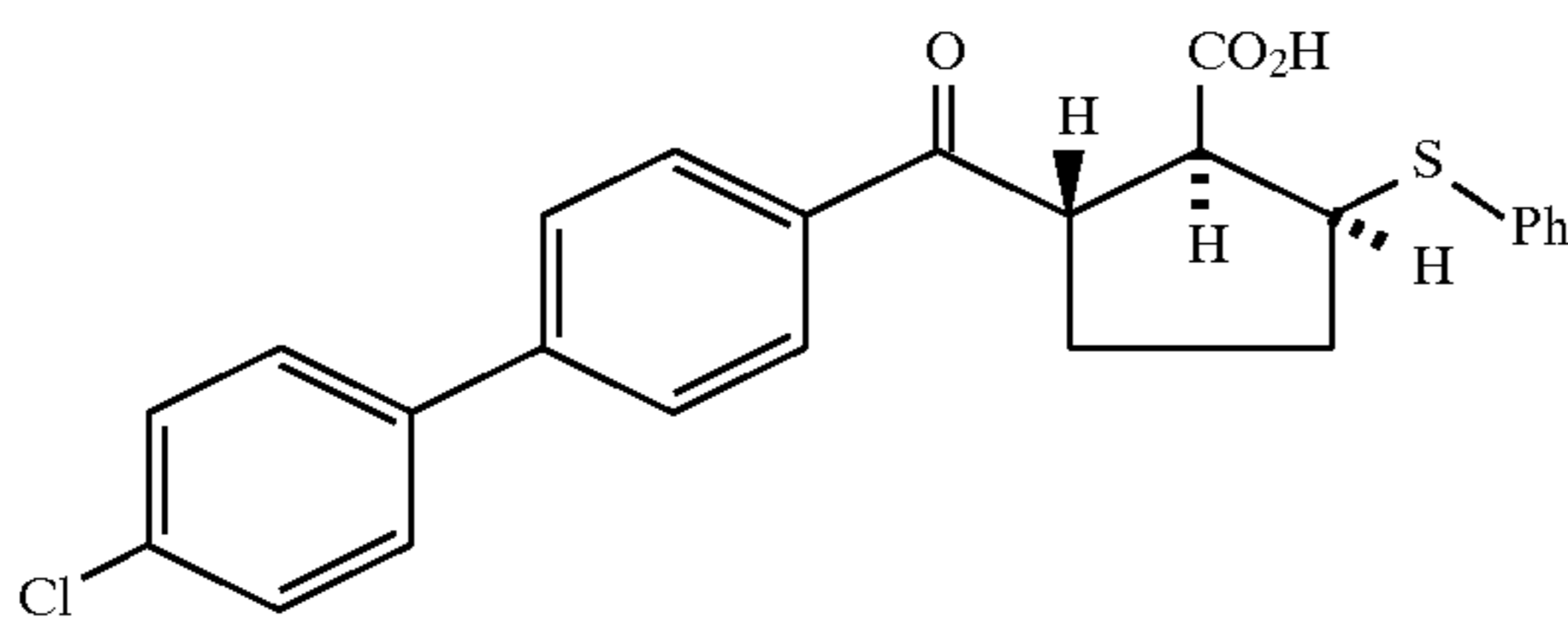
Example 210 (racemate)
