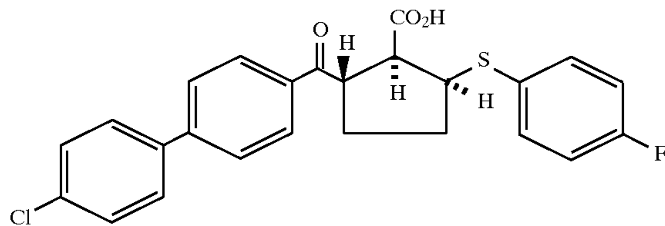
Example 215 (racemate)
