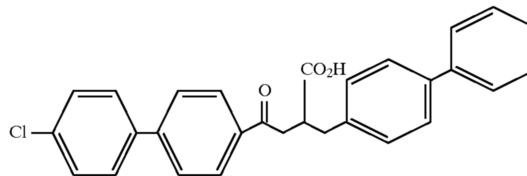
Example 110
