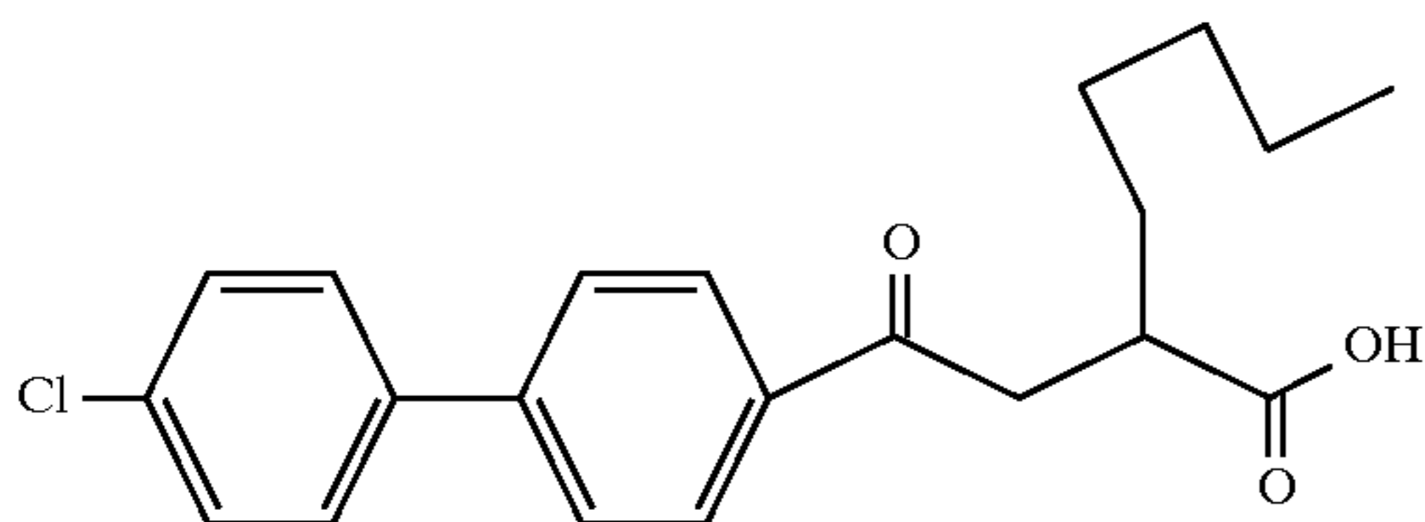
Example 36
