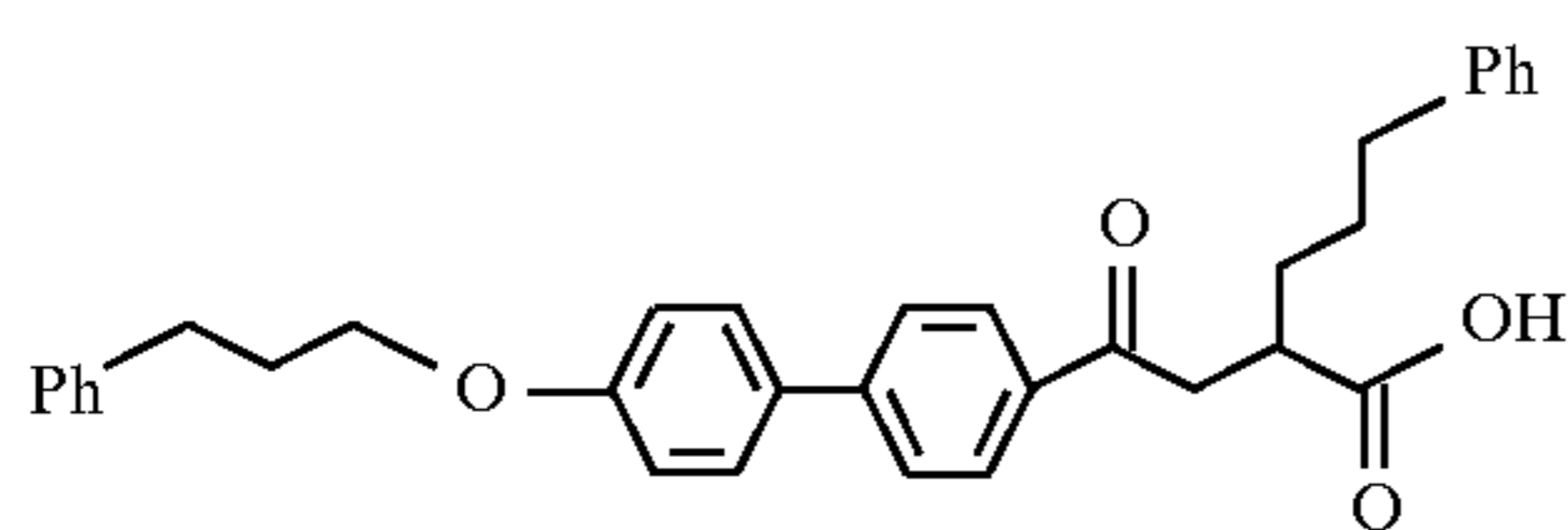
Example 84
