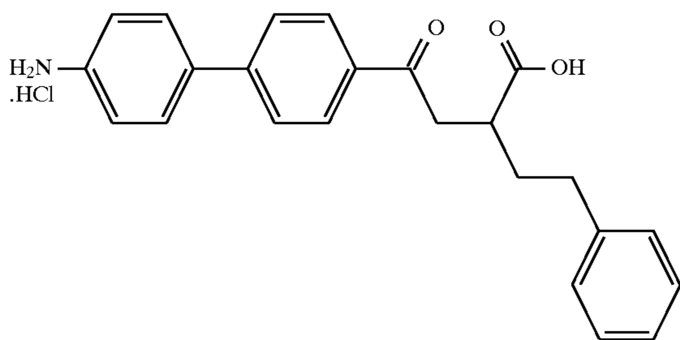
Example 100
