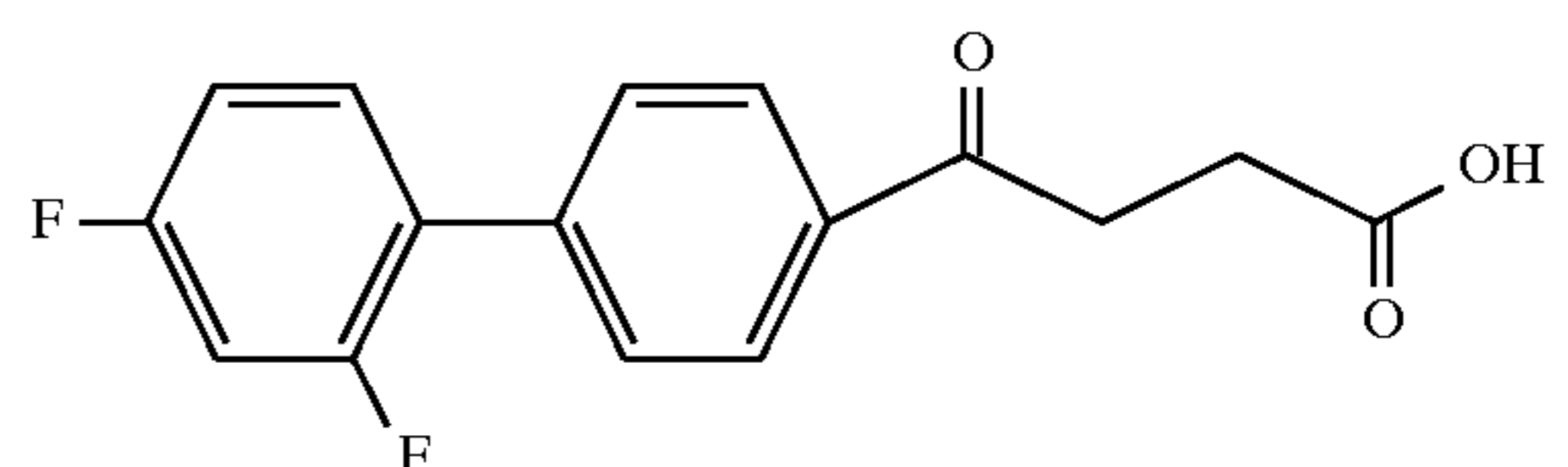
Example 11
