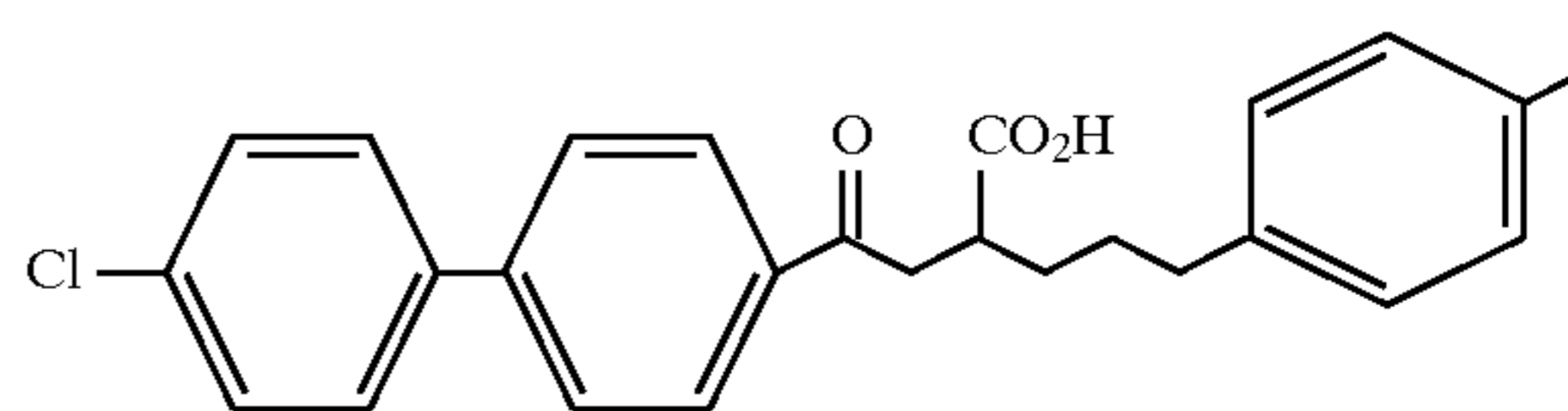
Example 112
