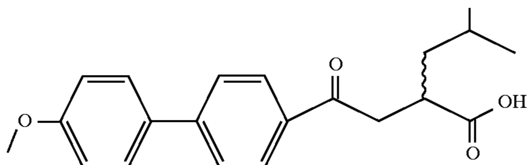
Example 19
