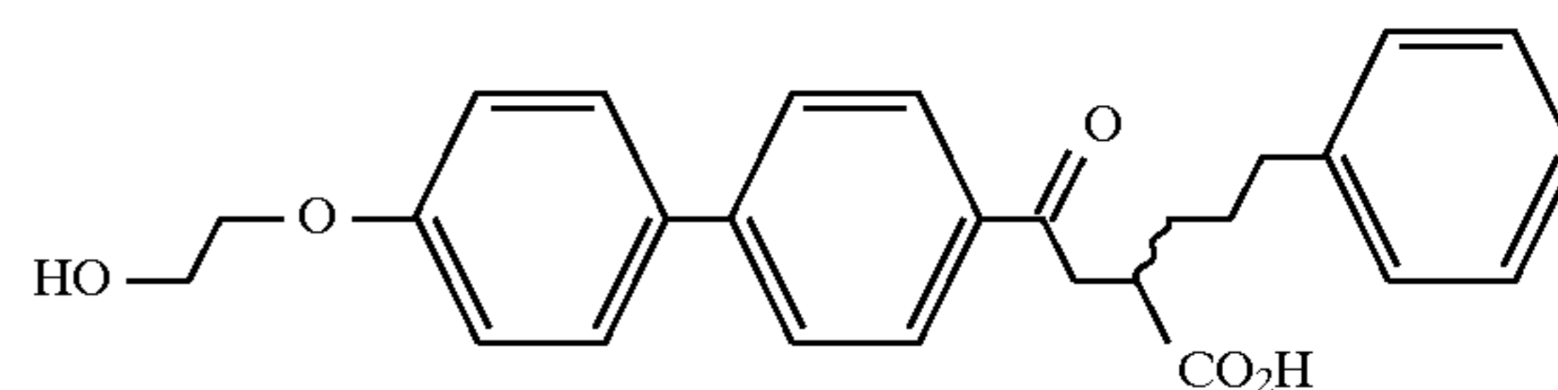
Example 54
