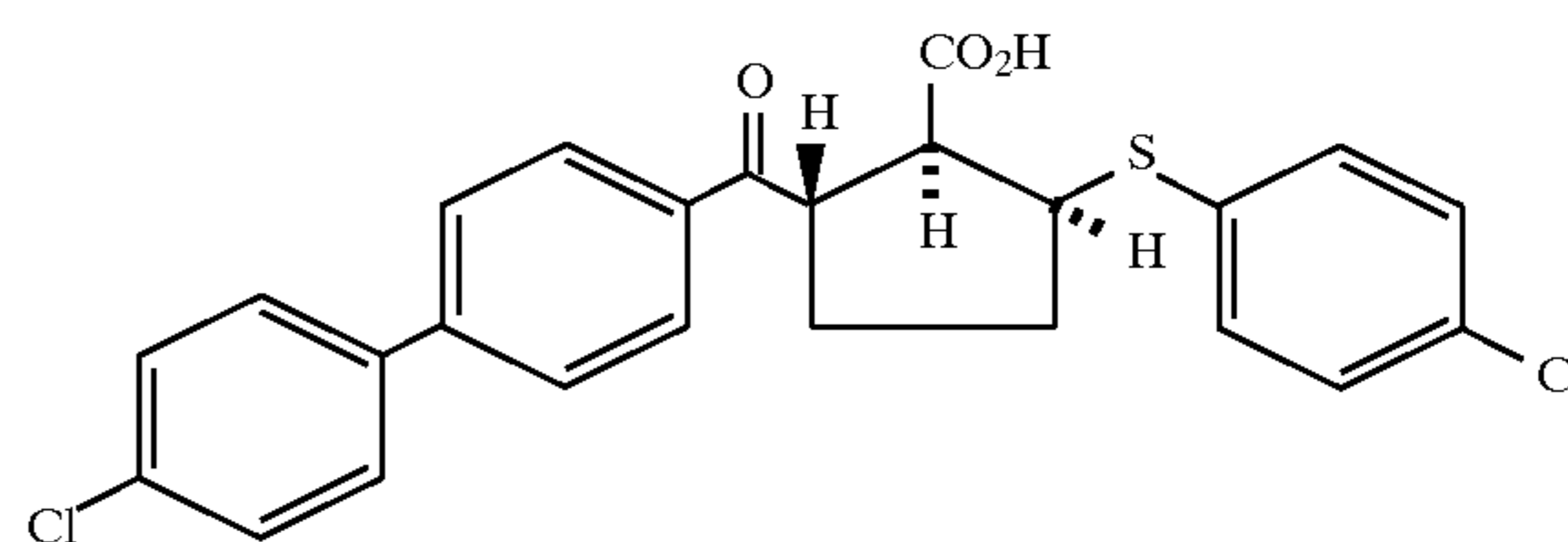
Example 223 (racemate)
