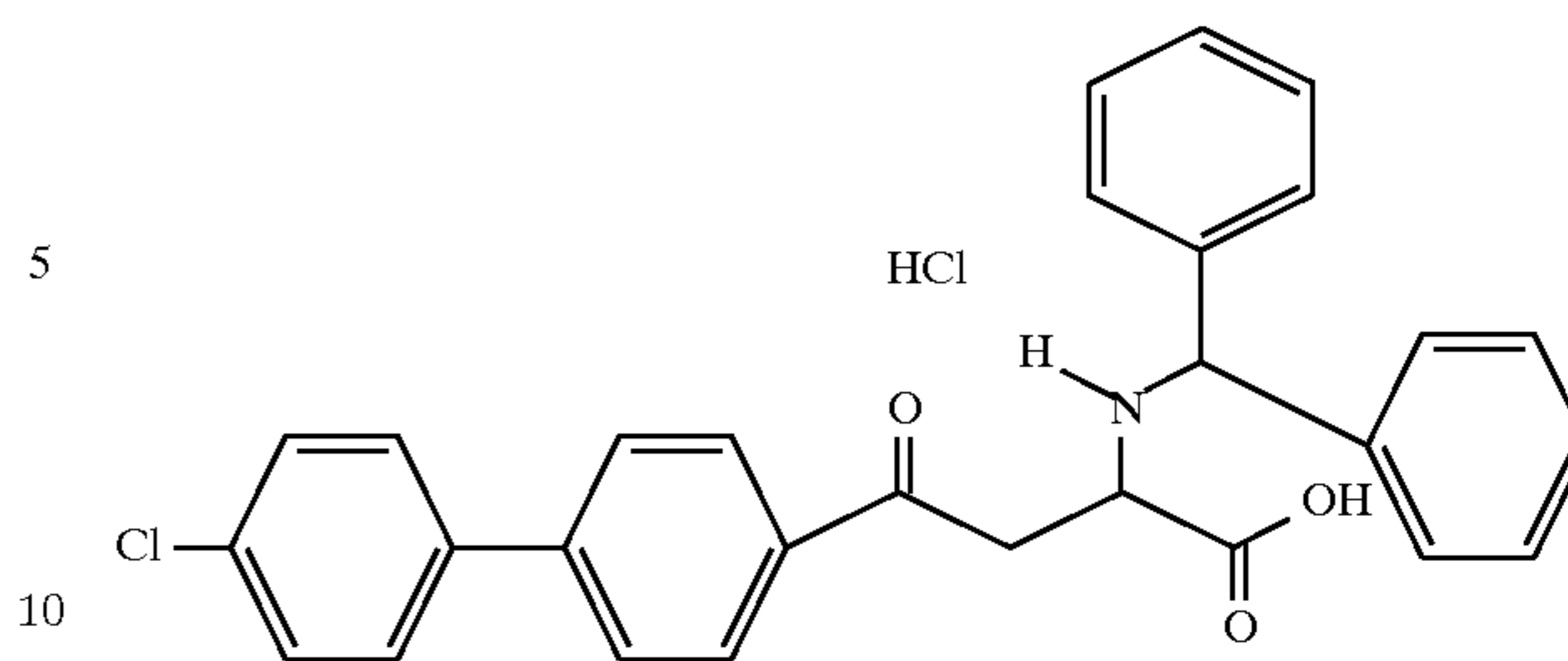
Example 185
