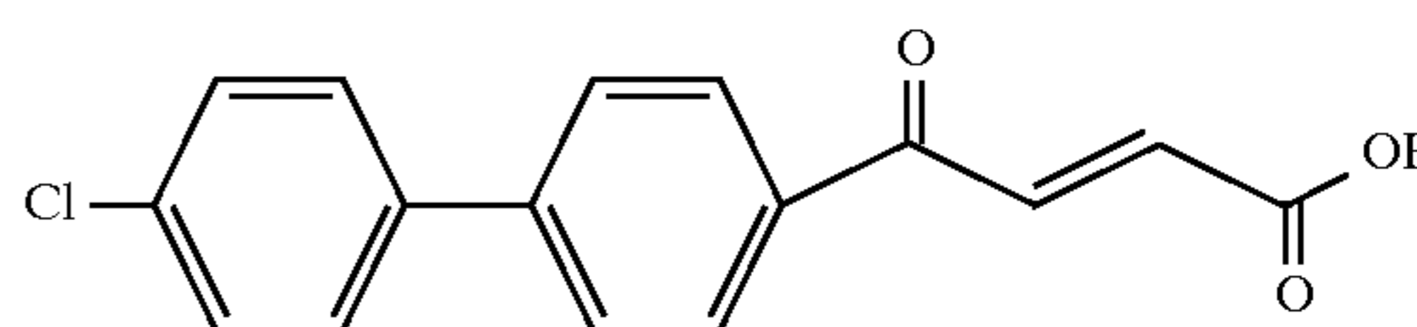
Example 34
