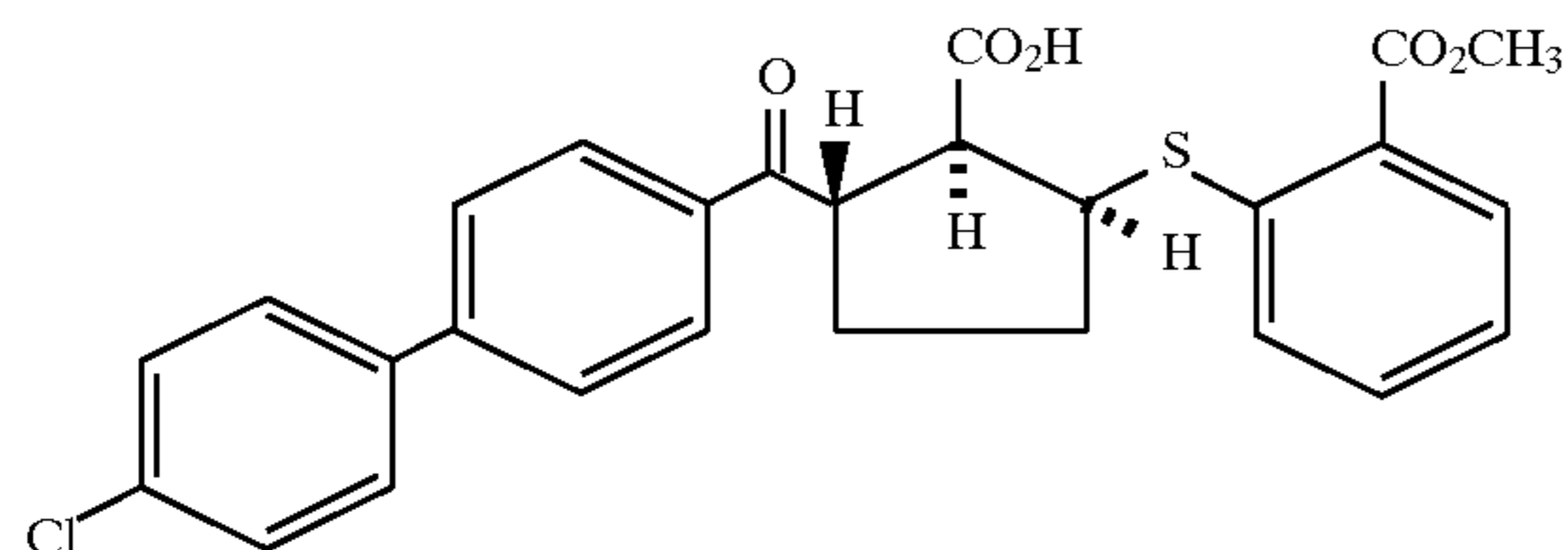
Example 221 (racemate)
