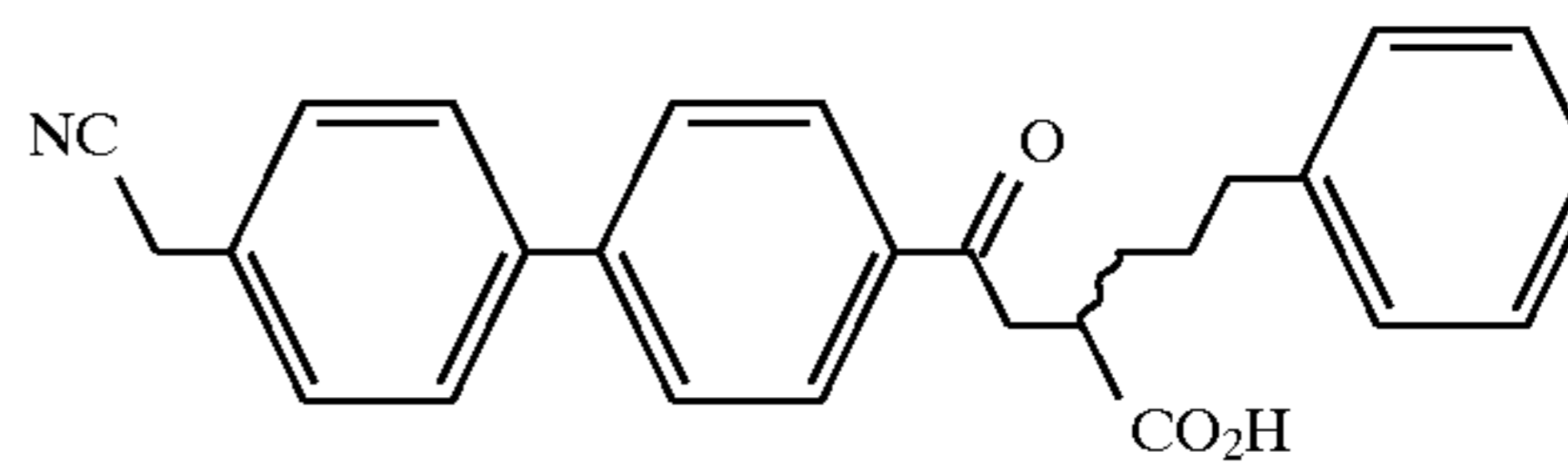
Example 50
