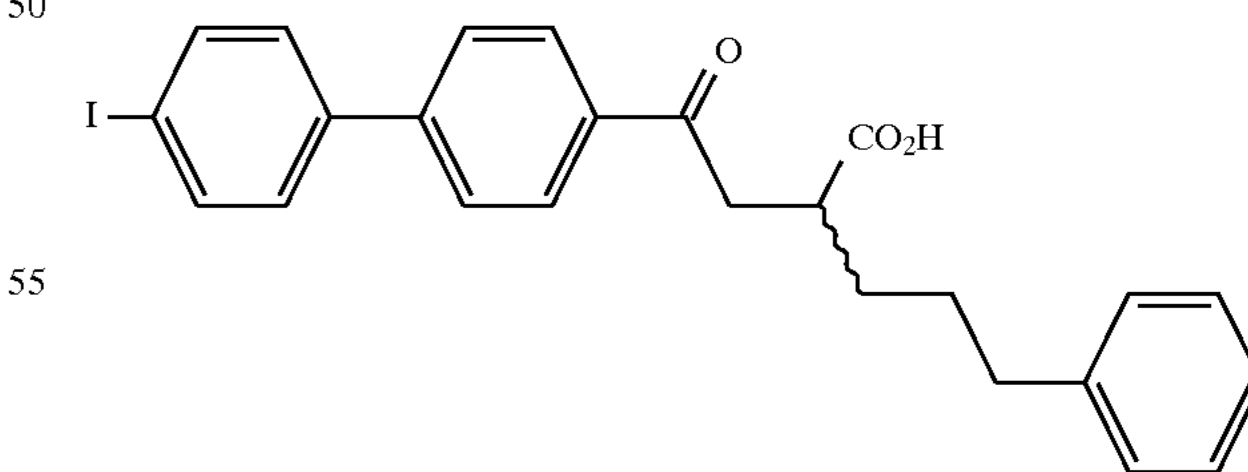
Example 40
