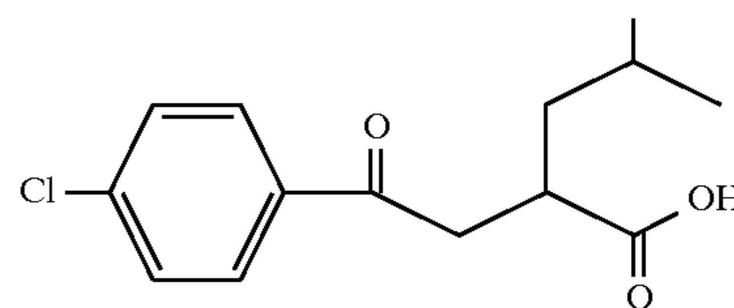
Example 22
