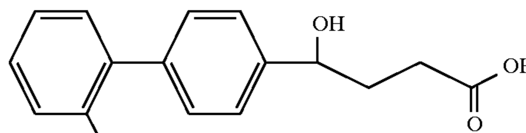
Example 39
