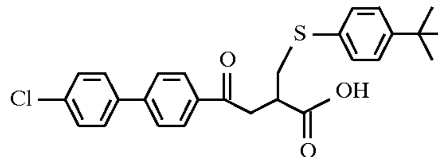
Example 143
