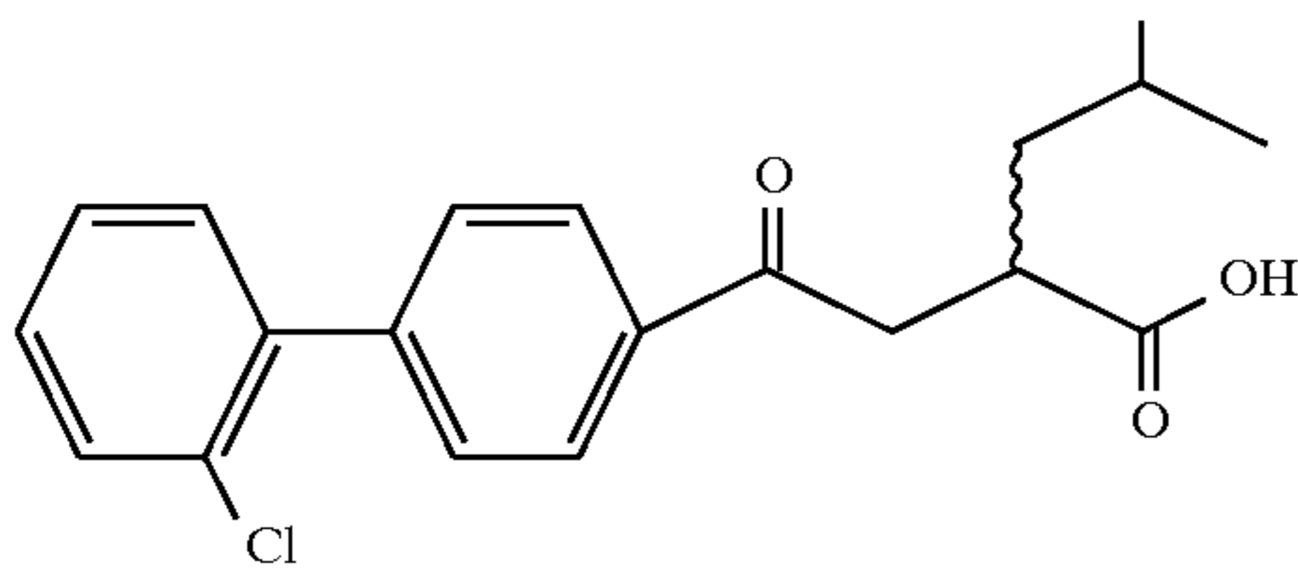
Example 18
