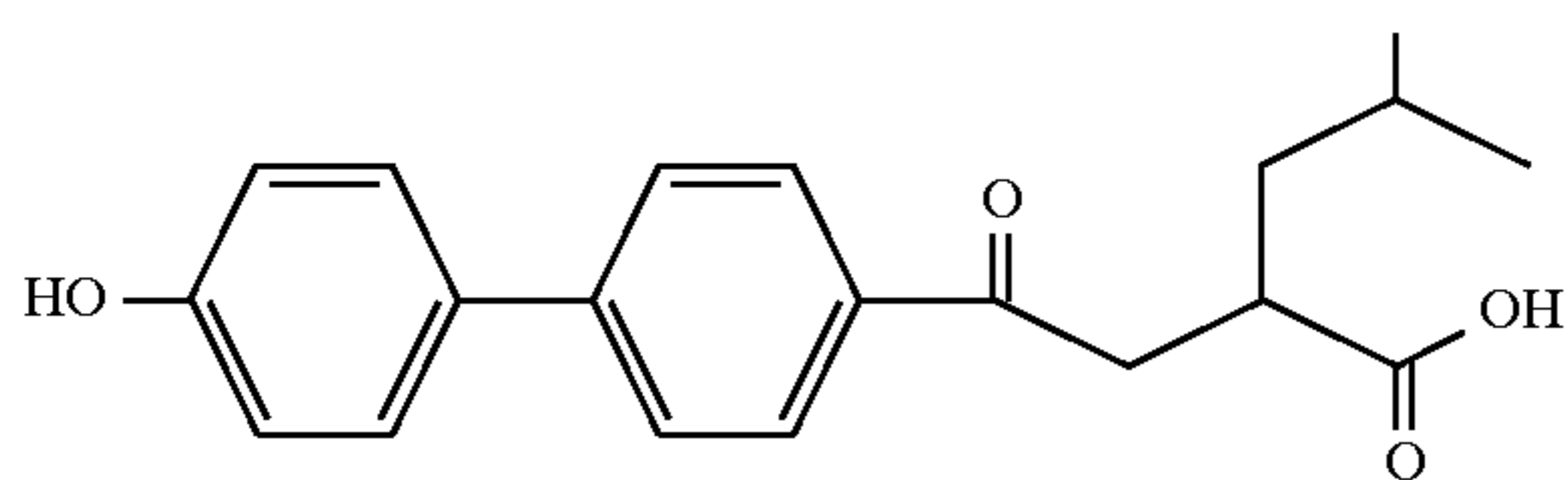
Example 24
