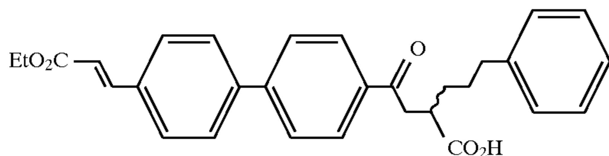
Example 42
