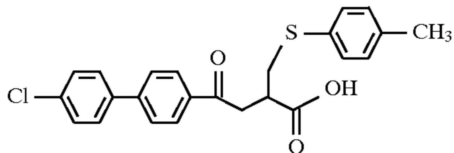
Example 141
