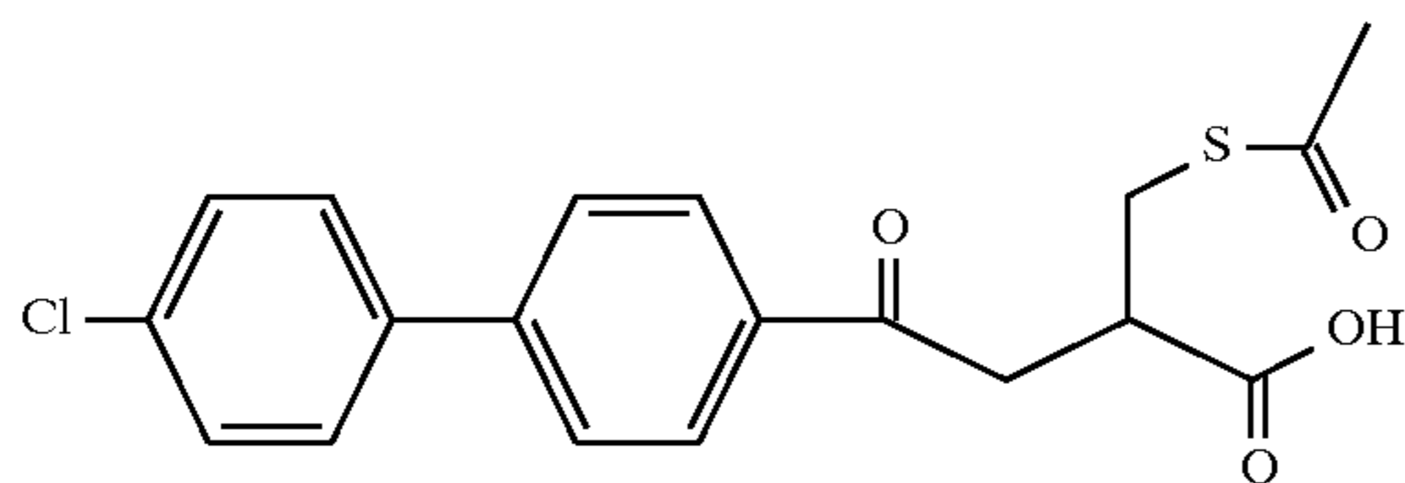
Example 130
