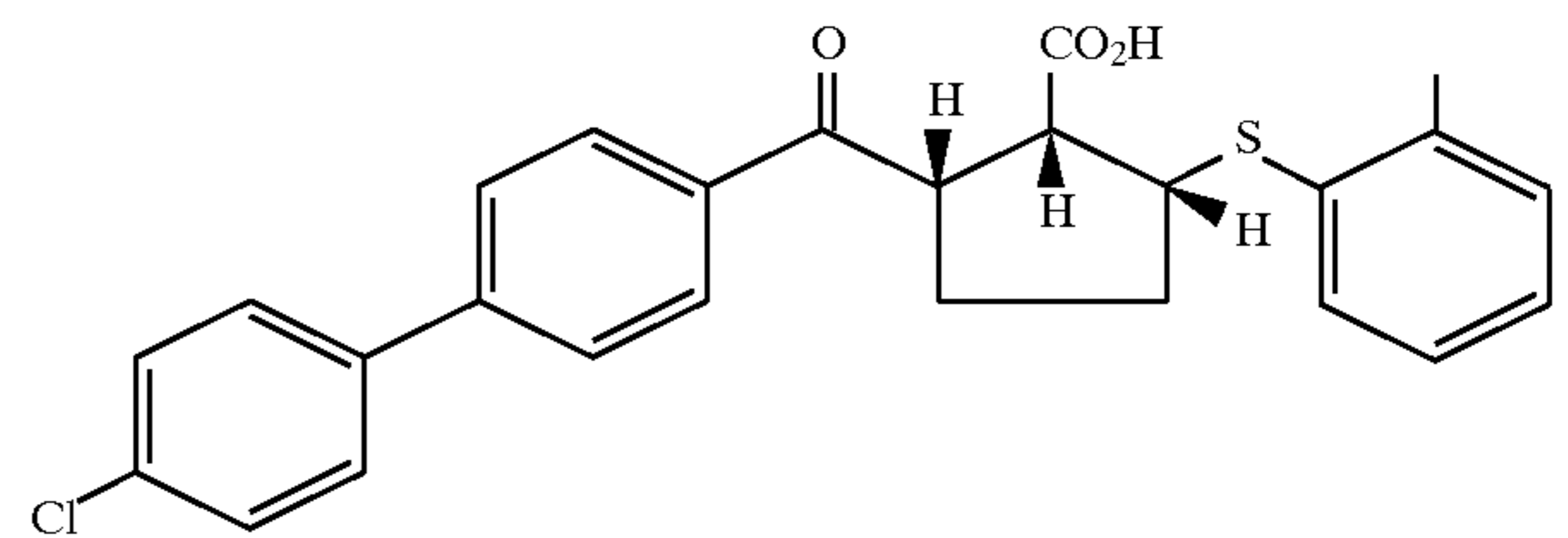
Example 217 (racemate)
