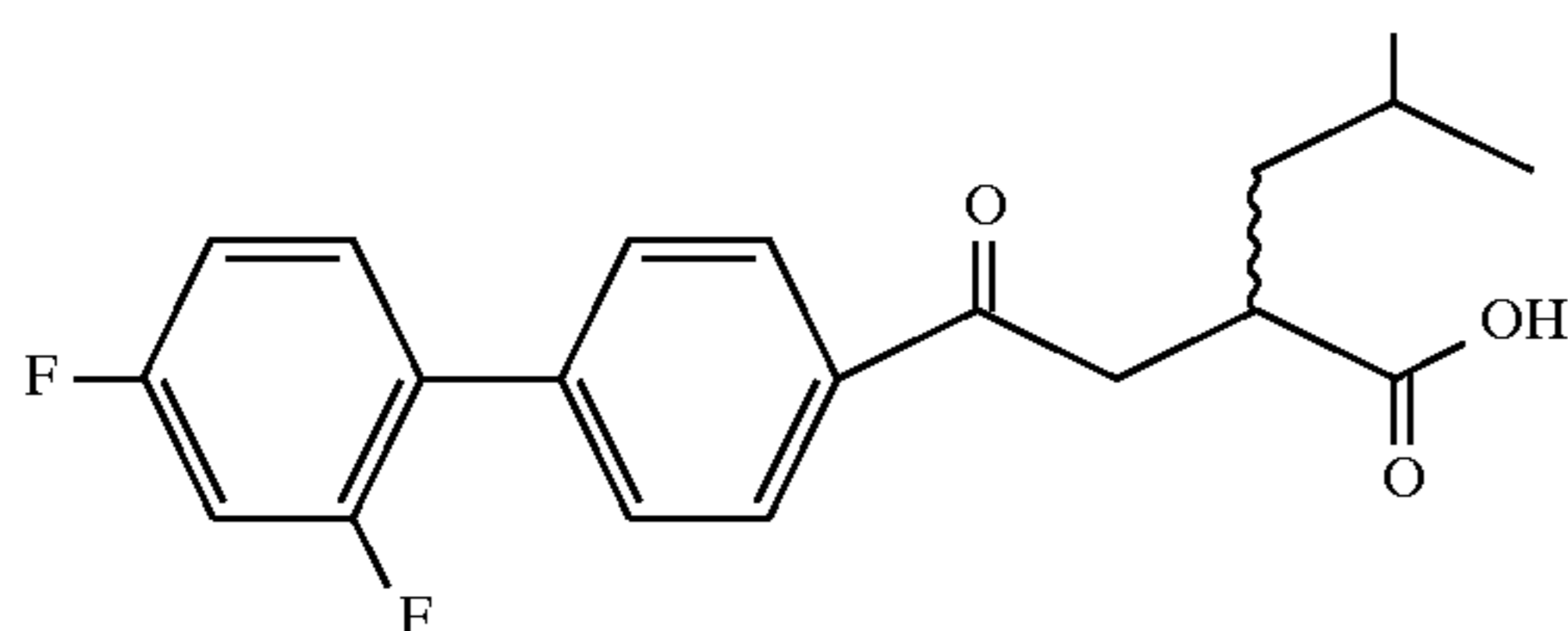
Example 20
