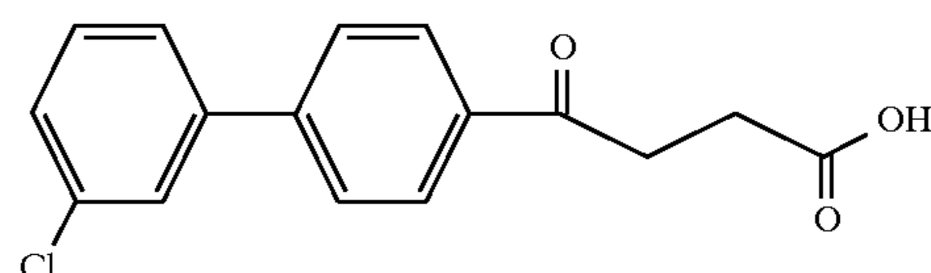
Example 12
