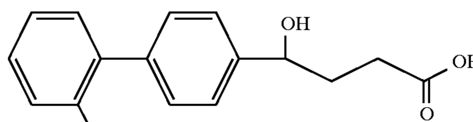
Example 39
