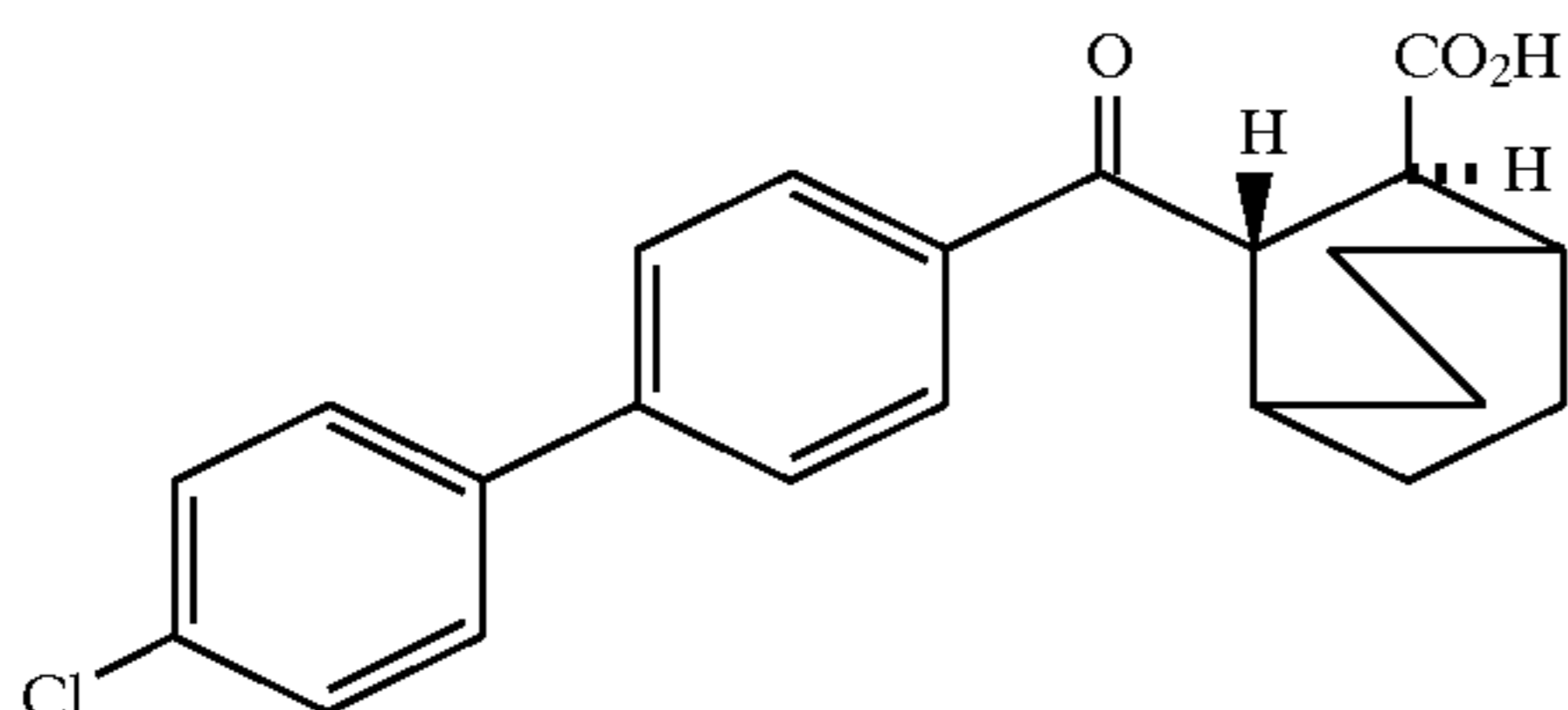
Example 232 (racemate)
