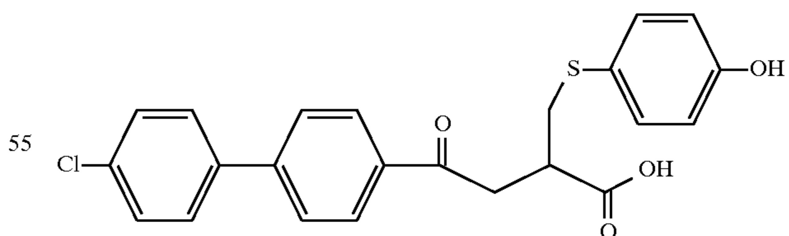
Example 134
