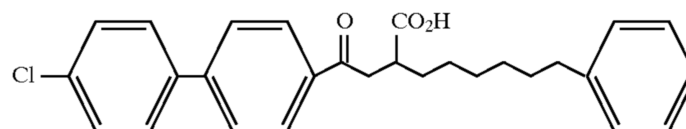
Example 109
