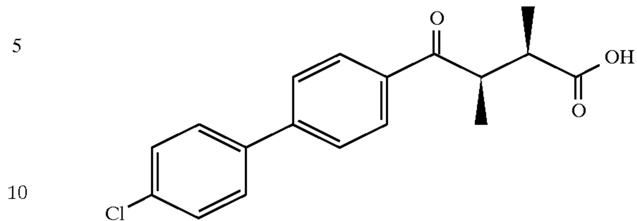
Example 198 (racemate)
