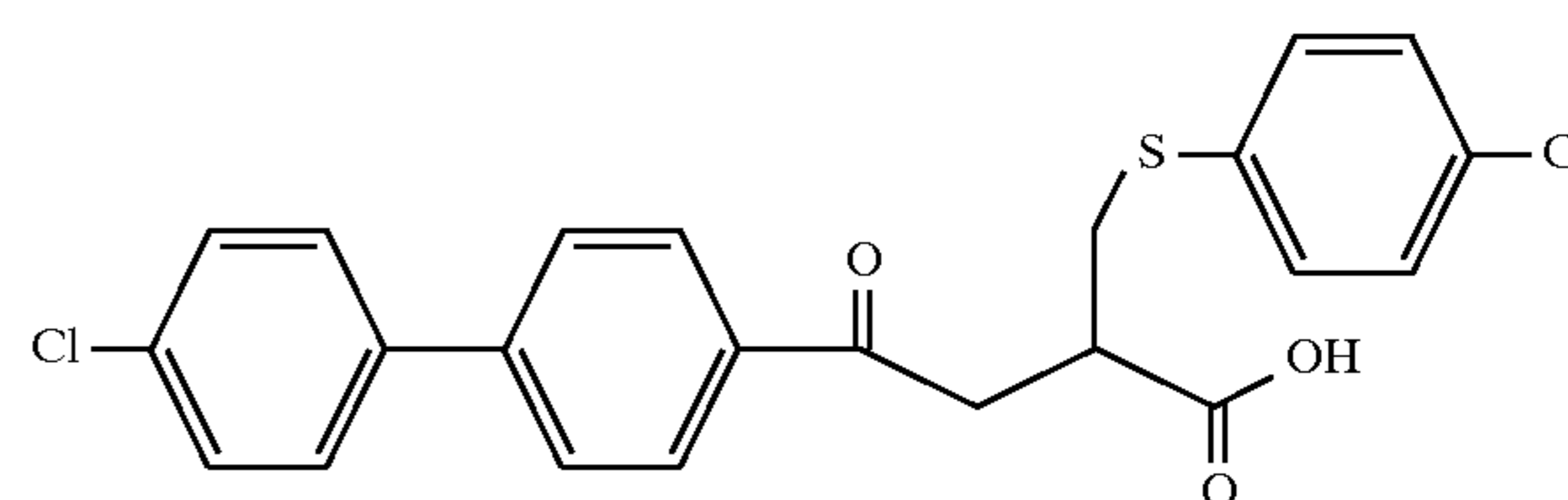
Example 139
