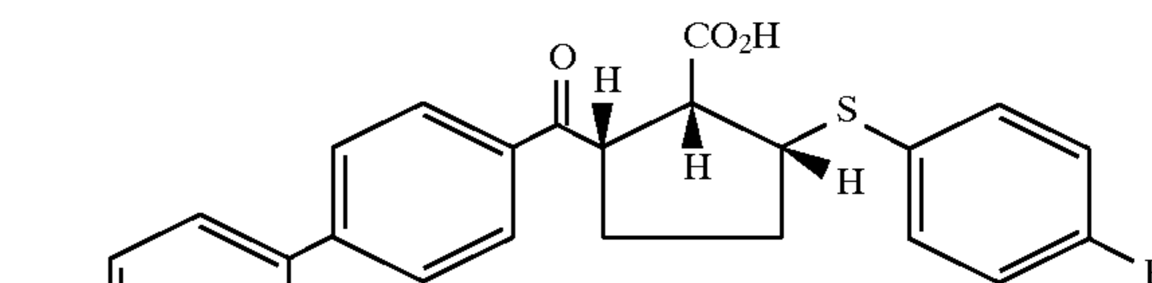
Example 214 (racemate)
