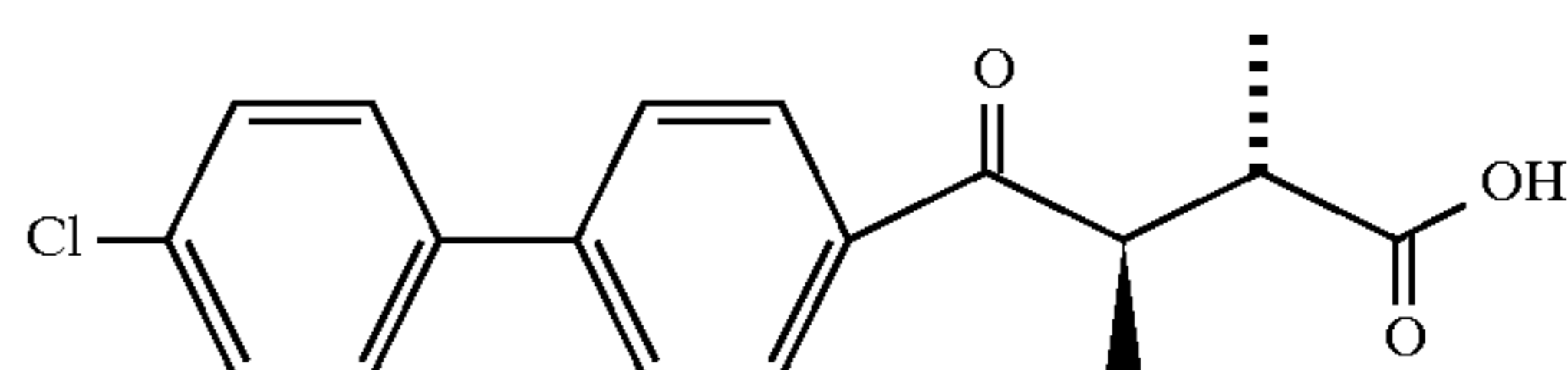
Example 199 (racemate)
