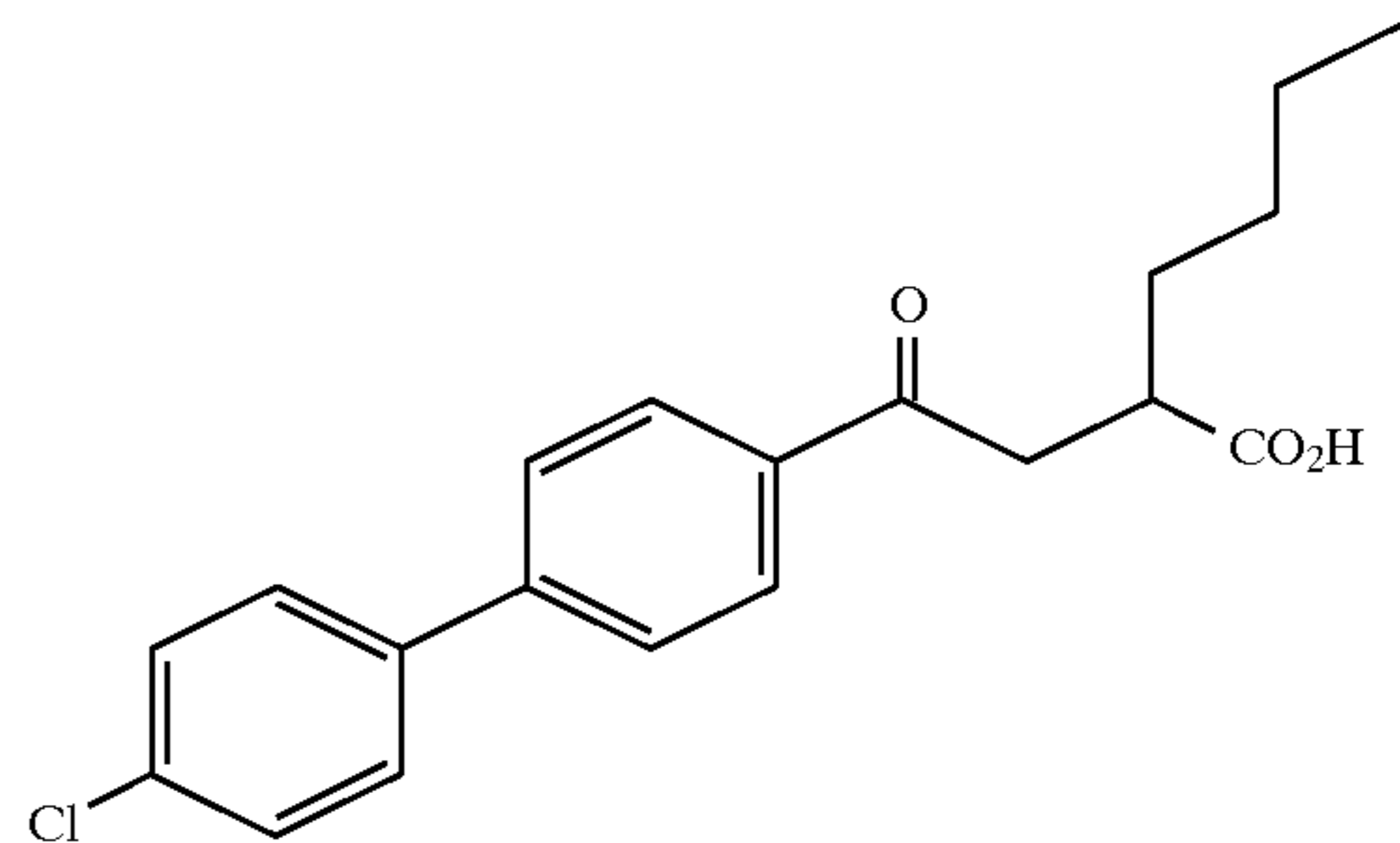
Example 95
