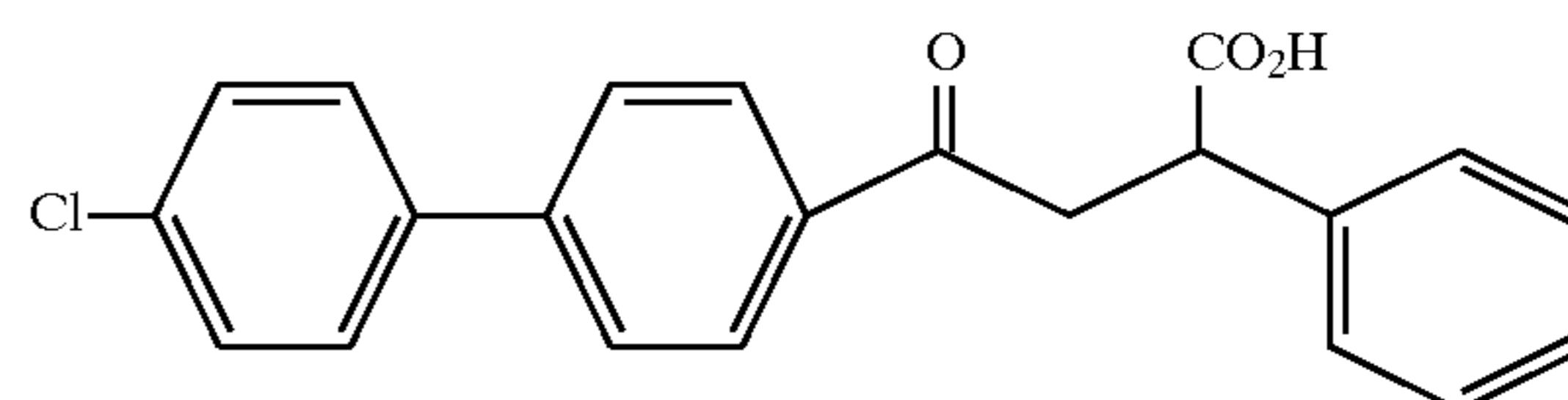
Example 104
