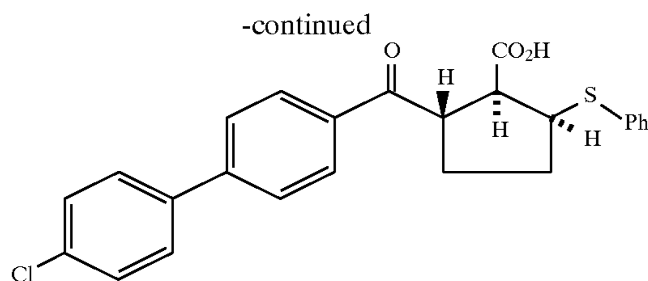
Example 210 (racemate)
