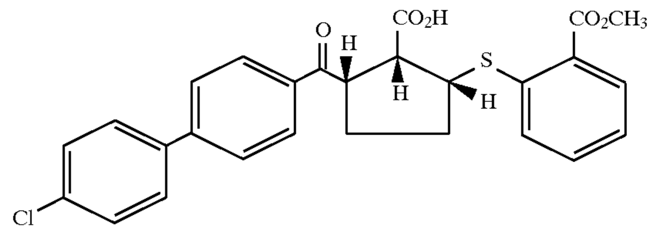
Example 220 (racemate)
