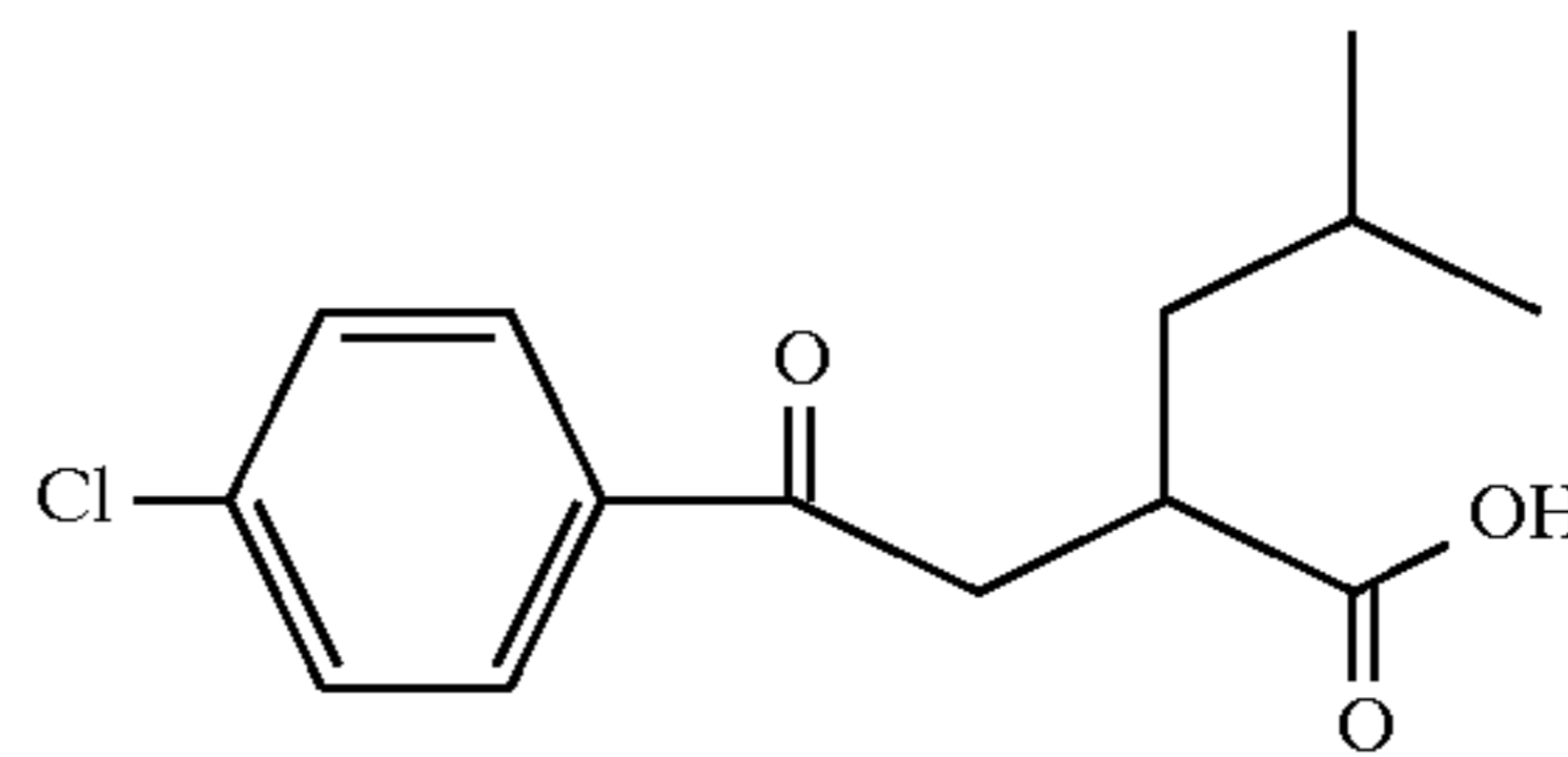
Example 22
