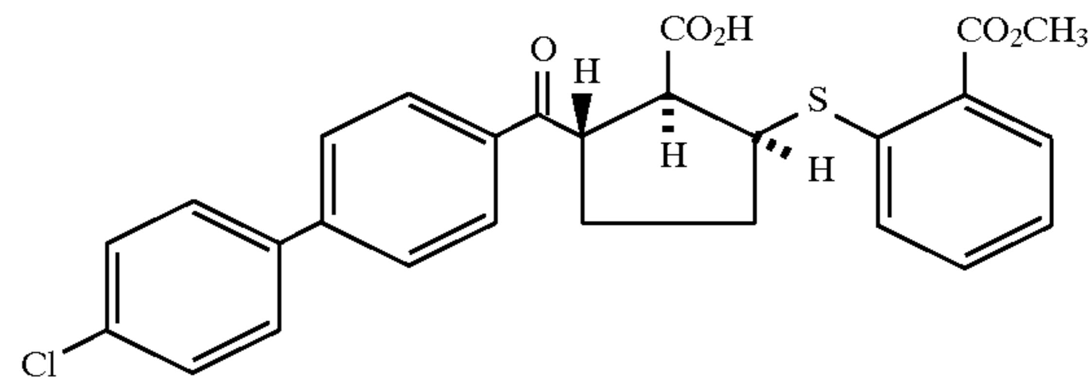
Example 221 (racemate)
