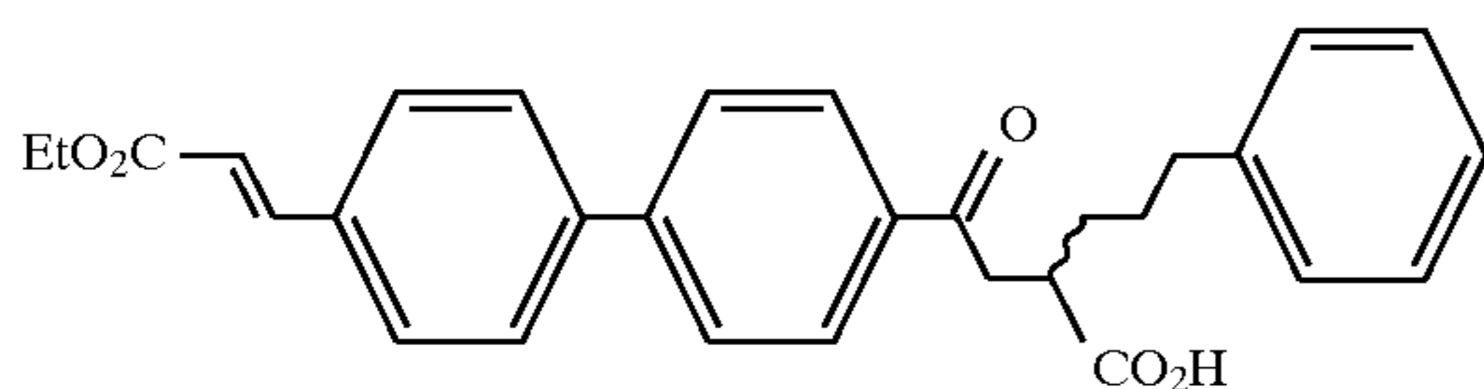
Example 42
