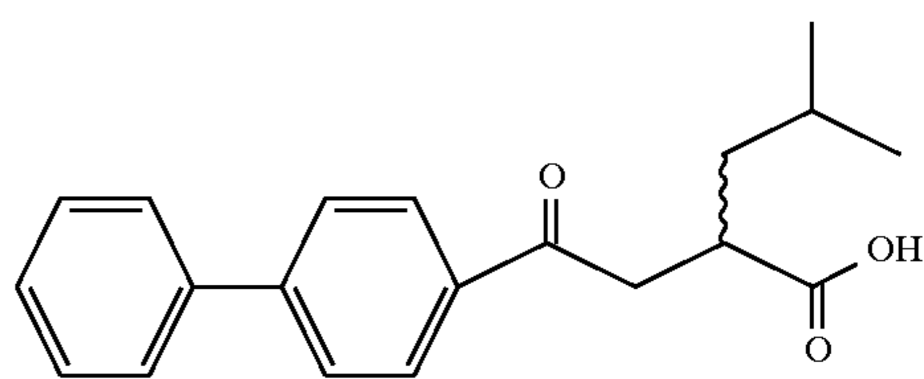
Example 13
