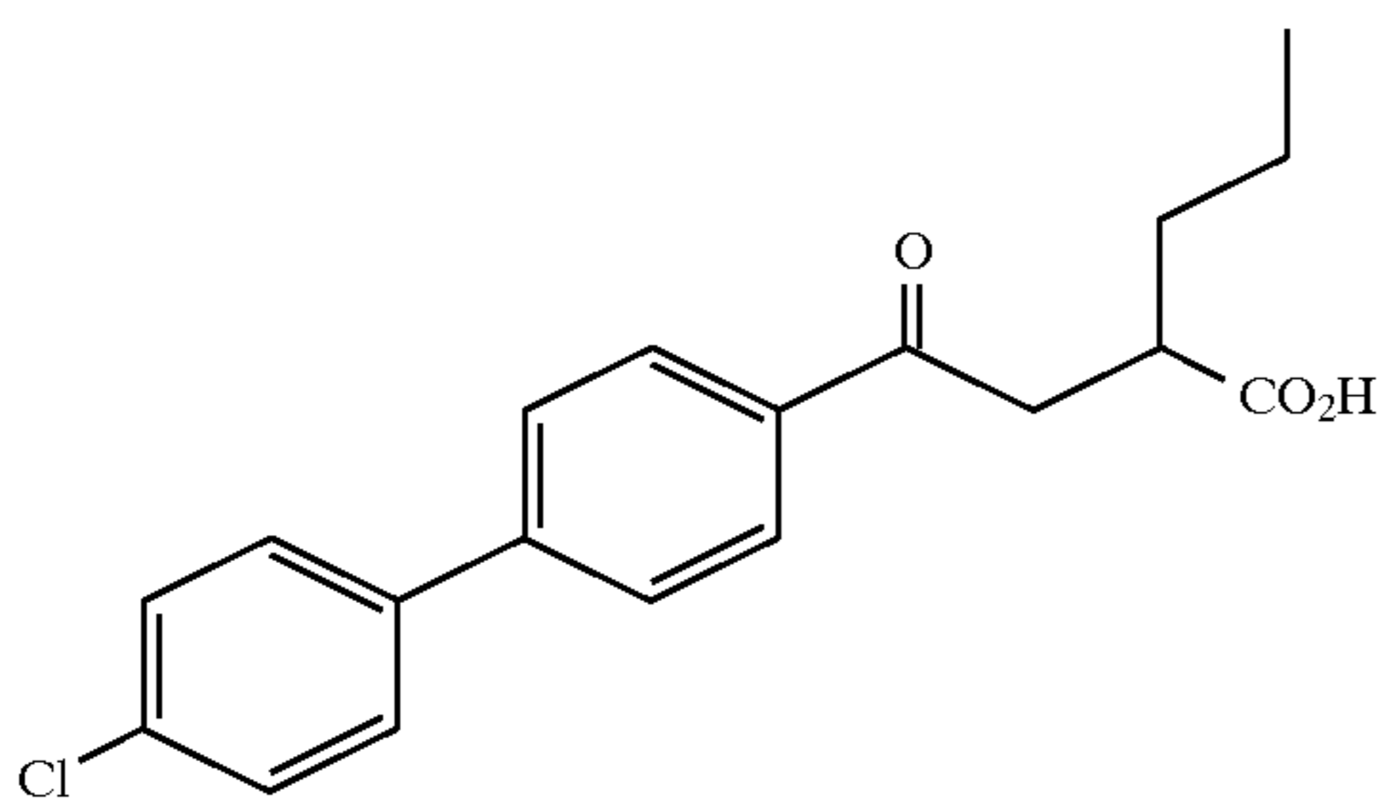
Example 93
