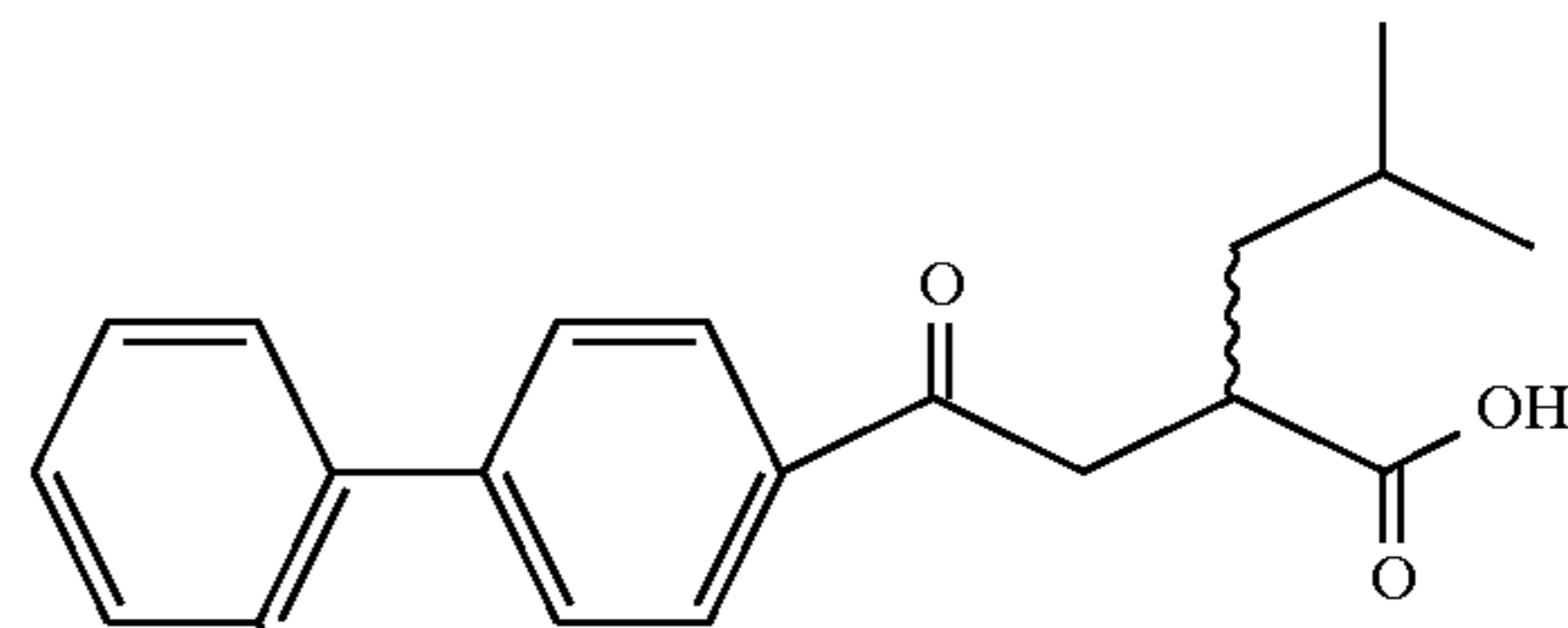
Example 17
