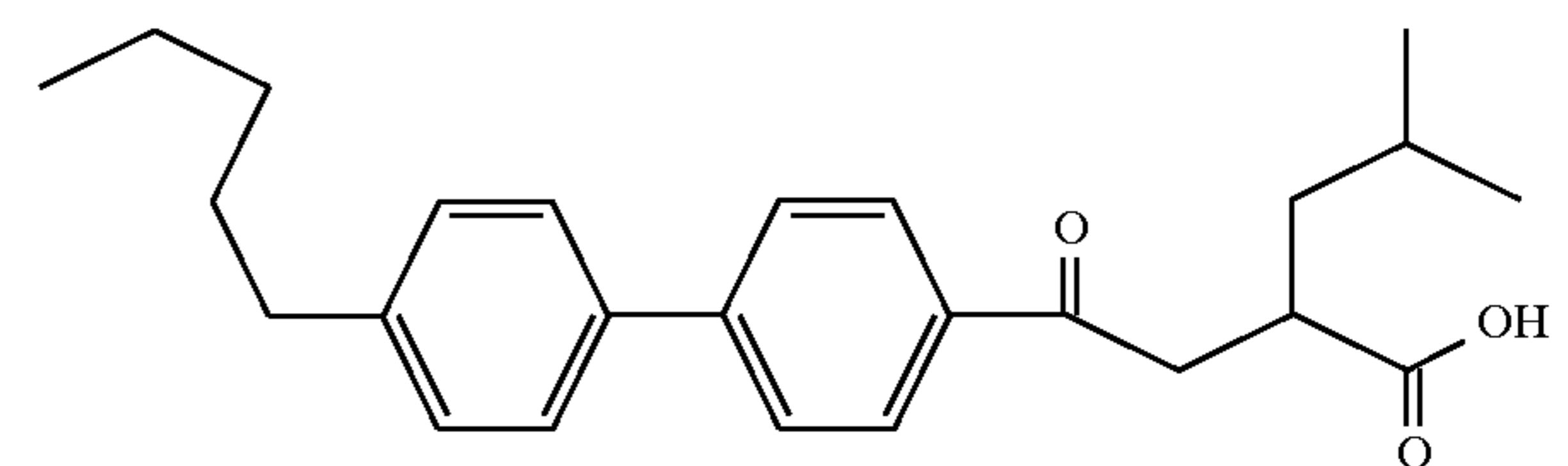
Example 23
