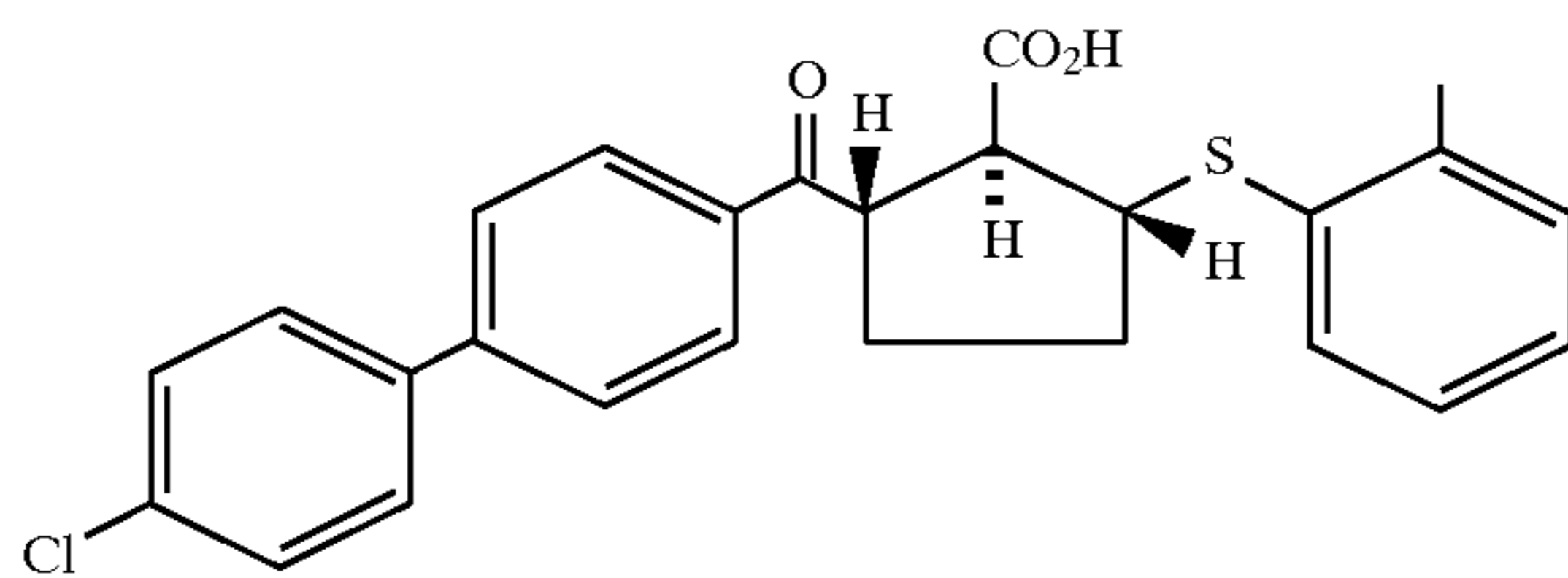
Example 216 (racemate)
