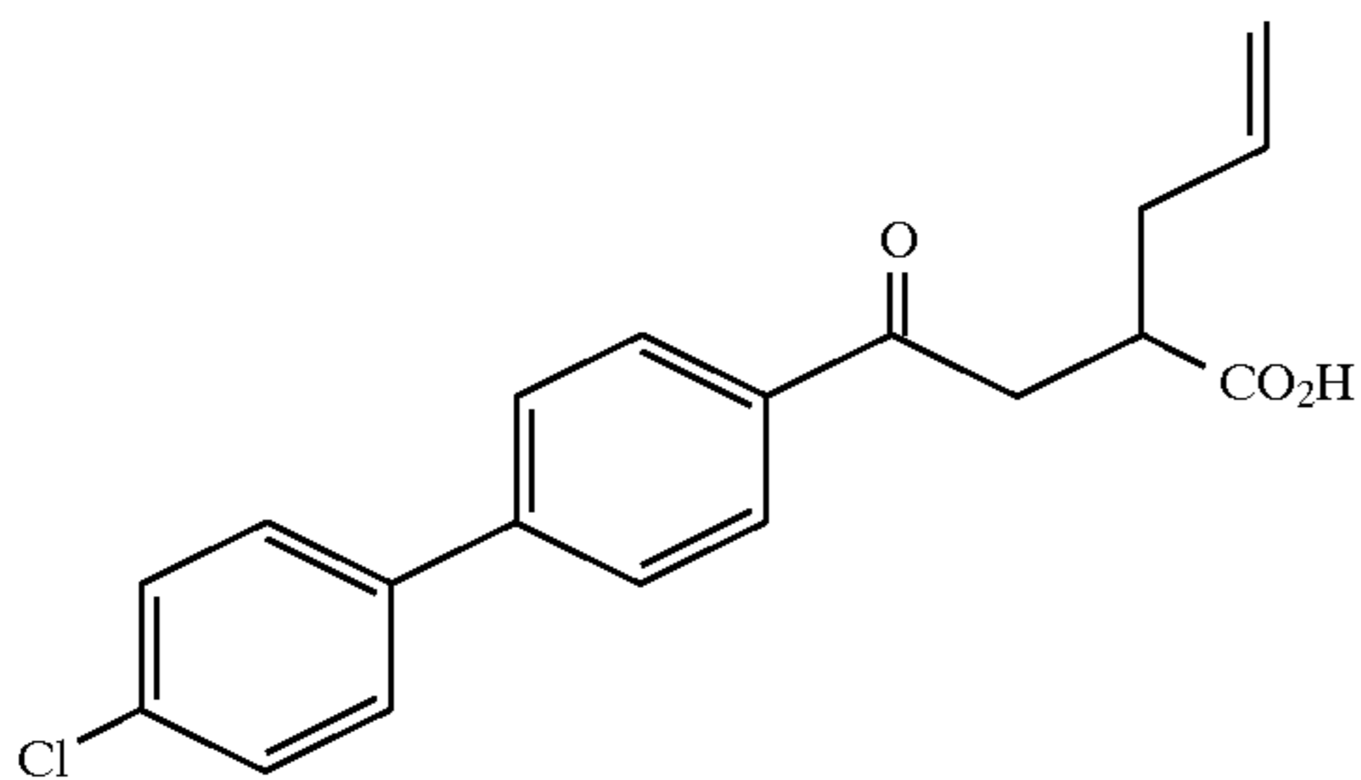
Example 94
