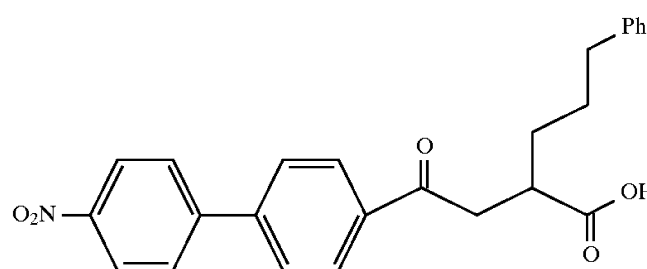
Example 63
