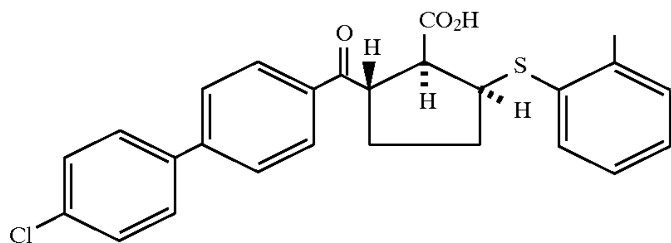
Example 218 (racemate)
