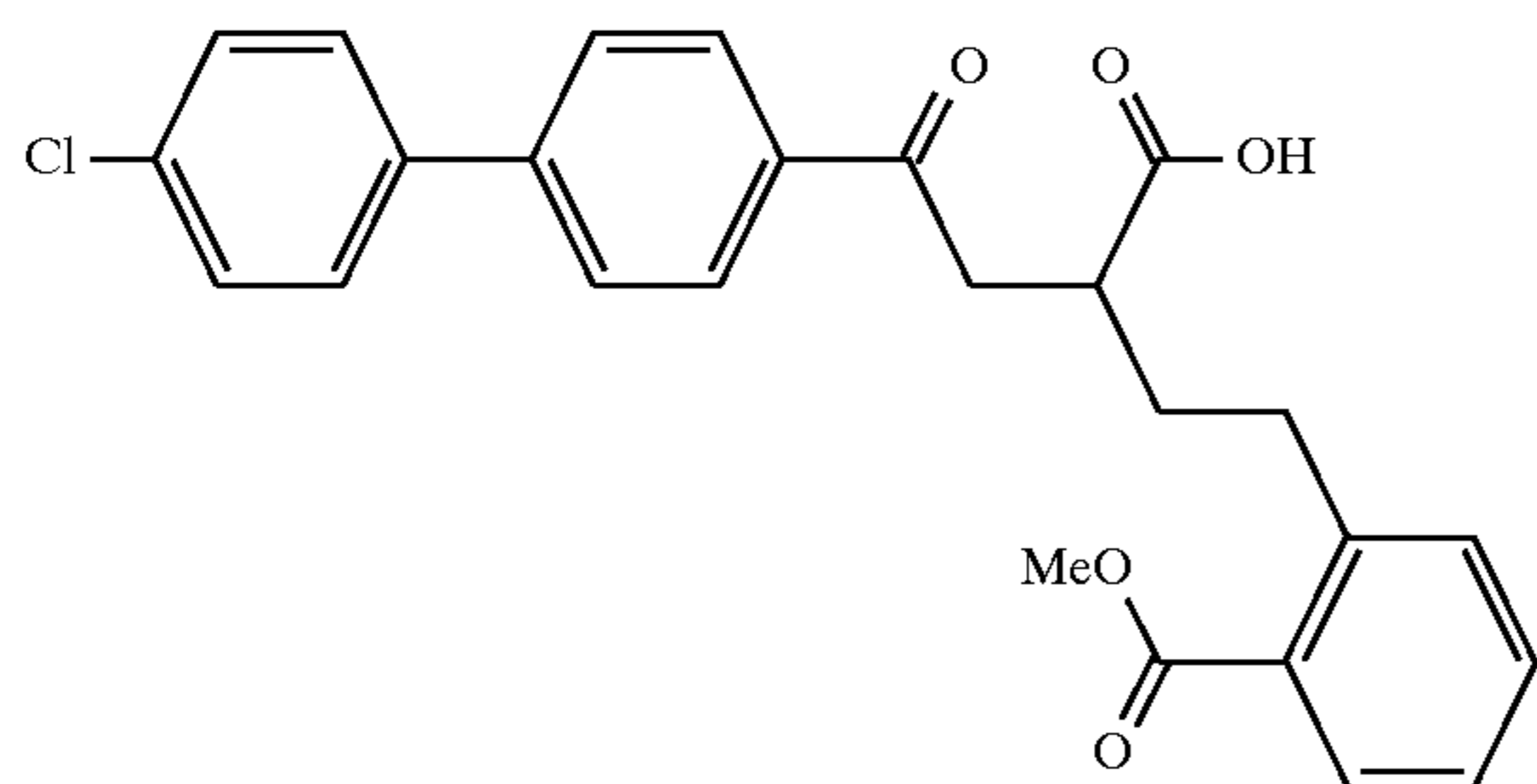
Example 103
