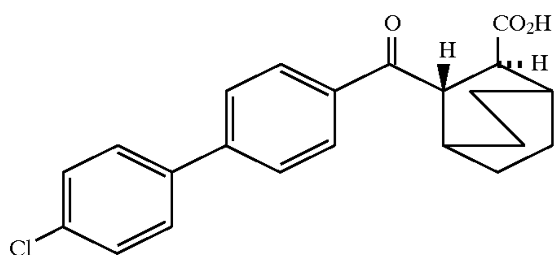
Example 232 (racemate)
