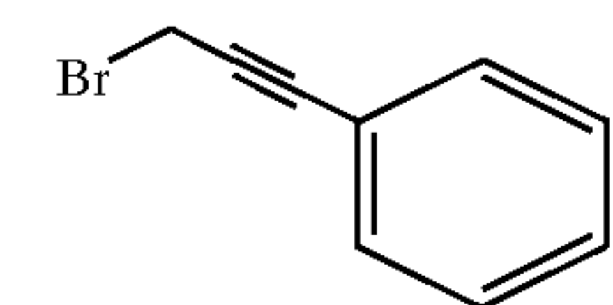
1-phenyl-3-bromo-1-propyn
