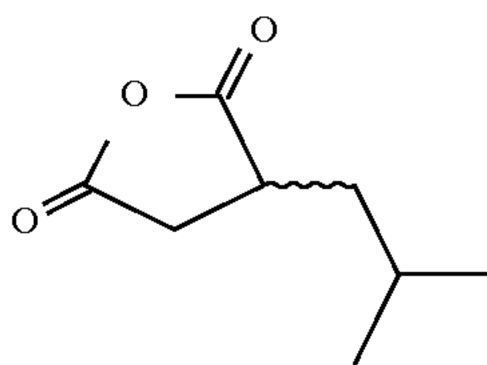
Dihydro-3-(2-methylpropyl)-2,5-furandione
