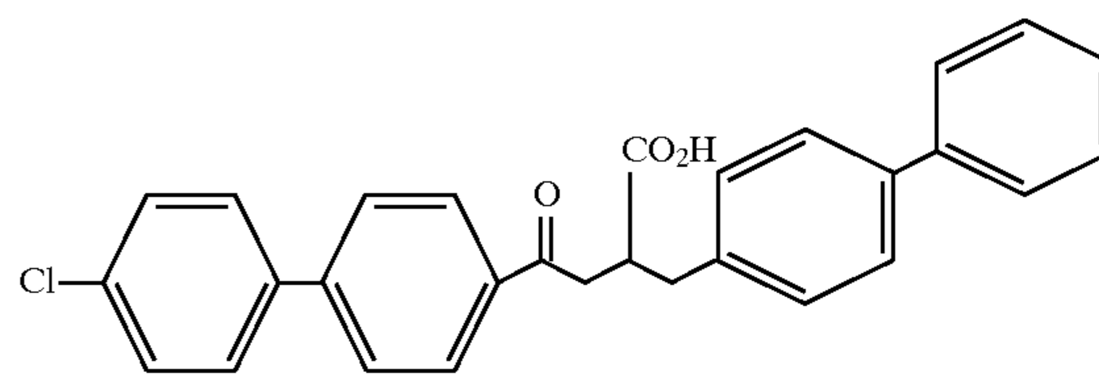
Example 110
