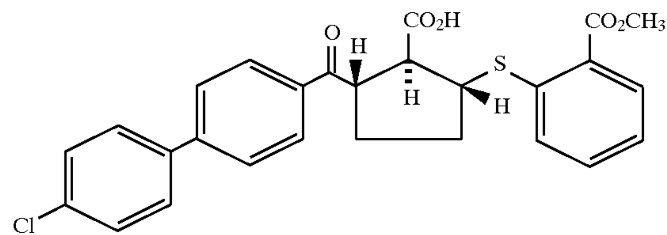
Example 219 (racemate)
