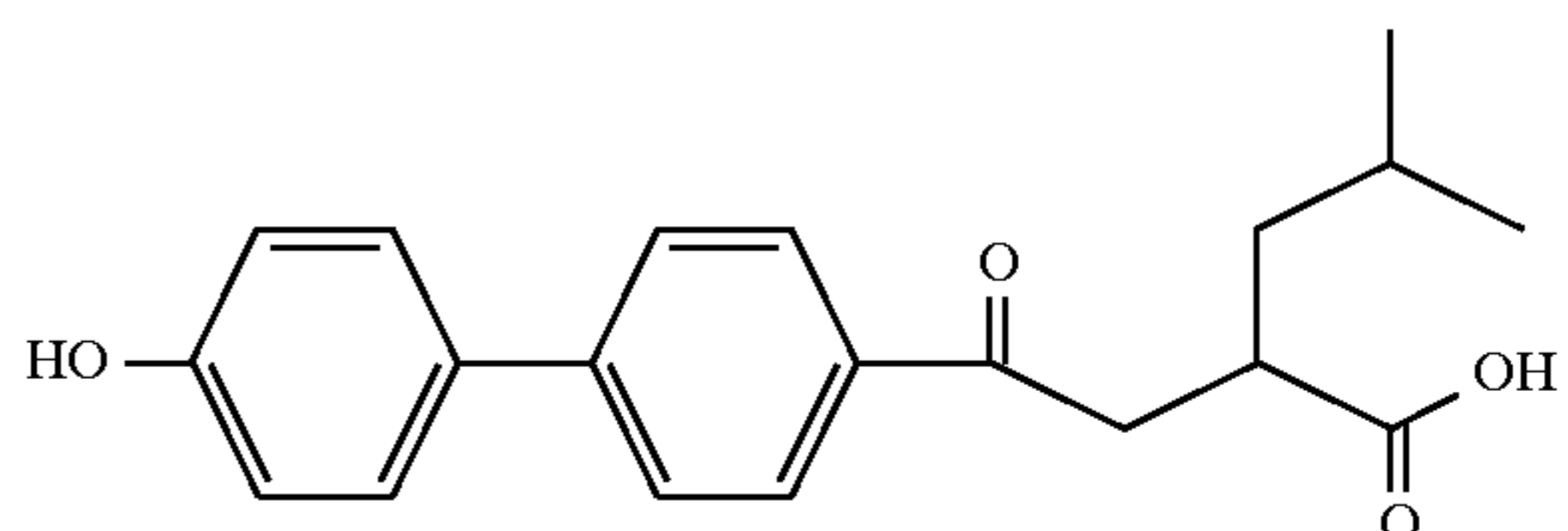
Example 24
