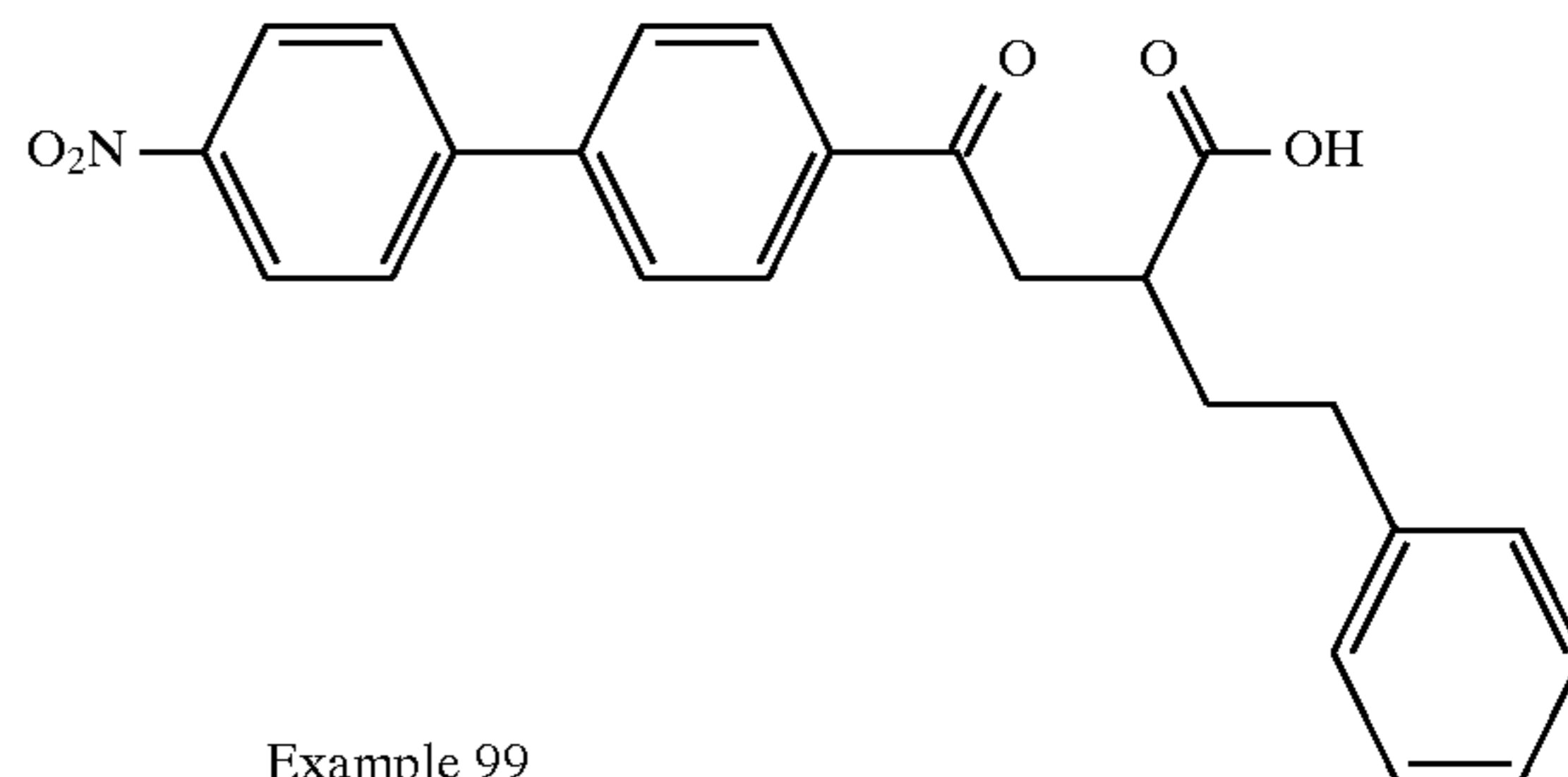
Example 99
