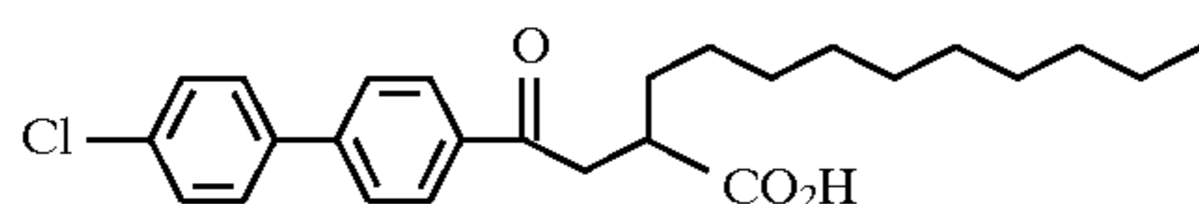
Example 98
