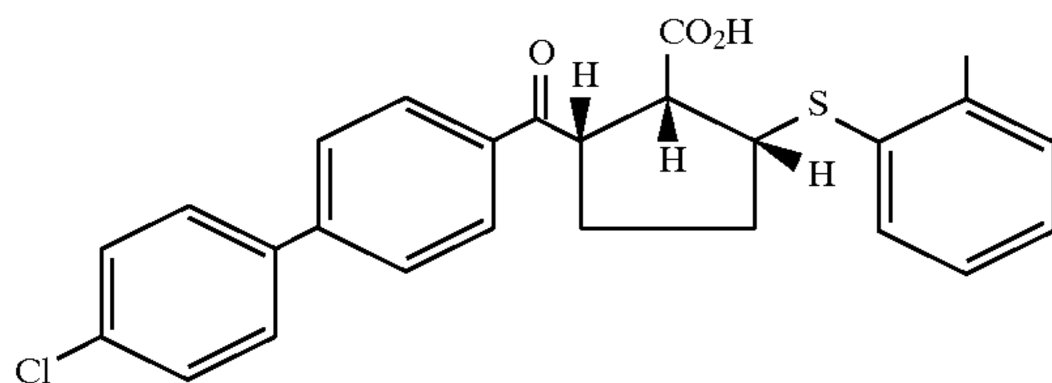
Example 217 (racemate)
