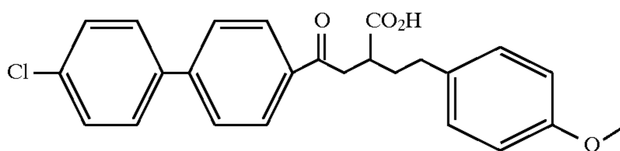
Example 115
