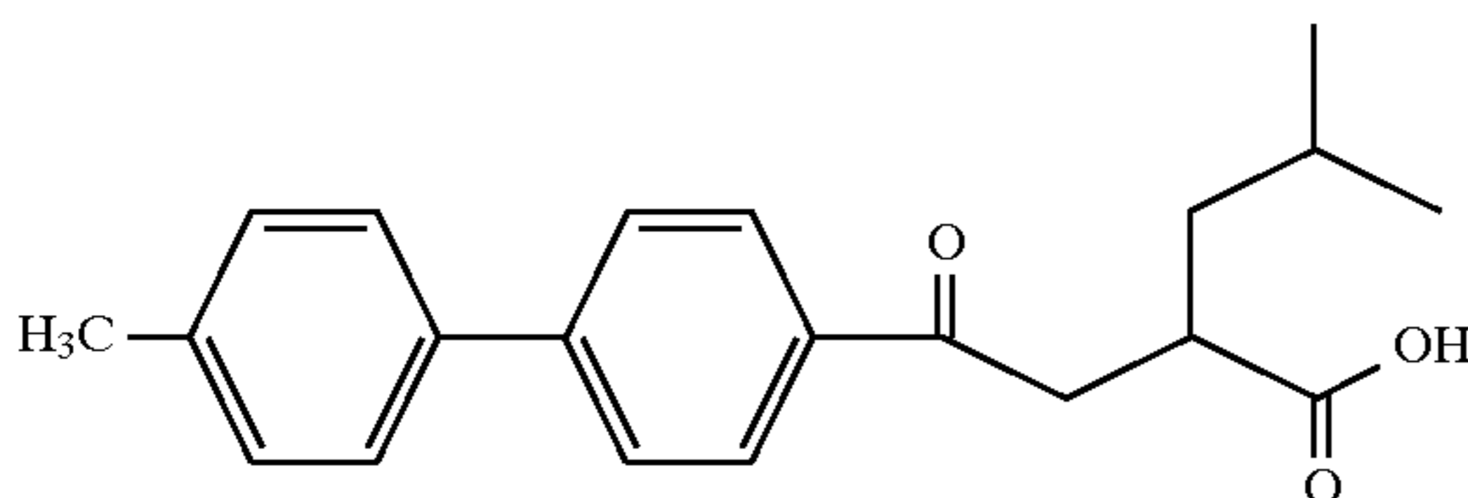
Example 21
