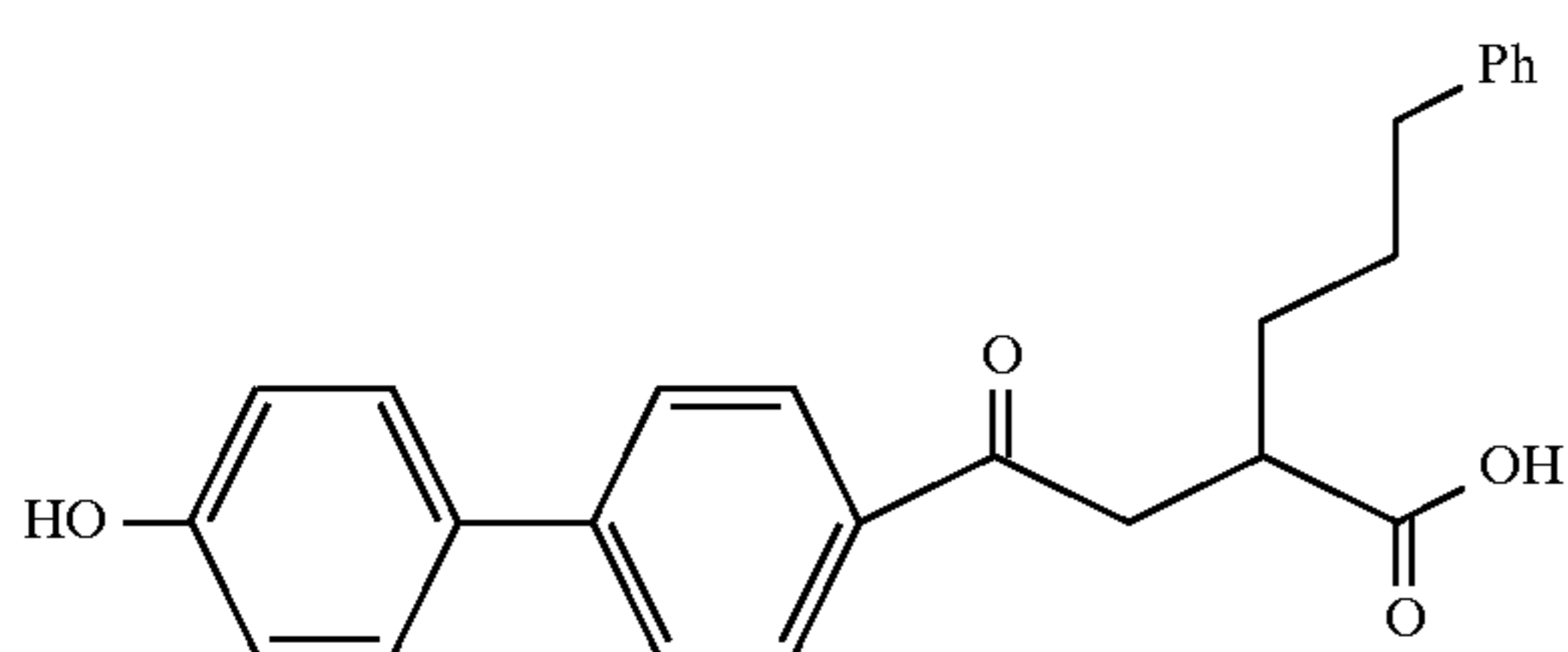
Example 79
