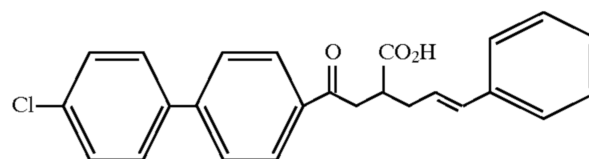
Example 111
