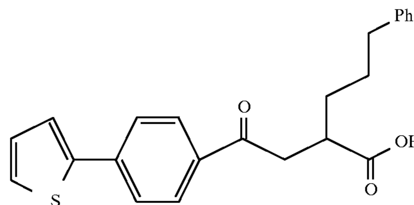
Example 76
