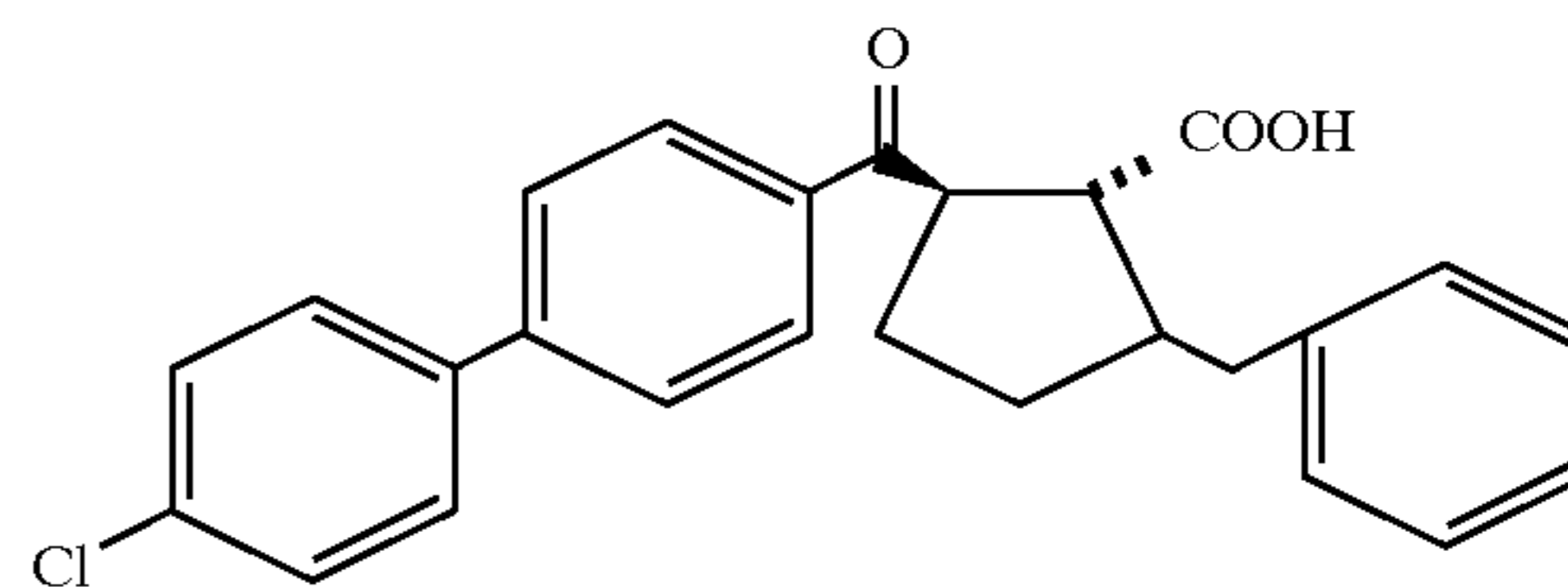
Example 227 (racemate)
