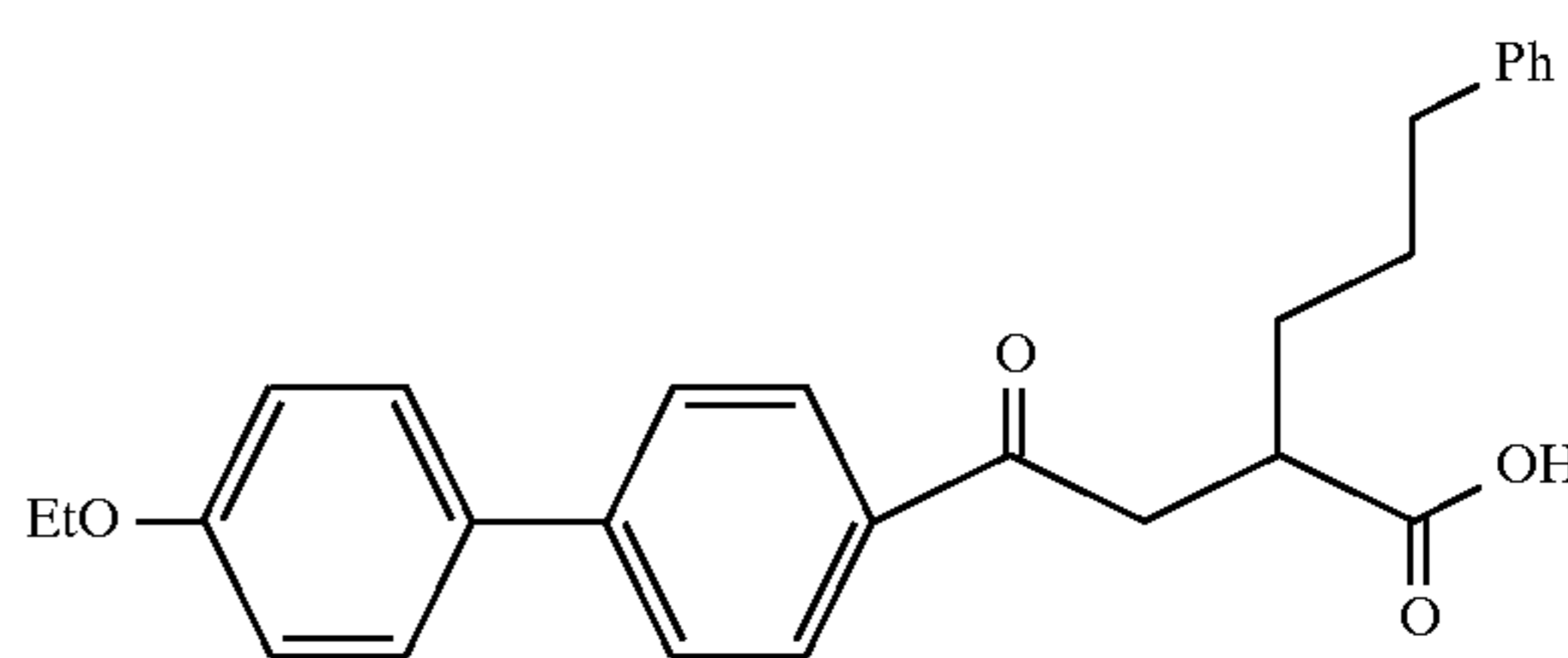
Example 71
