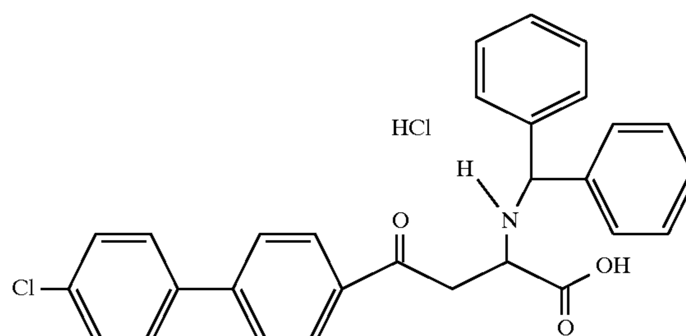
Example 185
