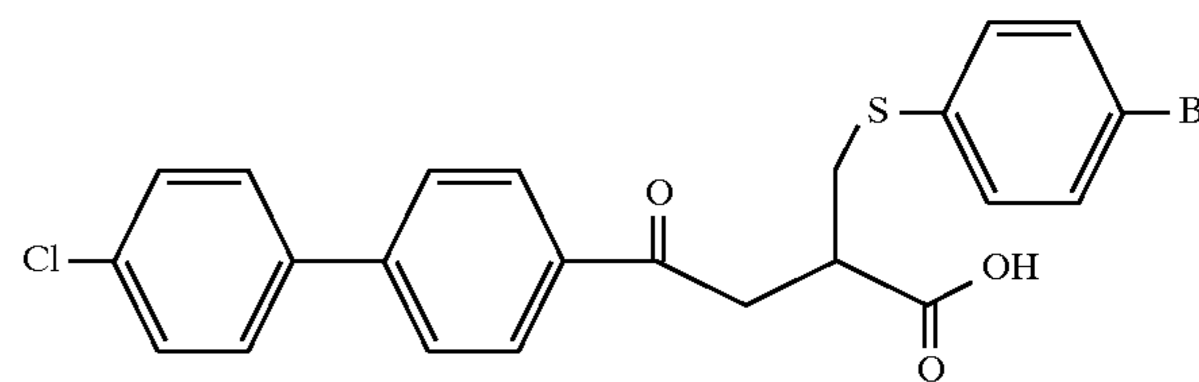
Example 140
