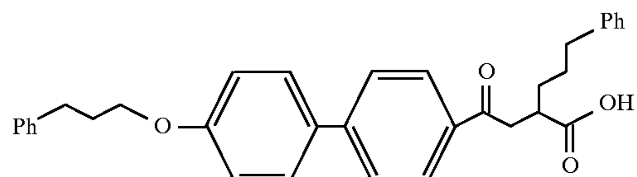
Example 84
