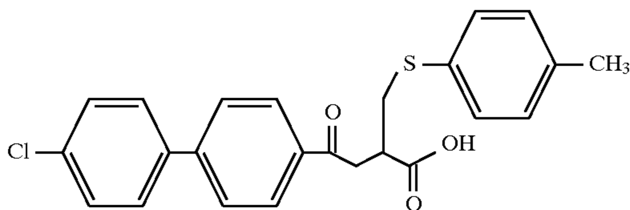
Example 141
