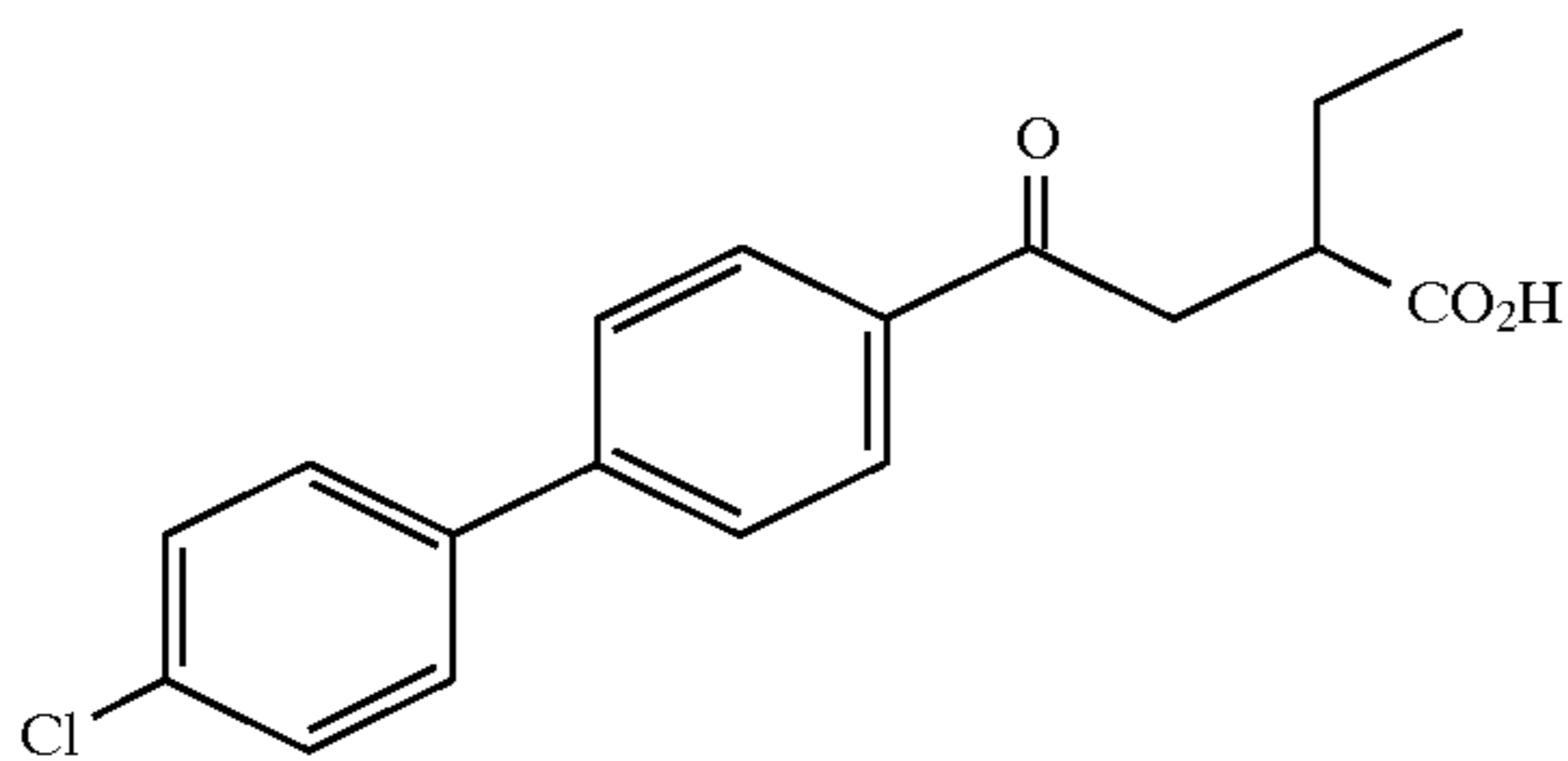
Example 92
