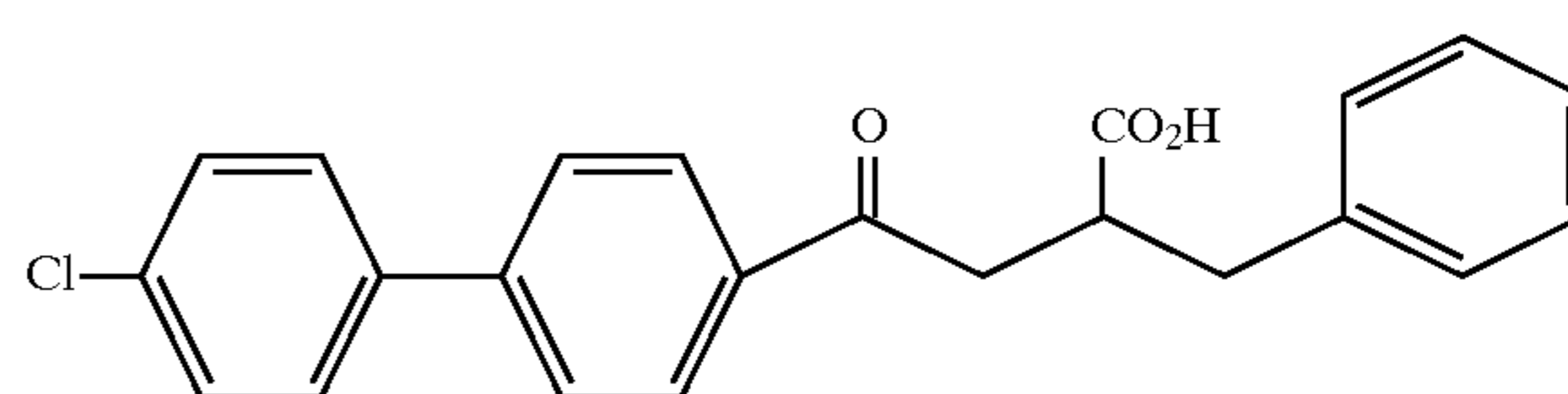
Example 105
