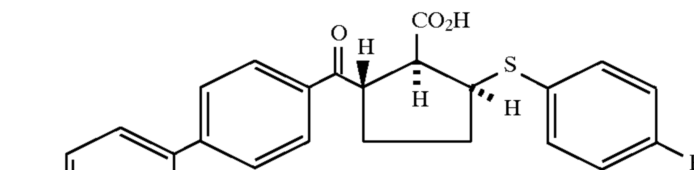
Example 215 (racemate)
