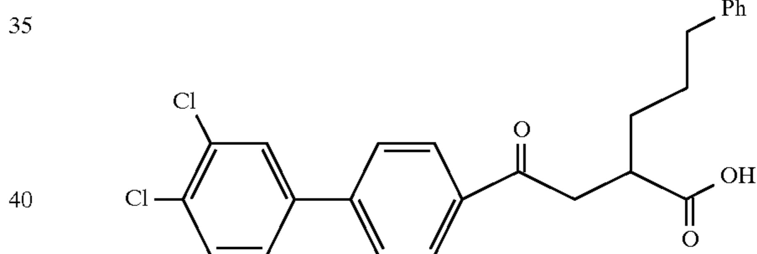
Example 65
