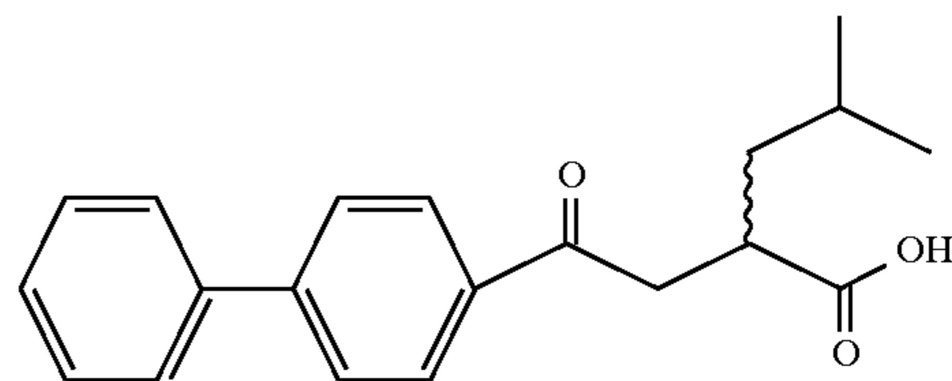
Example 18
