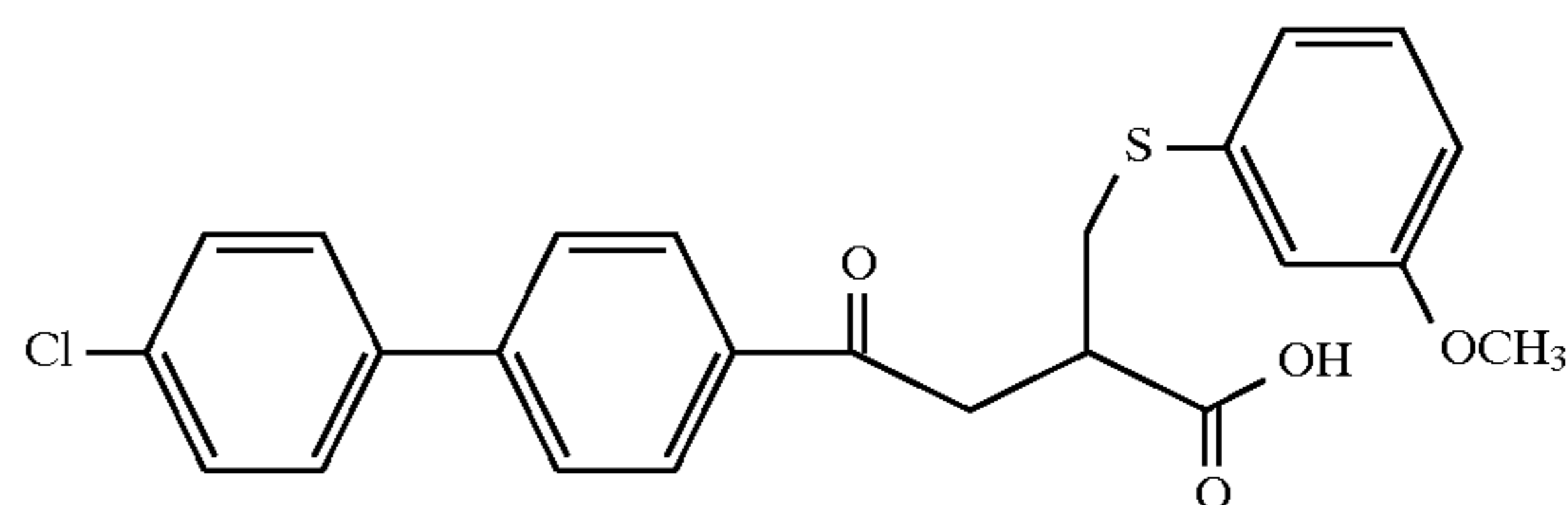
Example 164
