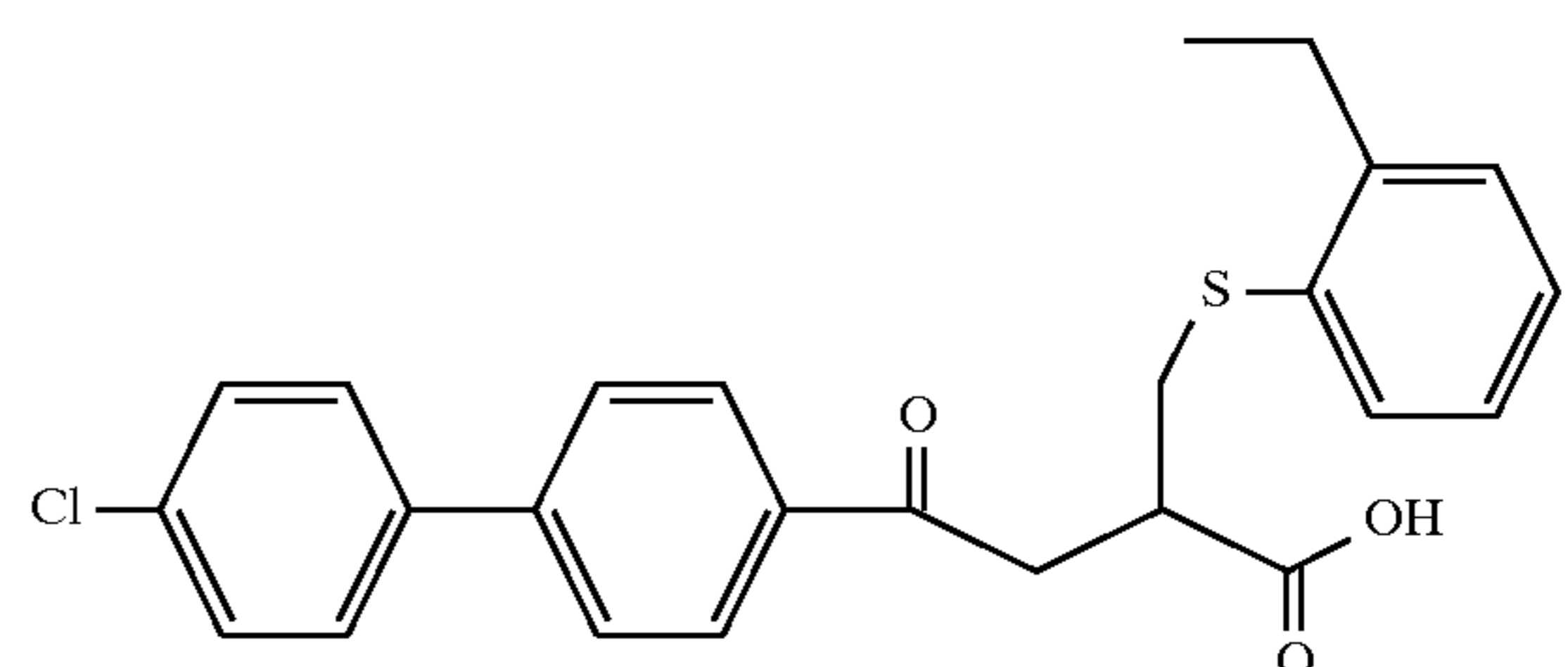
Example 150
