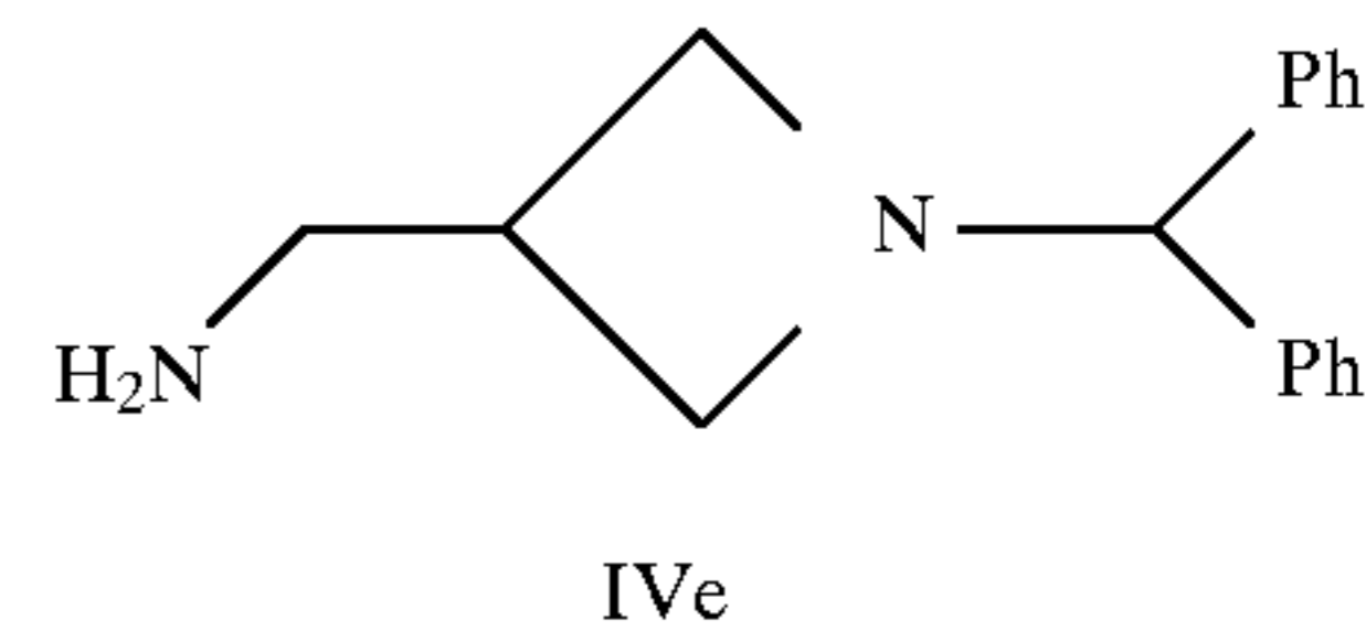
Scheme (3). Route to 3-(aminomethyl)-azetidide starting material (IVe)
