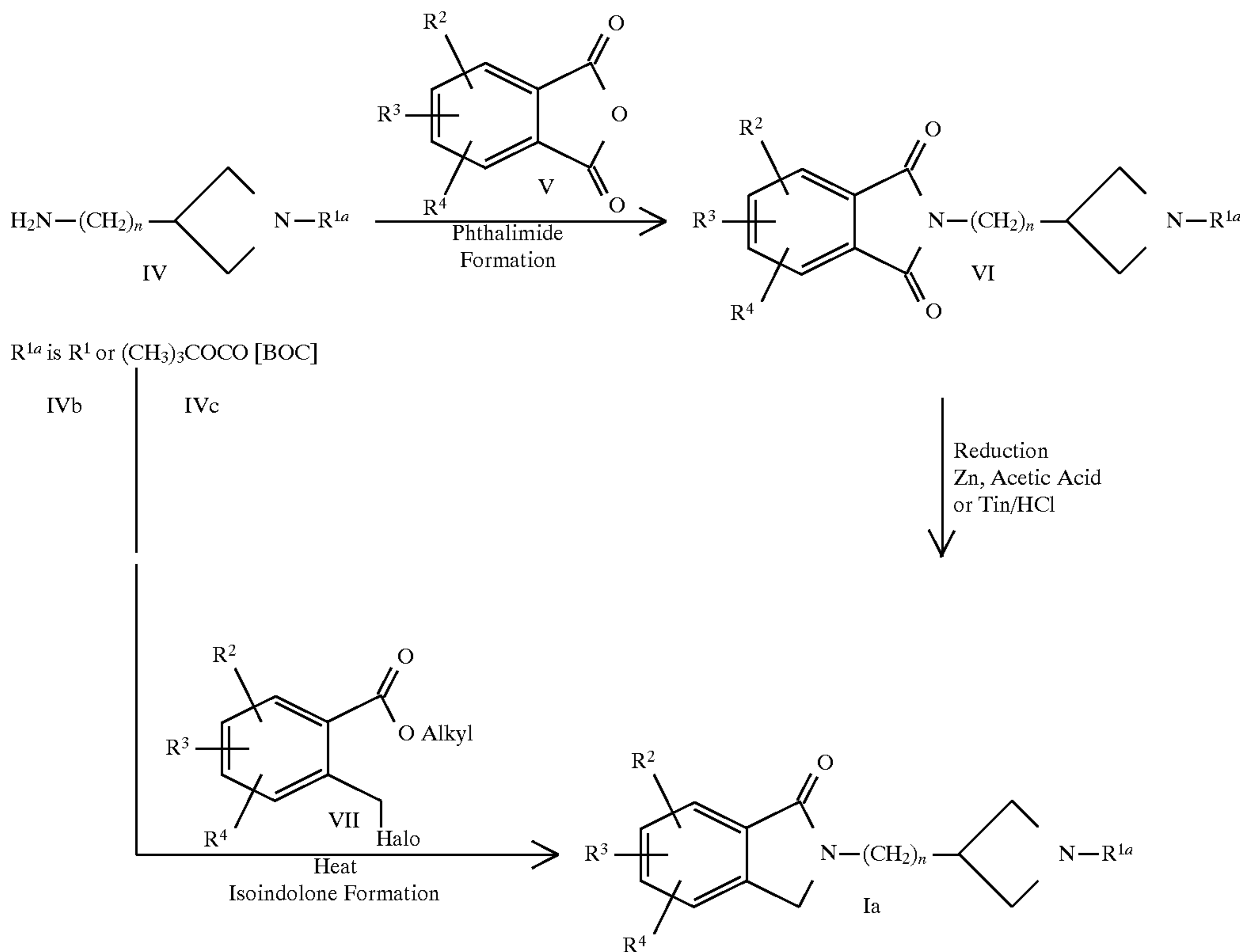
Scheme I. Routes to Isoindolinone Azetidines
