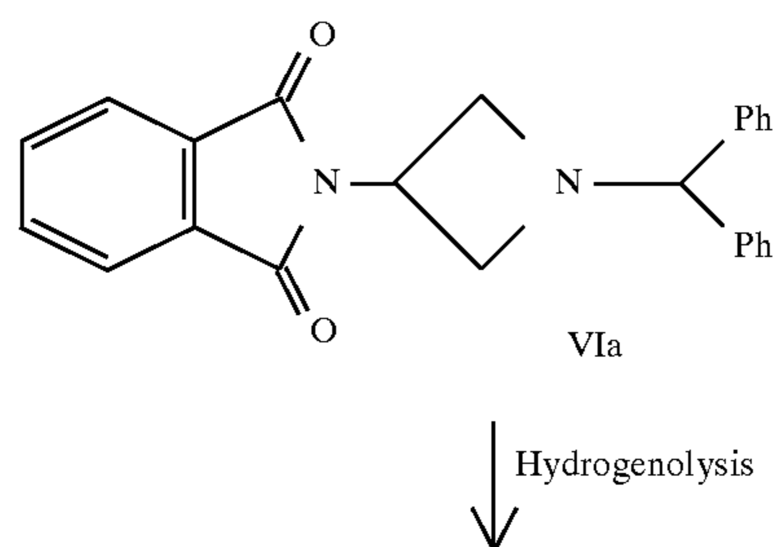
Scheme (2). Routes to IVb and IVc
