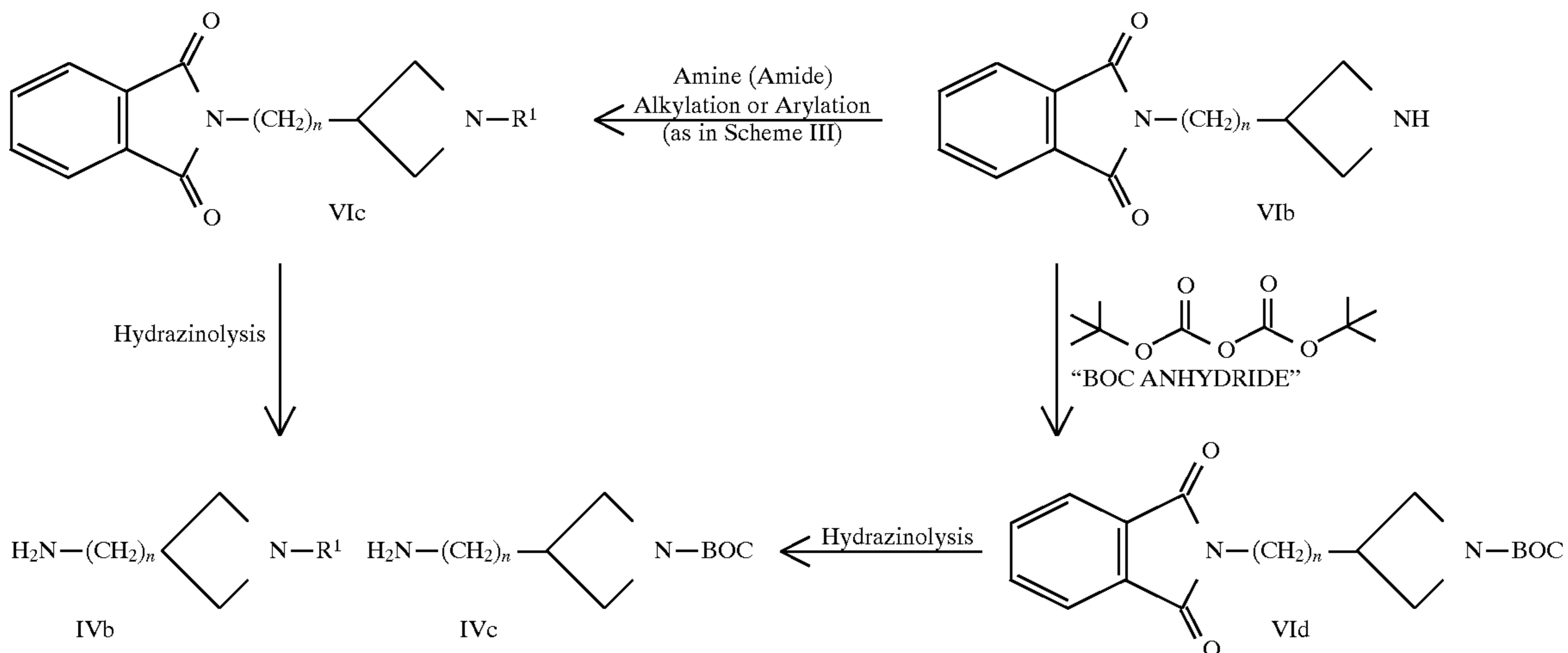
-continued Scheme (2). Routes to IVb and IVc
