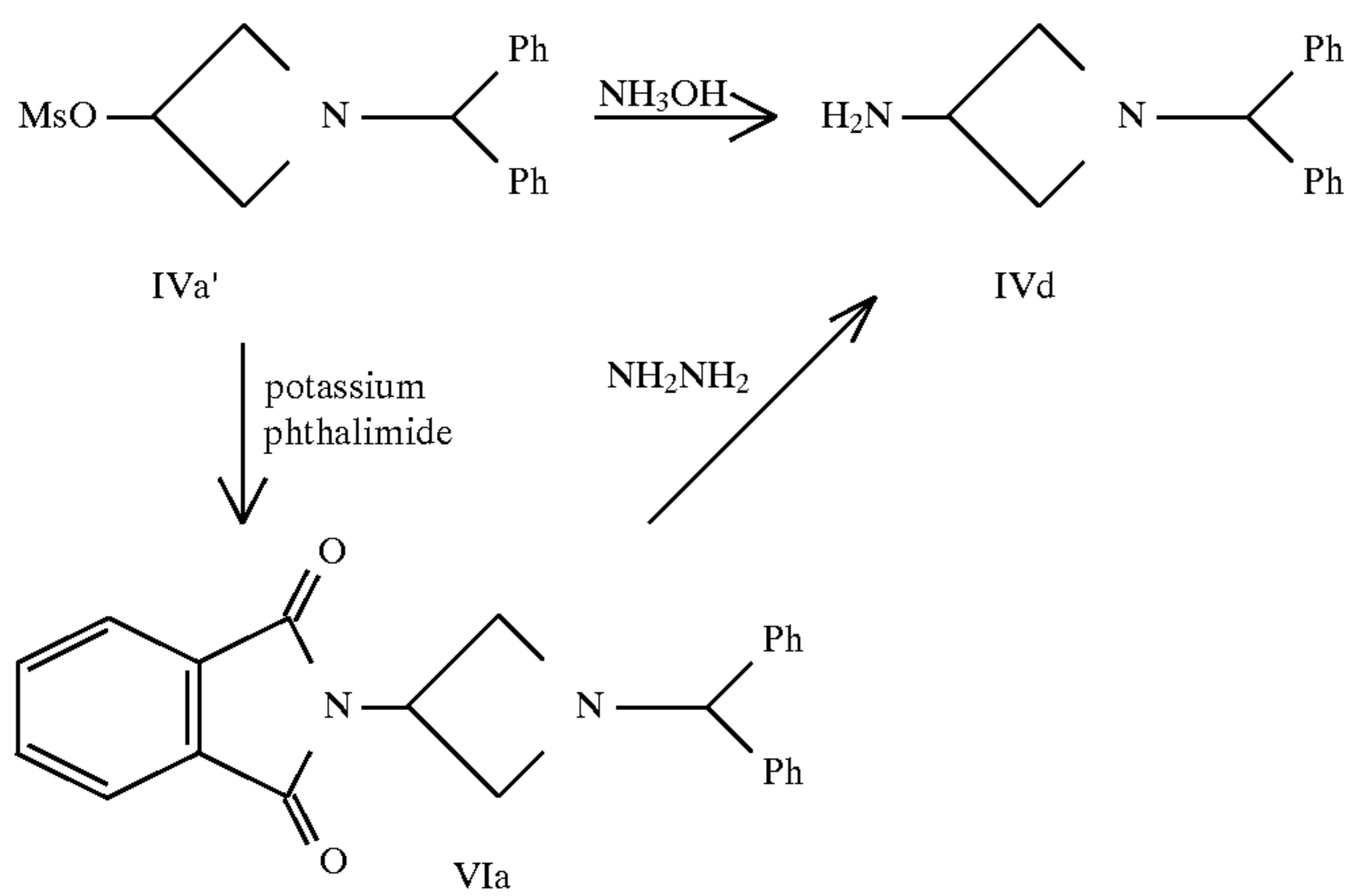
Scheme (1). Route to 3-amino-azetidine starting material (IVd)
