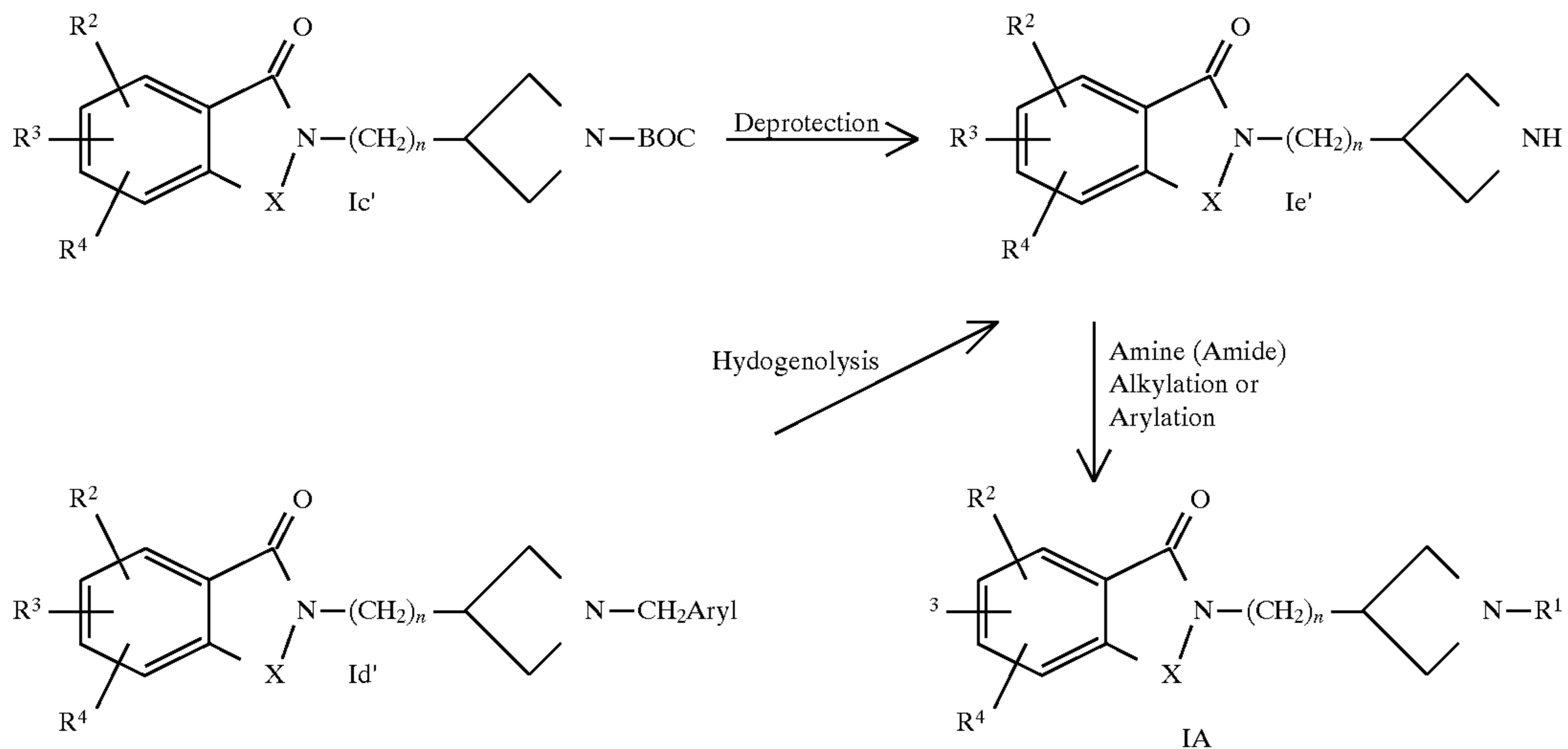
Scheme III. Introduction of R 1 by Alkylation or Arylation
