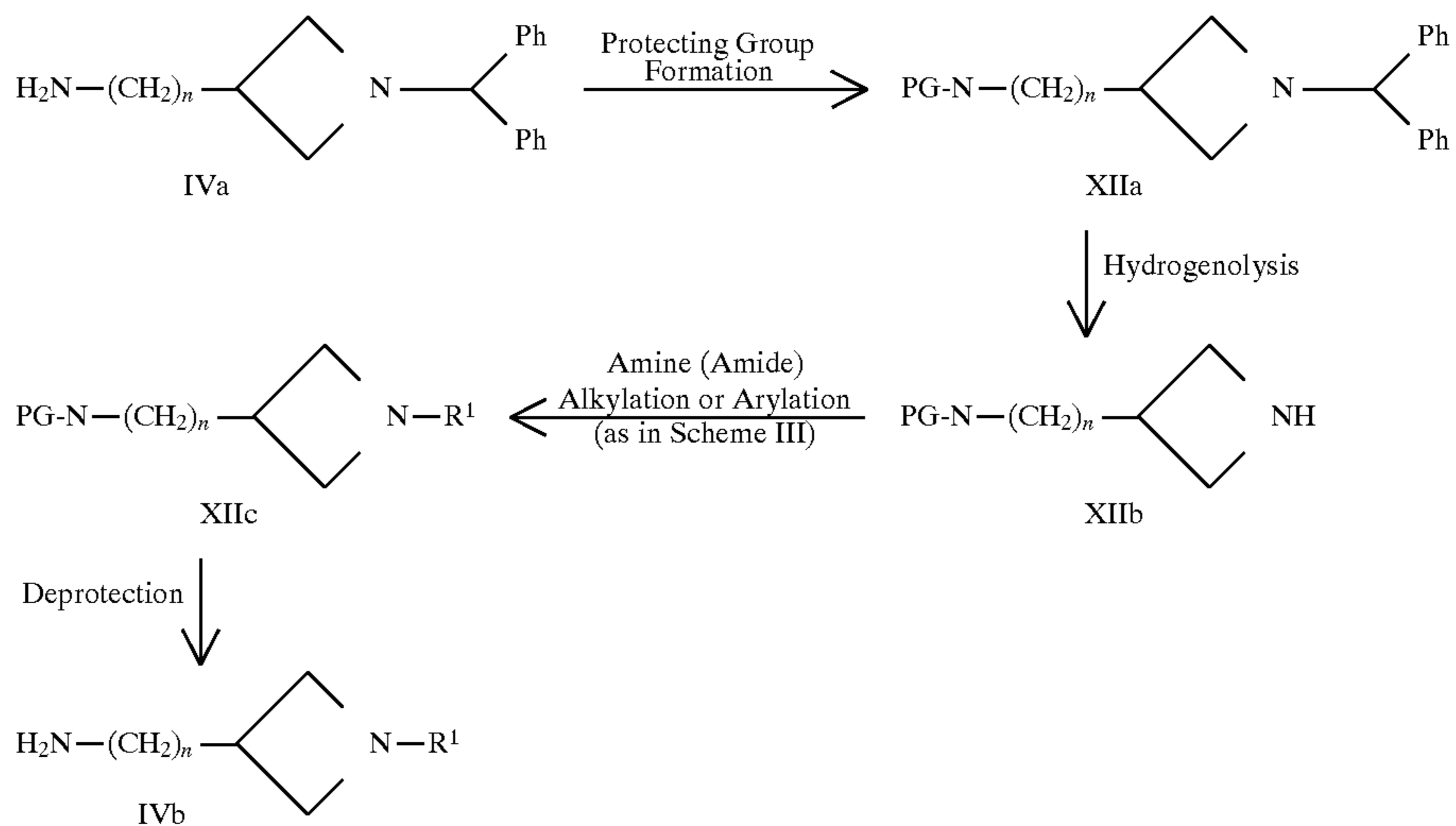
Scheme V. General Routes to Starting Materials IVb
