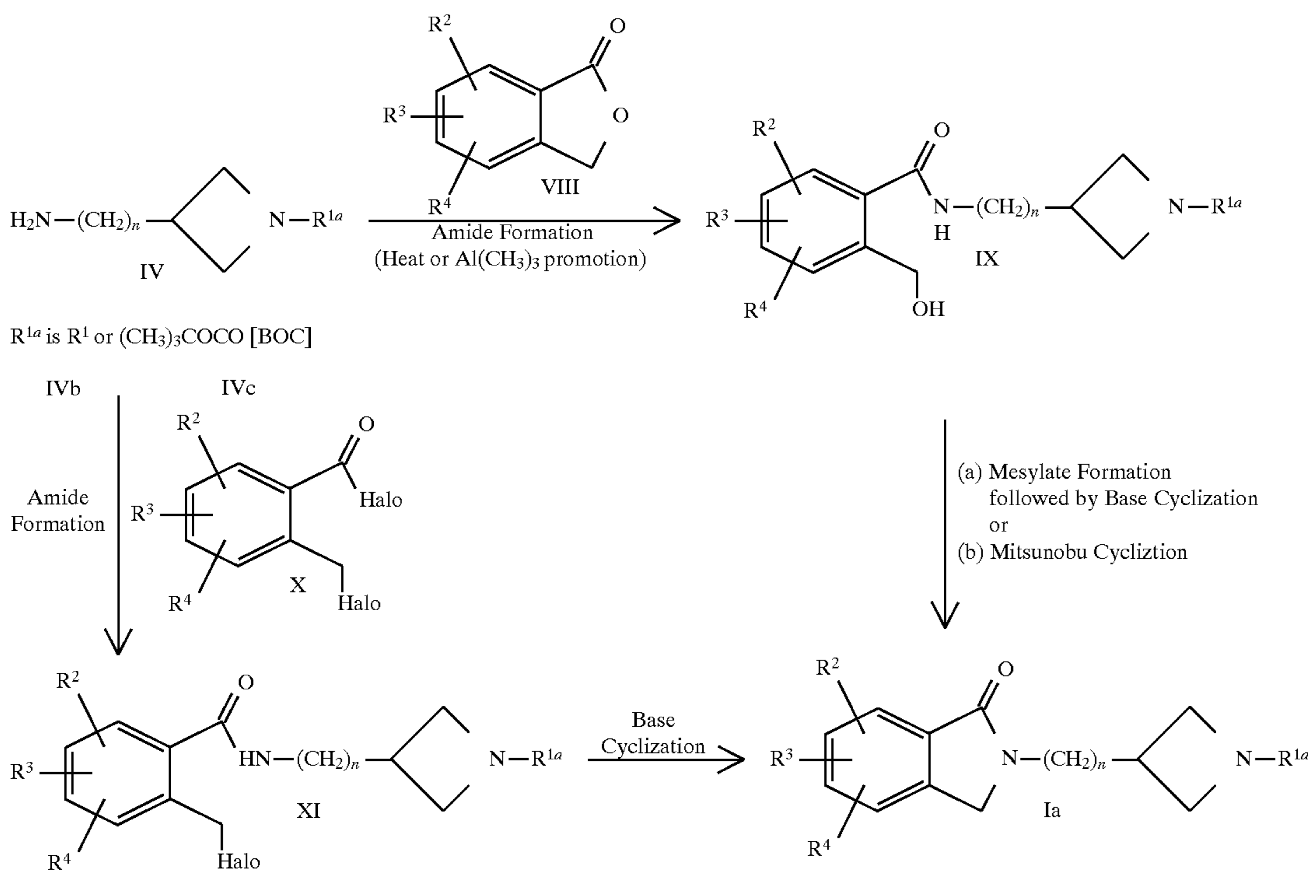
Scheme II. Additional Routes to Isoindolinone Azetidines
