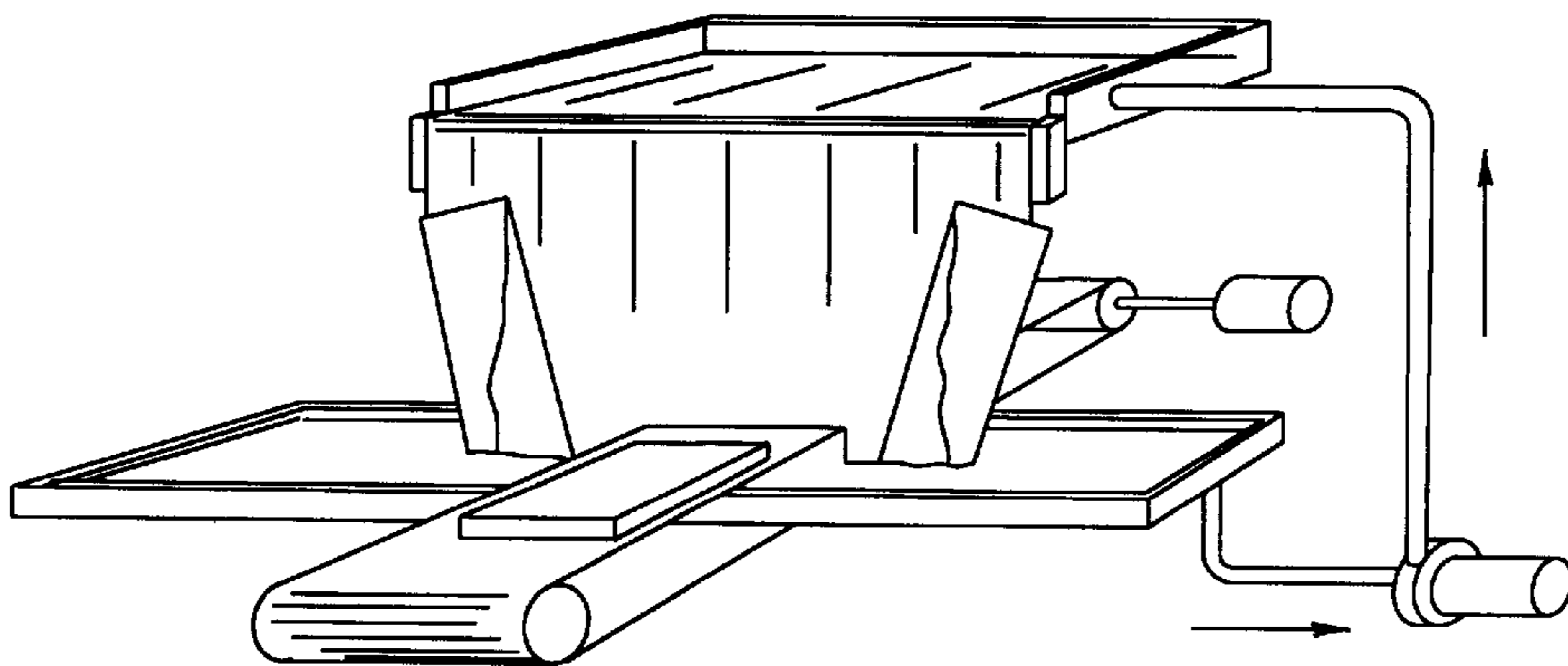
FIG. 1C (PRIOR ART)
