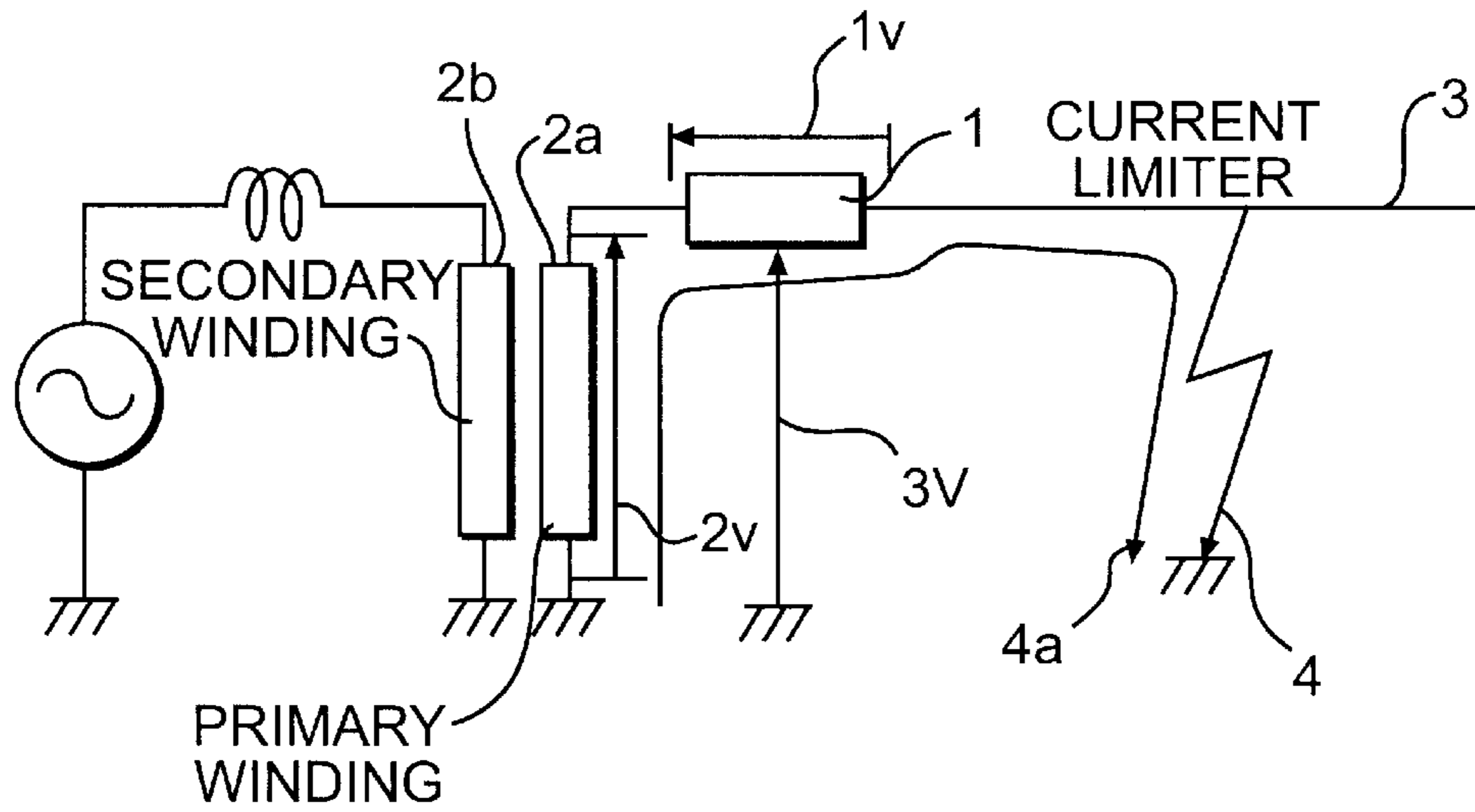
FIG. 3 PRIOR ART
