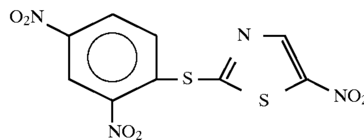
COMPOUND 12
