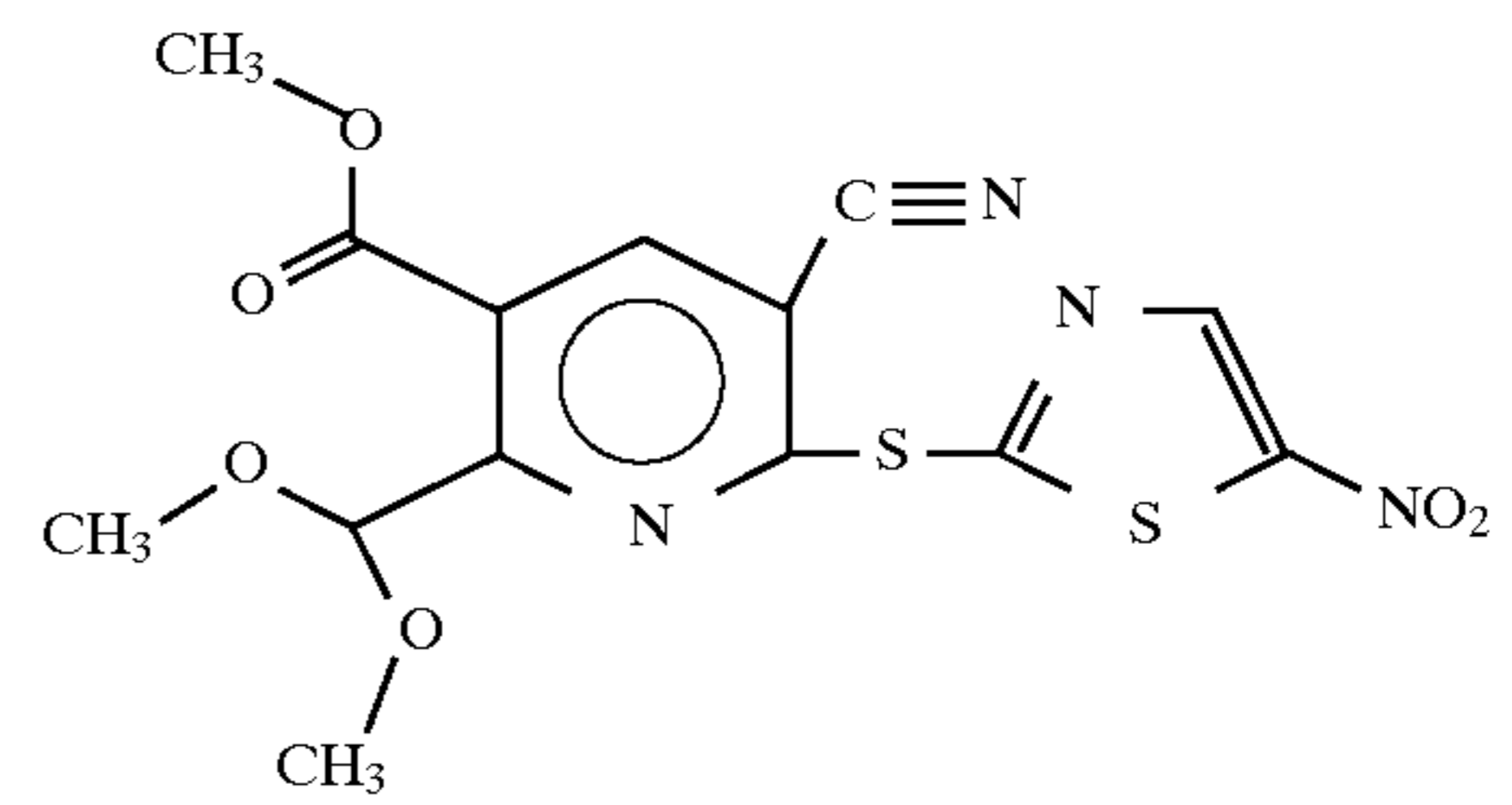
COMPOUND 10
