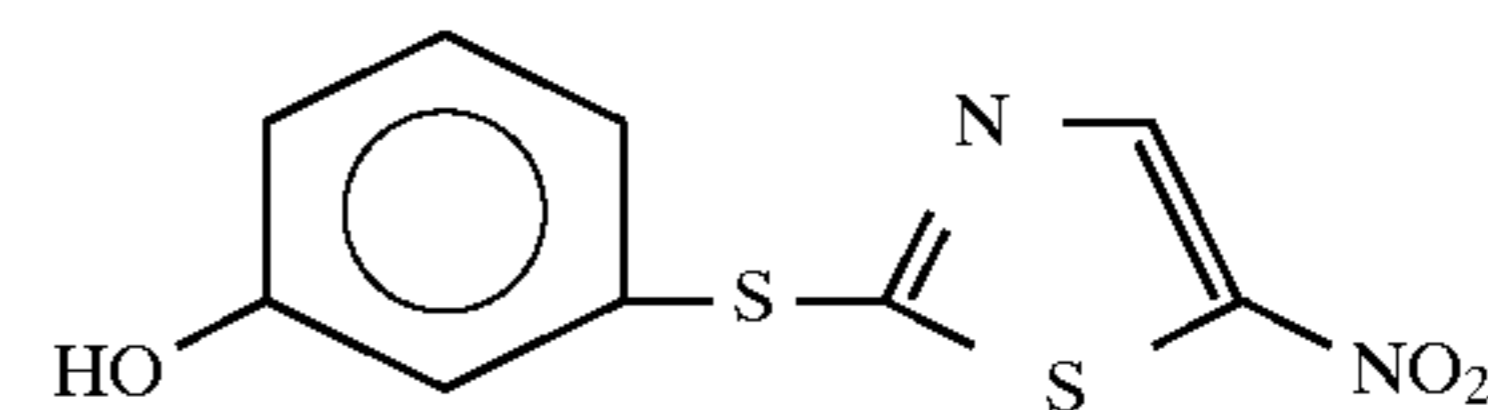
COMPOUND 11
