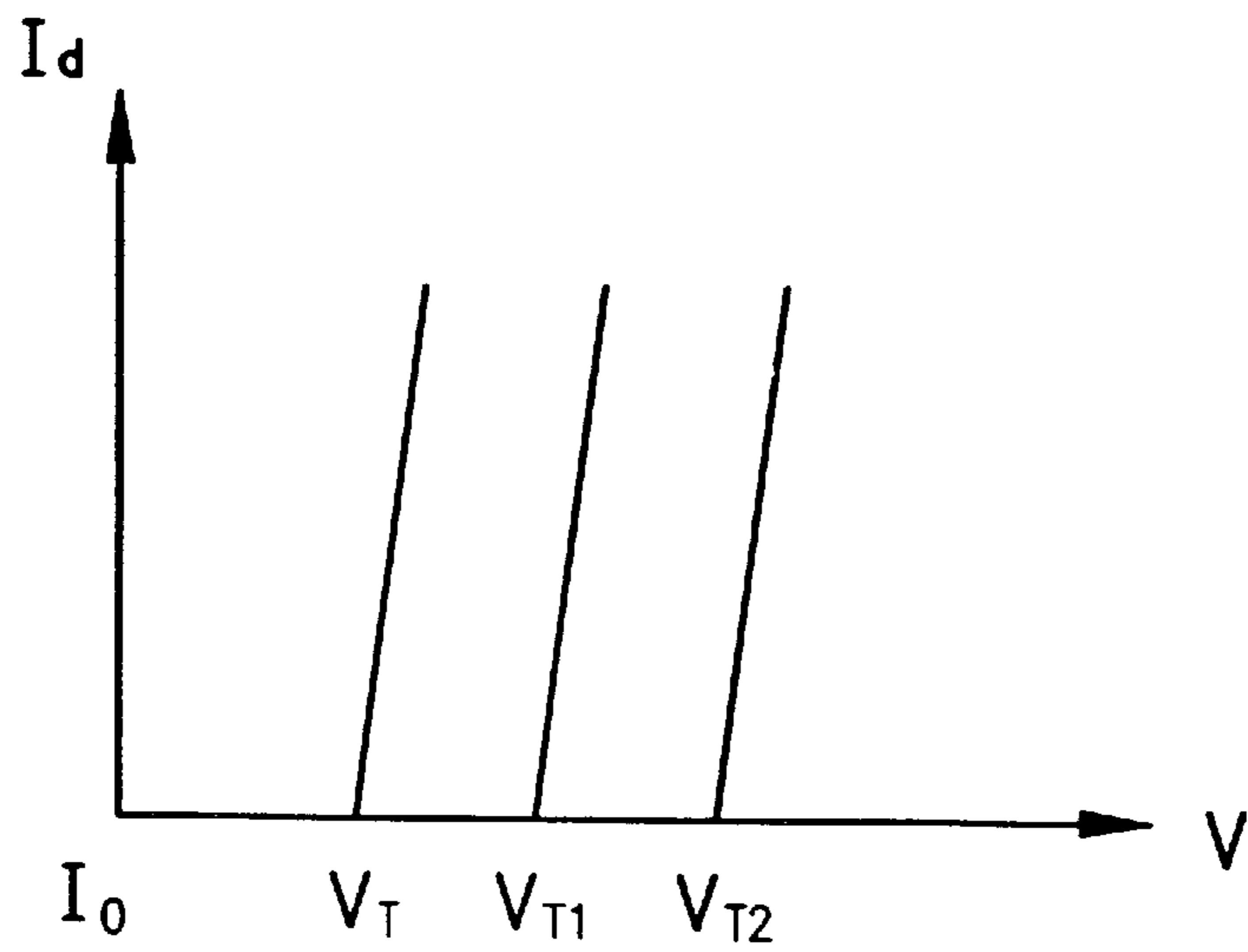
FIG. 2 (PRIOR ART)
