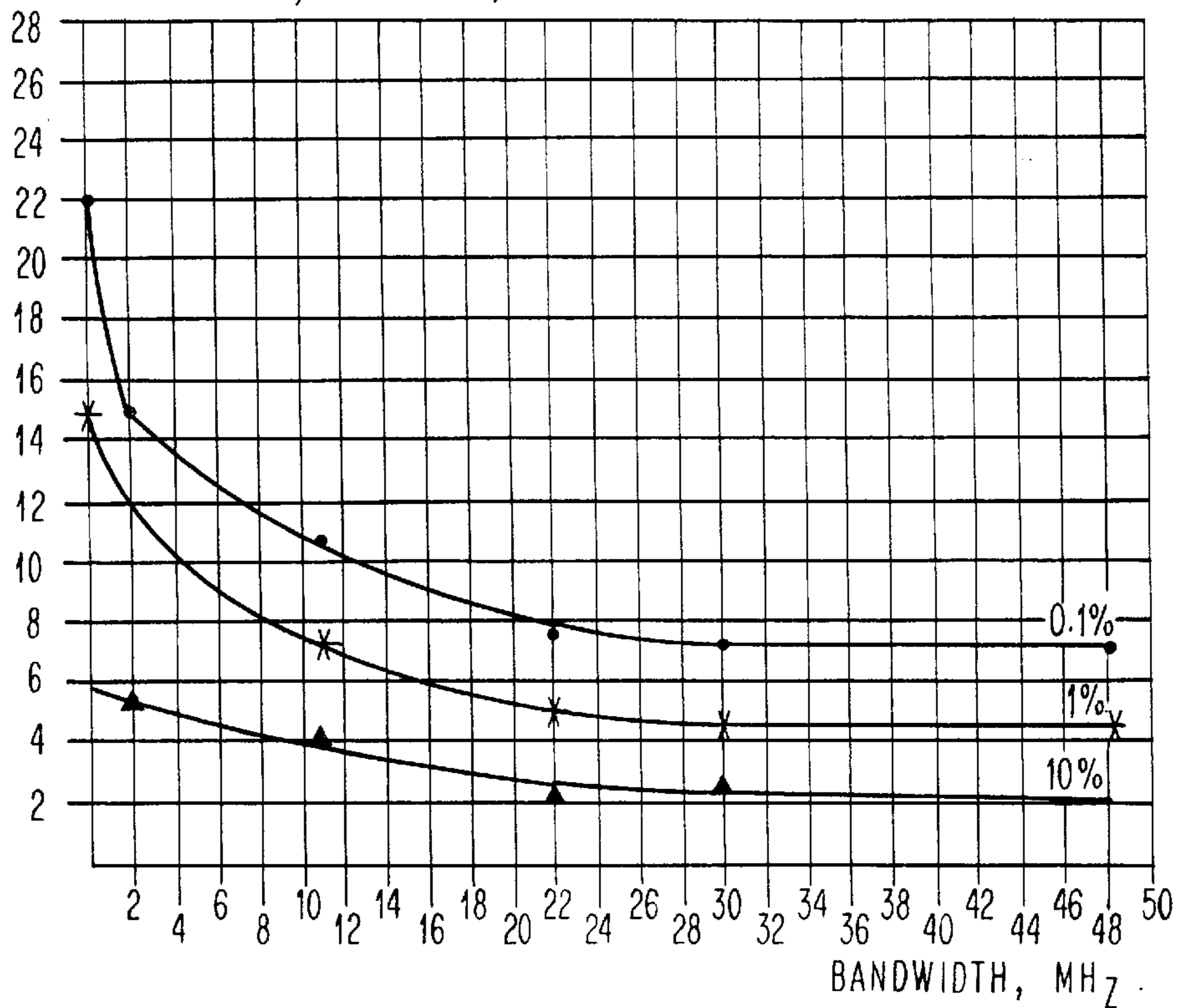
FADE DEPTH, dB Fig. 16
