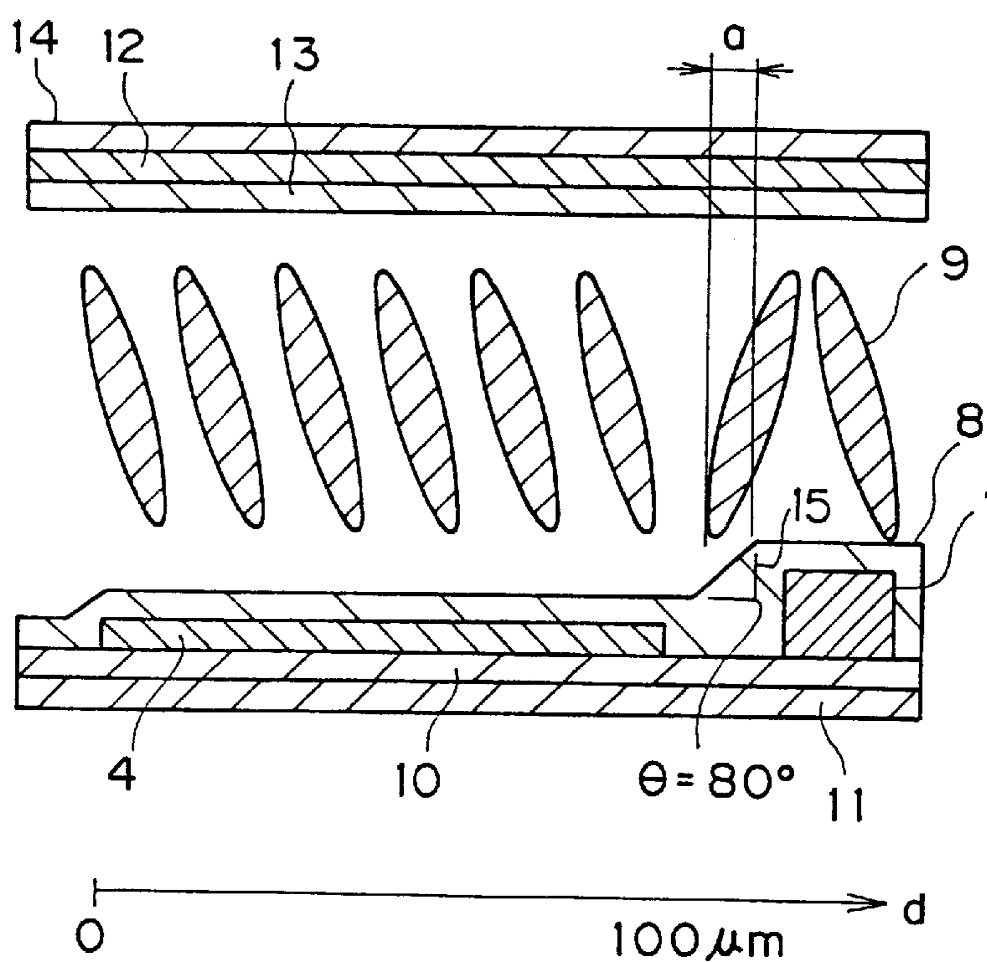
Fig.11 PRIOR ART
