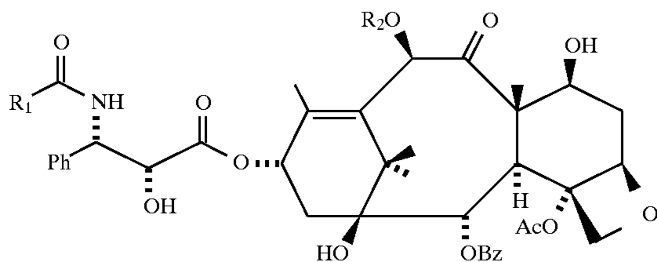
Taxol: R 1 = C 6 H 5 ; R 2 = CH 3 CO Taxotere: R 1 = (CH 3 ) 3 CO; R 2 = H
