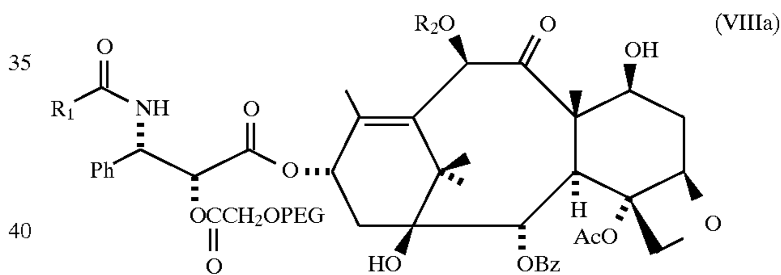
ProTaxol: R 1 = C 6 H 5 ; R 2 = CH 3 CO ProTaxotere: R 1 = (CH 3 ) 3 CO; R 2 = H
