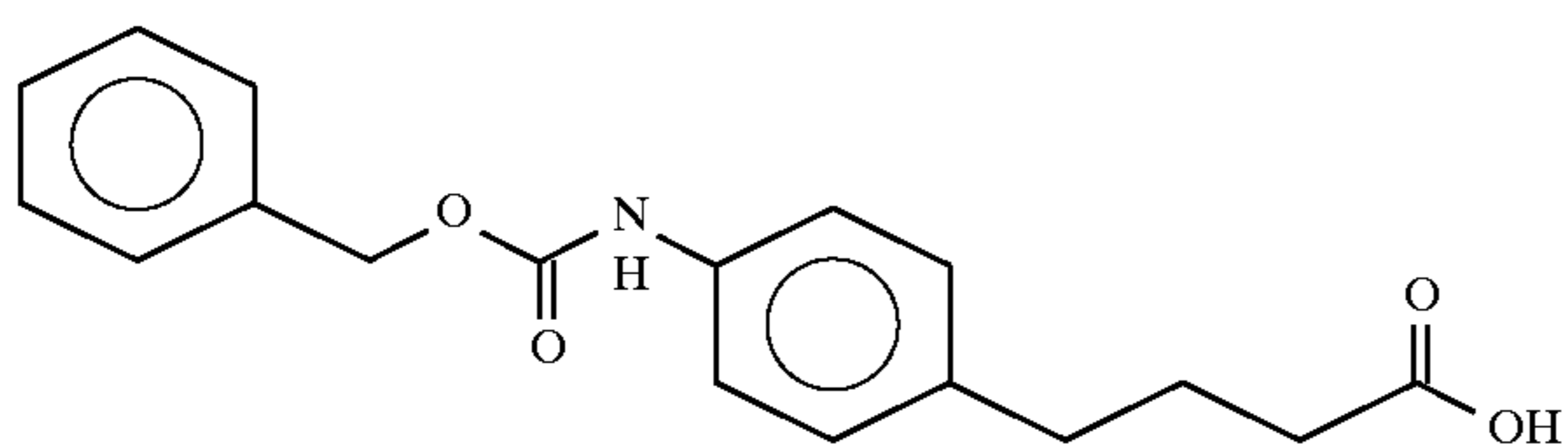
4-(4-benzyloxycarbonylamino)phenylbutyric acid
