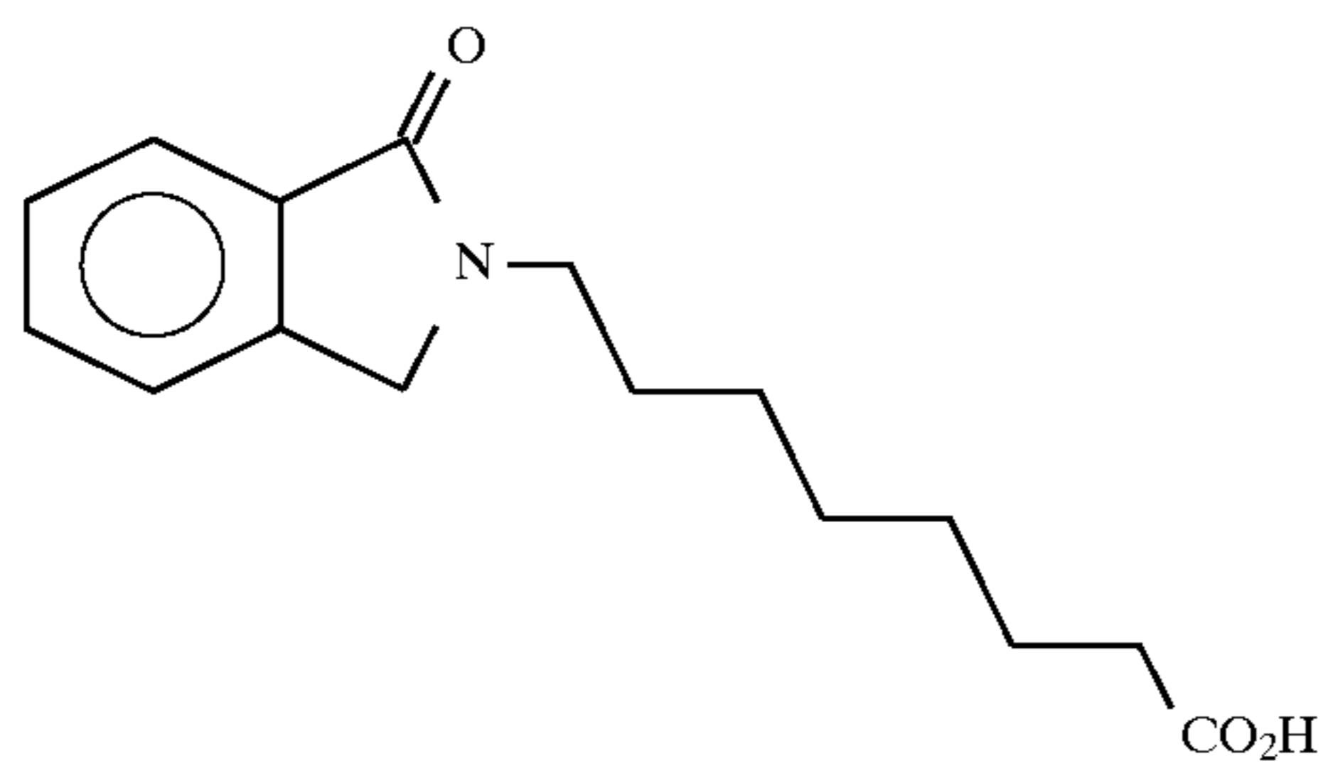
8-(2-(1,2-dihydroisoindole-1-one))octanoic acid
