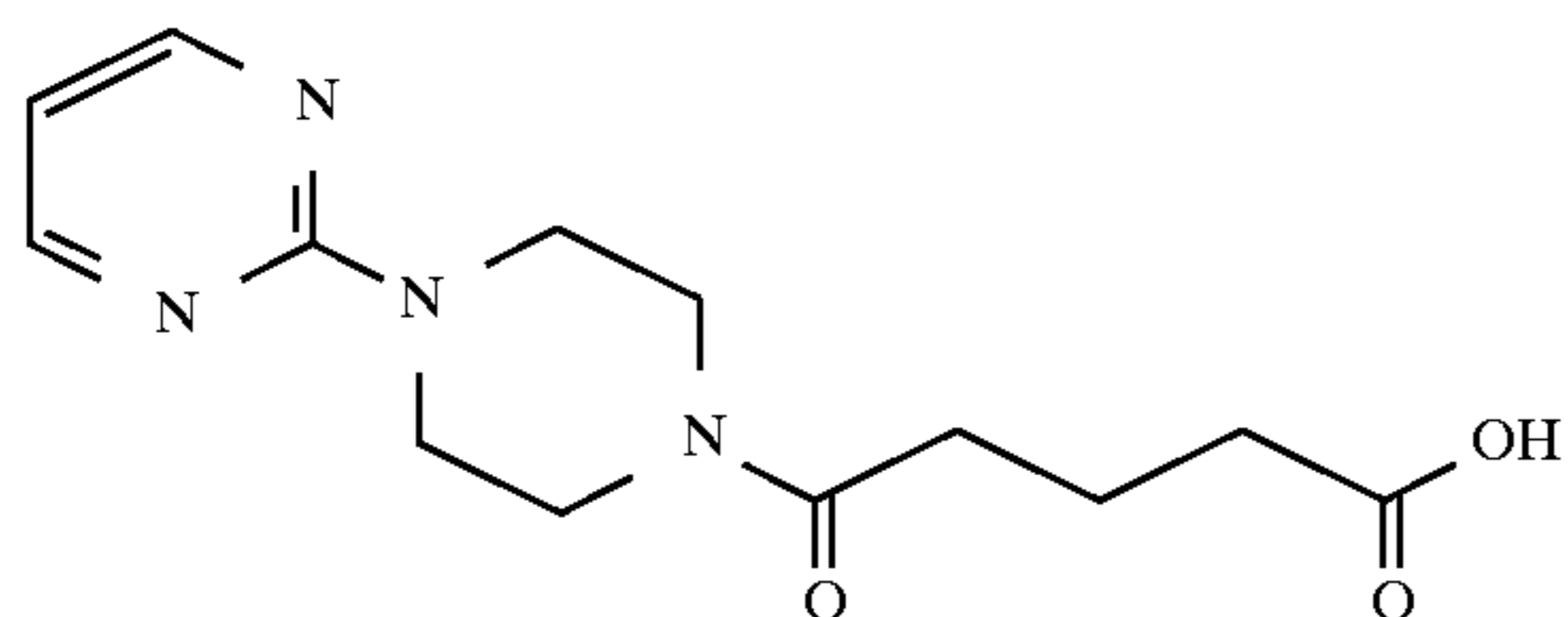
4-(1-(2-pyrimidyl)piperazinoyl)butyric acid
