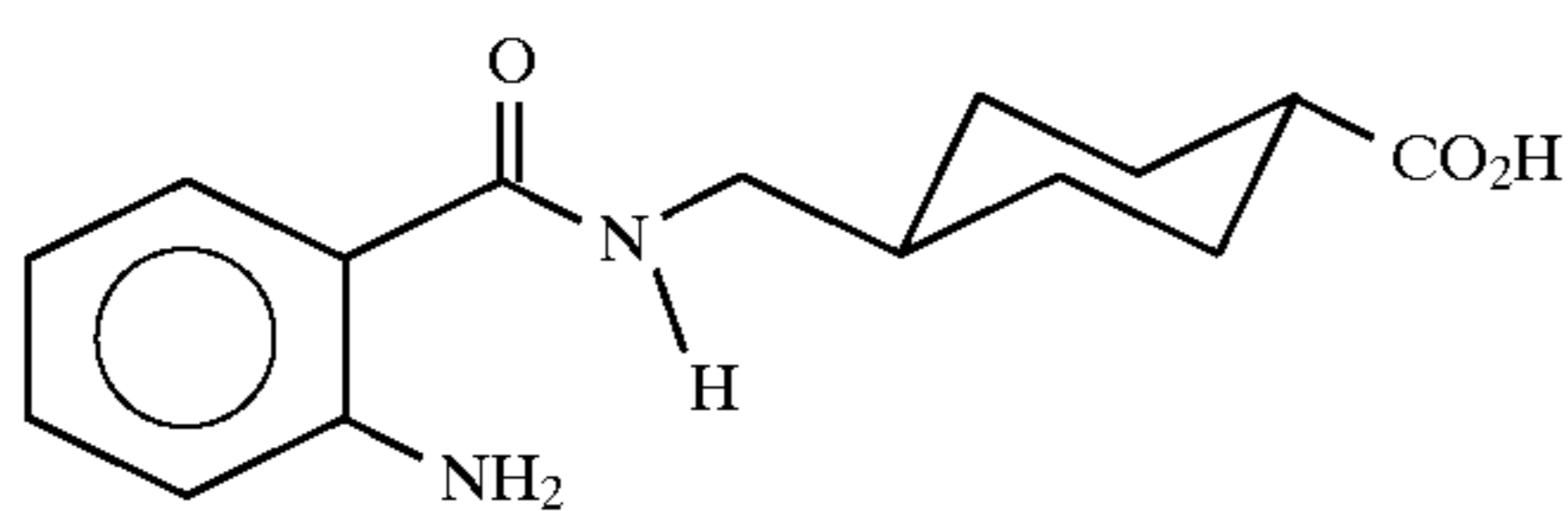
trans-4-(2-aminobenzamidomethyl)cyclohexanecarboxylic acid
