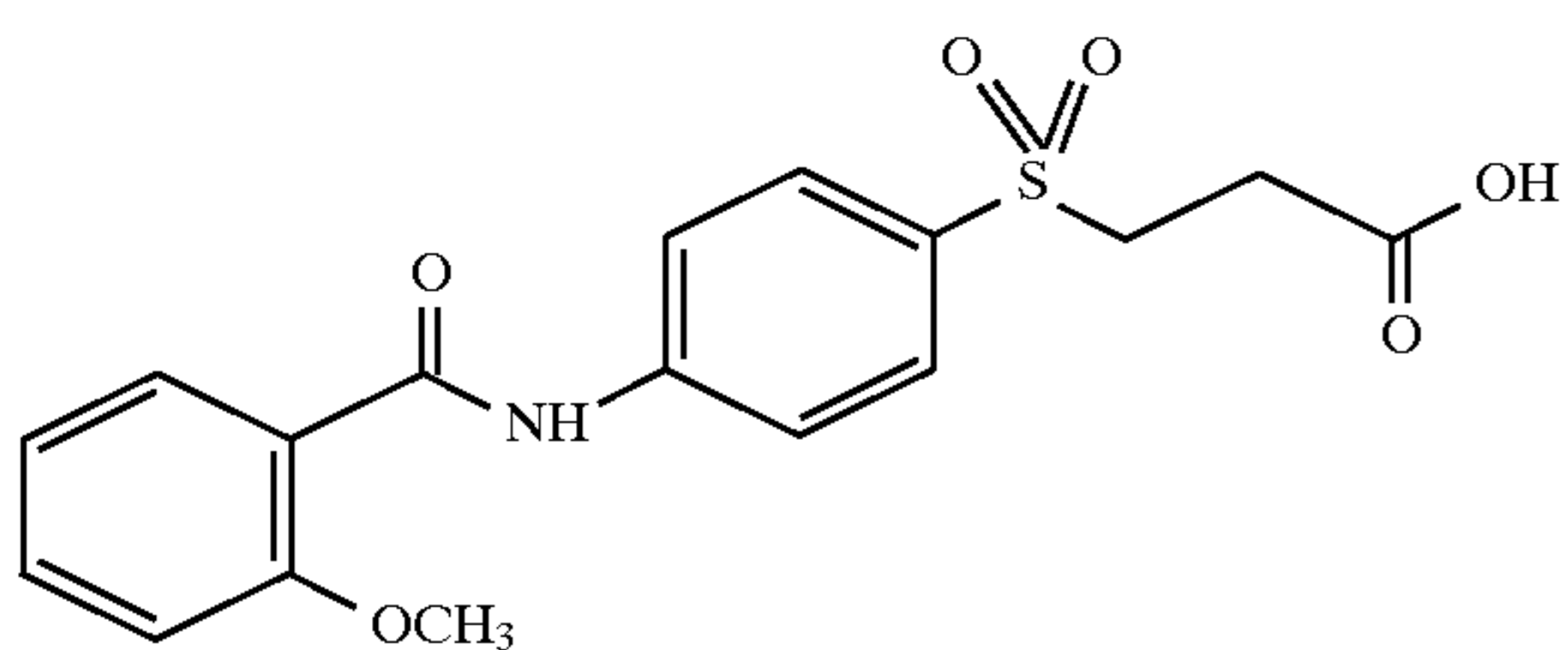
4-(2-methoxybenzoyl)amino 3-carboxypropylsulfone
