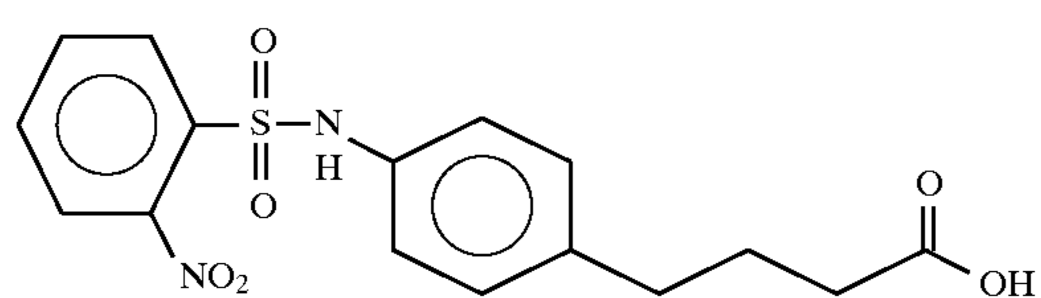
4-(4-(2-nitrobenzenesulfonyl)aminophenyl)butyric acid
