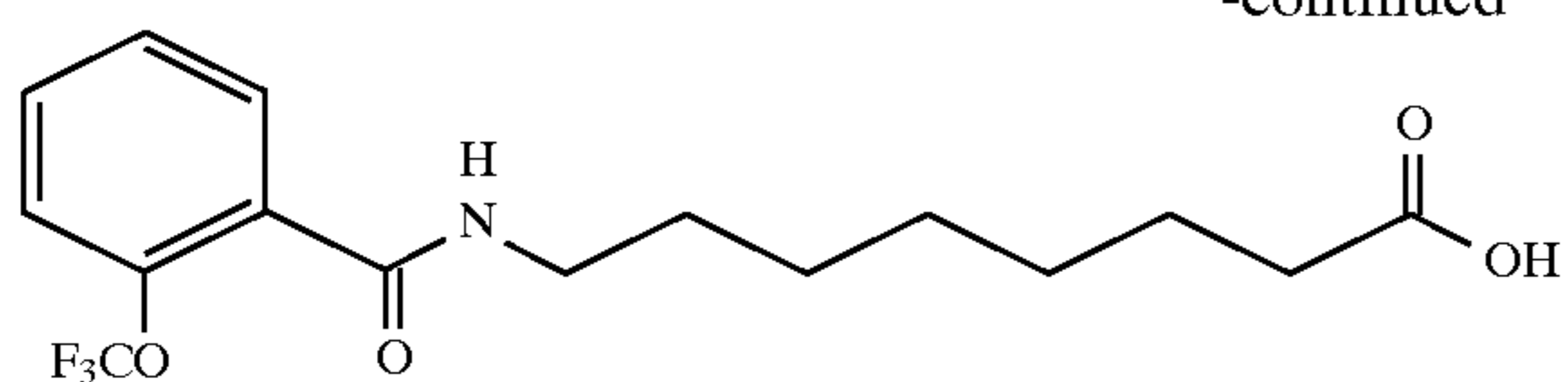
8-(2-trifluoromethoxy)benzoylamino caprylic acid
