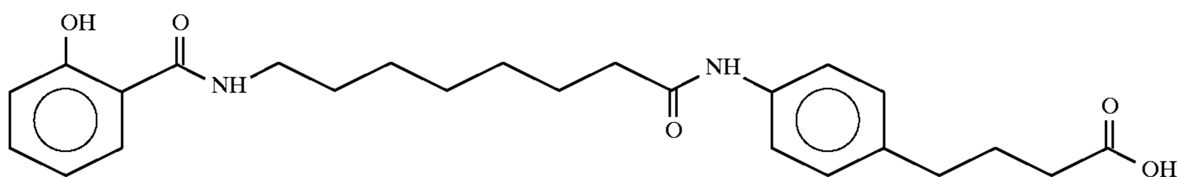
4-(4-(N-8(N-Salicyloyl)aminocaprylic)aminophenyl)butyric acid
