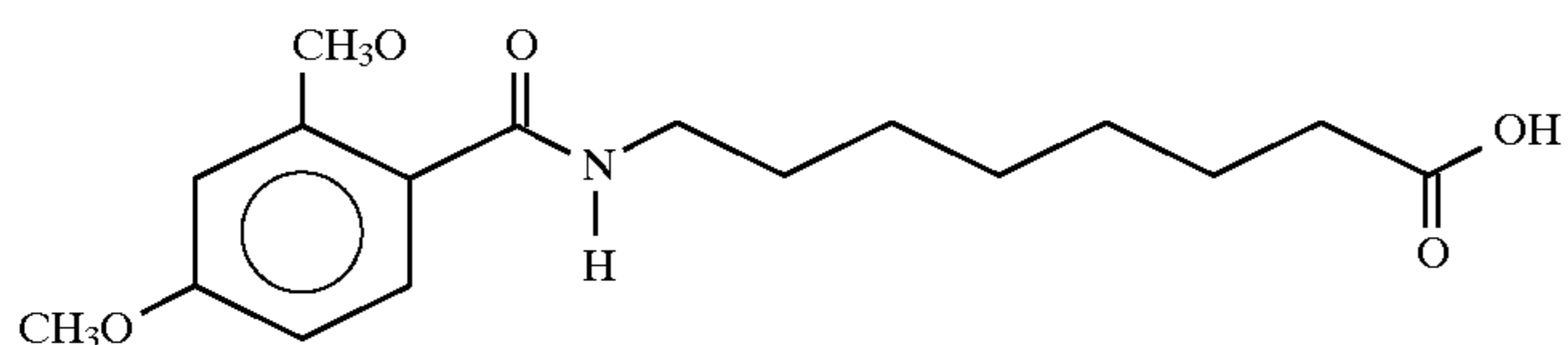
8-(N-2,4-Dihydroxybenzoyl)aminocaprylic acid
