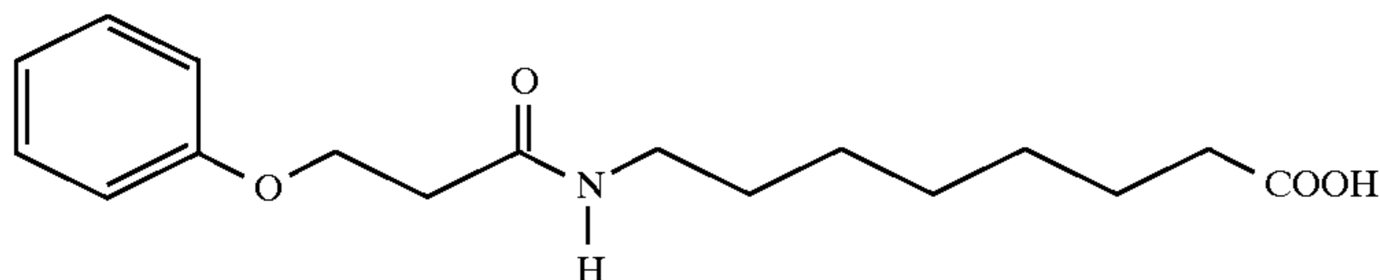
8-(3-Phenoxypropionylamino)caprylic acid
