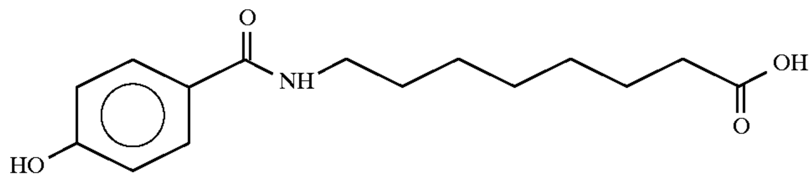
8-(4-Hydroxybenzoyl)aminocaprylic acid
