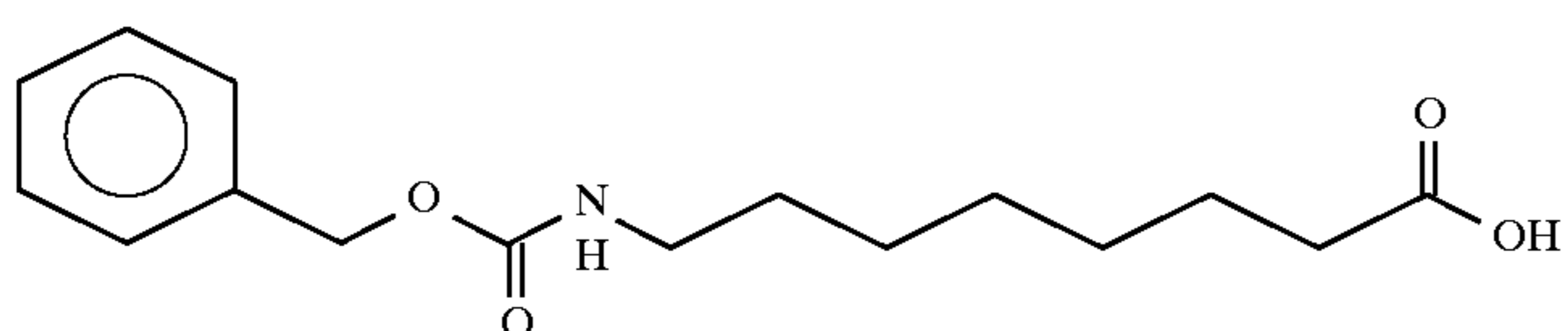
8-(Benzylcarbonylamino)caprylic acid
