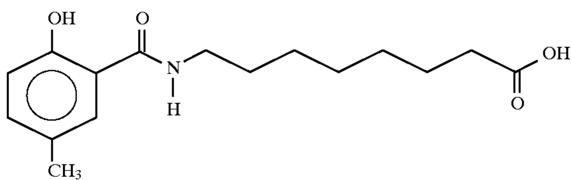
8-(N-5-methylsalicyloyl)aminocaproic acid
