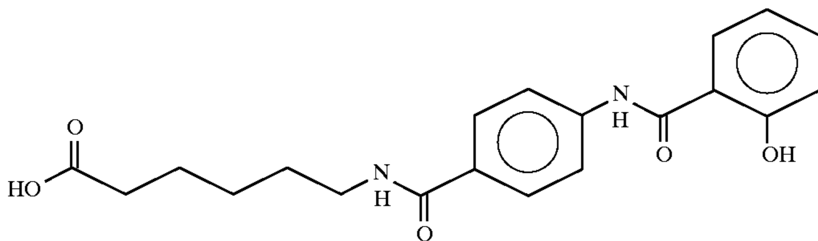
N-(4-salicyloylamino)-6-caproic acid
