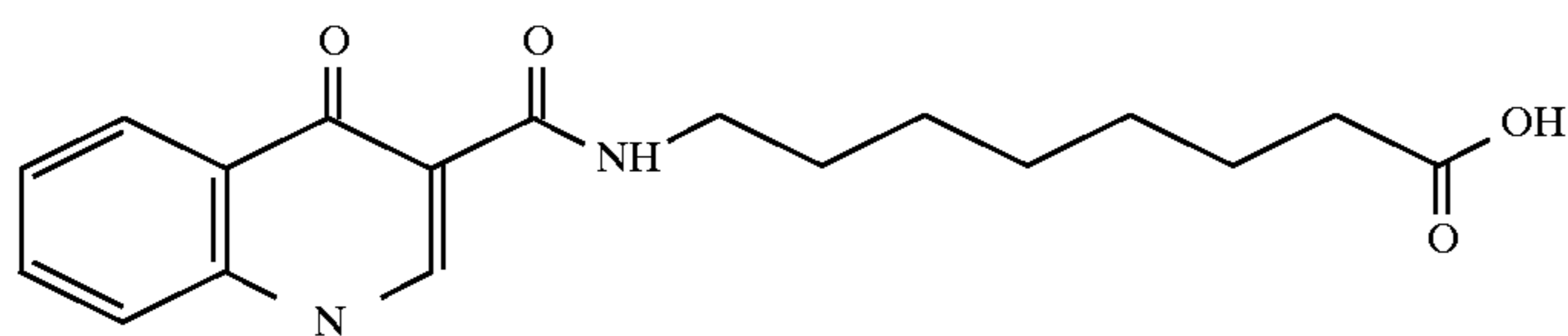
8-(chromone-3-carbonyl)aminocaprylic acid
