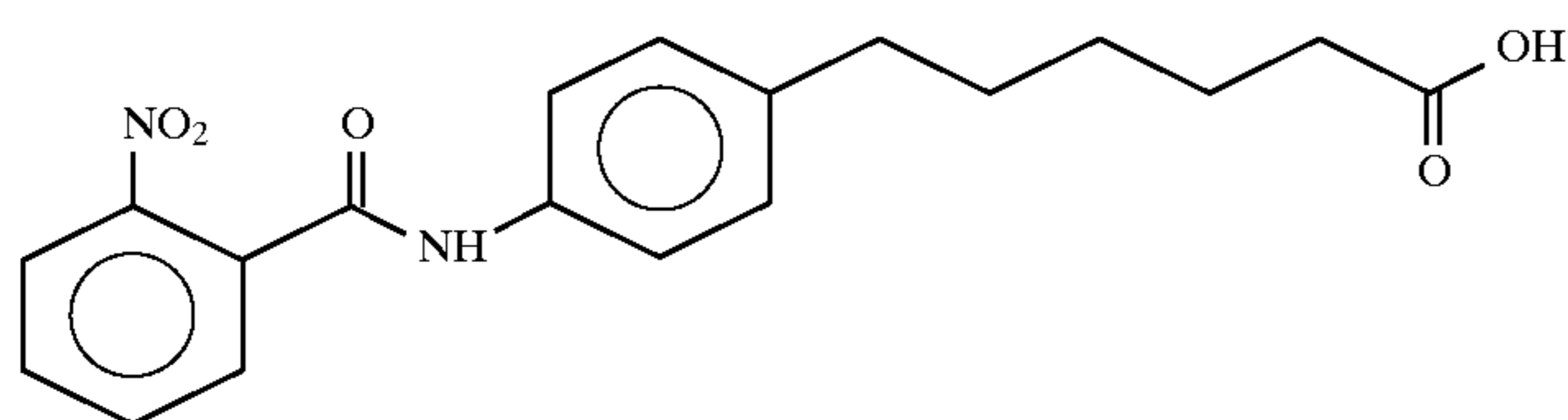
6-(4-(N-(2-Nitrobenzoyl)aminophenyl)hexanoic acid
