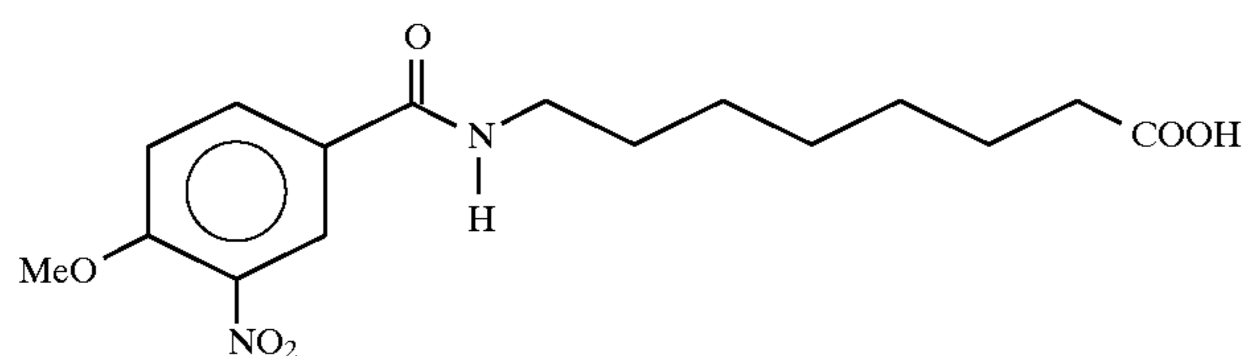
8-N-(4-methoxy-3-nitrobenzoyl)aminocaprylic acid
