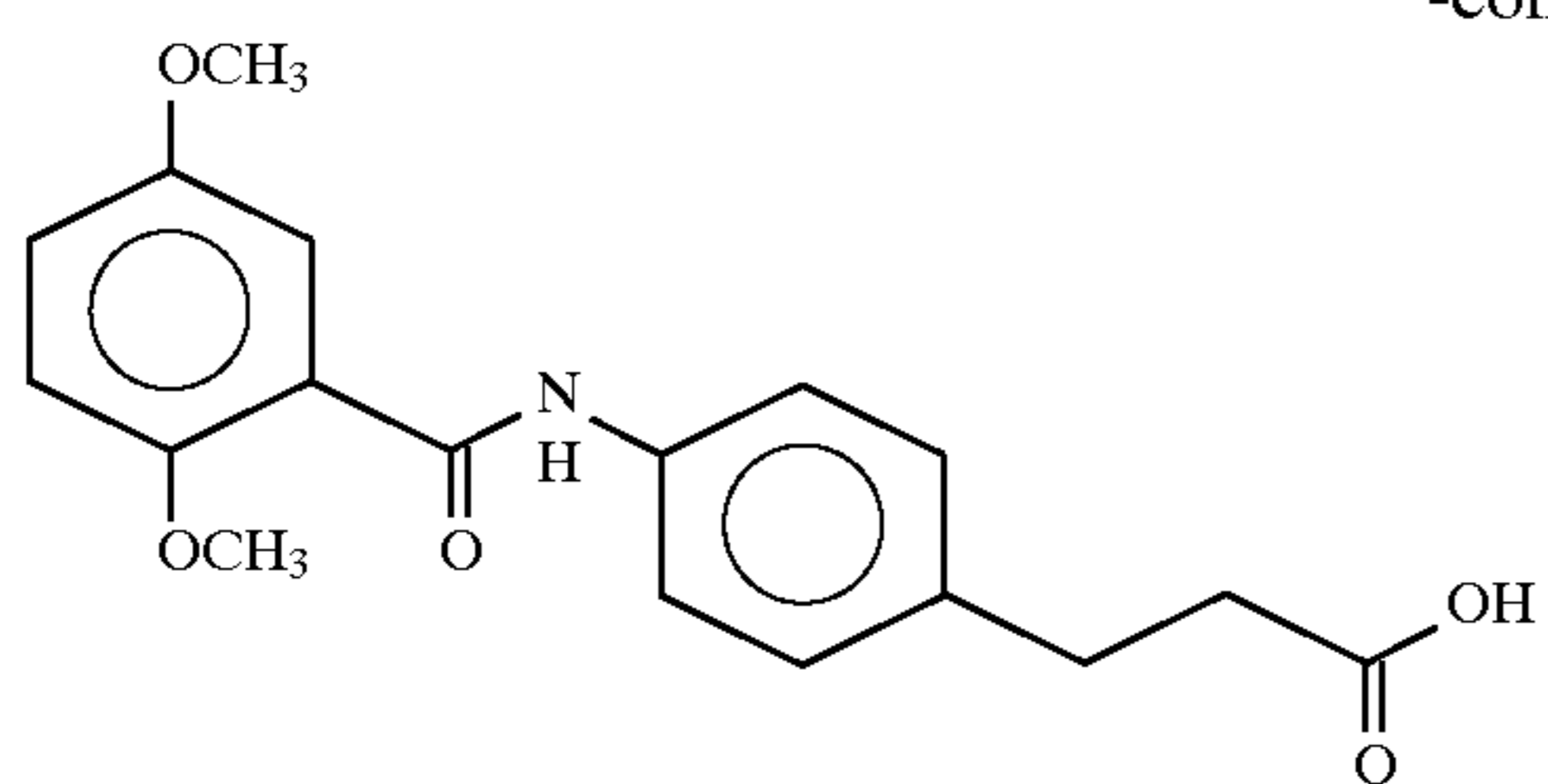
3-(4-(2,5-dimethoxybenzoyl)aminophenyl)propionic acid
