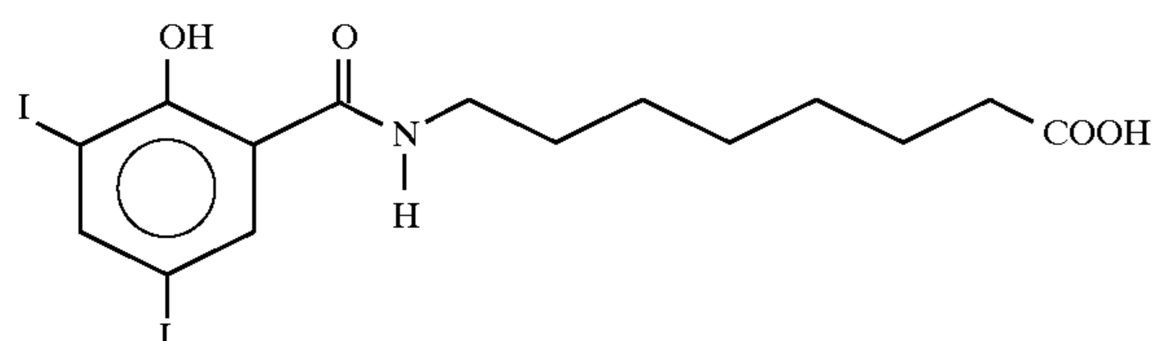
8-(N-(2-hydroxy-3,5-diiodobenzoyl)aminocaprylic acid
