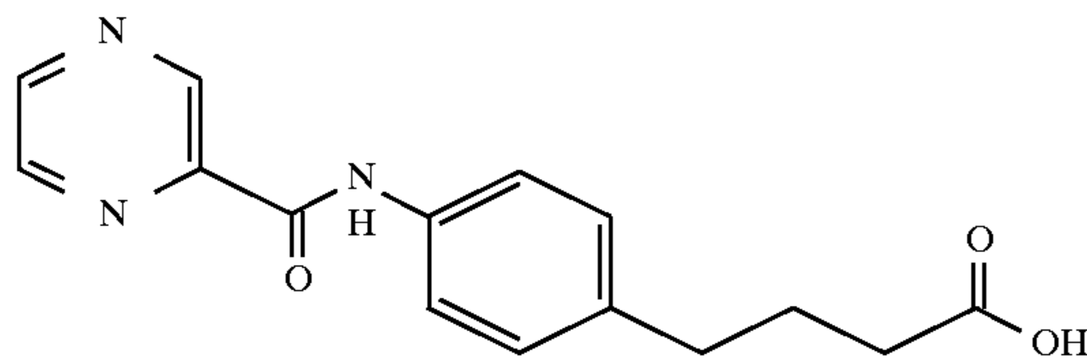
4-(4-(2-pyrazinecarbonyl)aminophenyl)butyric acid
