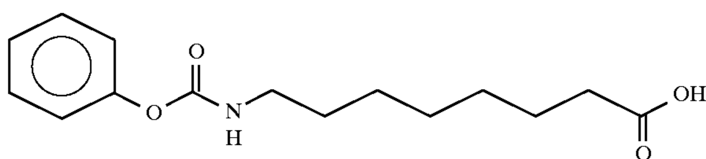
8-(phenylcarbonylamino)caprylic acid
