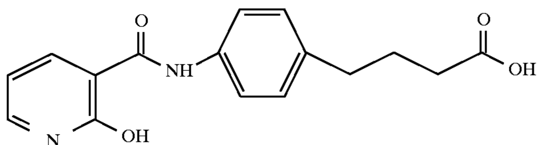
4-(4-(2-hydroxynicotinoyl)aminophenyl)butyric acid
