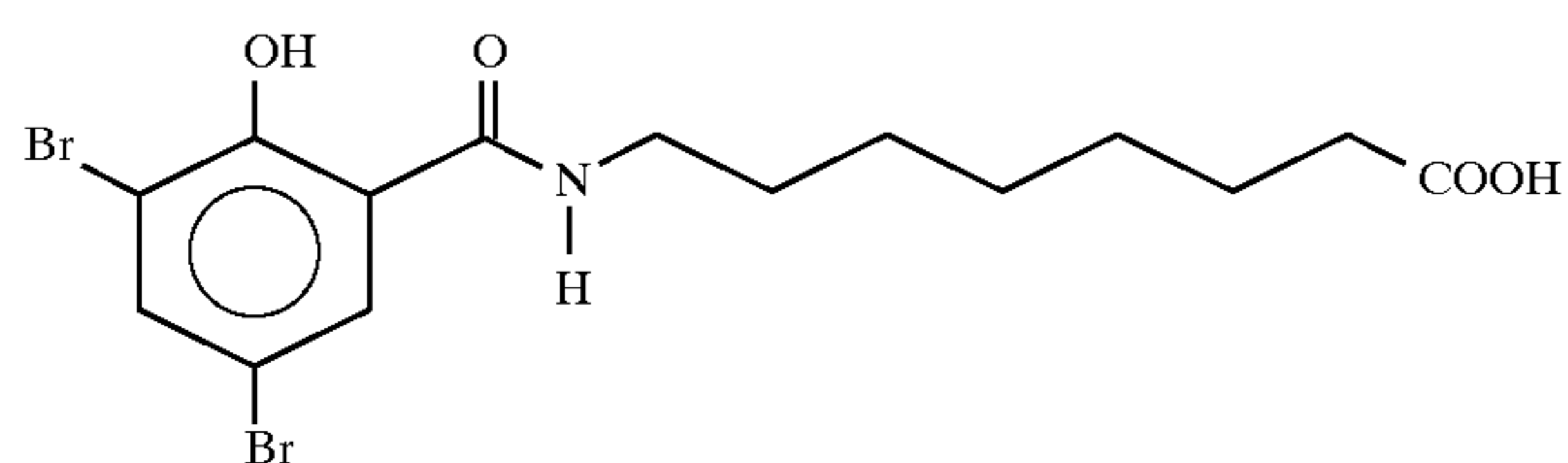
8-[N-(2-hydroxy-3,5-dibromobenzoyl)]aminocaprylic acid
