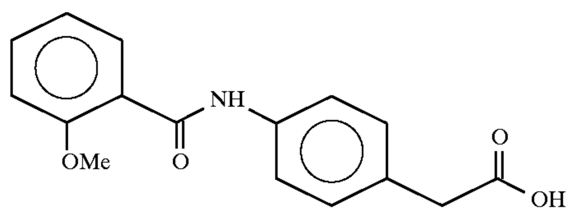
4-(o-anisoyl)aminophenylacetic acid
