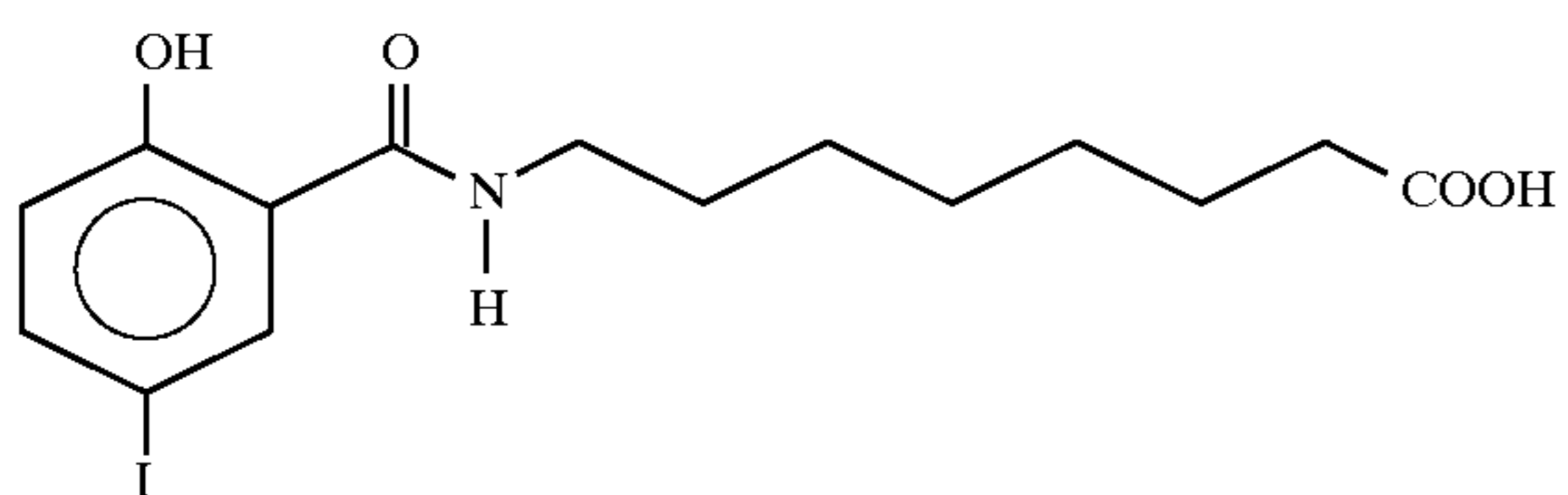
8-(N-(2-hydroxy-5-iodobenzoyl)aminocaprylic acid
