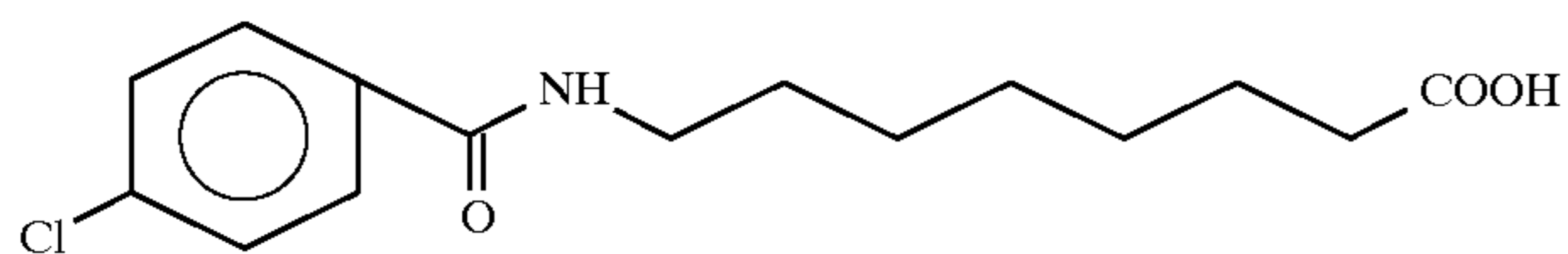
8-[N-(4-chlorobenzoyl)]aminocaprylic acid
