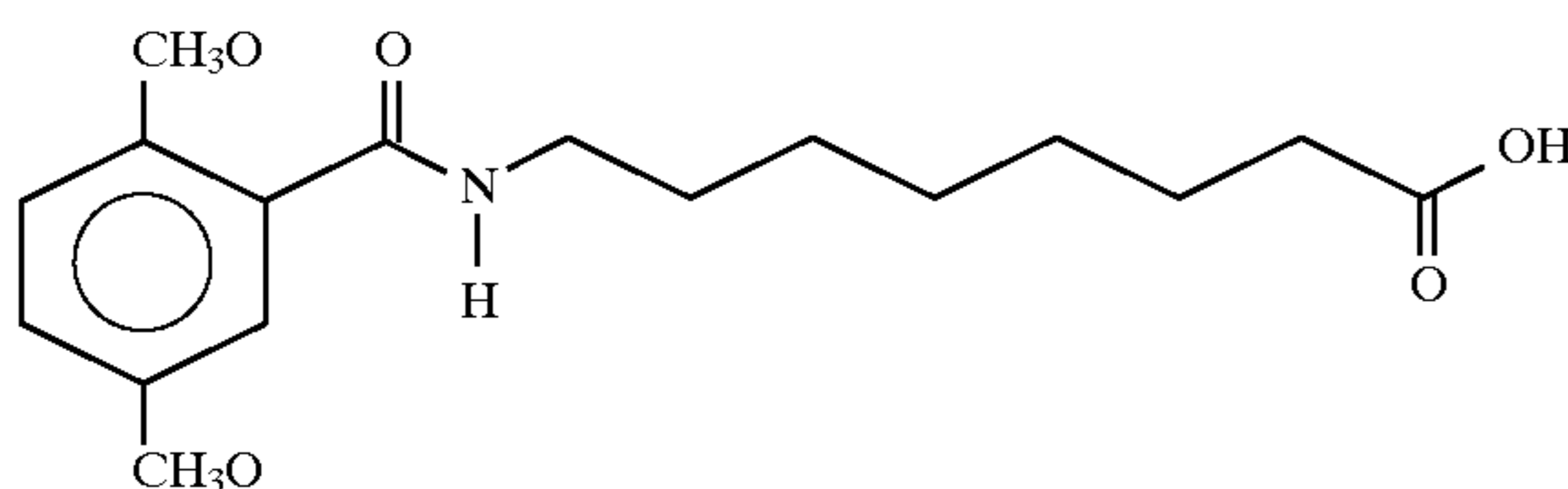
8-(N-2,5-Dimethoxybenzoyl)aminocaprylic acid
