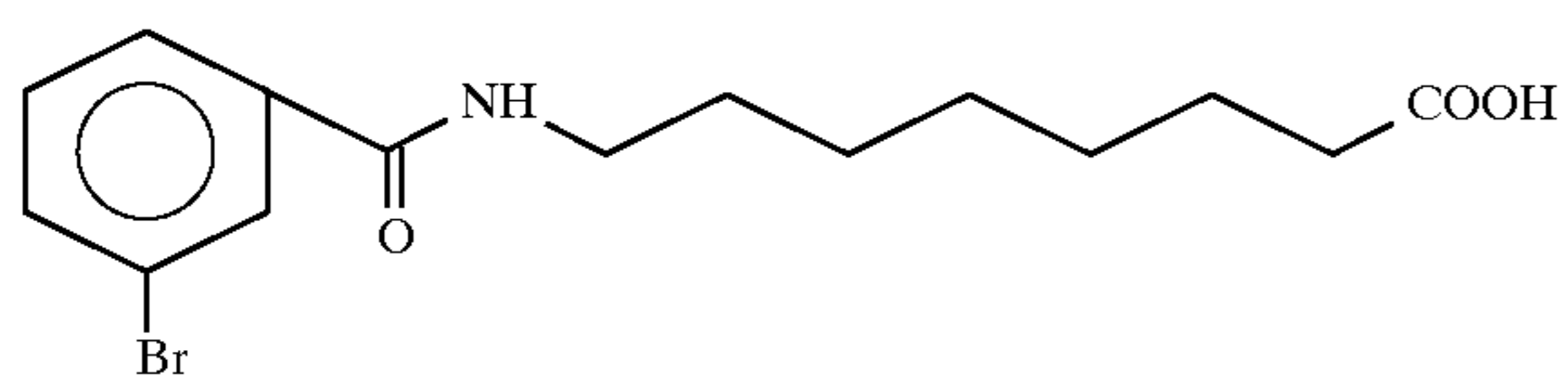
8-[N-(3-bromobenzoyl)]aminocaprylic acid
