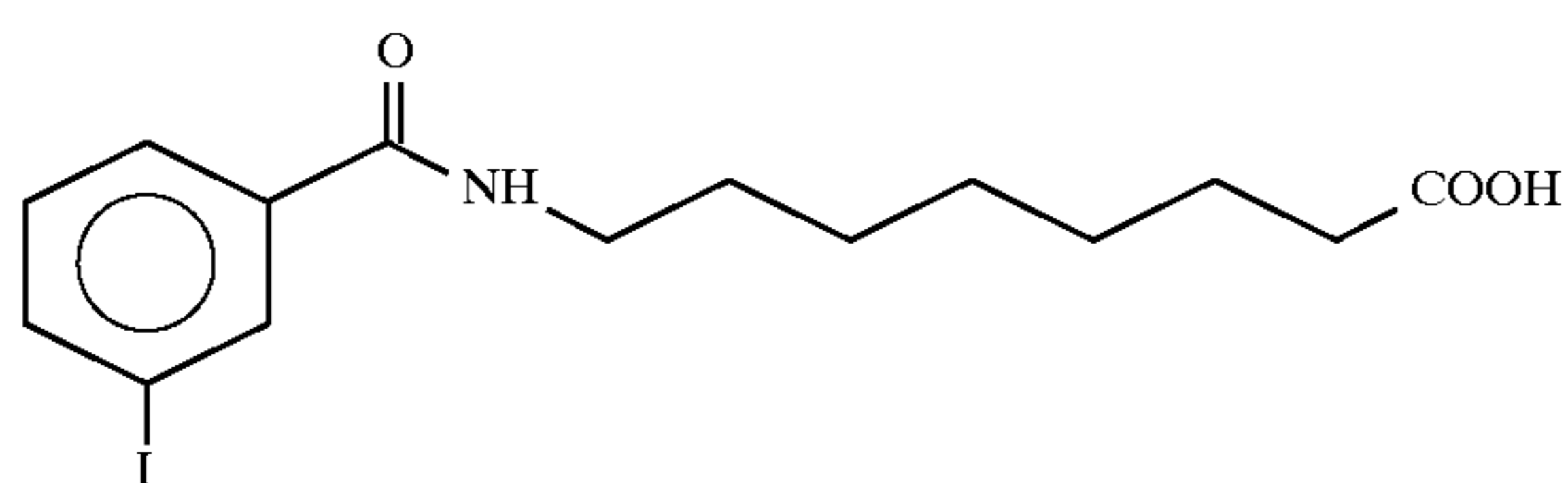
8-N-(3-iodobenzoyl)aminocaprylic acid
