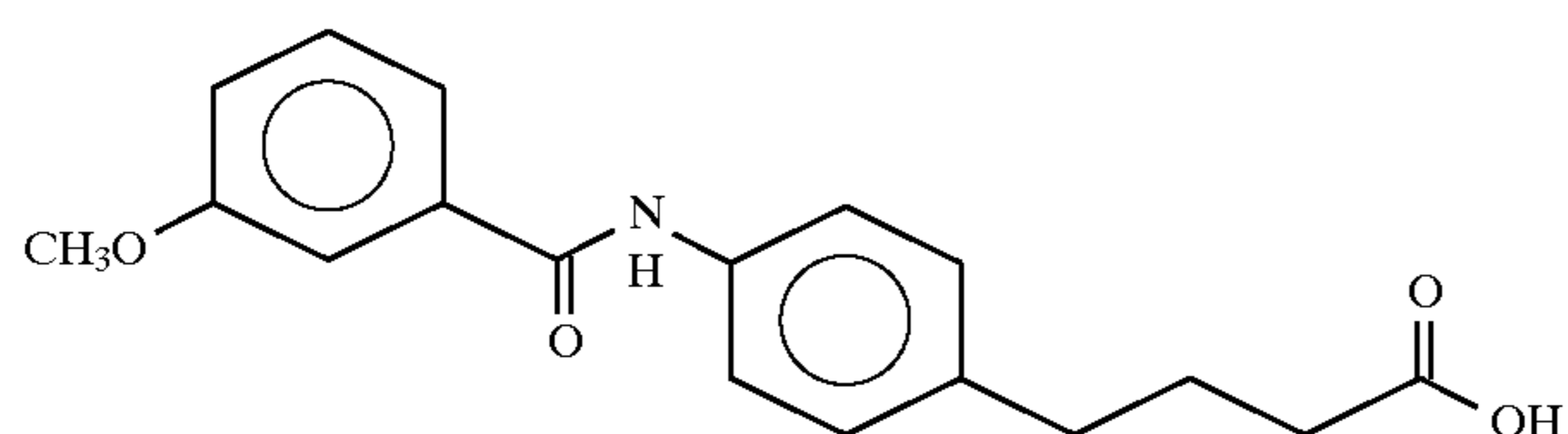
4-(4-(3-anisoyl)aminophenyl)butyric acid
