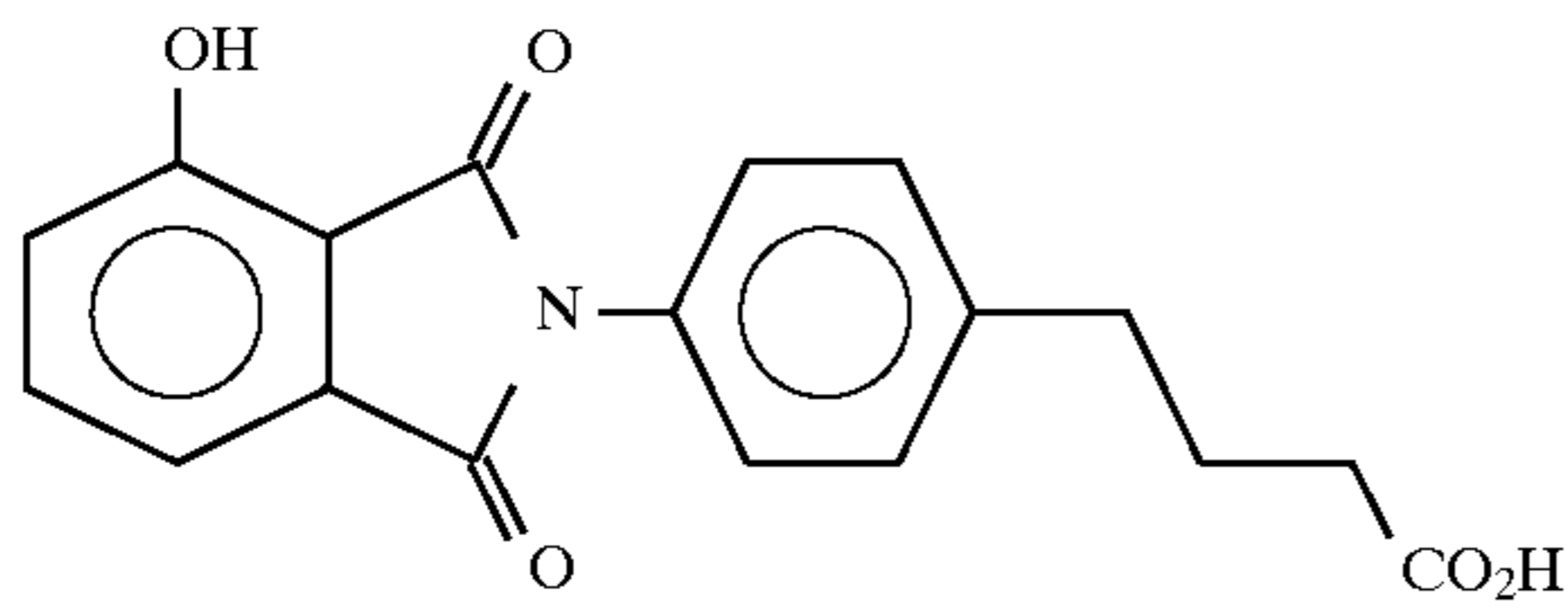
4-(4-(3-hydroxyphthalimido)phenyl)butyric acid
