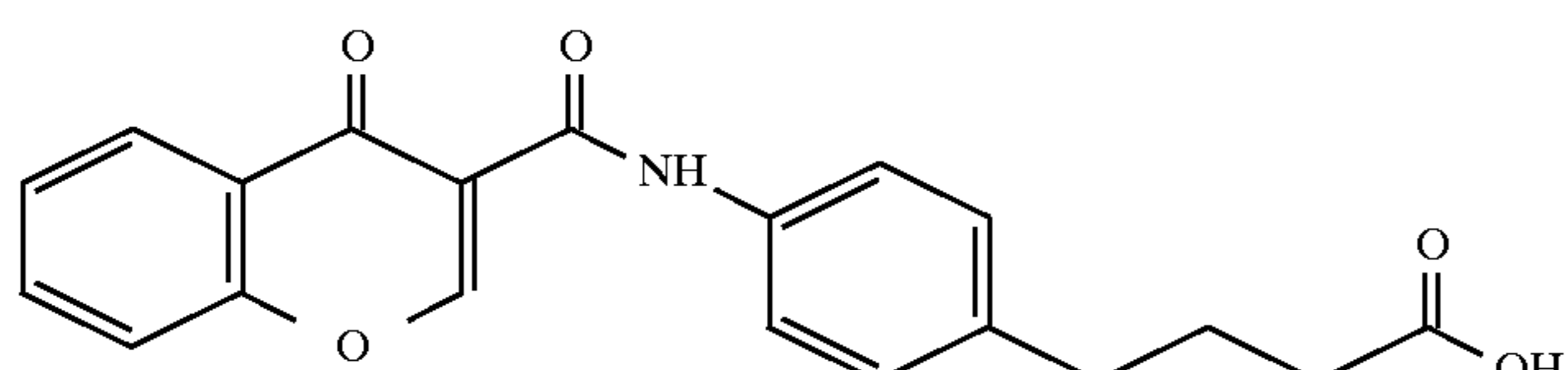
4-(4-chromone-3-carbonyl)aminophenylbutyric acid
