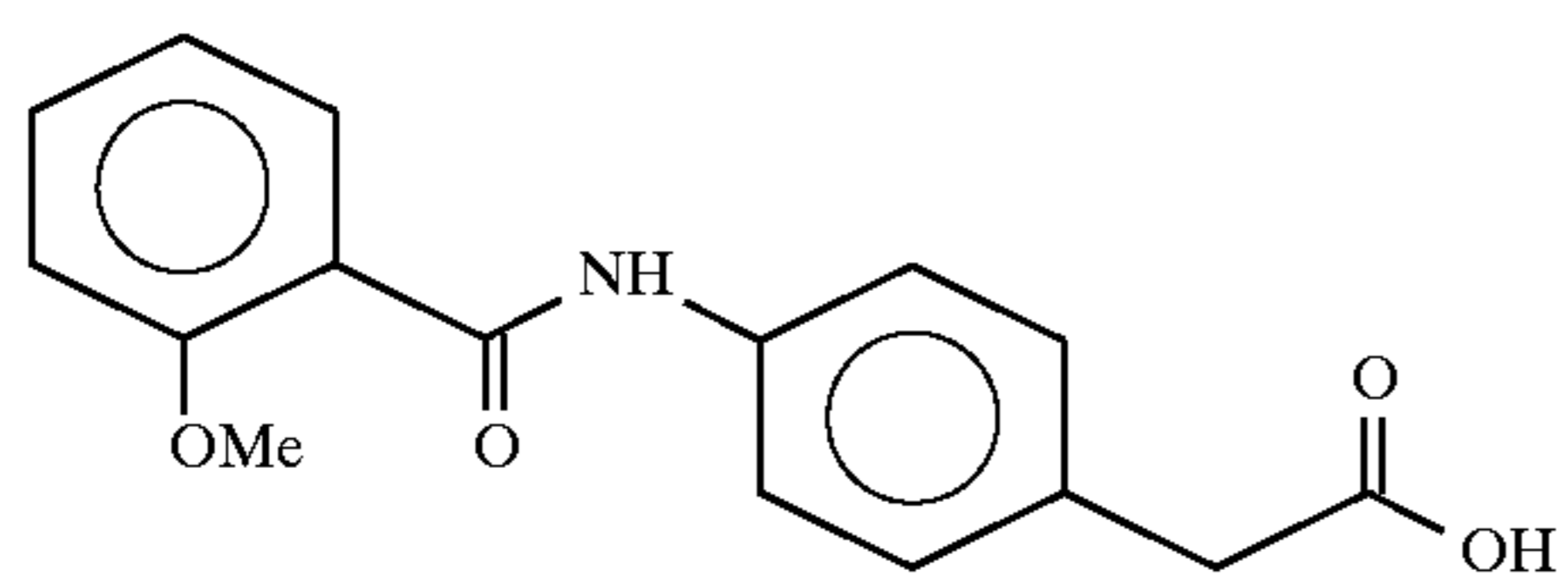
4-(o-anisoyl)aminophenylacetic acid
