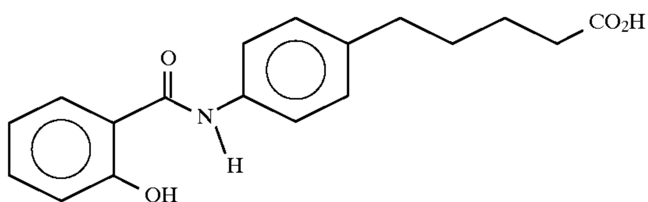
N-salicyloyl-5-(4-aminophenyl)valeric acid
