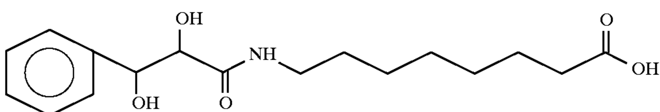
(3-phenyl-2,3-dihydroxypropanoyl)8aminocaproic acid
