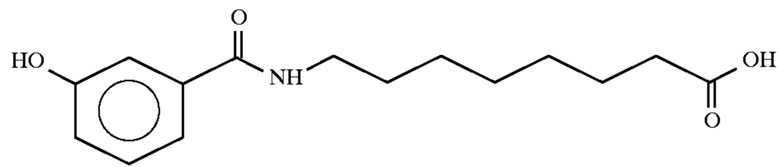
8-(3-Hydroxybenzoyl)aminocaprylic acid
