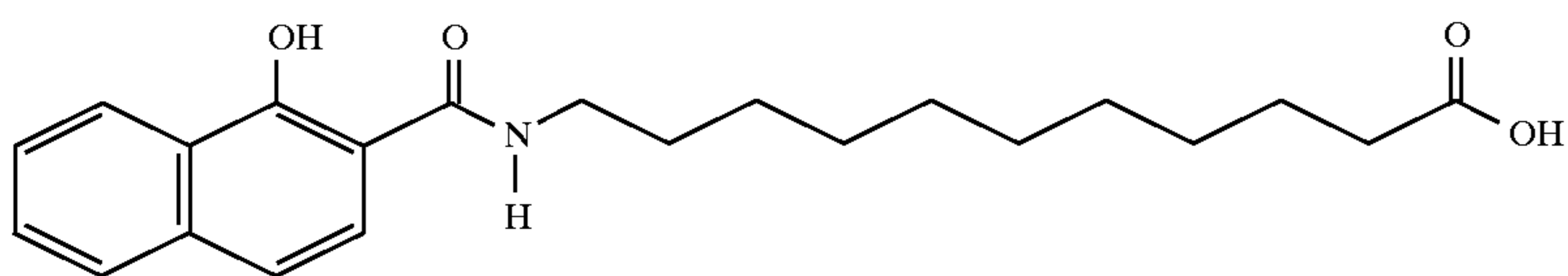
11-N-(1-hydroxy-2-naphthoyl)aminoundecanoic acid
