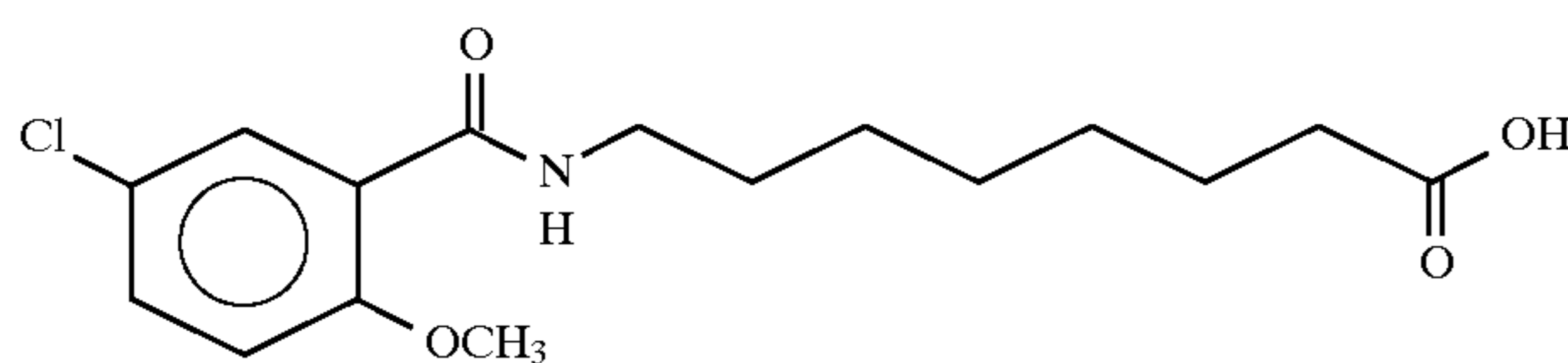
8-(5-chloro-o-anisoyl)aminocaproic acid
