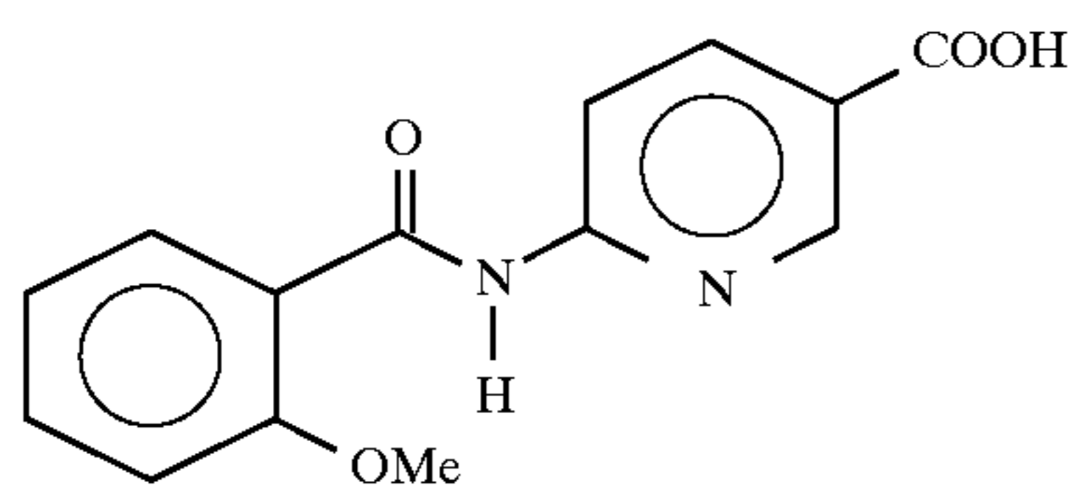
6-(2-methoxybenzoyl)amino nicotinic acid
