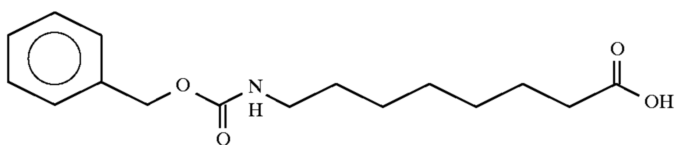
8-(Benzylcarbonylamino)caprylic acid
