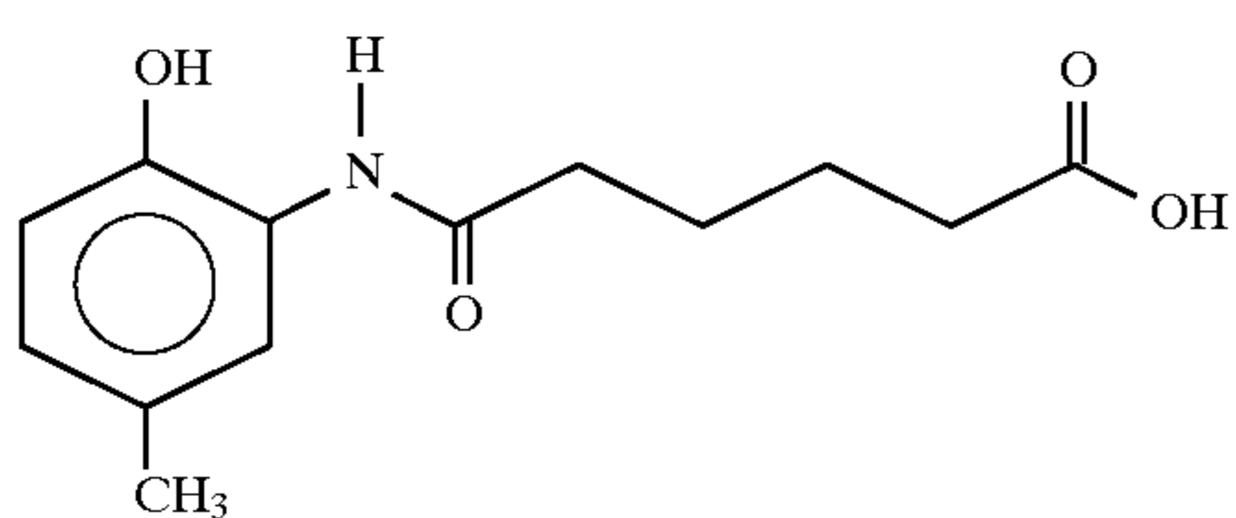
5-(2-hydroxy-5-methylanilino)valeric acid
