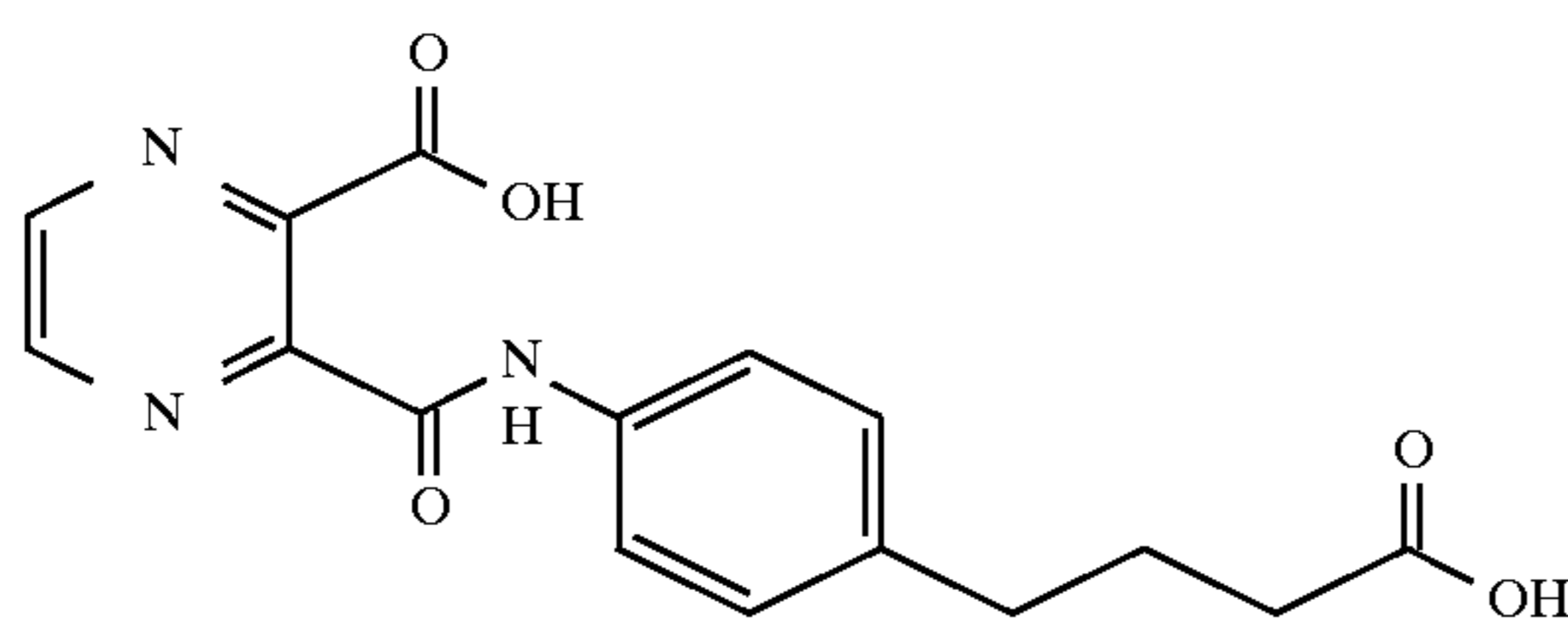
4-(4-(2-(3-carboxyl)pyrazinecarbonyl)aminophenyl)butyric acid
