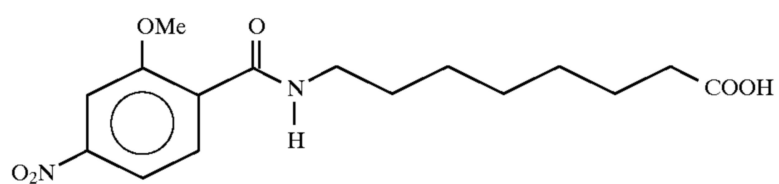
8-N-(4-methoxy-3-nitrobenzoyl)aminocaprylic acid
