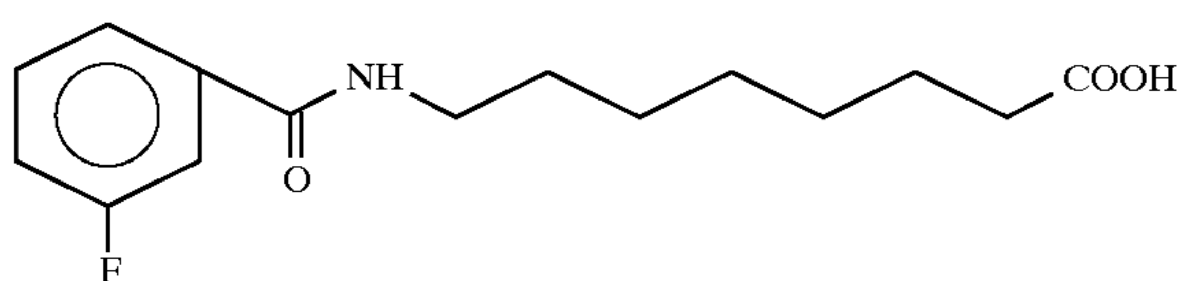
8-(N-3-fluorobenzoyl) aminocaprylic acid
