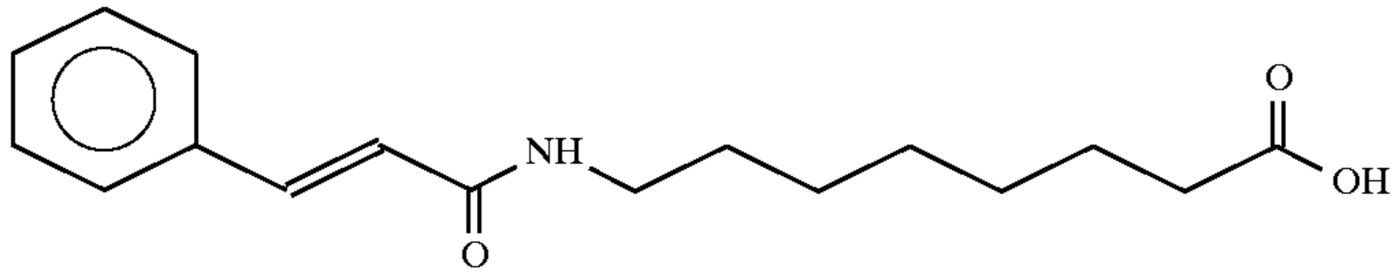
8-cinnamoylaminovaleric acid
