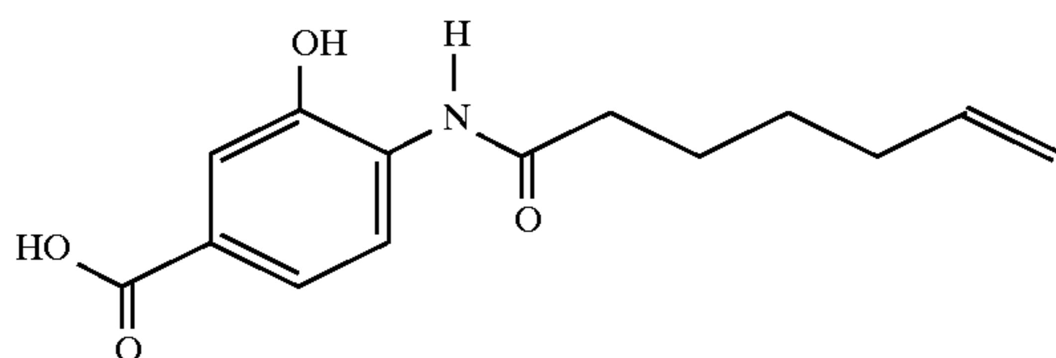
N-(2-hydroxy-4-carboxy)-6-heptenamide
