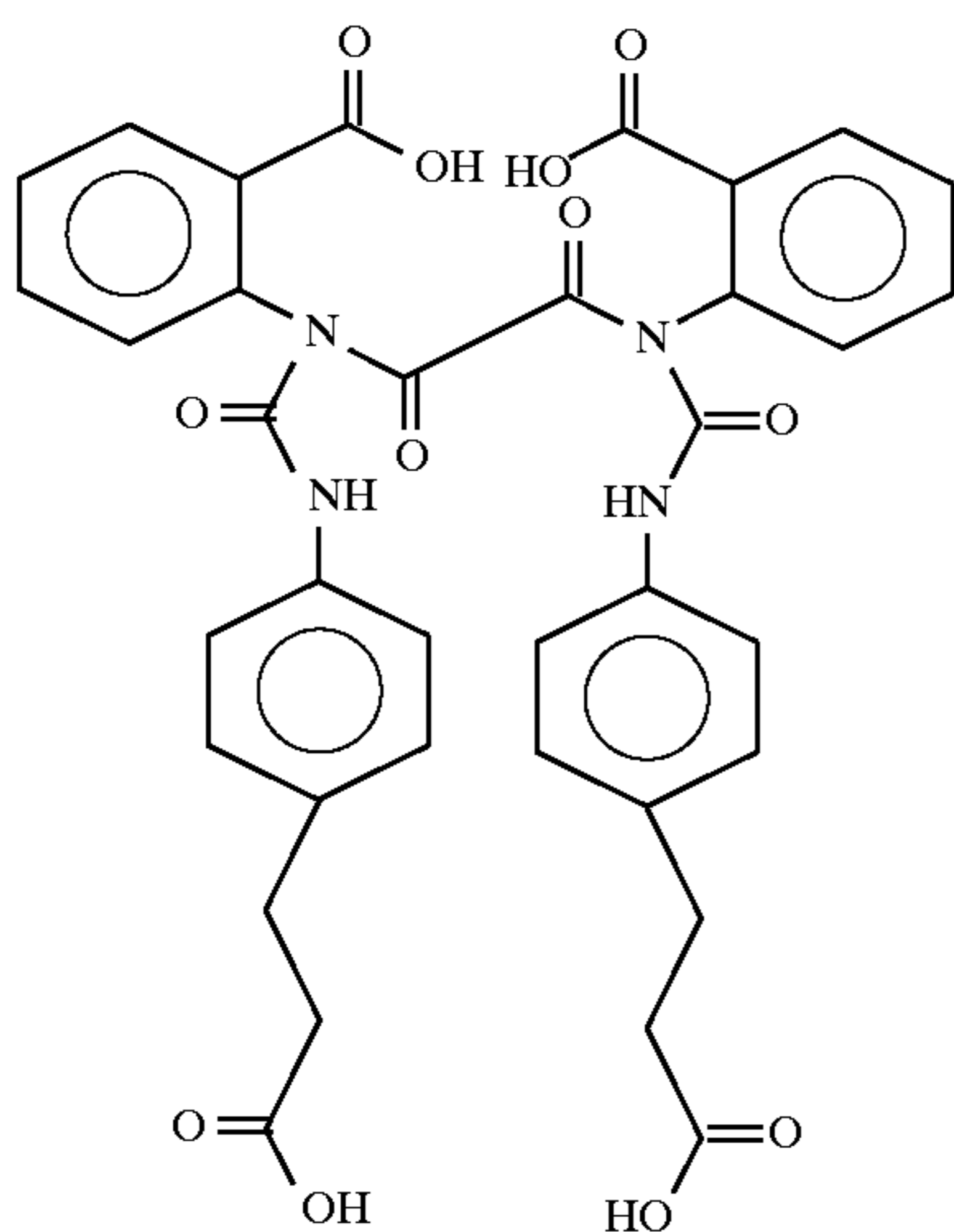
Bis(N-2-carboxyphenyl-N-(N'-3(4-aminophenyl)propionic acid)ureal)oxalylyl diamide
