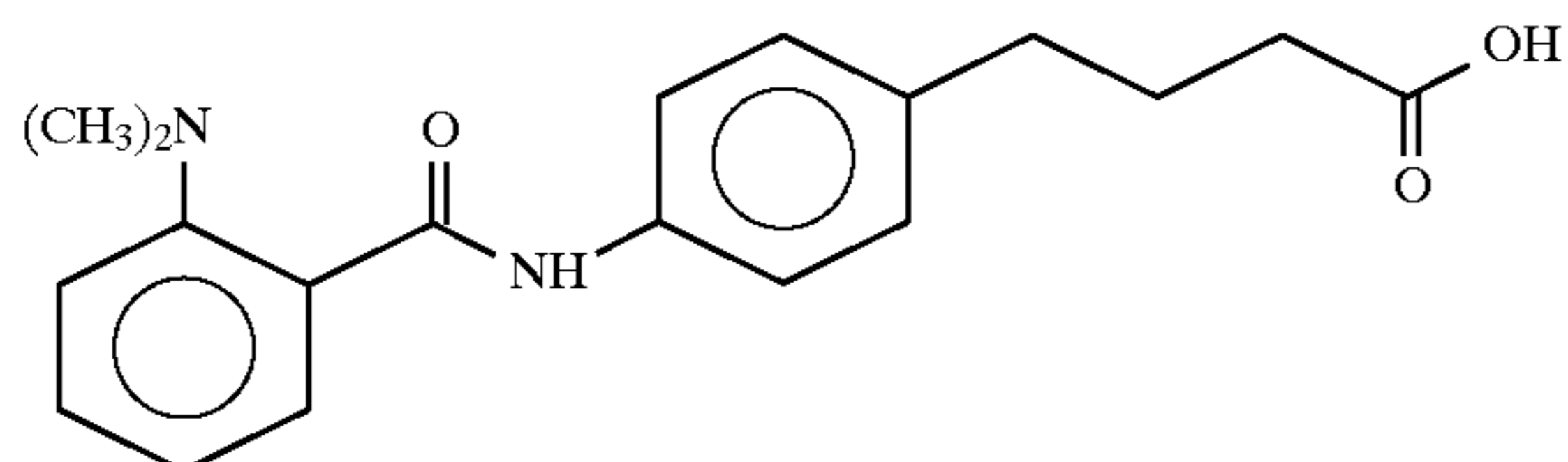
4-(4-(2-Dimethylamino benzoic)aminophenyl)butyric acid
