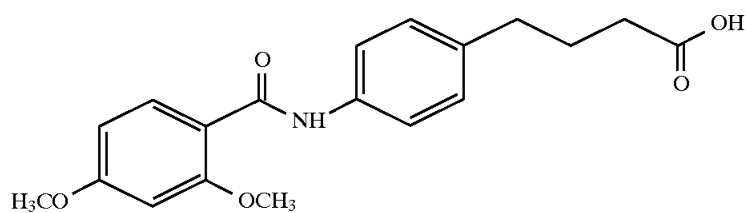
4-(4-(2,4-dimethoxybenzoyl)aminophenyl)butyric acid
