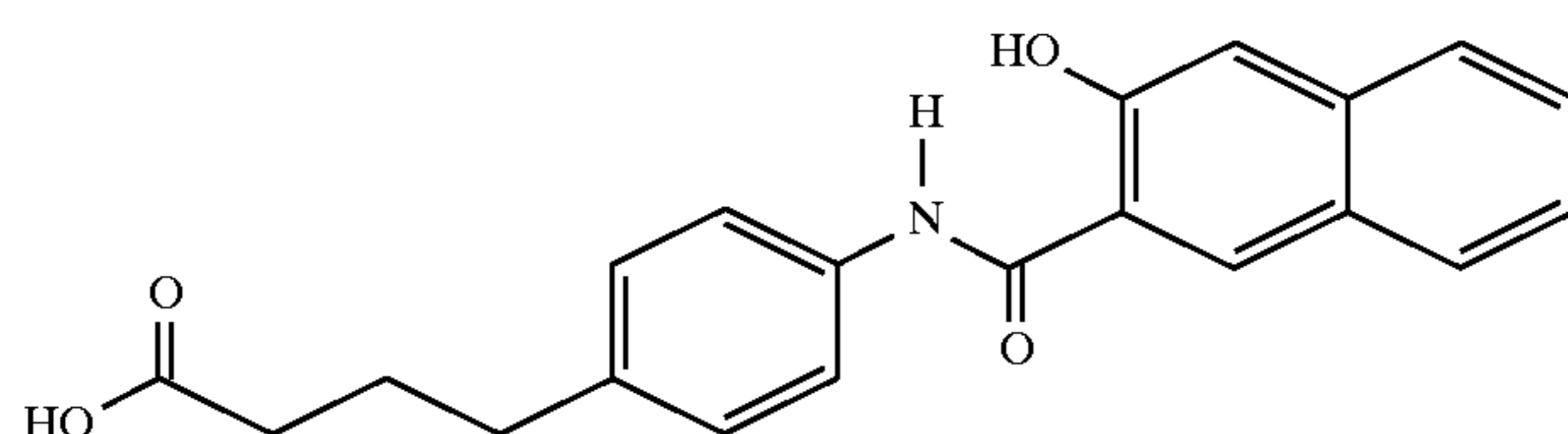
4-(4-(N-(3-hydroxy-2-naphthoyl)aminophenyl)butanoic acid
