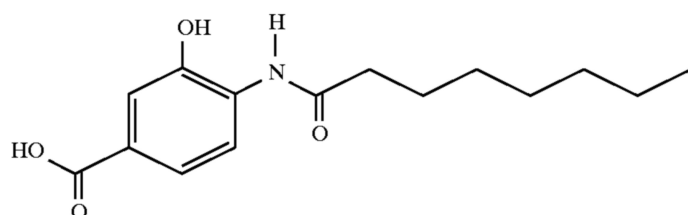
4-octanoylamino-3-hydroxybenzoic acid
