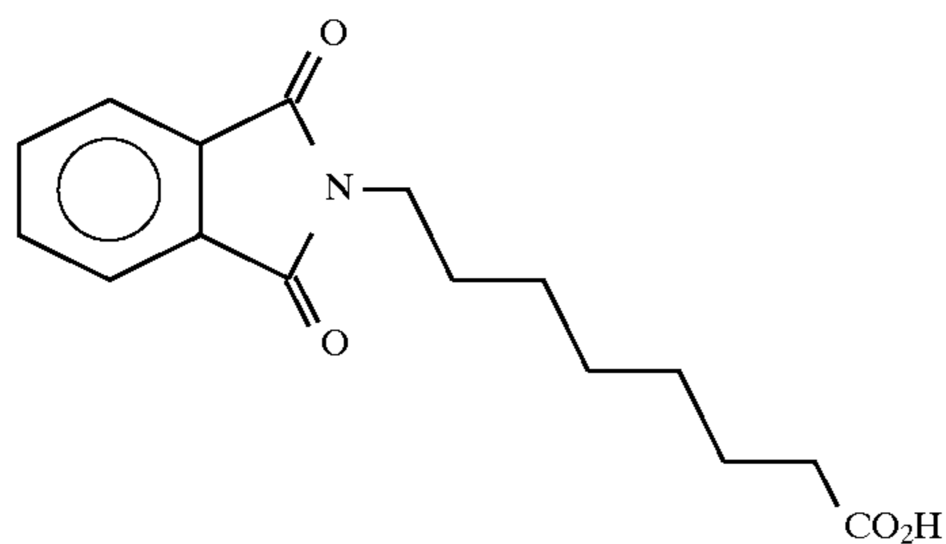
8-(phthalimido)caprylic acid
