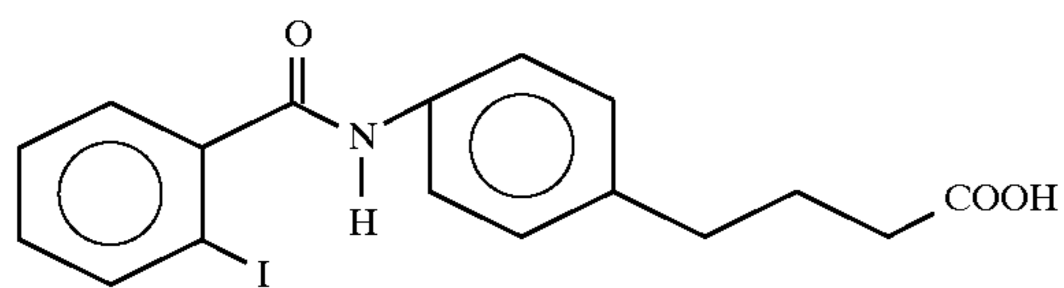
4-{4-[N-(2-iodobenzoyl)aminophenyl]}butyric acid
