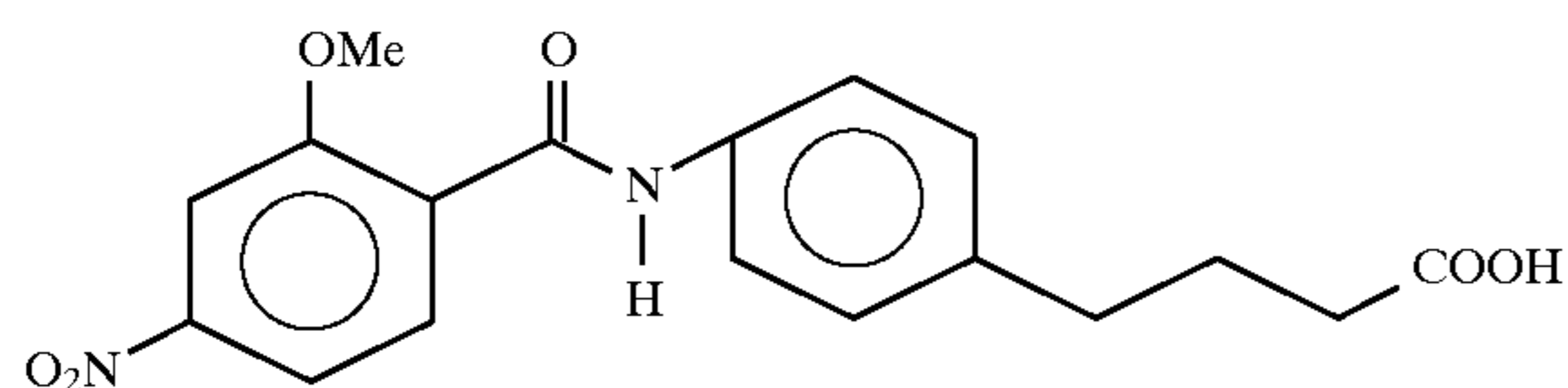
4-{N-[4-(2-methoxy-4-nitrobenzoyl)aminophenyl]}butyric acid
