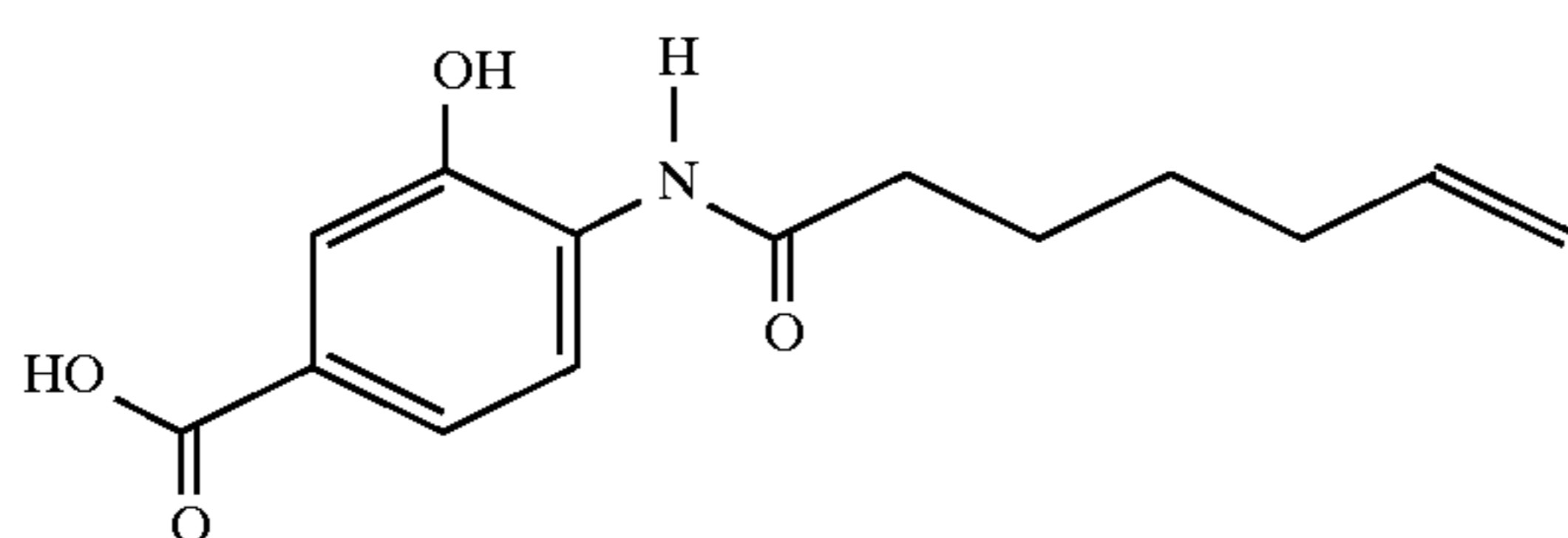
N-(2-hydroxy-4-carboxy)-6-heptenamide
