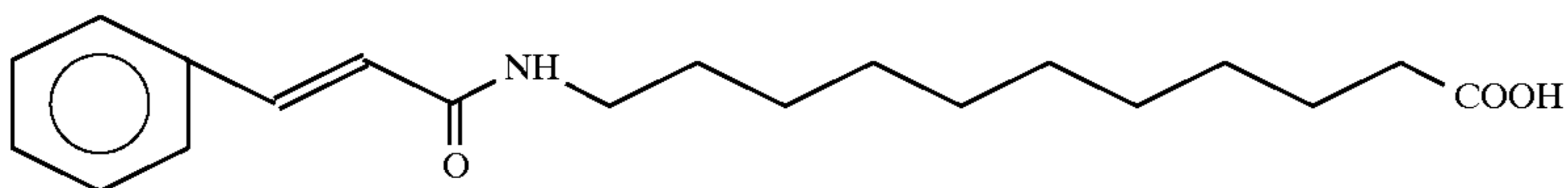
11-cinnamoylaminoundecanoic acid
