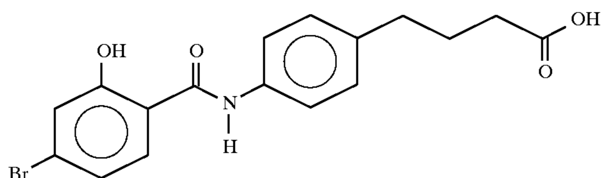
4-[N-(2-hydroxy-4-bromobenzoyl)aminophenyl]butyric acid
