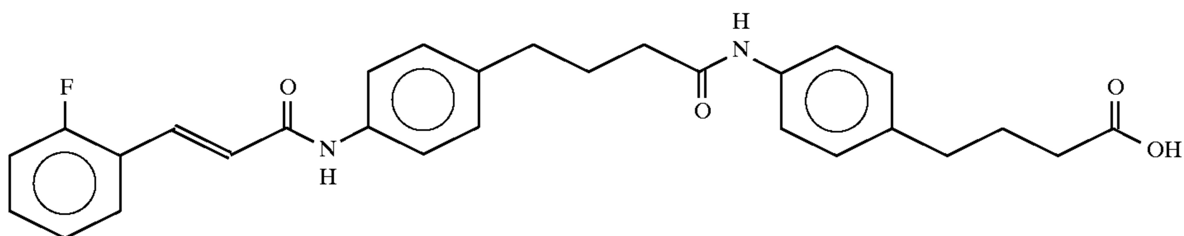
4-(4-(N-(2-Fluorocinnamoyl)aminophenyl)butyric)butyric acid
