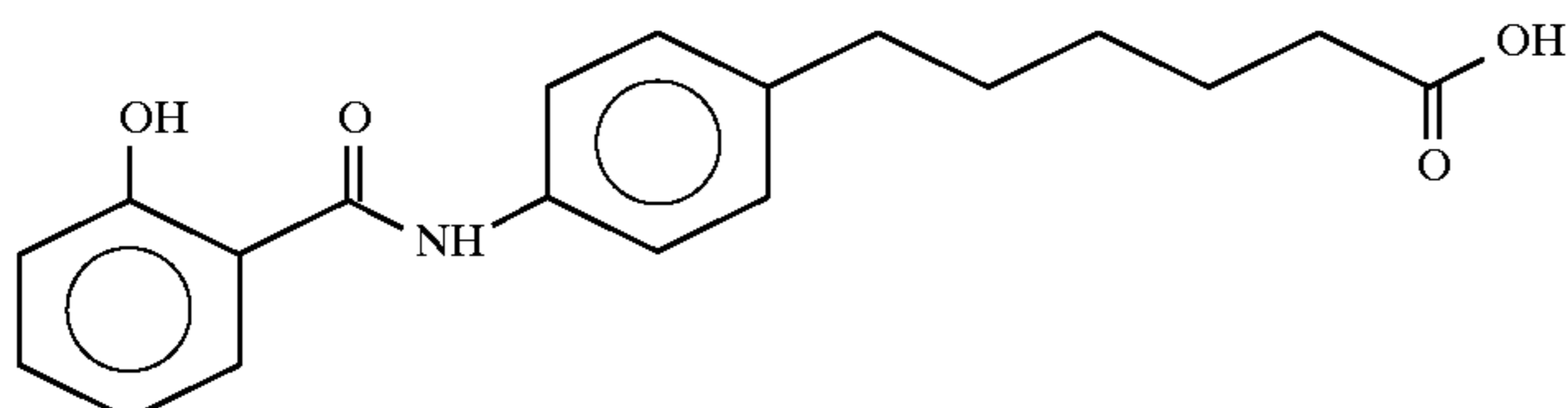
6-(4-(salicyloyl)aminophenyl)hexanoic acid
