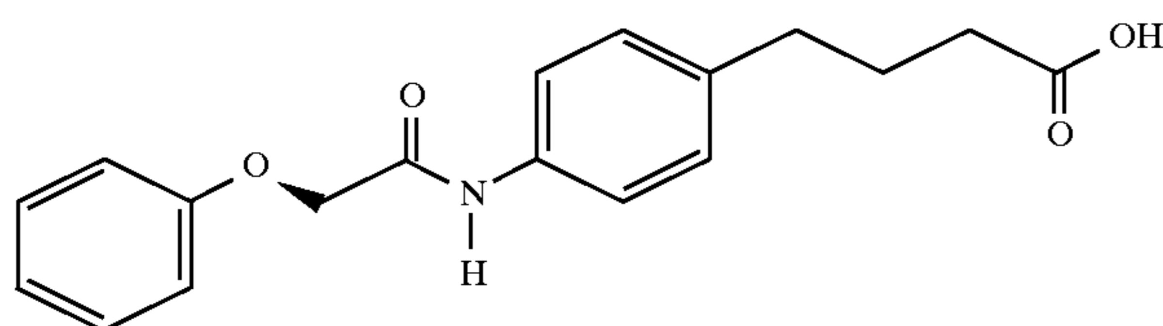
4-(4-(phenoxyacetyl)aminophenyl)butyric acid
