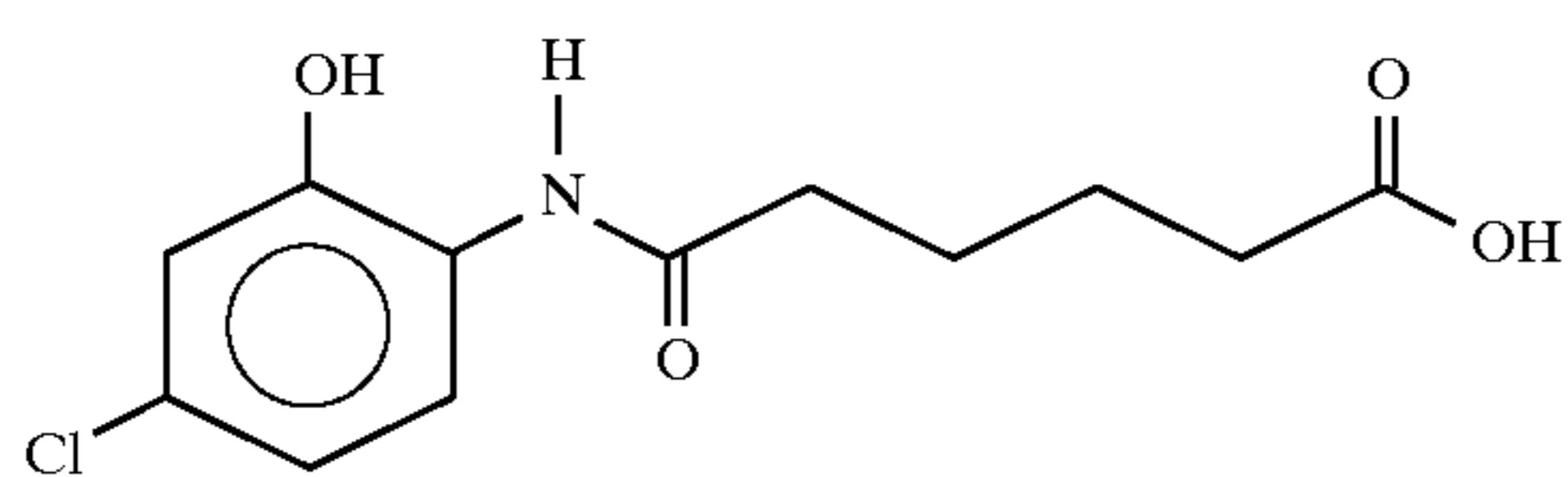
5-(4-chloro-2-hydroxyanilino)valeric acid
