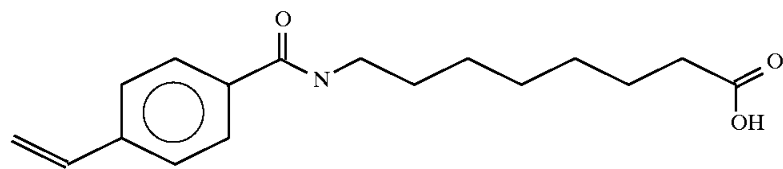
8-(vinylbenzoyl)aminocaprylic acid
