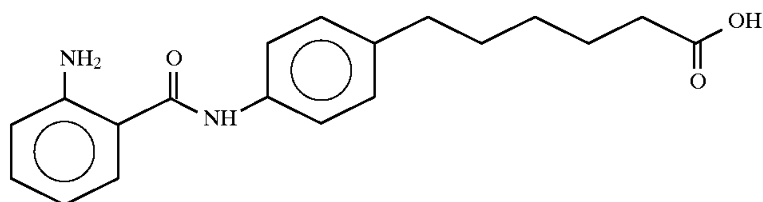
6-(4-(N-(2-aminobenzoyl)aminophenyl)hexanoic acid
