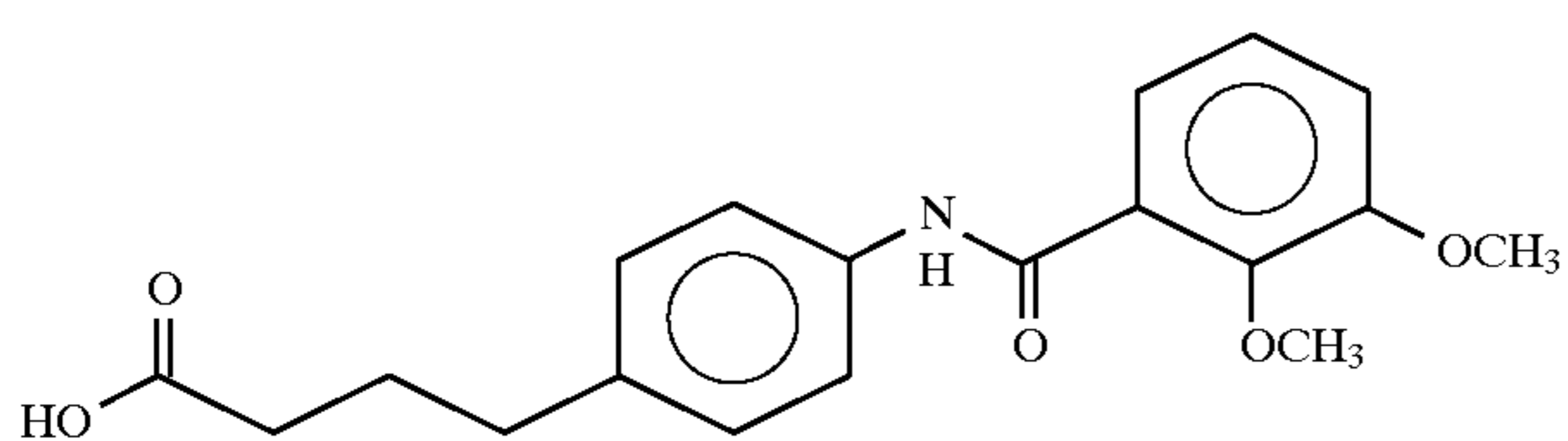
4-(4-(2,3-dimethoxybenzoyl)aminophenyl)butyric acid
