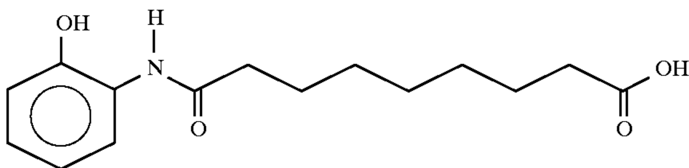
9-(2-hydroxybenzamido)nonanoic acid
