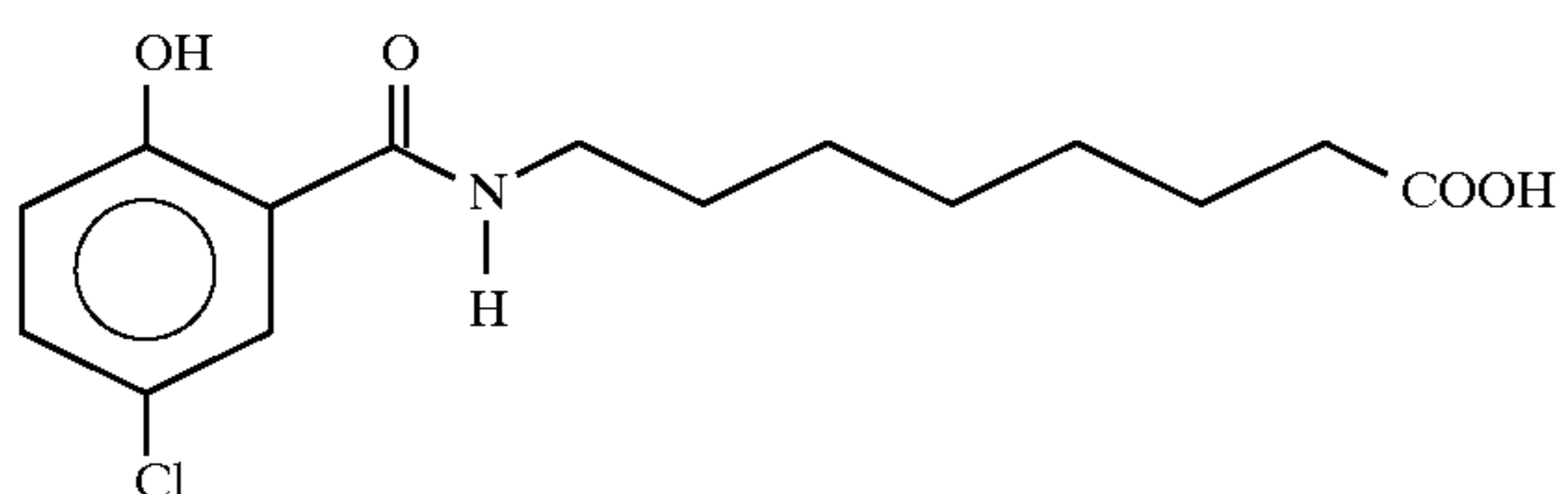
8-(N-(2-hydroxy-5-chlorobenzoyl)aminocaprylic acid
