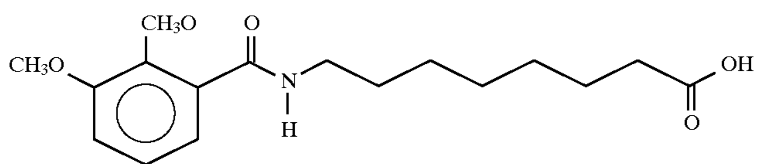
8-(N-2,3-Dimethoxybenzoyl)aminocaprylic acid
