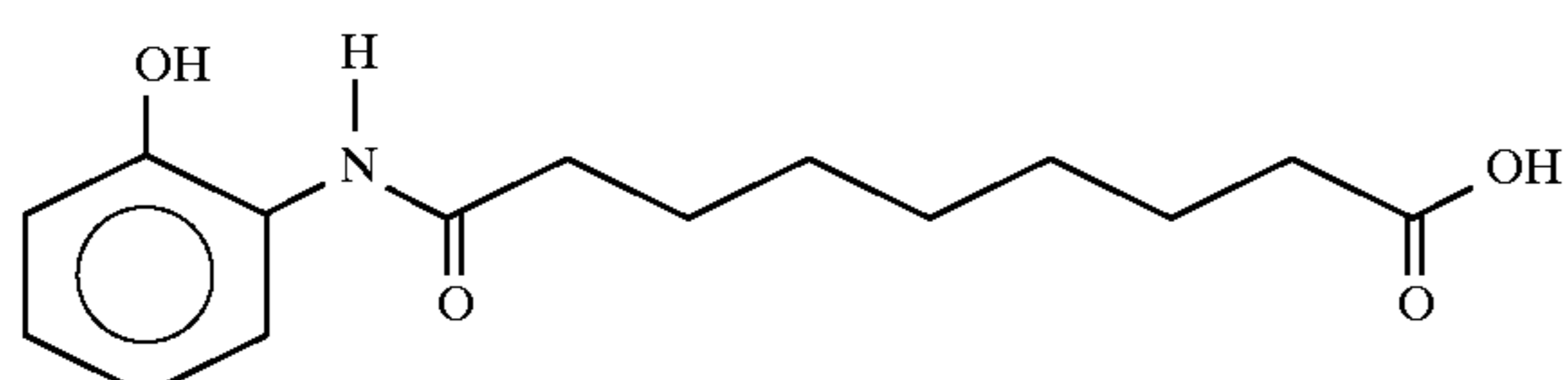
9-(2-hydroxybenzamido)nonanoic acid
