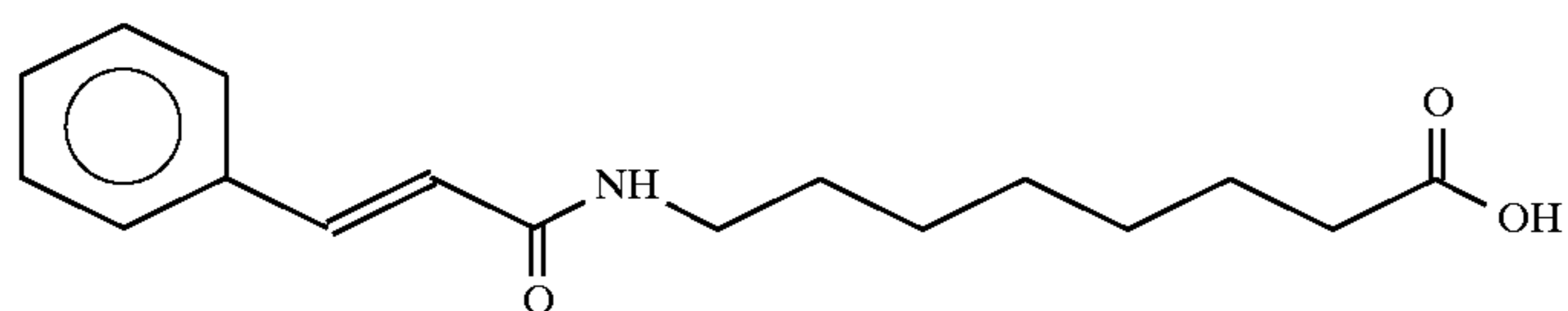
8-cinnamoylaminovaleric acid
