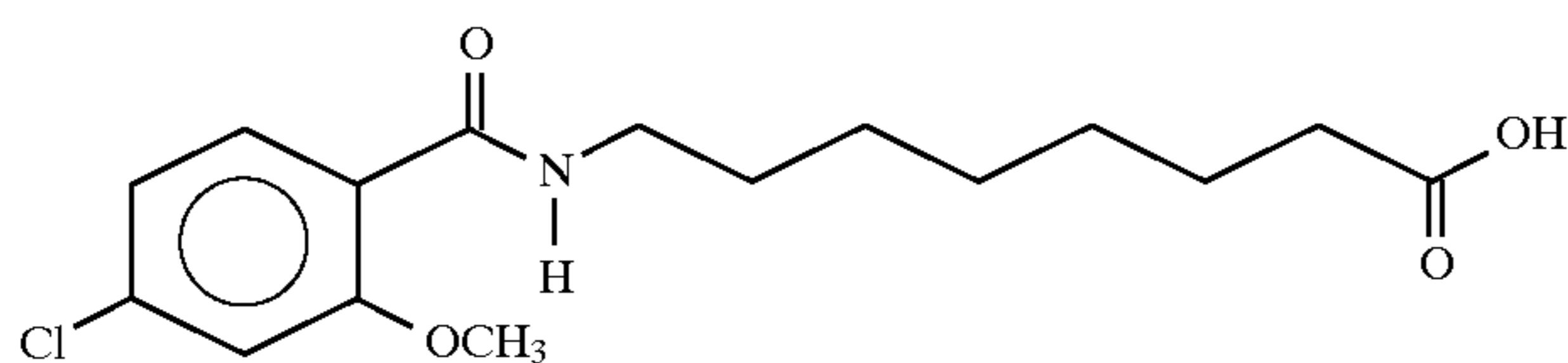
8-(4-chloro-o-anisoyl)aminocaproic acid
