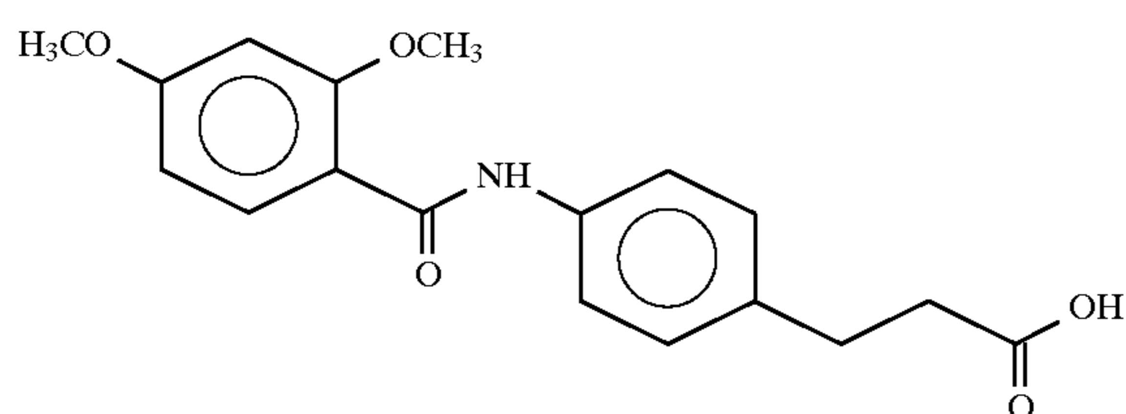
3-[4-(2,4-dimethoxybenzoyl)aminophenyl]propionic acid
