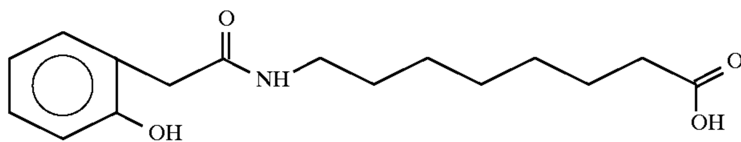
8-(2-hydroxyphenoxy)aminocaproic acid
