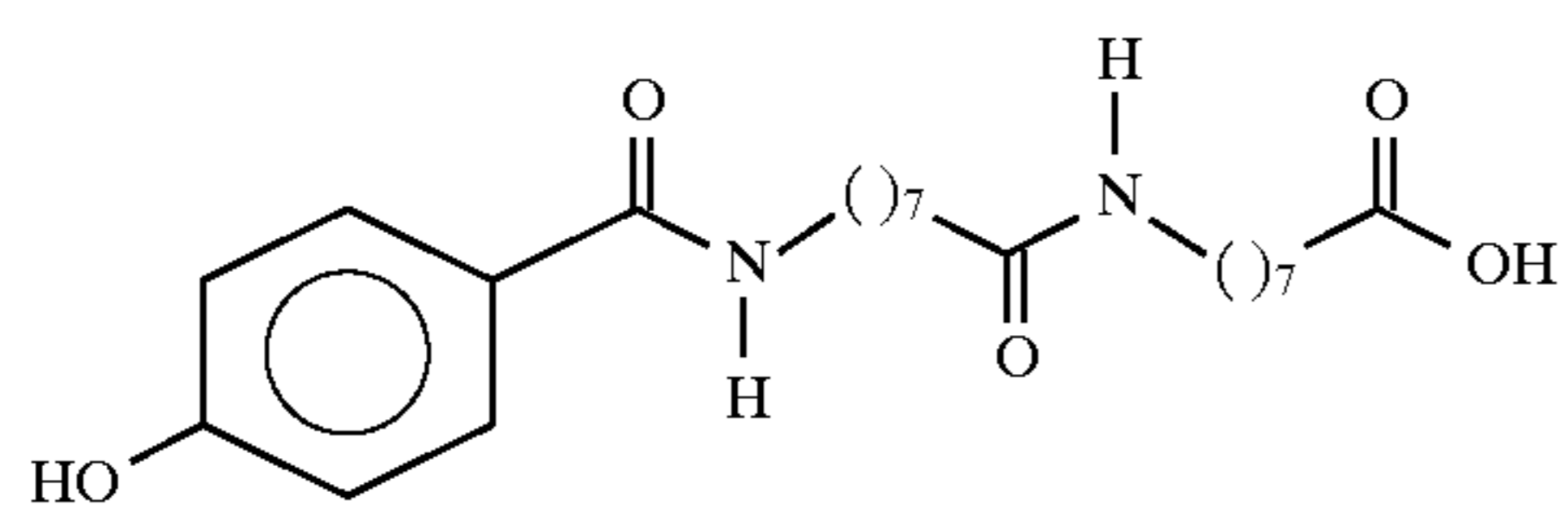
8-(N-4-Hydroxybenzoyl)aminocaprylic acid (dimer)
