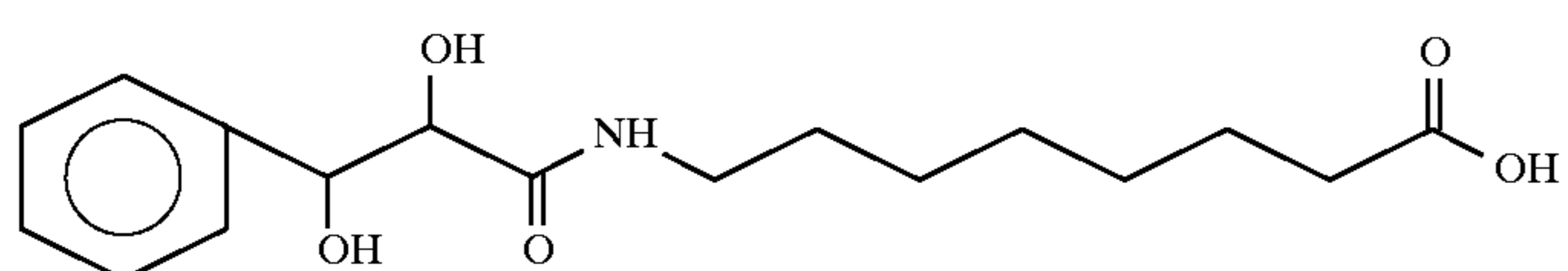
(3-phenyl-2,3-dihydroxypropanoyl)8aminocaproic acid
