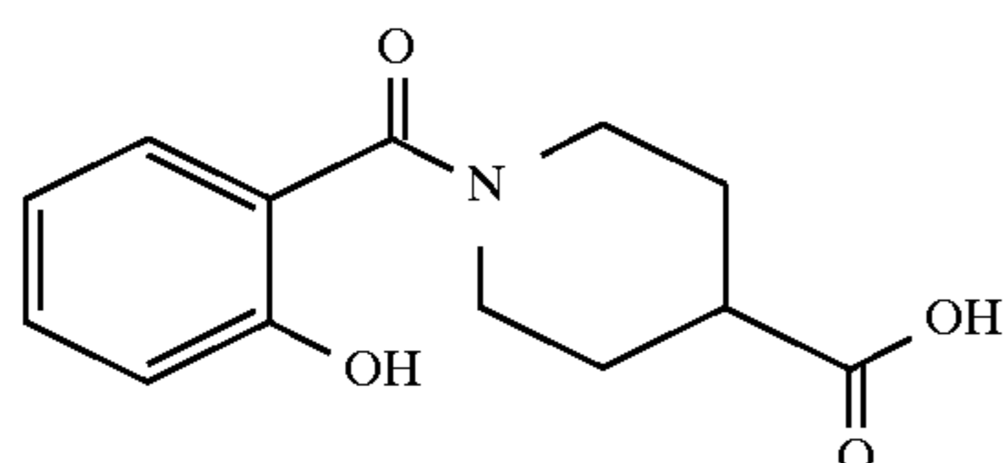
N-(2-hydroxybenzoyl)isonipecotic acid
