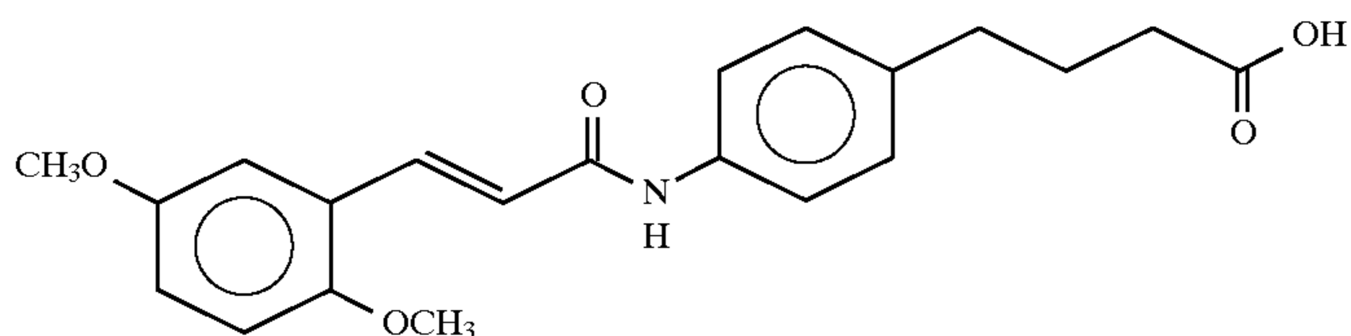
4-(4-(2,5-dimethoxycinnamoyl)aminophenyl)butyric acid
