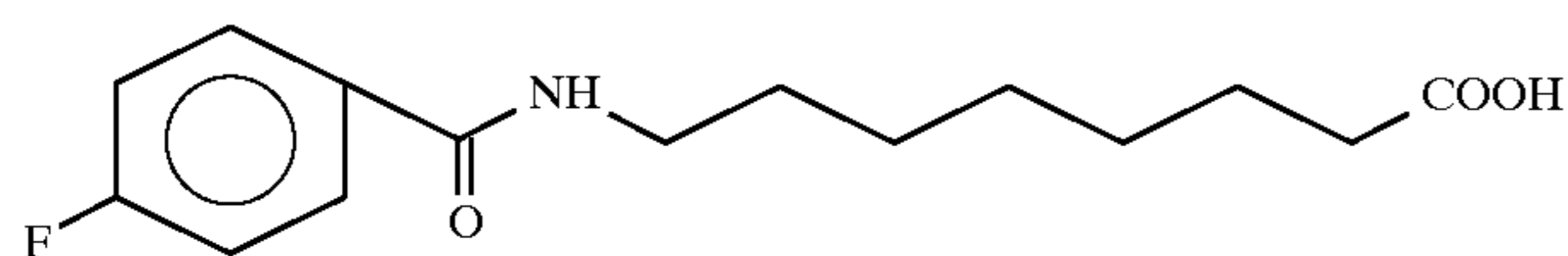
8-[N-(4-fluorobenzoyl)]aminocaprylic acid
