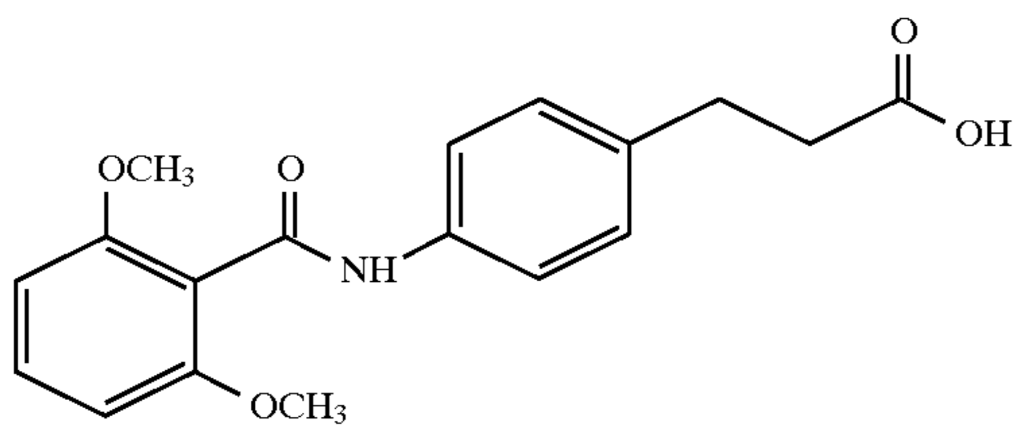
3-(4-(2,6-dimethoxybenzoyl)aminophenyl)propionic acid
