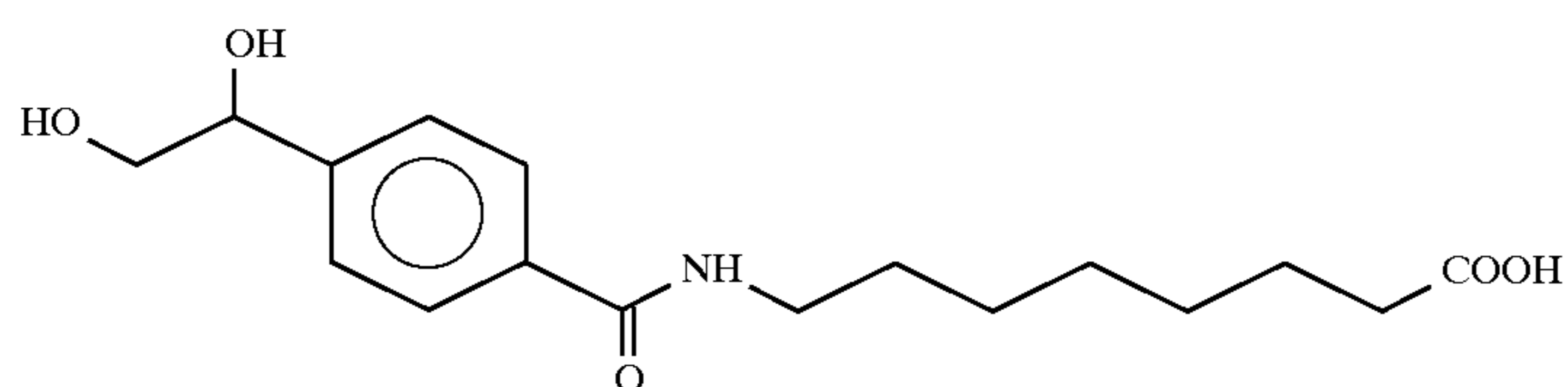
8-(4-(1,2-dihydroxyethyl)benzoyl)aminocaprylic acid
