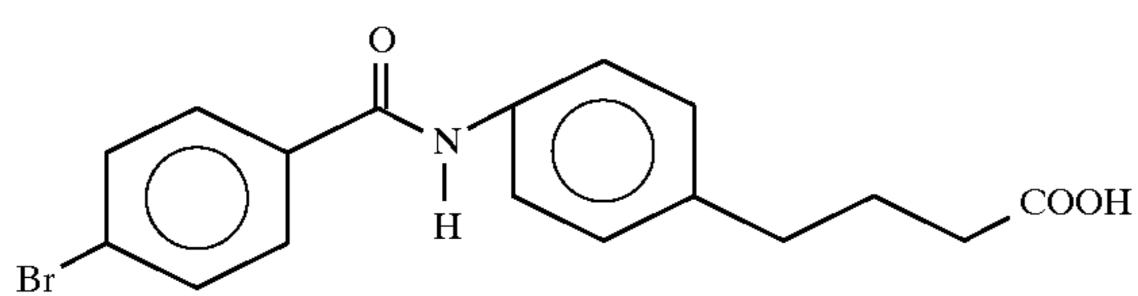
4-{4-[N-(4-bromobenzoyl)aminophenyl]}butyric acid
