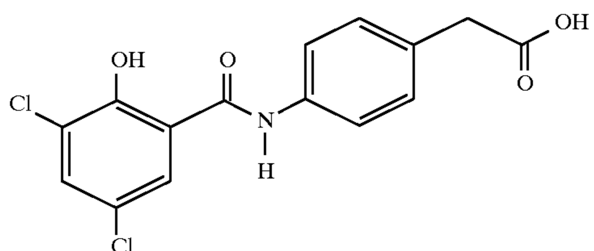
4-[N-(3,5-dichloro-2-hydroxybenzoyl)aminophenyl]acetic acid
