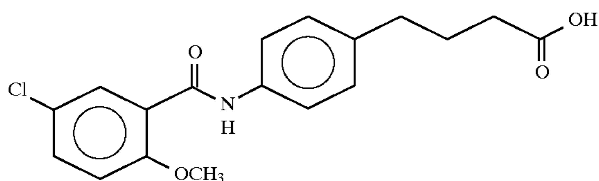
4-(4-(5-chloro-o-anisoyl)aminophenyl)butyric acid
