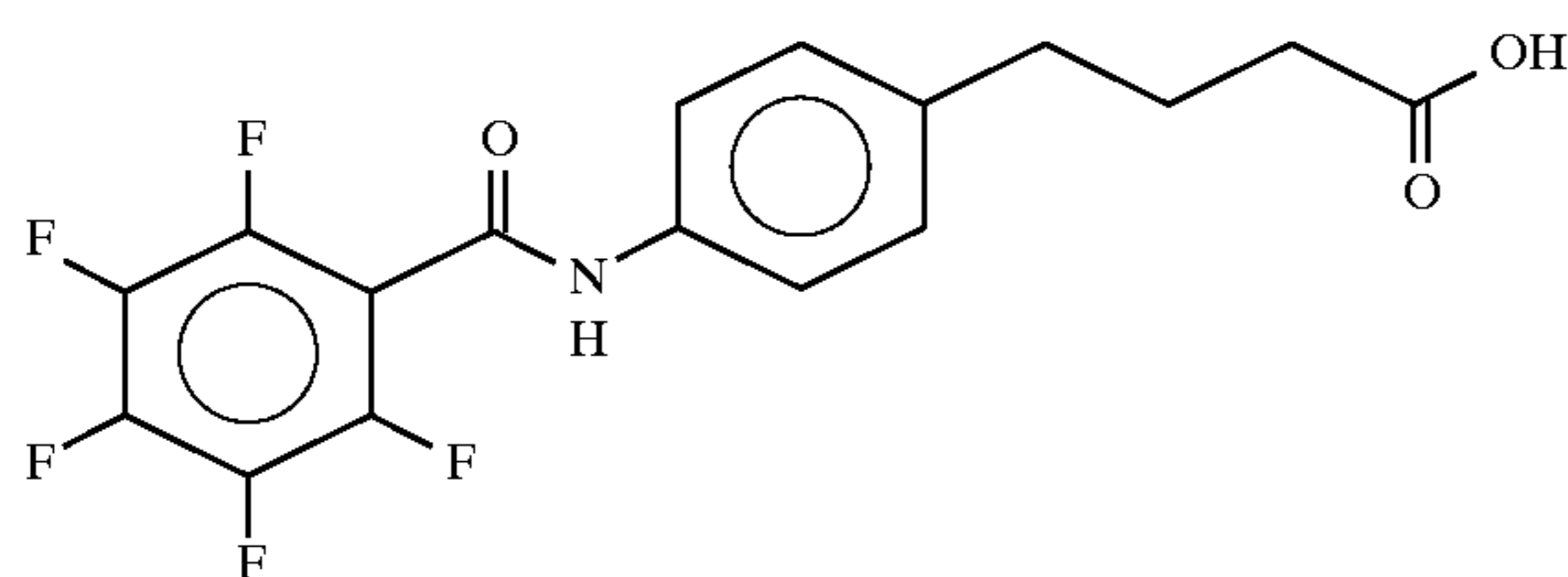
4-(4-(pentafluorobenzoyl)aminophenyl)butyric acid
