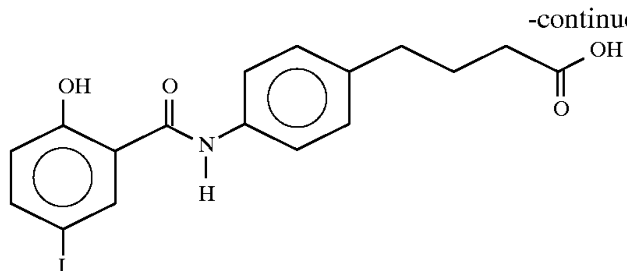
4-[N-(2-hydroxy-5-iodobenzoyl)]aminophenyl}butyric acid
