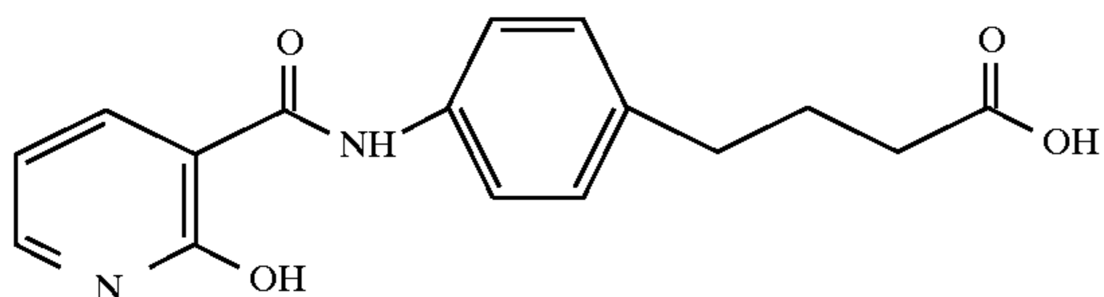
4-(4-(2-hydroxynicotinoyl)aminophenyl)butyric acid
