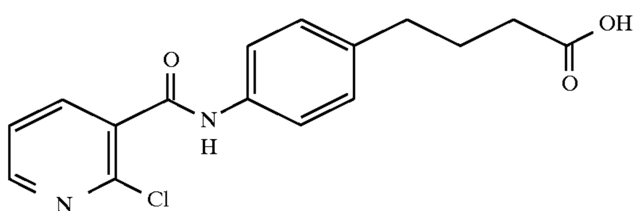
4-(4-(2-chloronicotinoyl)aminophenyl)butyric acid
