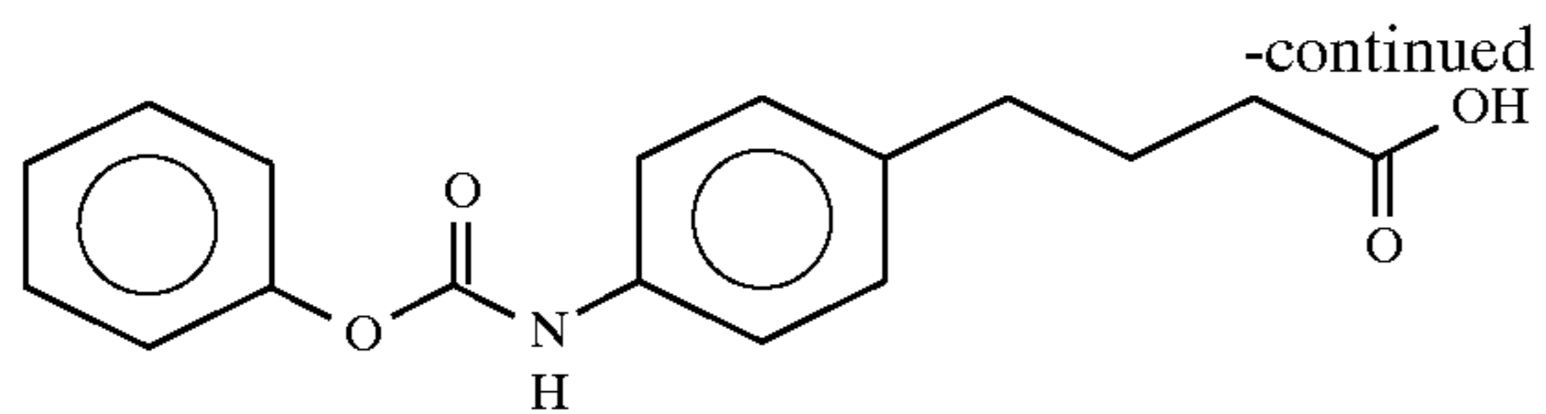
4-(4-phenyloxycarbonylamino)phenylbutyric acid
