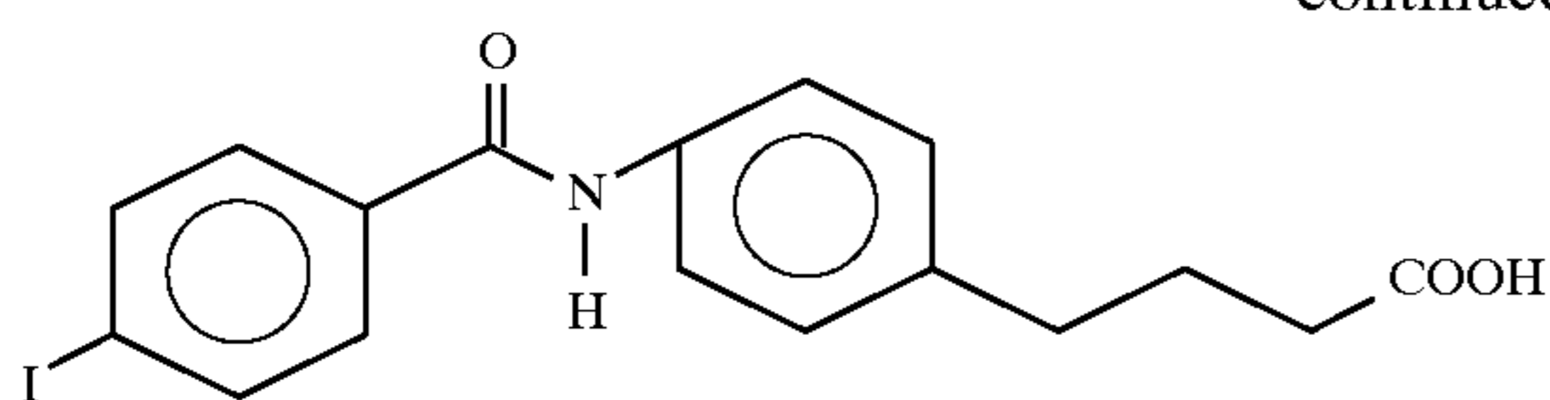
4-{4-[N-(4-iodobenzoyl)]aminophenyl} butyric acid
