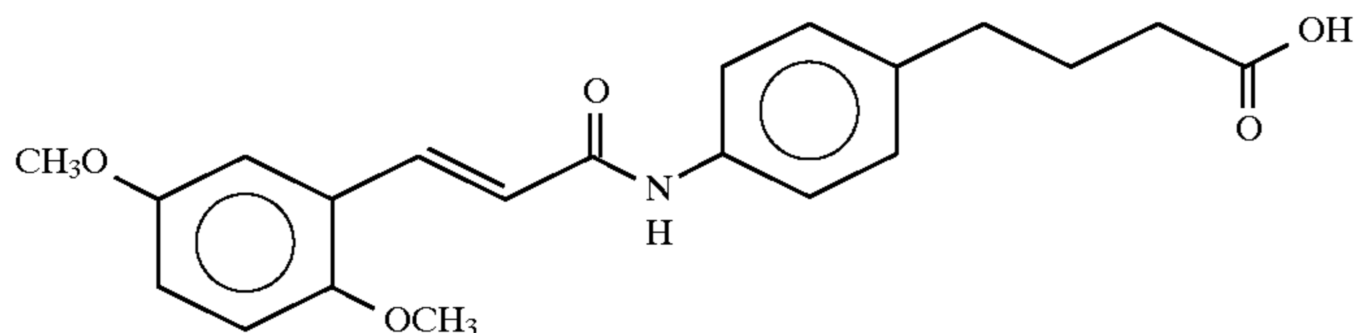
4-(4-(2,5-dimethoxycinnamoyl)aminophenyl)butyric acid
