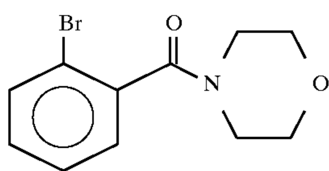
N-(2-bromobenzoyl)morpholine
