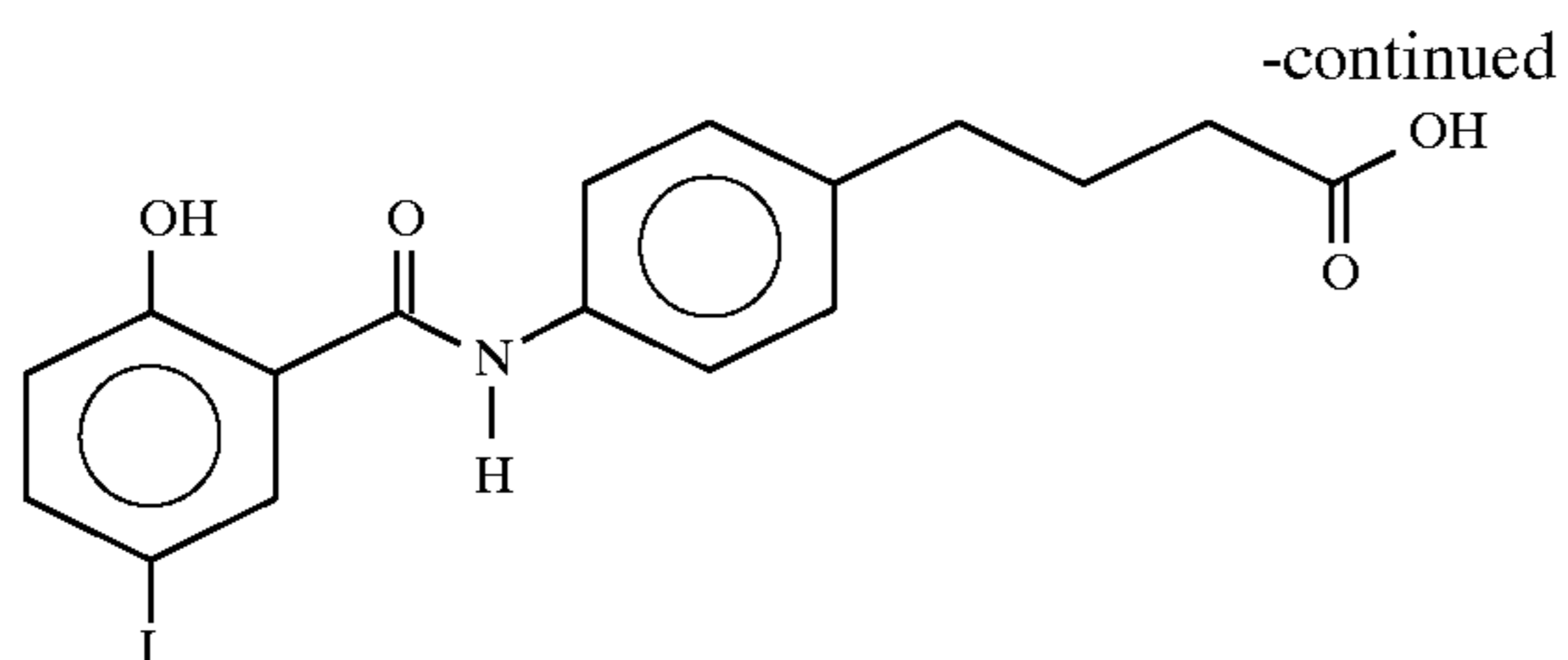
4-[N-(2-hydroxy-5-iodobenzoyl)]aminophenyl}butyric acid
