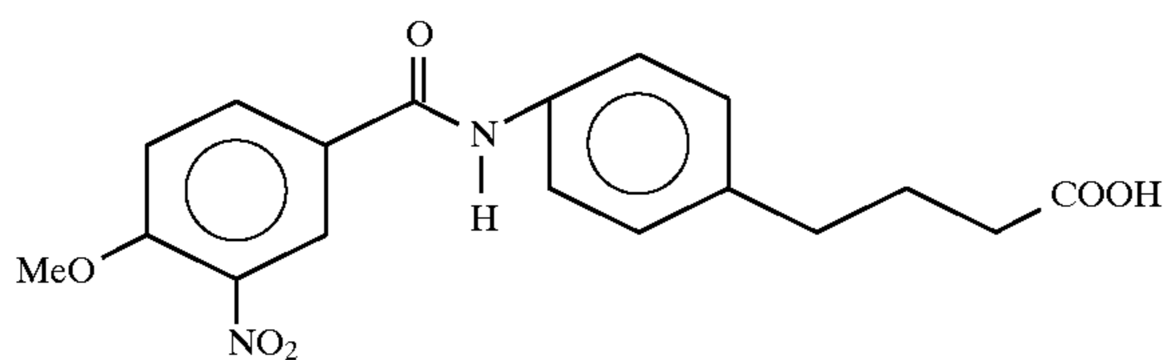
4-[4-N-(4-methoxy-3-nitrobenzoyl)aminophenyl]butyric acid
