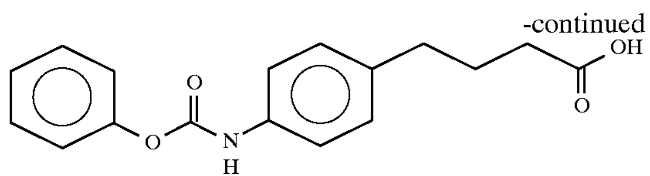
4-(4-phenyloxycarbonylamino)phenylbutyric acid
