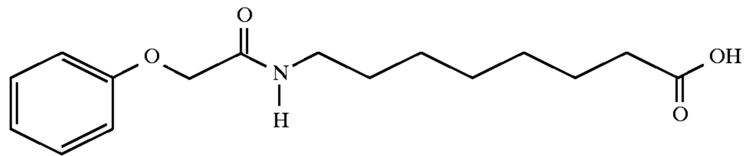
8-(Phenoxyacetyl)caprylic acid
