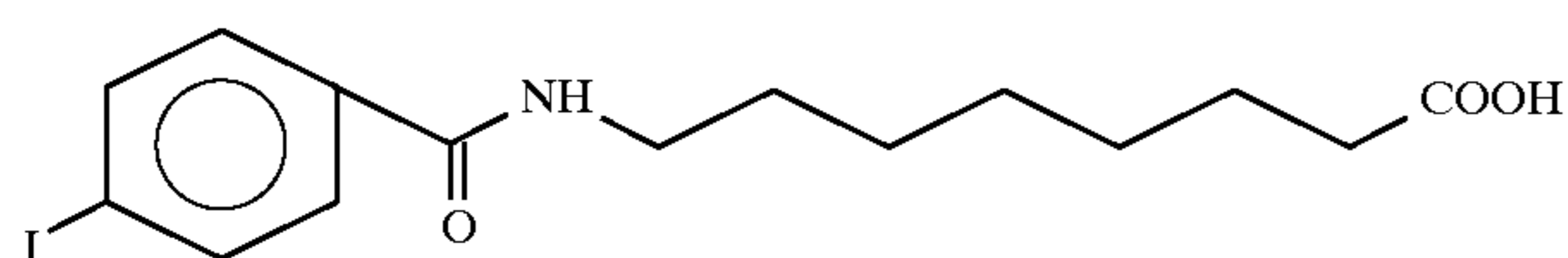
8-[N-(4-iodobenzoyl)]aminocaprylic acid
