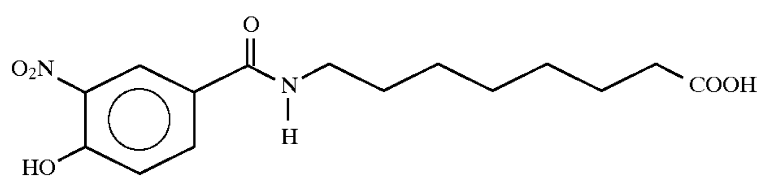
8-N-(4-hydroxy-3-nitrobenzoyl)caprylic acid
