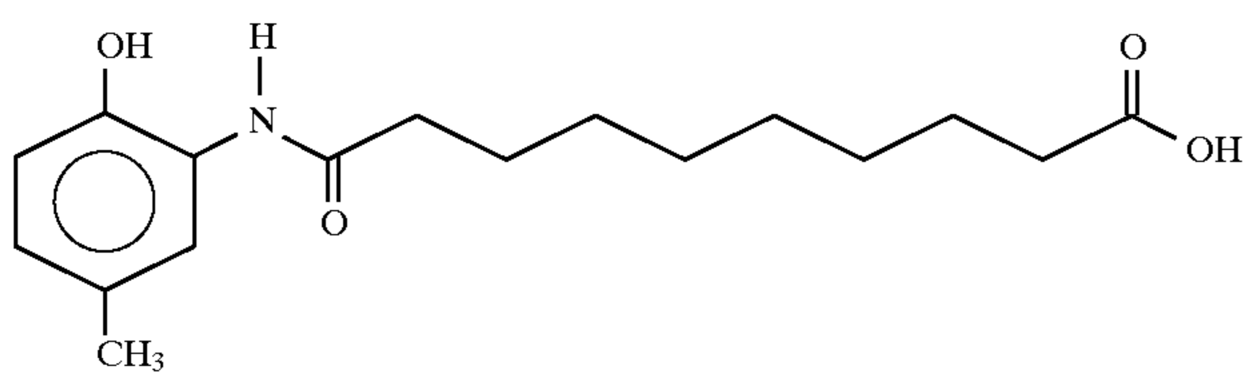
9-(2-hydroxy-5-methylanilino)nonanoic acid
