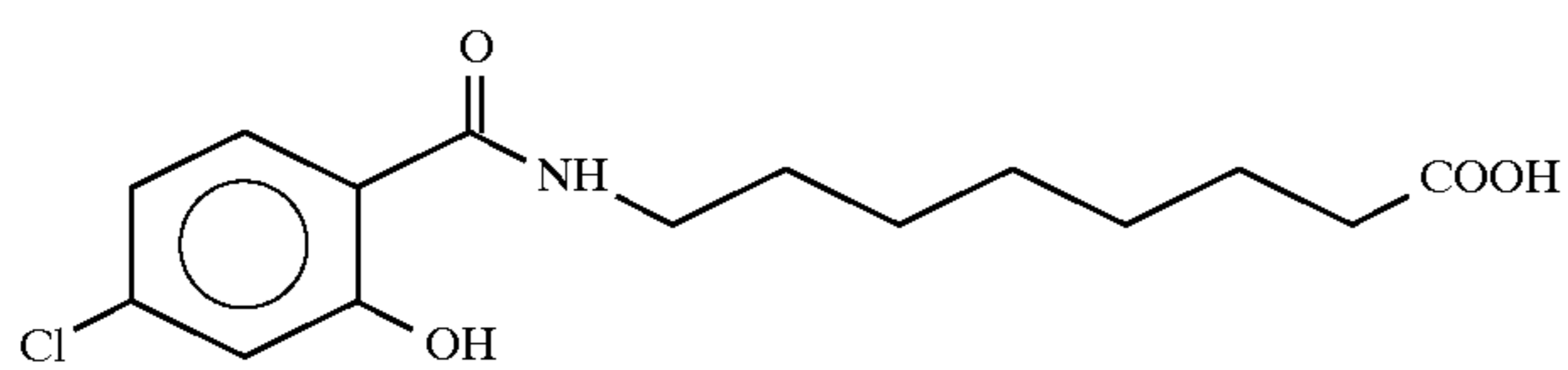
8-(2-hydroxy-4-chlorobenzoyl)aminocaprylic acid
