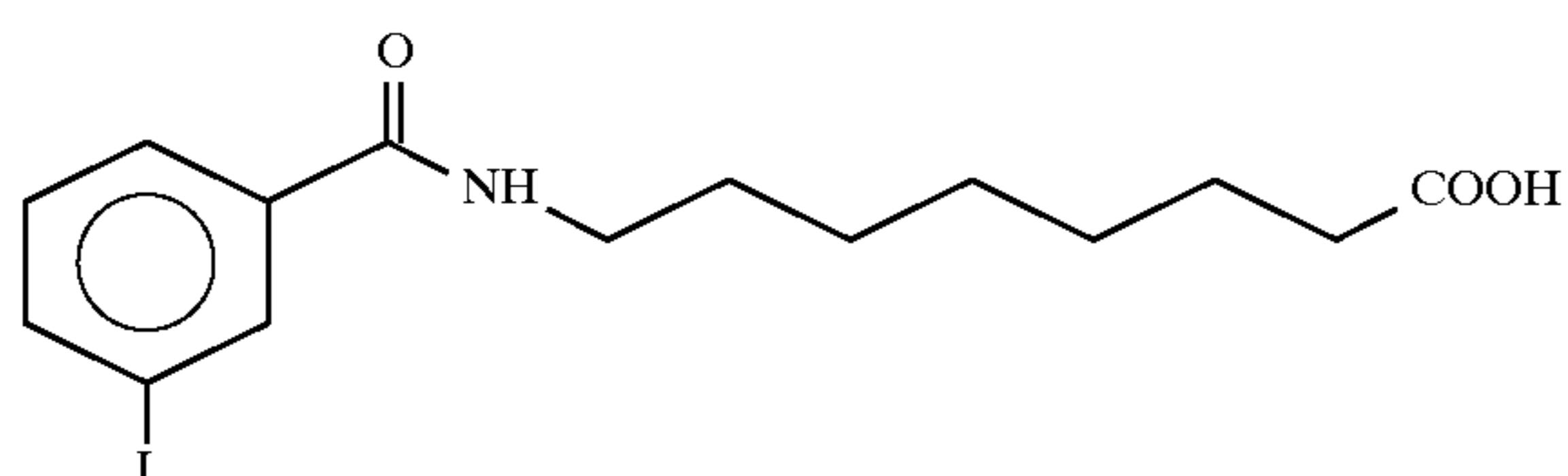
8-N-(3-iodobenzoyl)aminocaprylic acid
