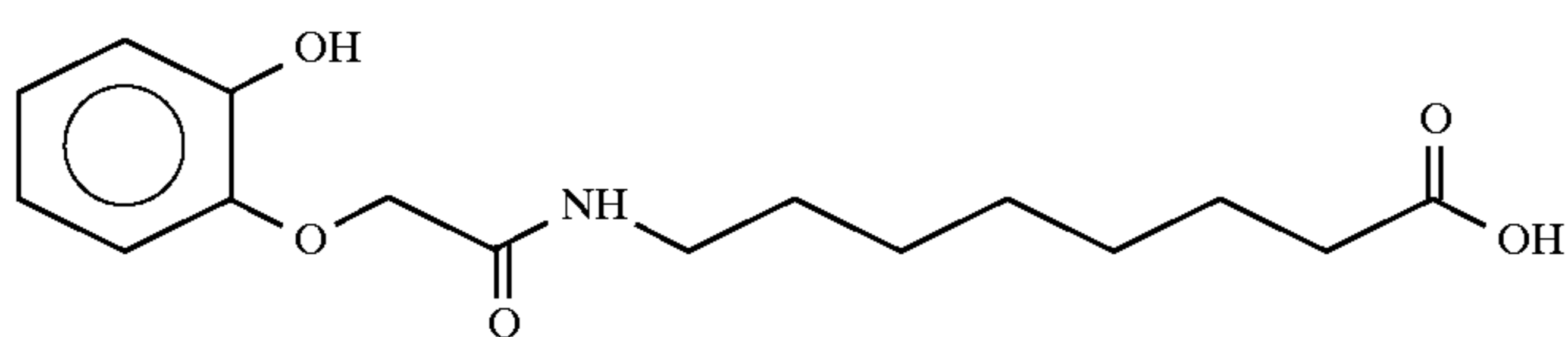
7-(2-hydroxyphenoxyacetyl)aminocaproic acid
