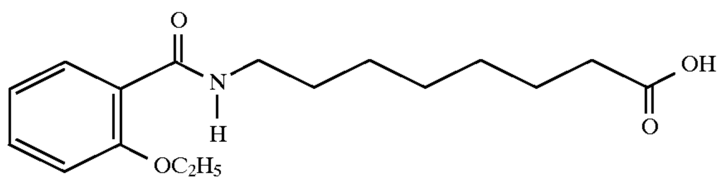
8-(2-ethoxybenzoyl)aminocaprylic acid
