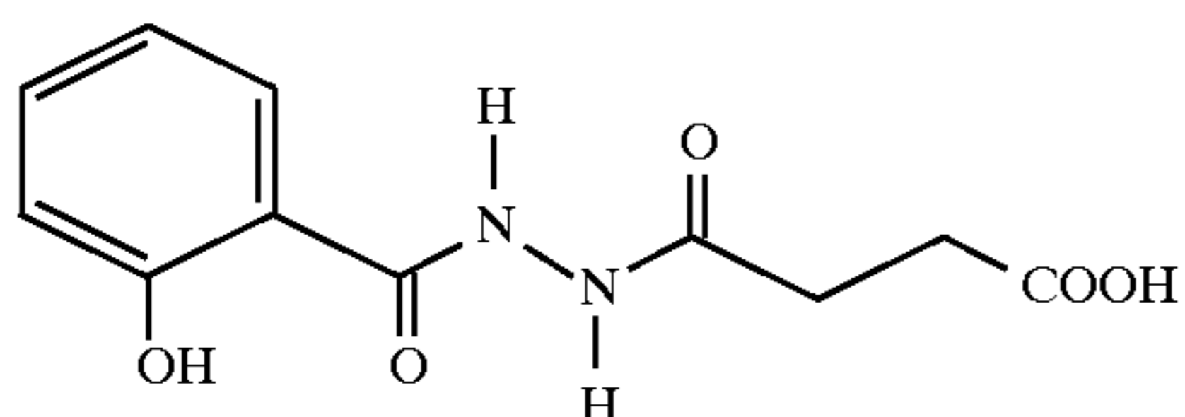
1-salicyloyl-2-succinyl hydrazide
