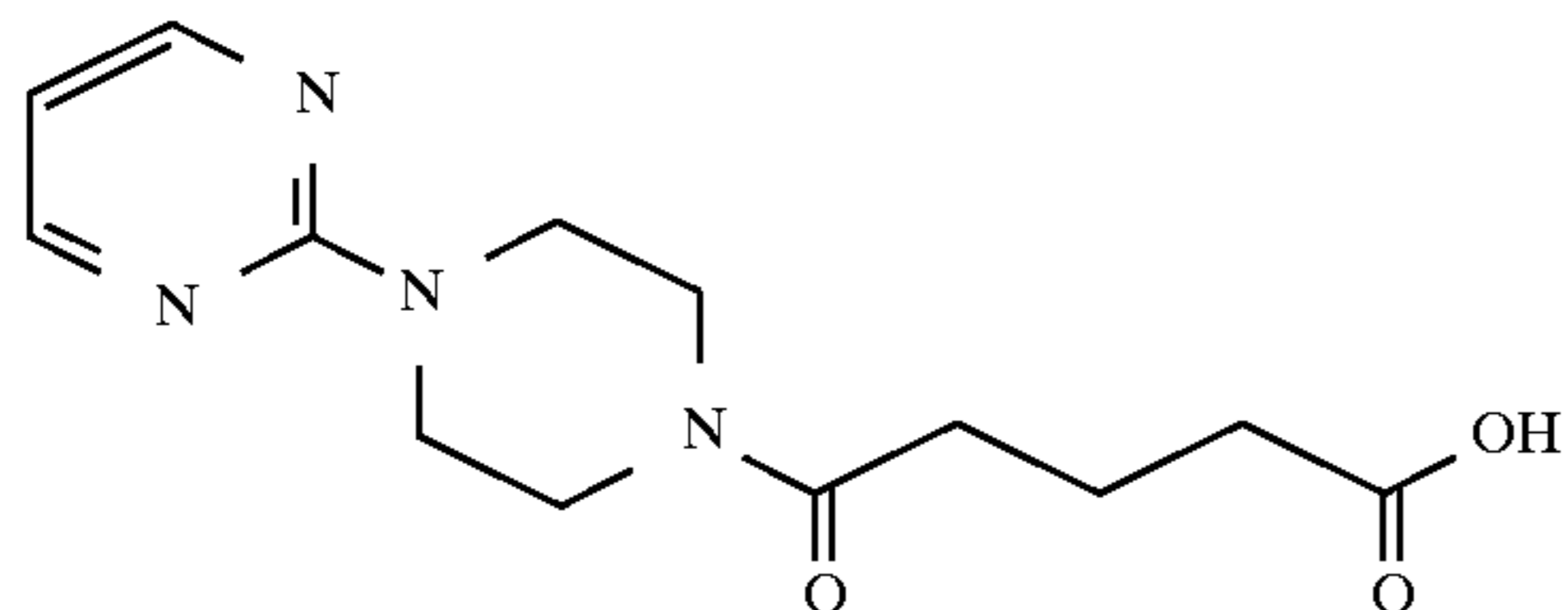
4-(1-(2-pyrimidyl)piperazinoyl)butyric acid
