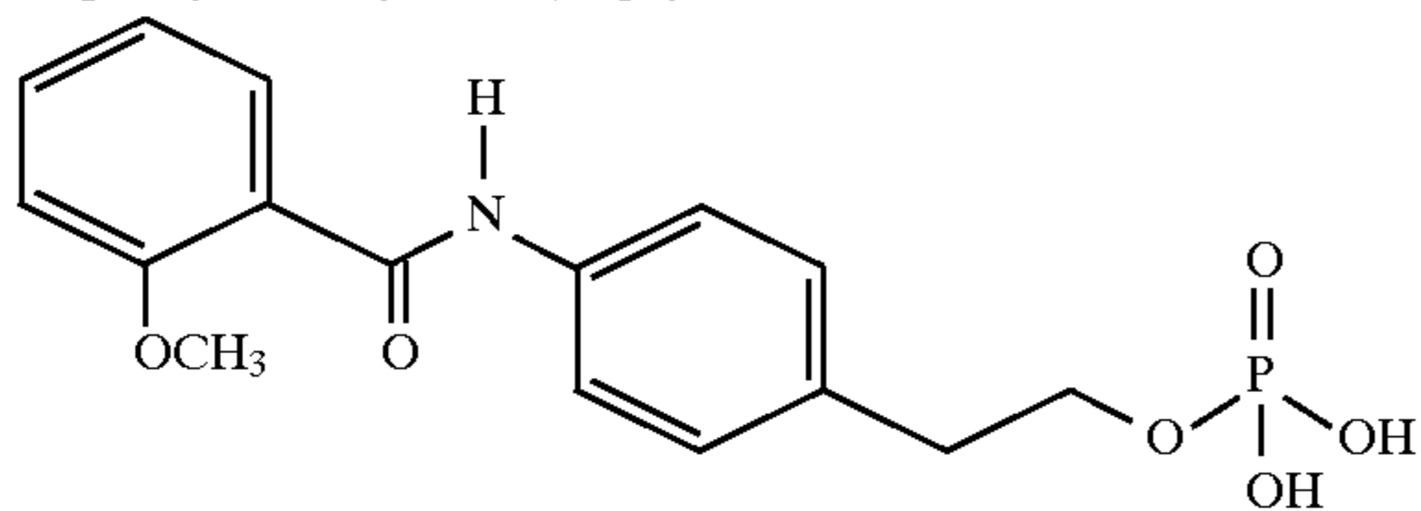
2-[4-(2-Methoxybenzoylamino)phenyl]ethyl H 2 PO 4
