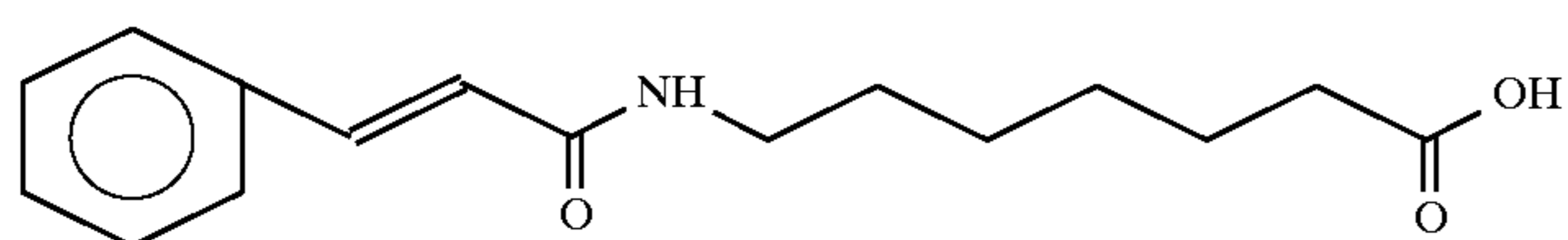
7-cinnamoylaminoheptanoic acid
