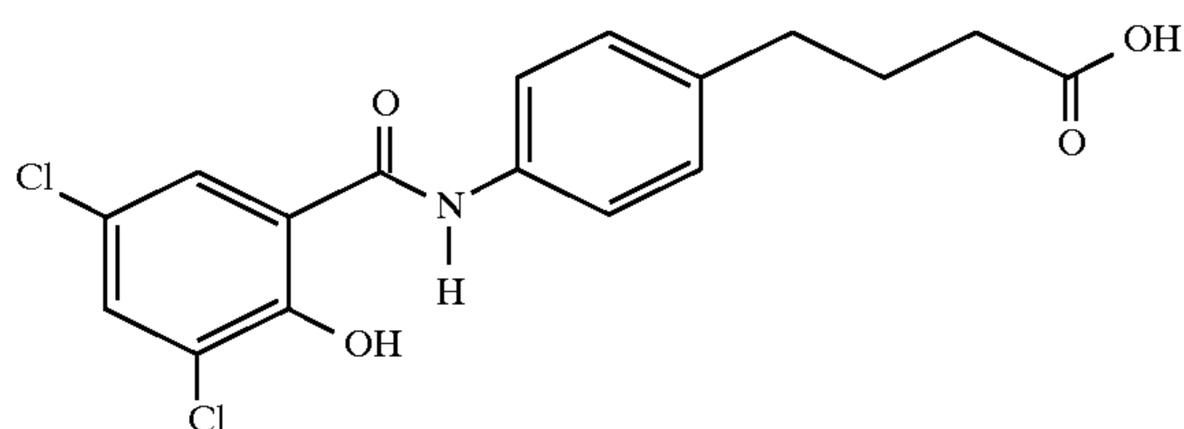
N-[3,5-dichloro-2-hydroxybenzoyl-4(4-aminophenyl)]butyric acid
