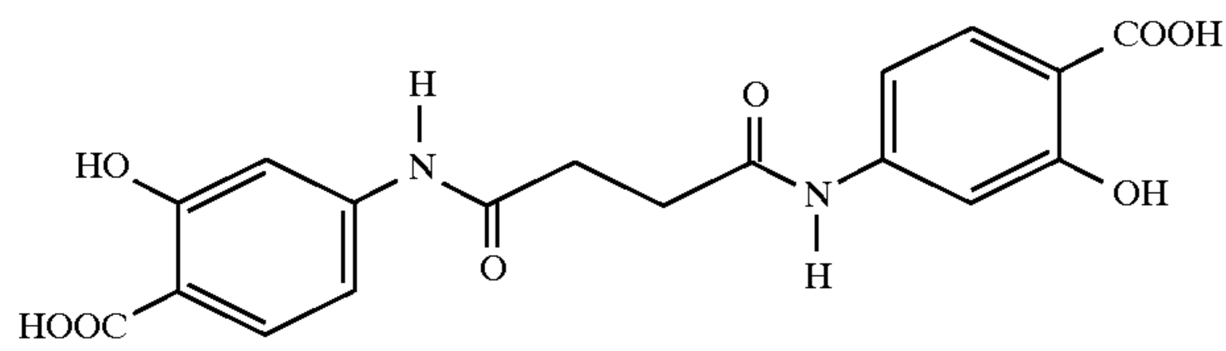
Succinyl-4-aminosalicylic acid
