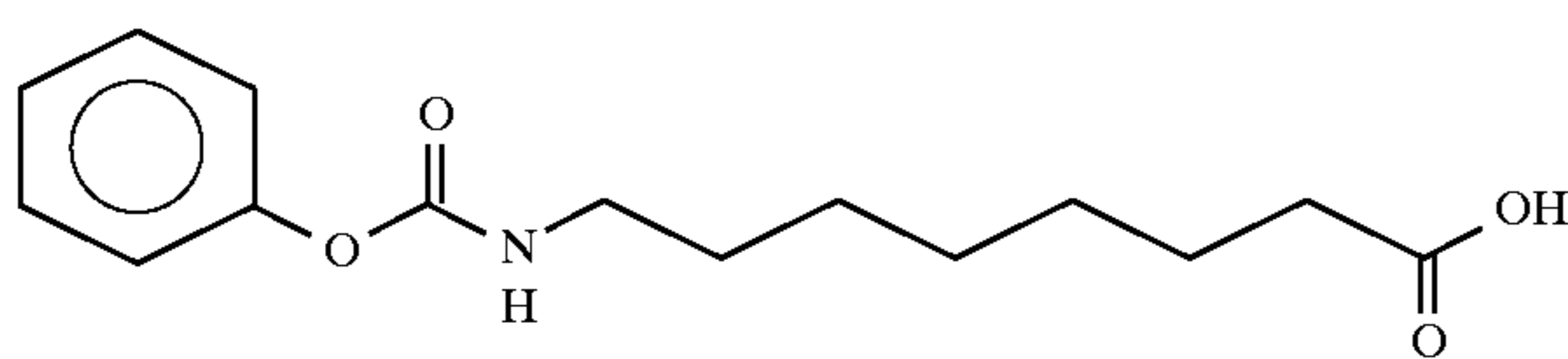
8-(phenylcarbonylamino)caprylic acid
