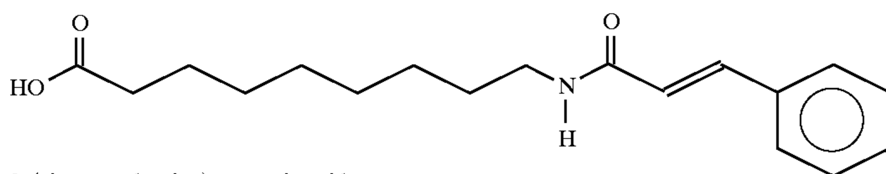
9-(cinnamoylamino)nonanoic acid
