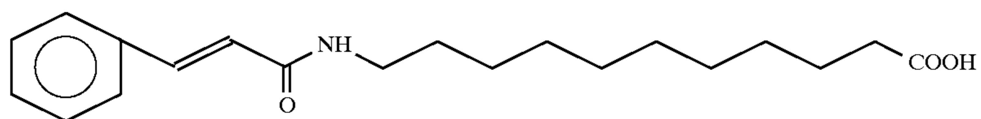
11-cinnamoylaminoundecanoic acid
