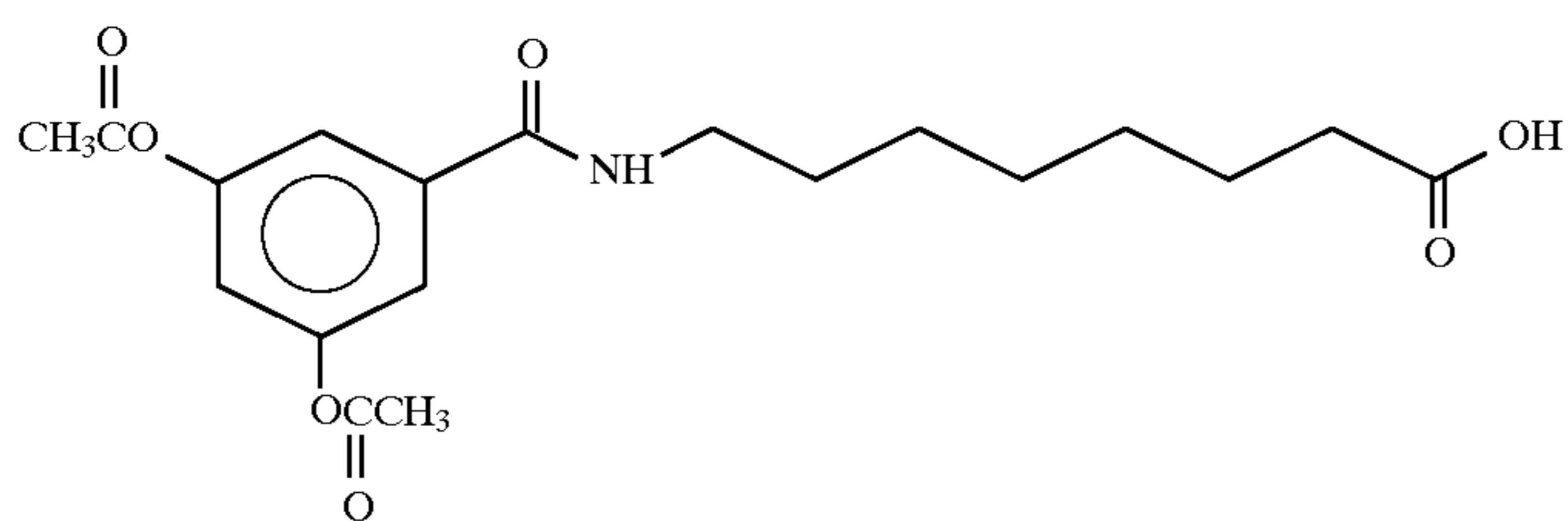
8-(N-3,5-Diacetyloxybenzoyl)aminocaprylic acid
