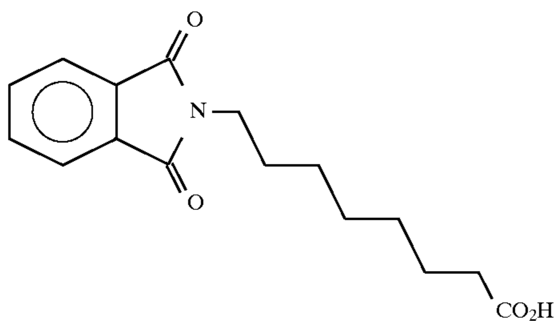
8-(phthalimido)caprylic acid
