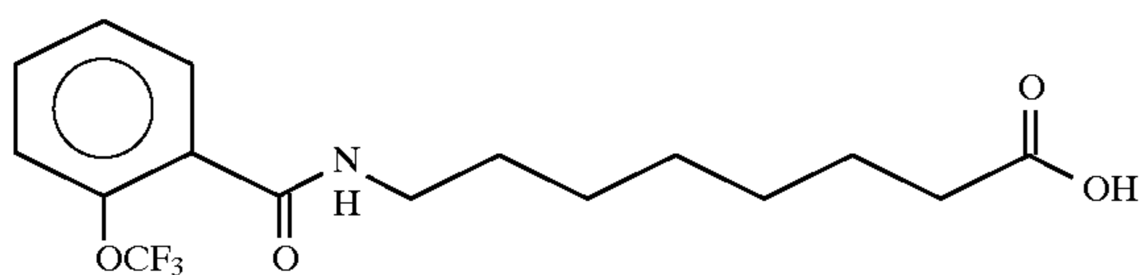
8-(2-(trifluoromethoxy)benzoyl)aminocaprylic acid
