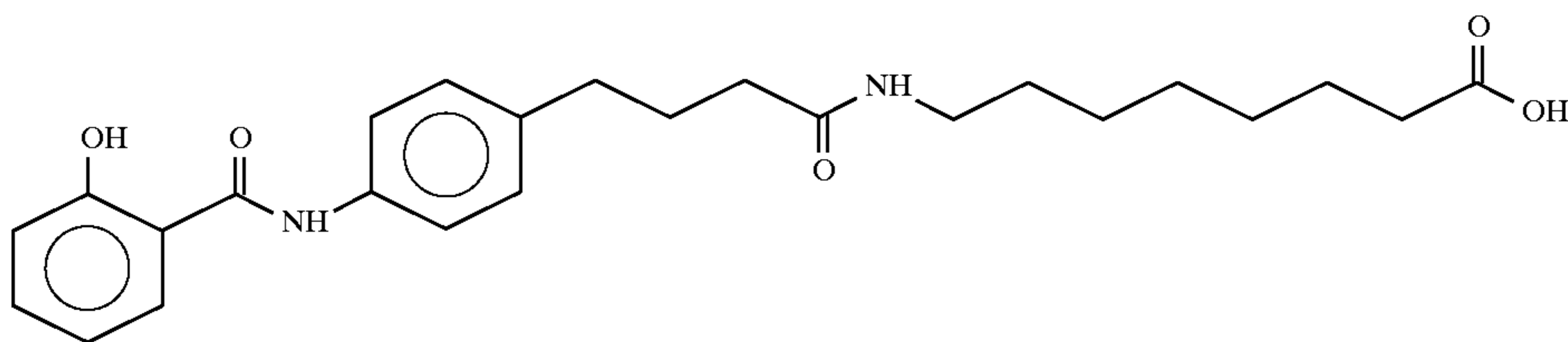
8-(4-(N-Salicyloyl-4aminophenyl)butyric)aminocaprylic acid
