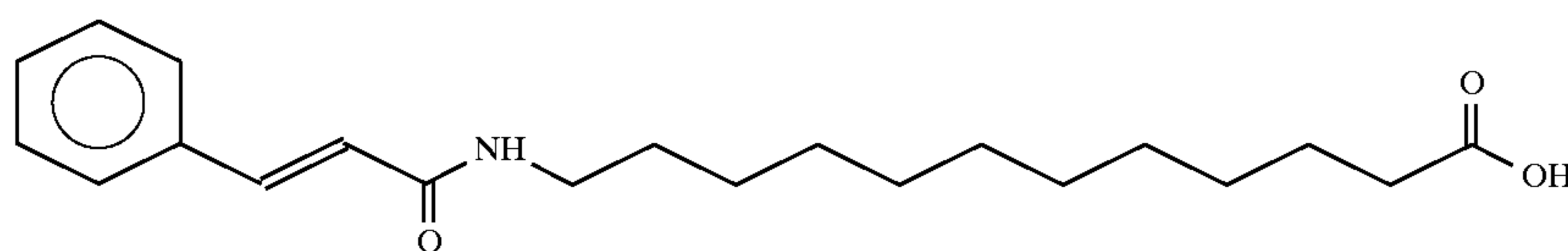
12-cinnamoyldodecanoic acid
