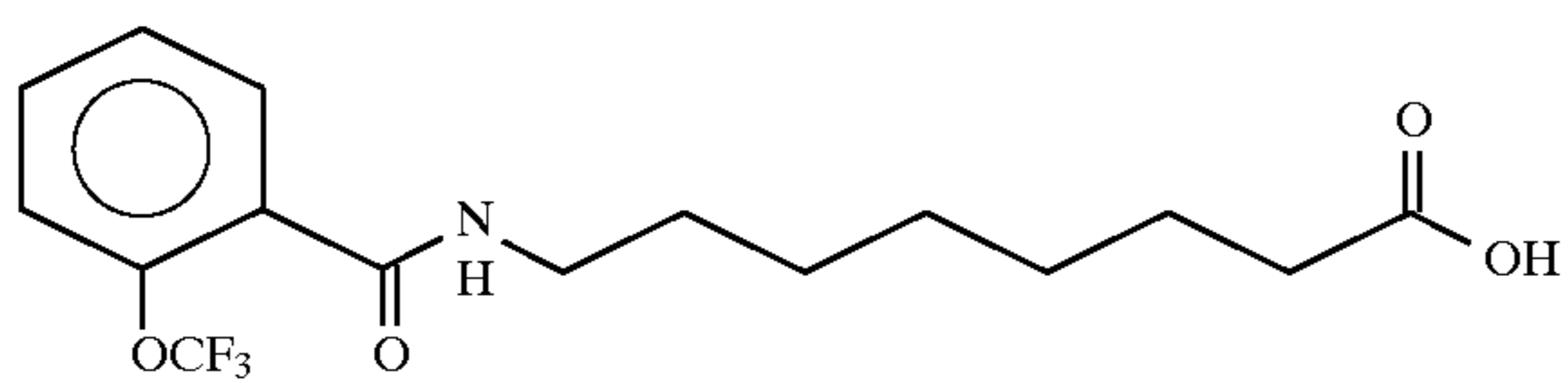
8-(2-(trifluoromethoxy)benzoyl)aminocaprylic acid
