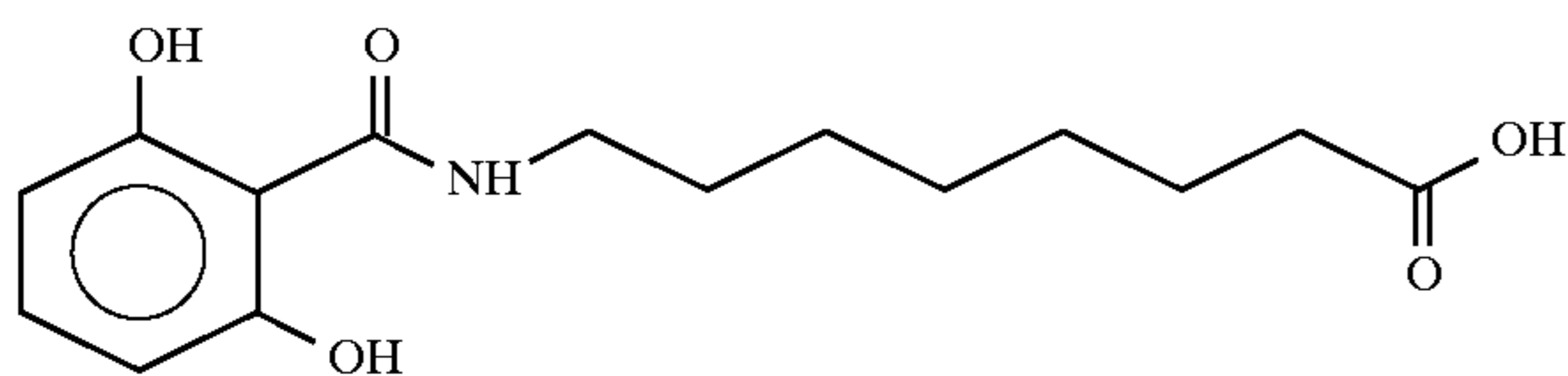
8-(N-2,6-Dihydroxybenzoyl)aminocaprylic acid
