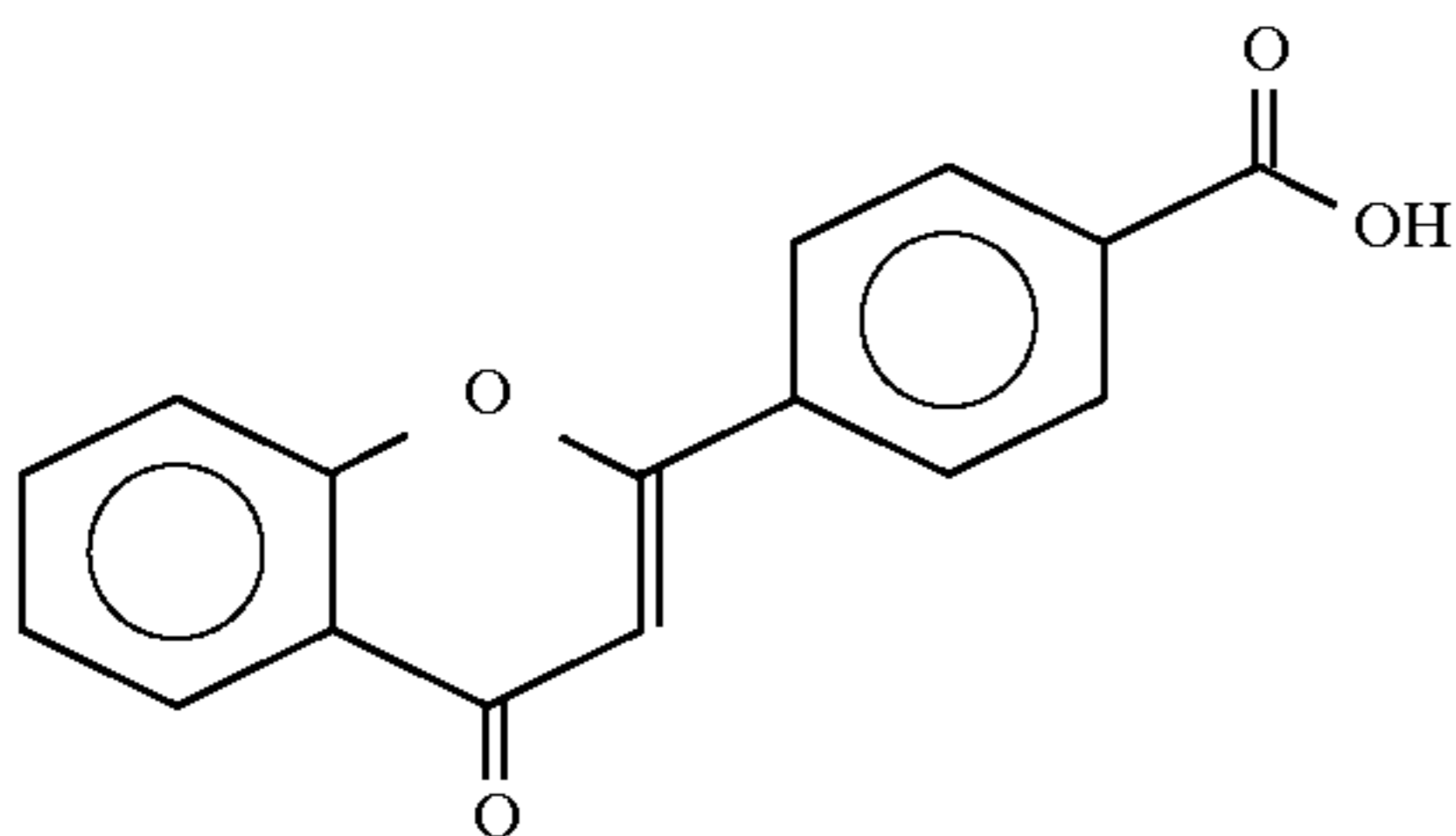
4'-flavonic acid
