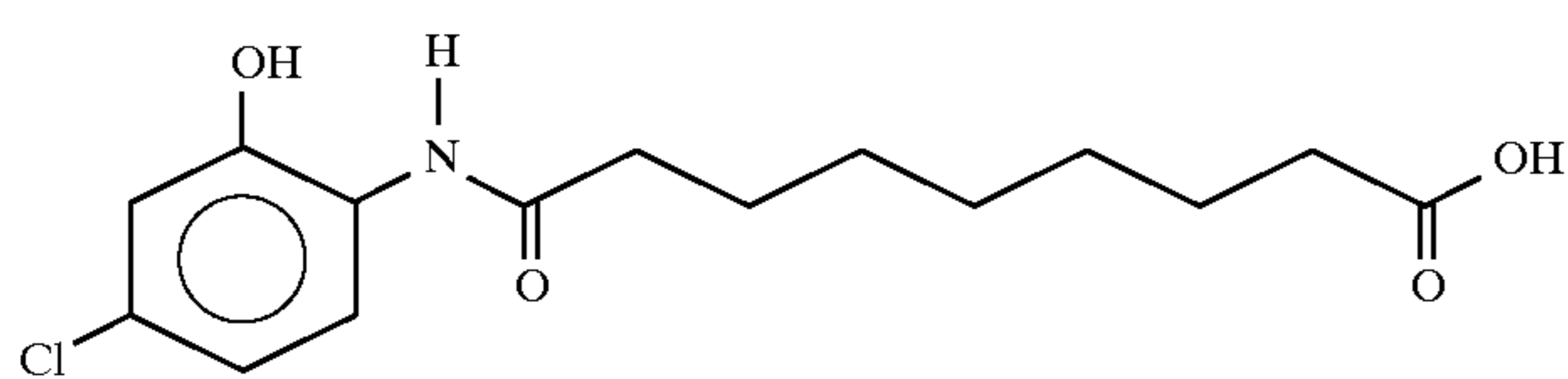
8-(2-hydroxy-5-chloroanilino)octanoic acid
