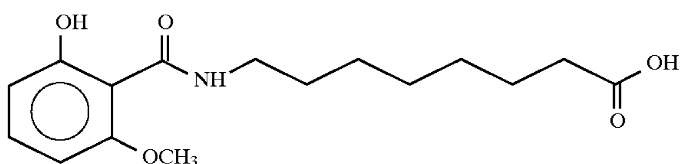
8-(N-2-Hydroxy-6-methoxybenzoyl)aminocaproic acid
