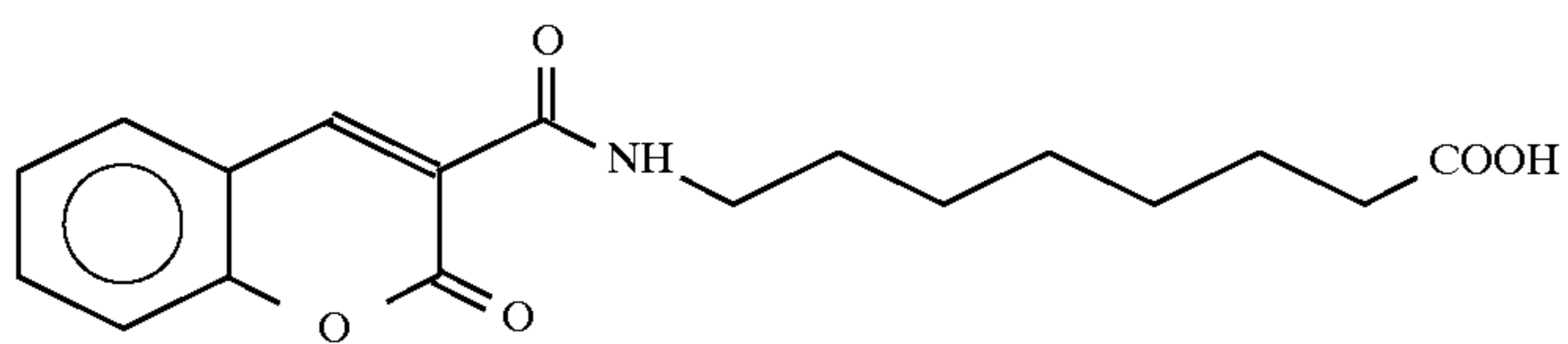
8-[N-(3-coumarincarboxyl)]aminocaprylic acid
