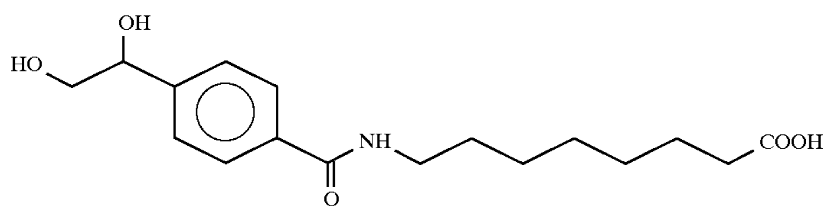
8-(4-(1,2-dihydroxyethyl)benzoyl)aminocaprylic acid
