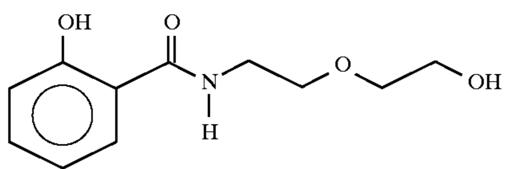
2-[N-(2-hydroxybenzoylamino)ethoxy]ethanol
