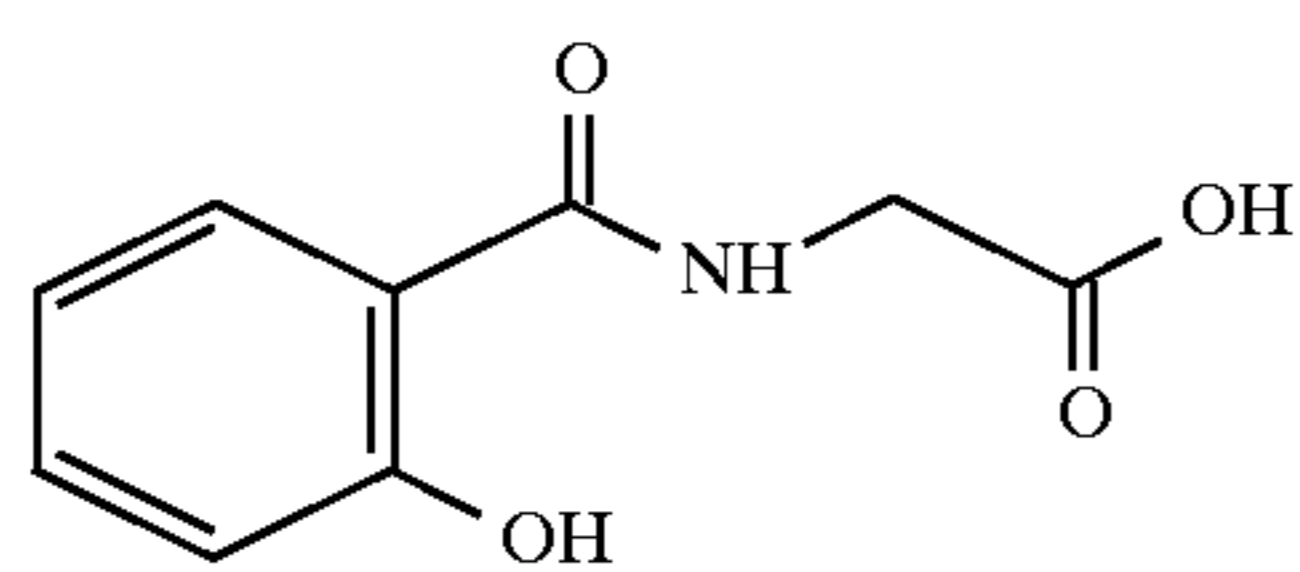
salicyloylglycine
