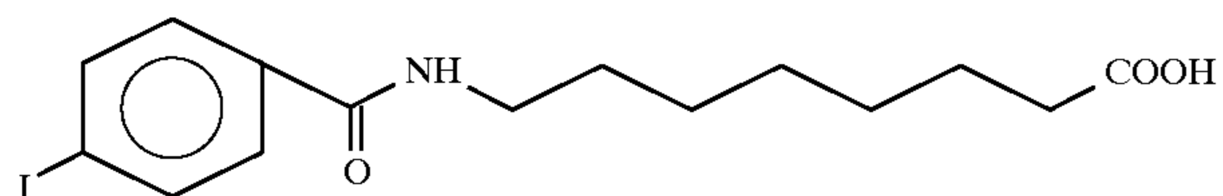
8-[N-(4-iodobenzoyl)]aminocaprylic acid
