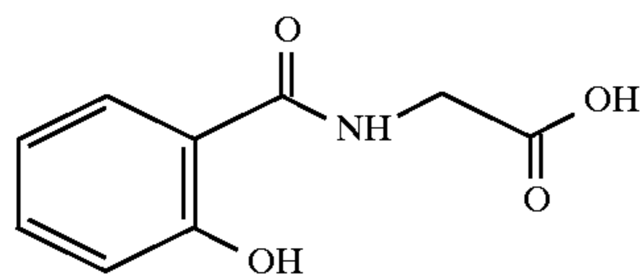
salicyloylglycine
