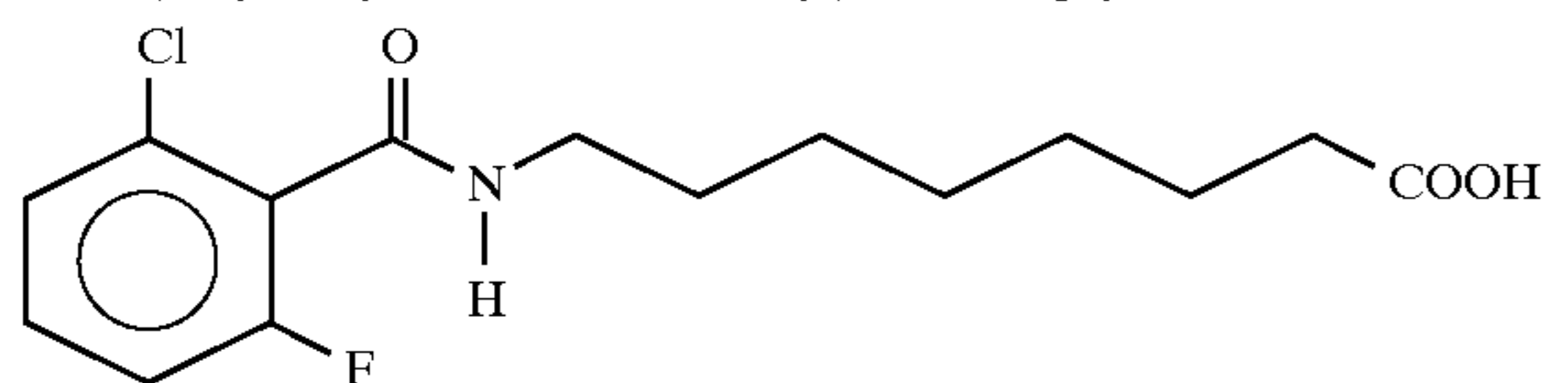
8-N-(2-chloro-6-fluorobenzoyl)aminocaprylic acid
