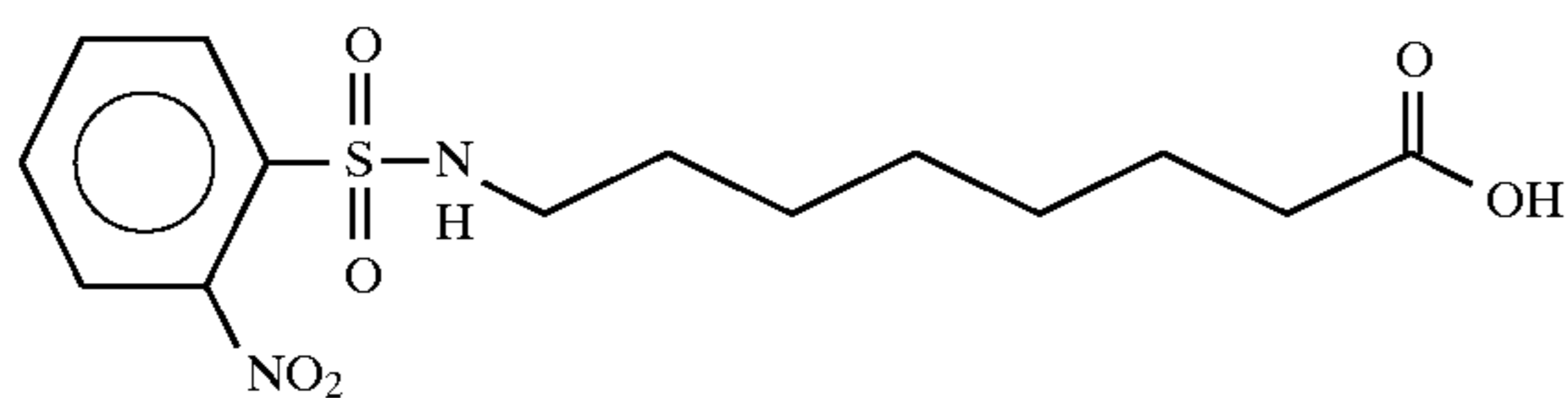
8-(2-nitrobenzenesulfonyl)aminocaproic acid
