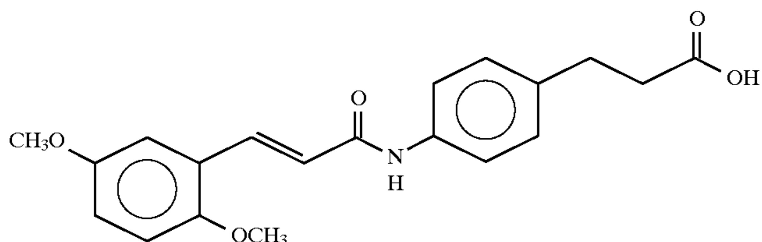
3-(4-(2,5-dimethoxycinnamoyl)aminophenyl)propionic acid
