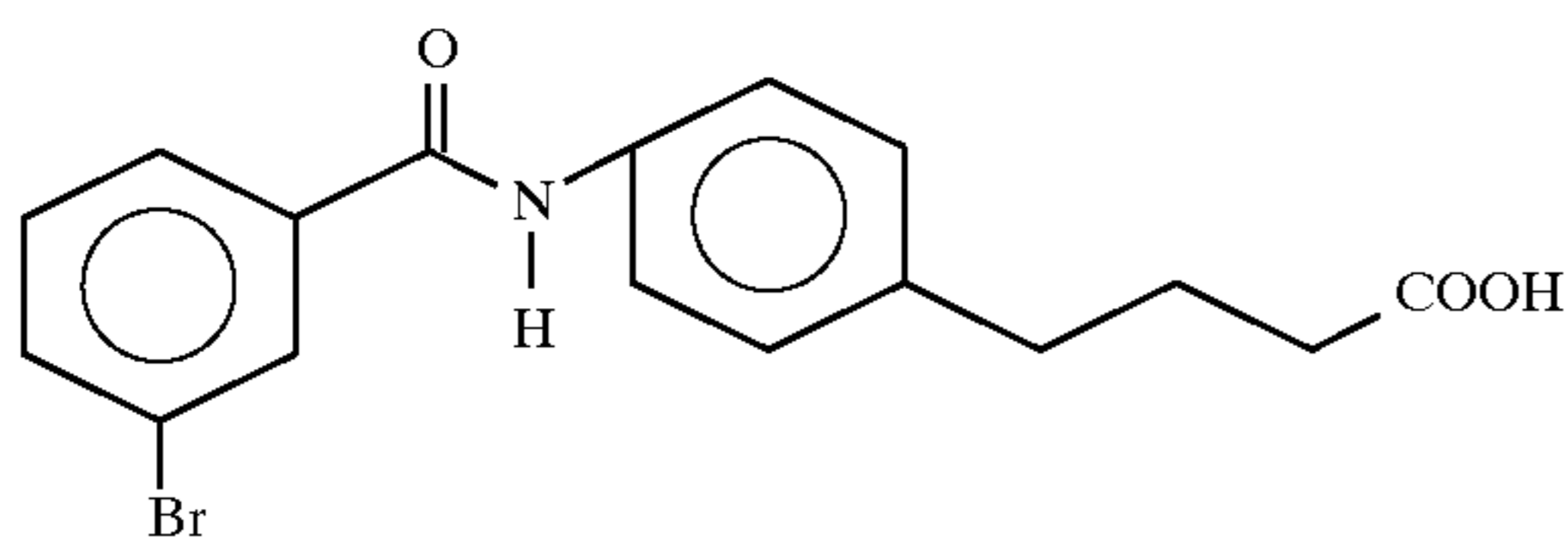
4{4-[N-3-bromobenzoyl; aminophenyl]} butyric acid
