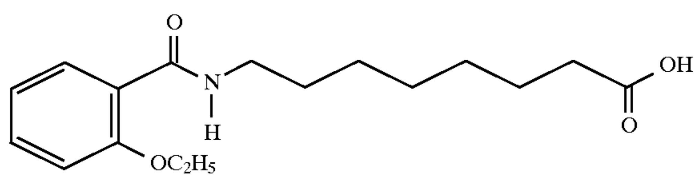
8-(2-ethoxybenzoyl)aminocaprylic acid
