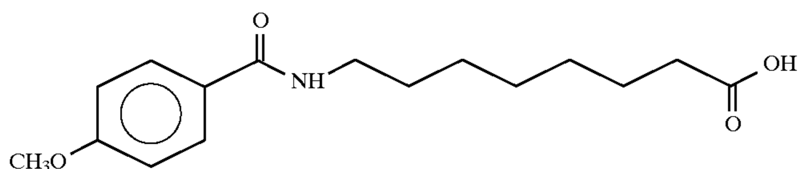
8-(p-anisoyl)aminocaprylic acid
