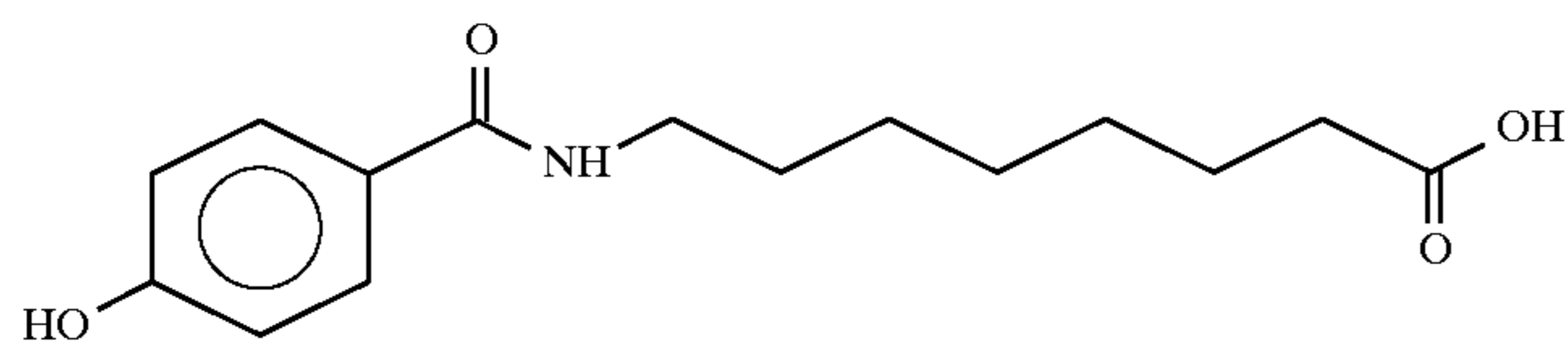
8-(4-Hydroxybenzoyl)aminocaprylic acid
