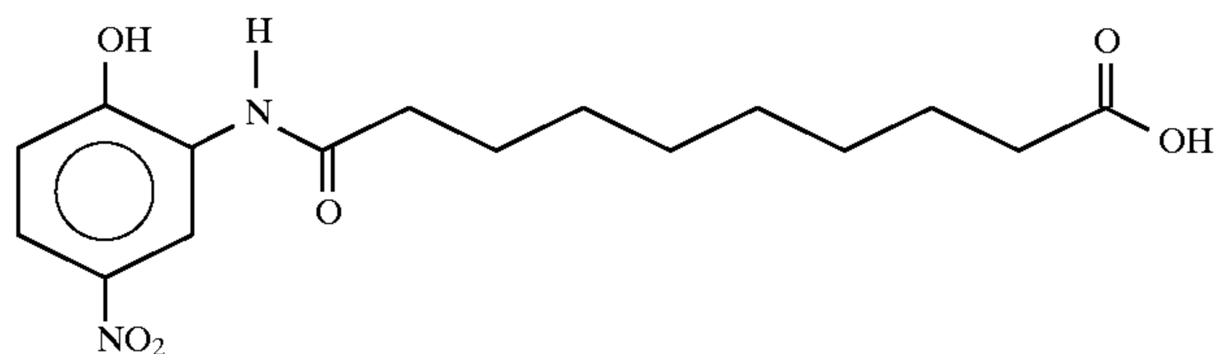
N-10-(2-hydroxy-5-nitroanilino)decanoic acid
