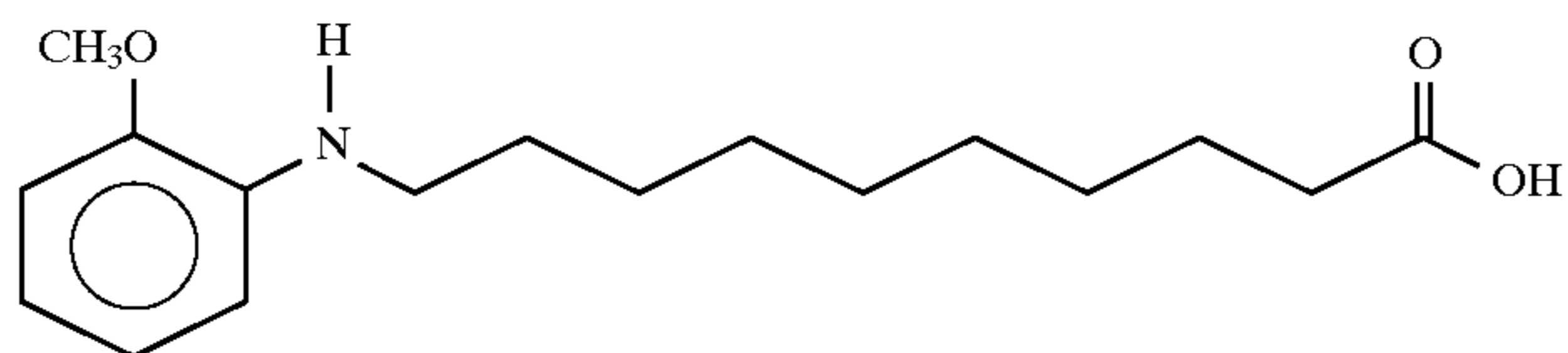
2-Methoxybenzenaminodecanoic acid
