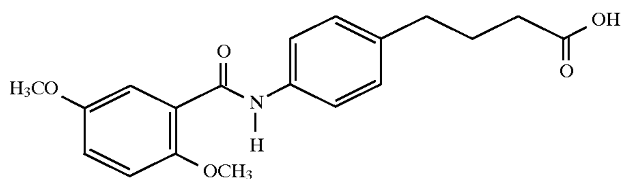
4-(4-(2,5-dimethoxybenzoyl)aminophenyl)butyric acid
