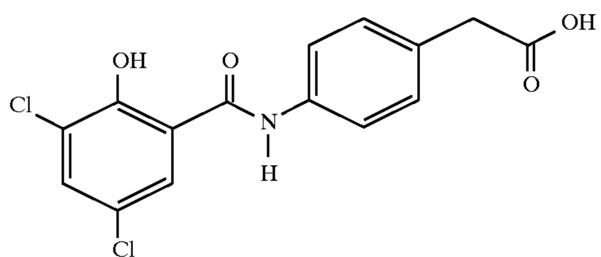
4-[N-(3,5-dichloro-2-hydroxybenzoyl)aminophenyl]acetic acid
