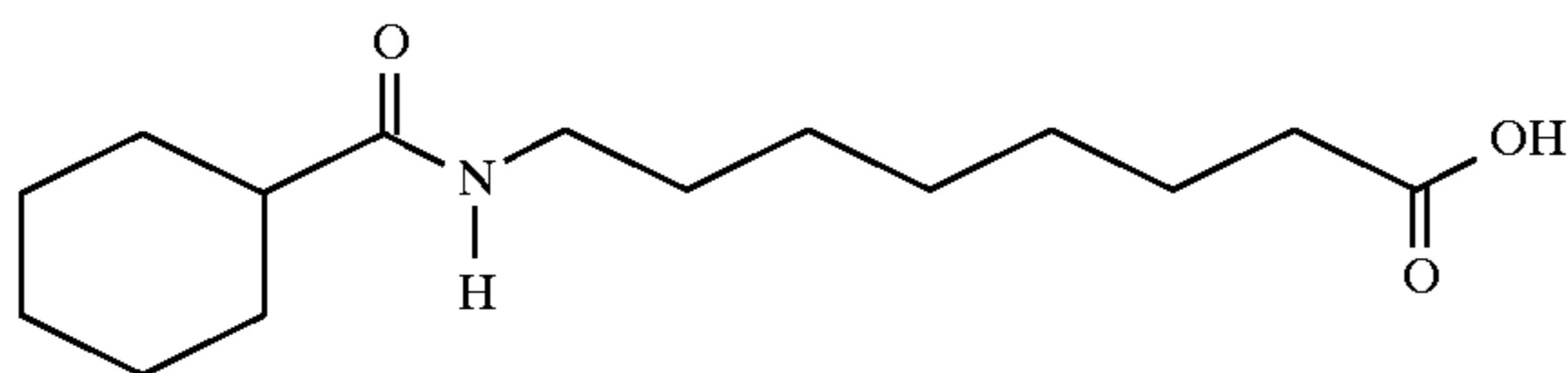
8-N-cyclohexanoylaminovaleric acid
