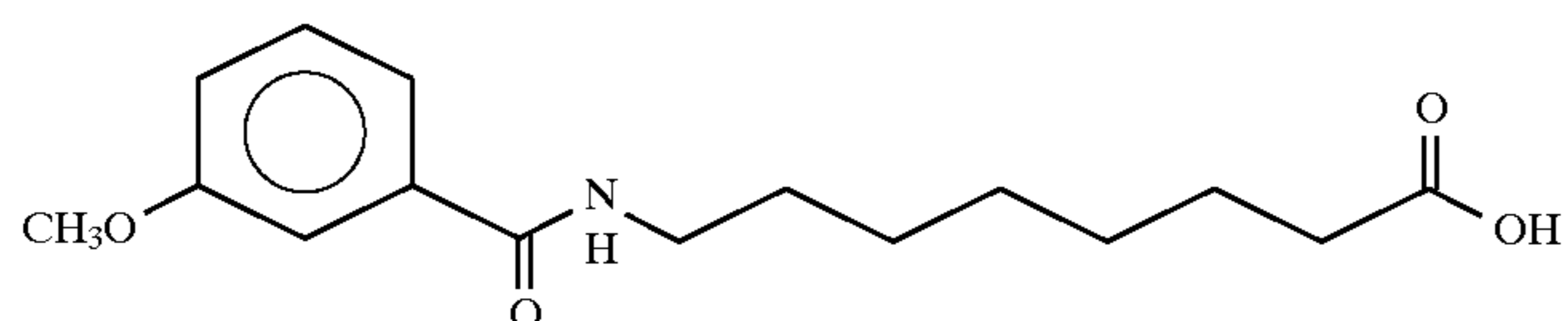
8-(3-anisoyl)aminocaprylic acid
