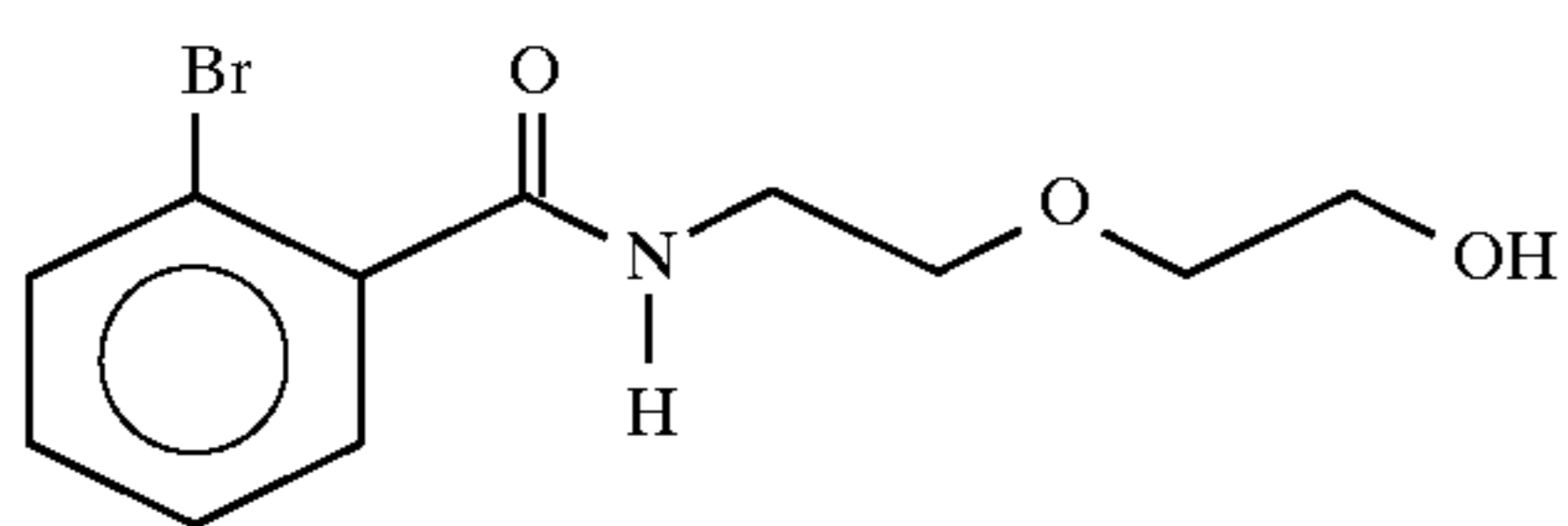
2-[N-(2-bromobenzoyl)aminoethoxy]ethanol
