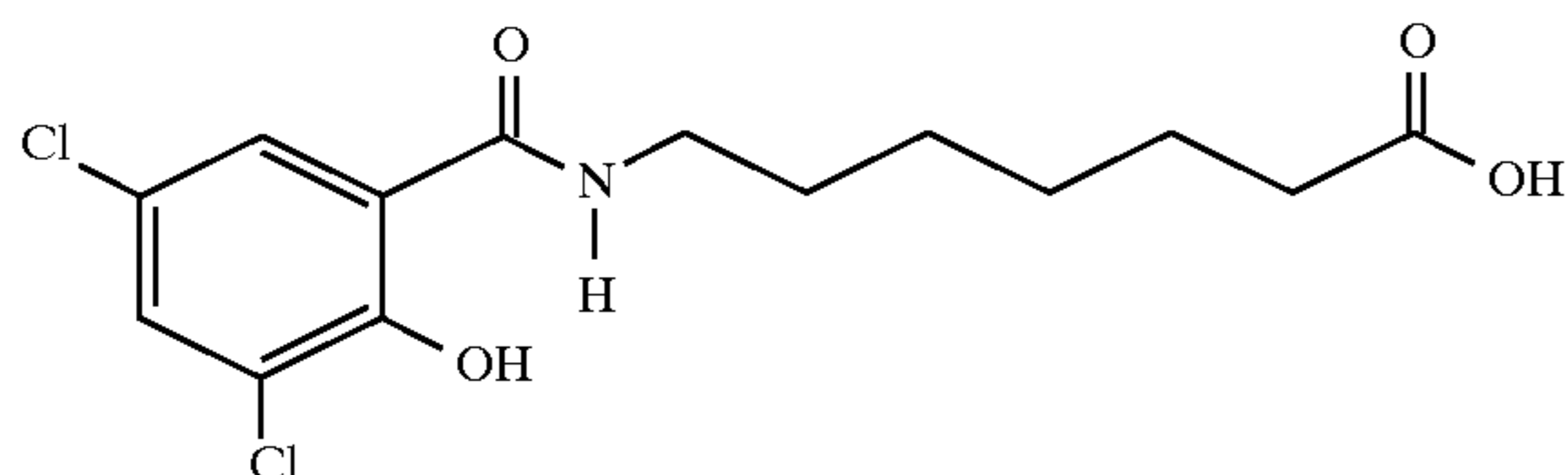
7-N-(3,5-dichloro-2-hydroxybenzoyl)aminoheptanoic acid
