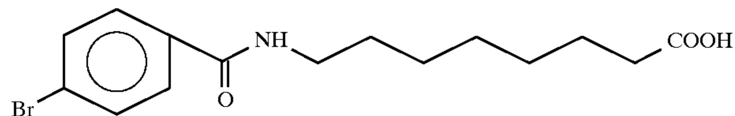
8-[N-(4-bromobenzoyl)]aminocaprylic acid
