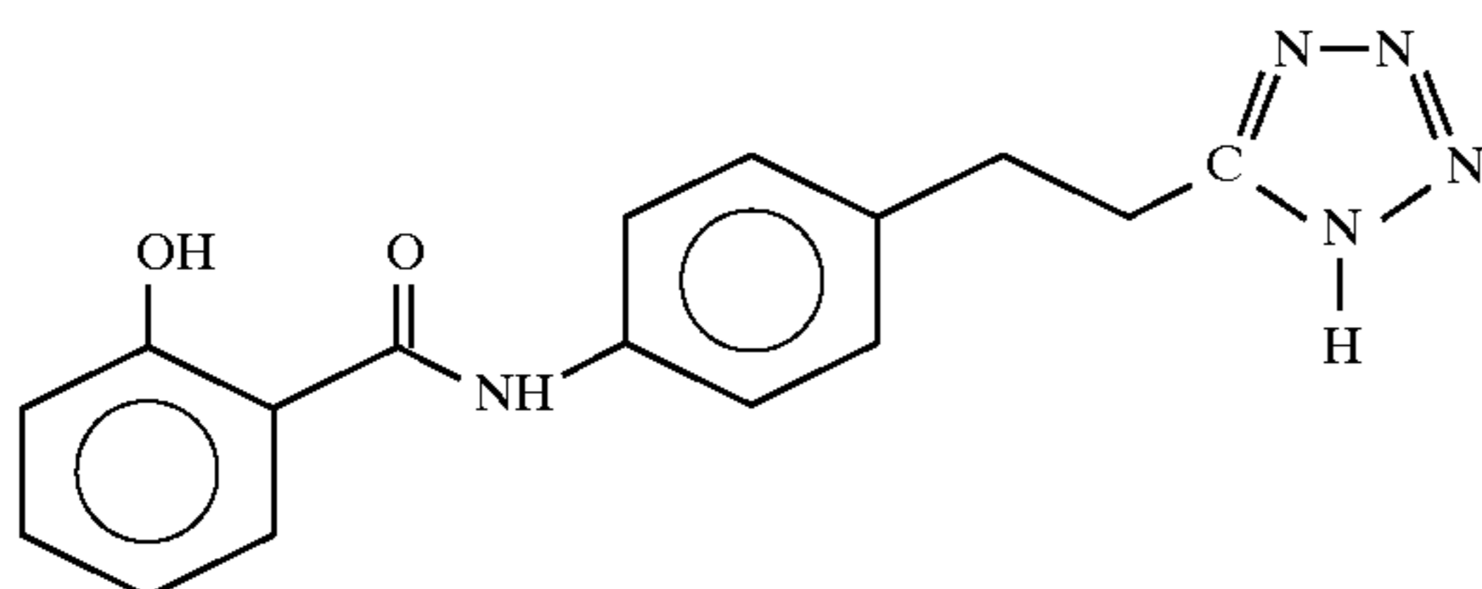
4-(Salicyloyl)aminophenylethyltetrazole
