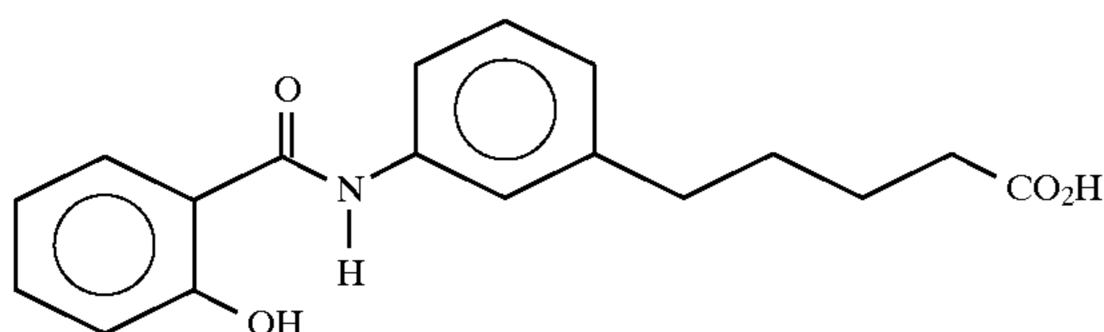
N-salicyloyl-5-(3-aminophenyl)valeric acid
