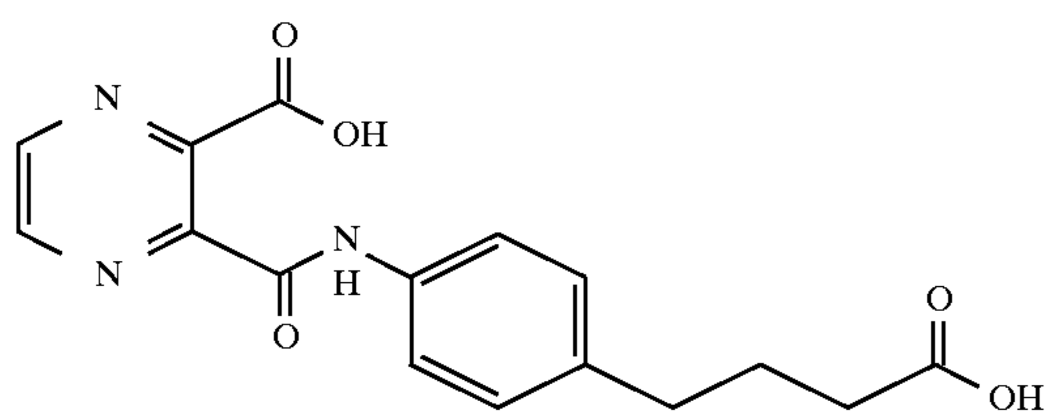
4-(4-(2-(3-carboxyl)pyrazinecarbonyl)aminophenyl)butyric acid
