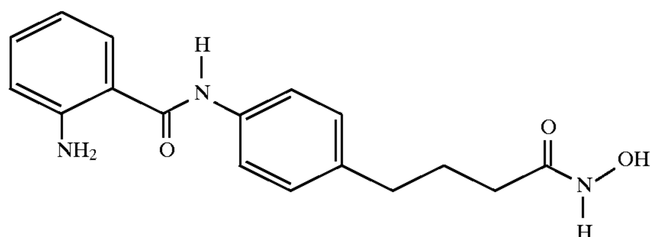
4-[4-(2-aminobenzoylamino)phenyl]butyrylhydroxamic acid
