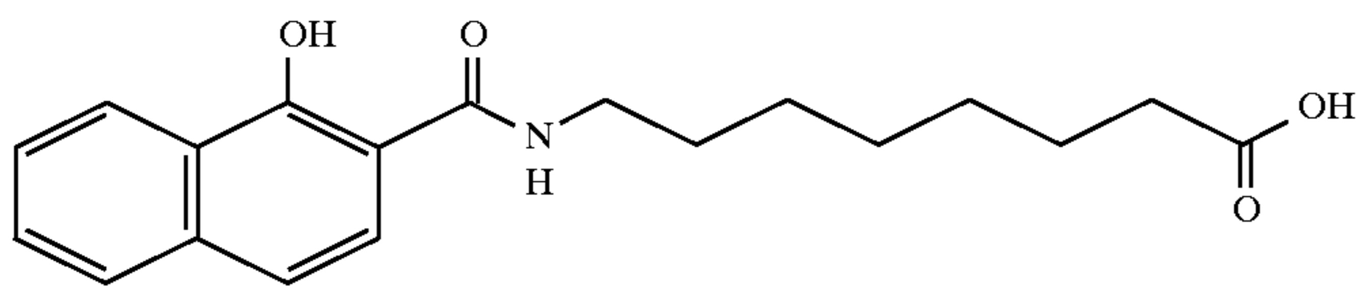
8-(N-(1-hydroxy-2-naphthoyl)aminocaprylic acid
