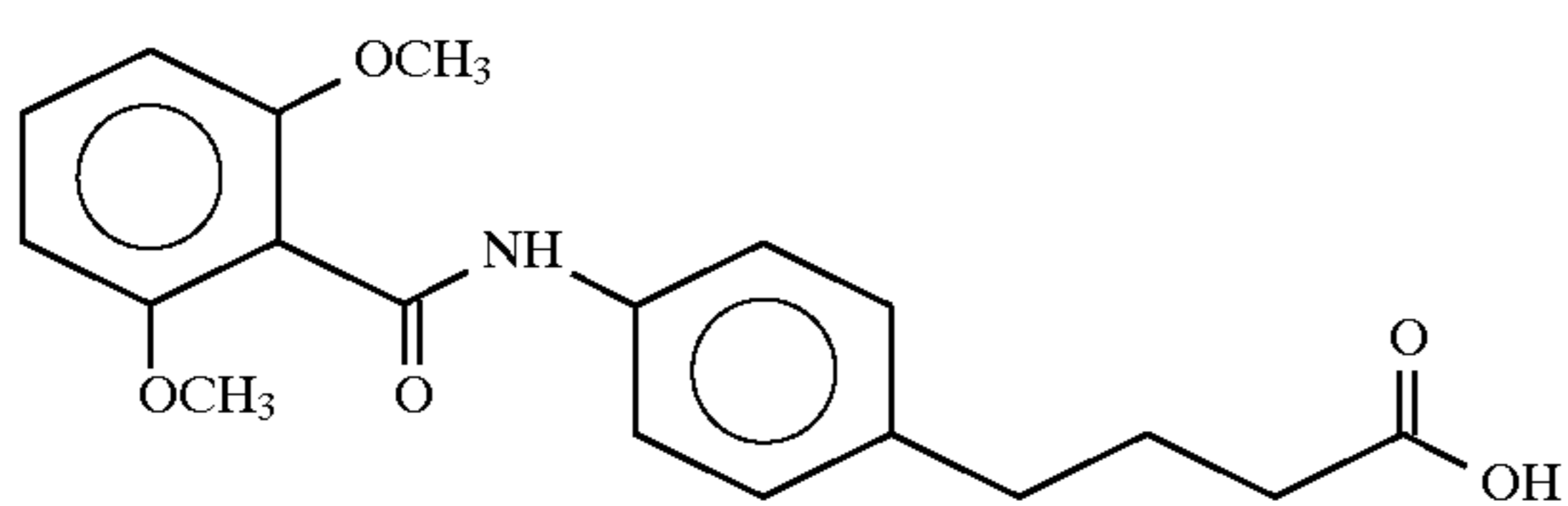
4-(4-(2,6-dimethoxybenzoyl)aminophenyl)butyric acid
