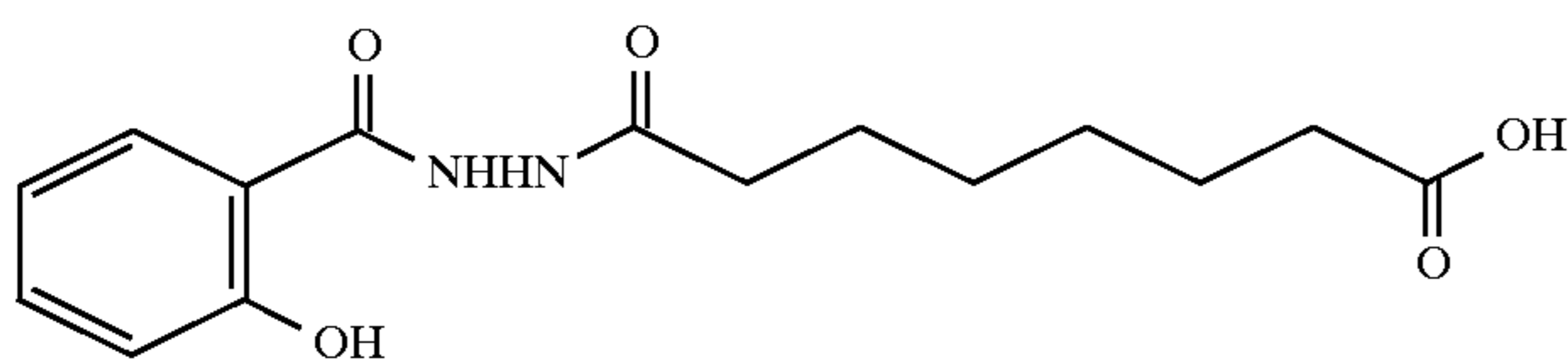
1-salicyloyl-2-suberyl hydrazide
