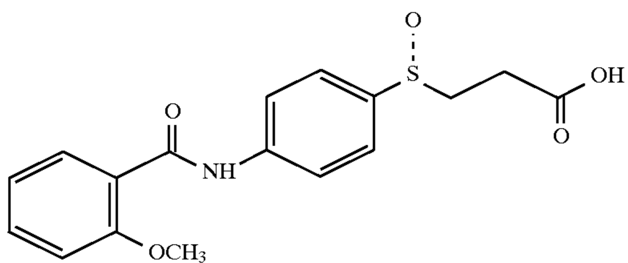
4-(2-methoxybenzoyl)amino 3-carboxysulfoxide
