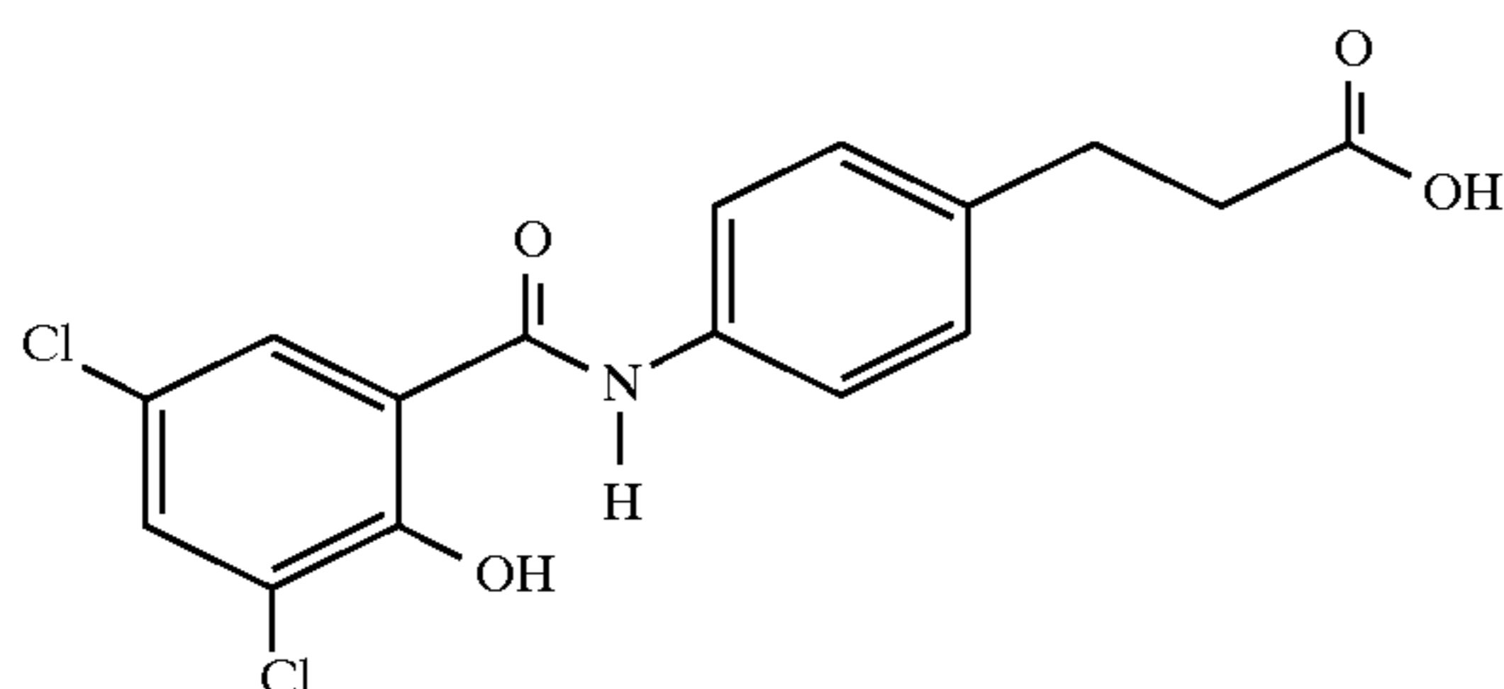
N-[3,5-dichloro-2-hydroxybenzoyl-3-(4-aminophenyl)]propionic acid
