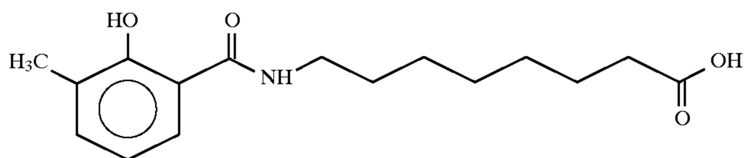
8-(N-3-methylsalicyloyl)aminocaproic acid
