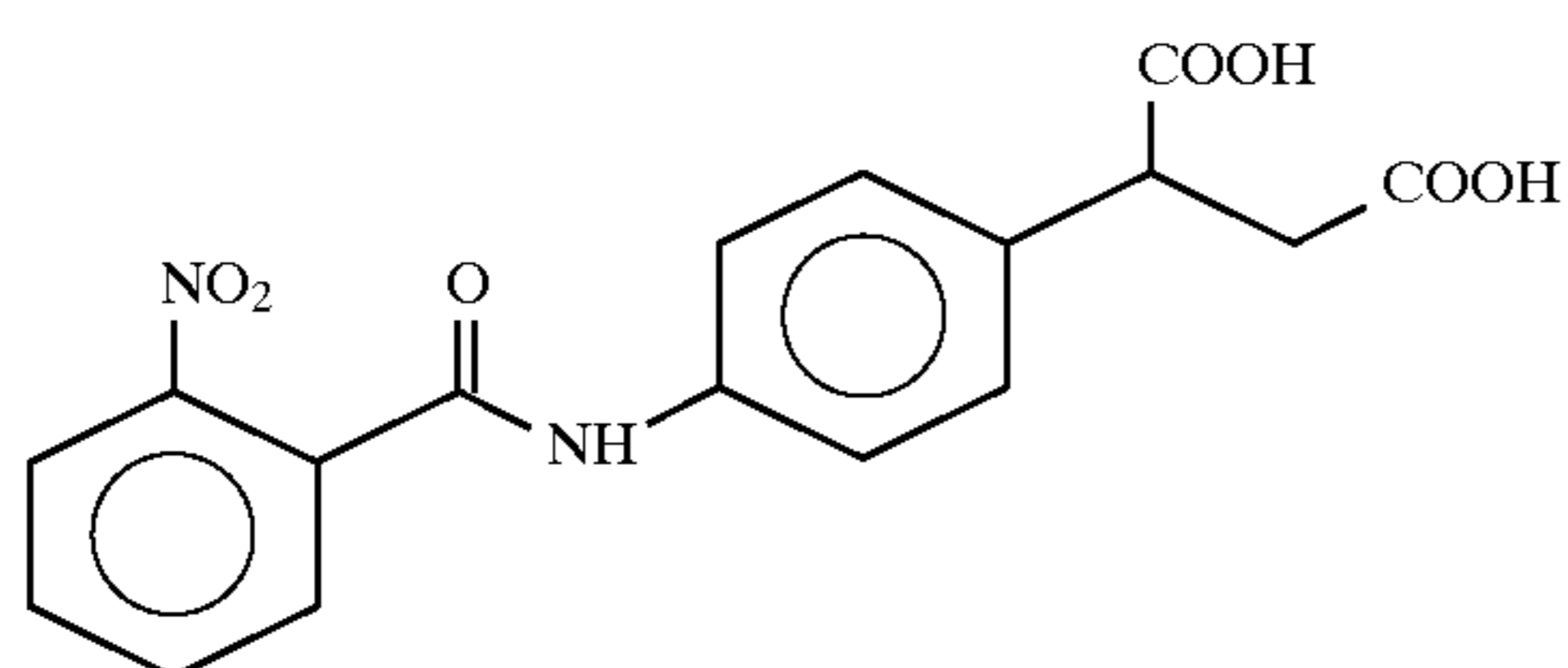
4-(2-Nitrobenzoyl)aminophenylsuccinic acid
