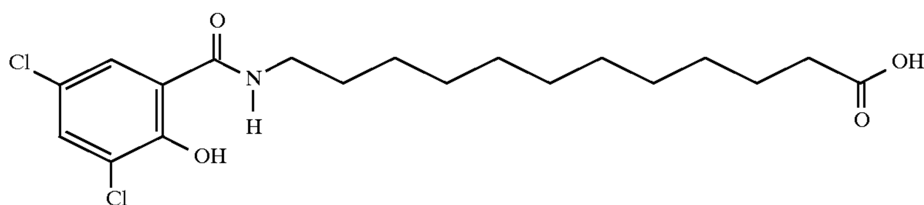
12-N-(3,5-dichloro-2-hydroxybenzoyl)aminododecanoic acid
