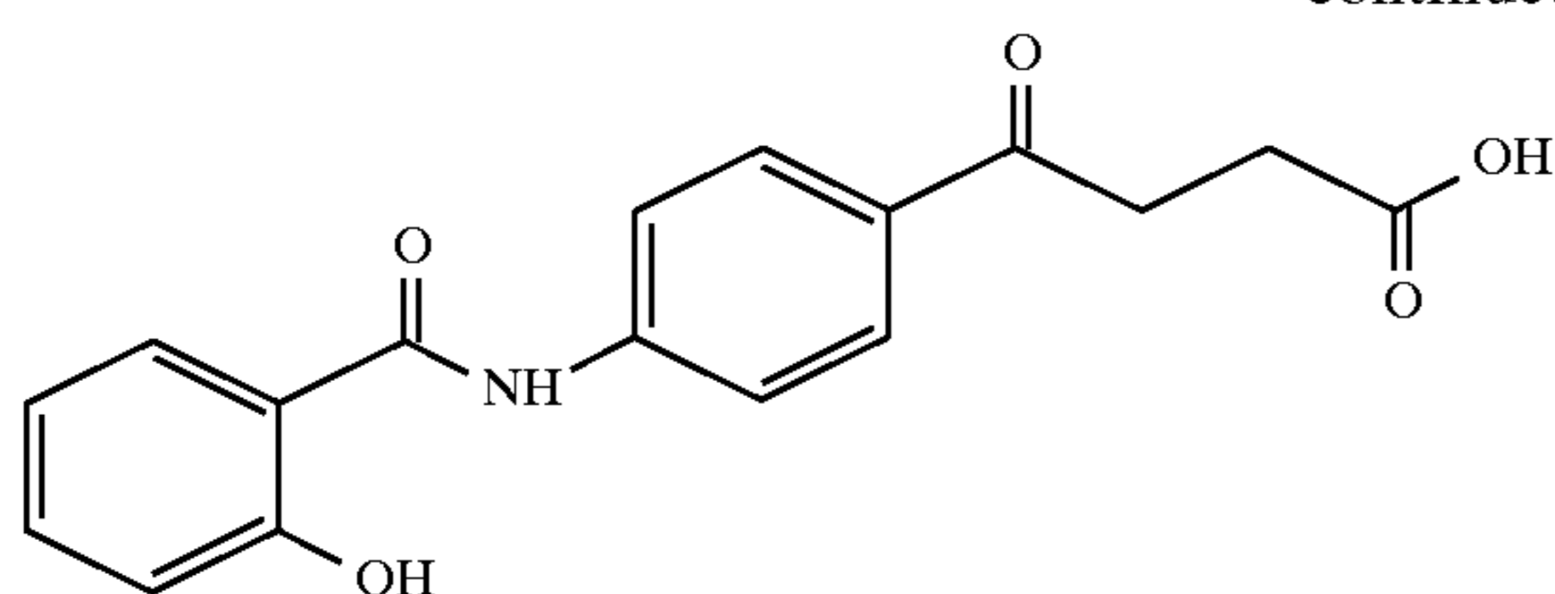
4-(4-salicyloylamino-phenyl)-4-oxobutanoic acid
