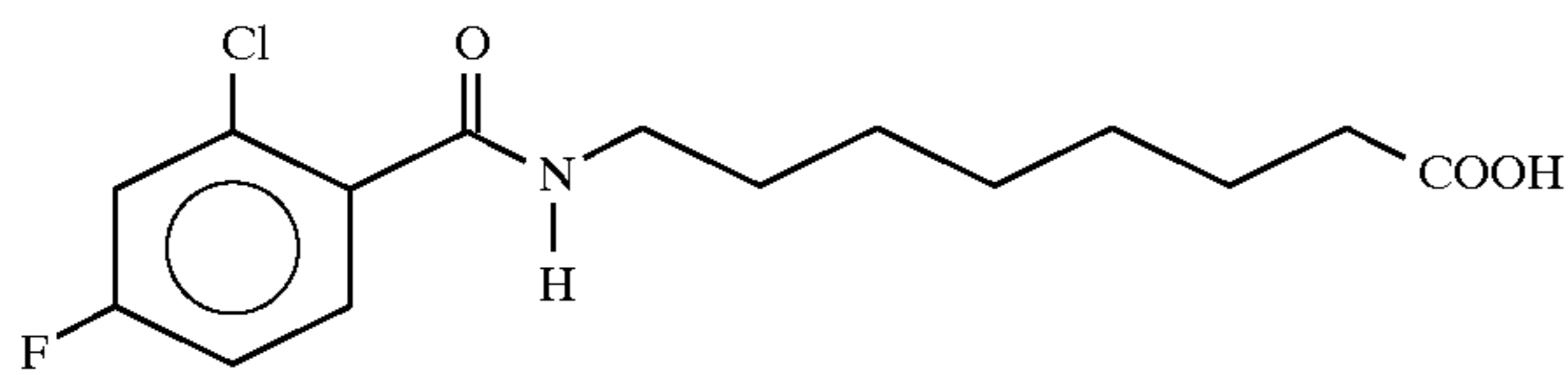
8-(N-(2-chloro-4-fluorobenzoyl)aminocaprylic acid
