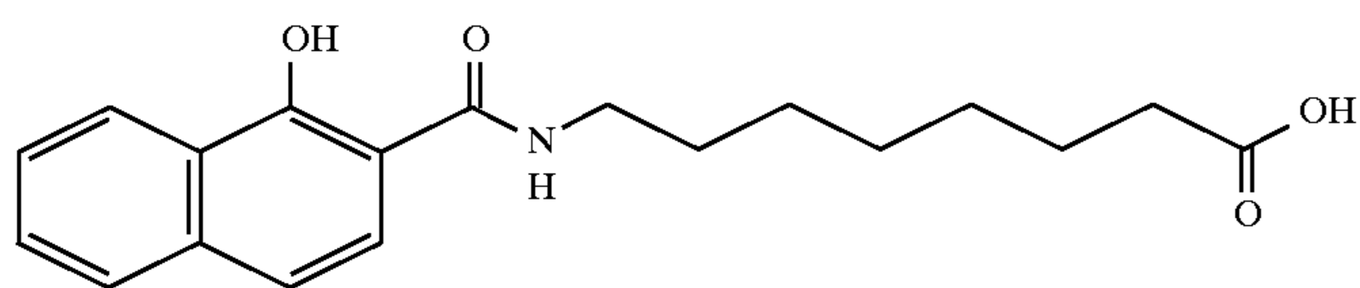
8-(N-(1-hydroxy-2-naphthoyl)aminocaprylic acid
