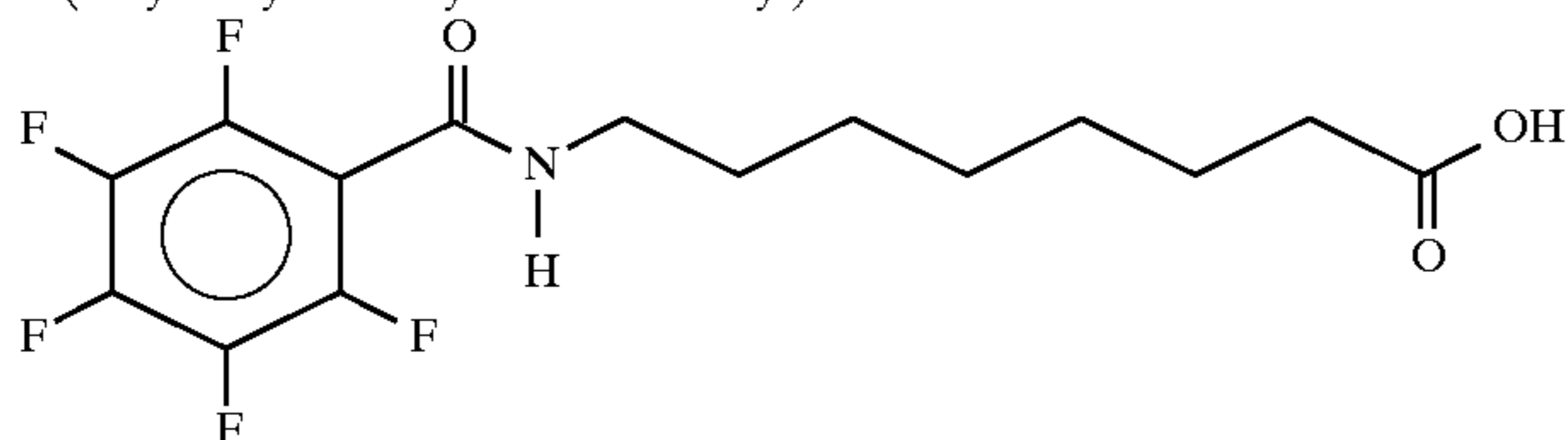
8-(pentafluorobenzoyl)aminocaproic acid
