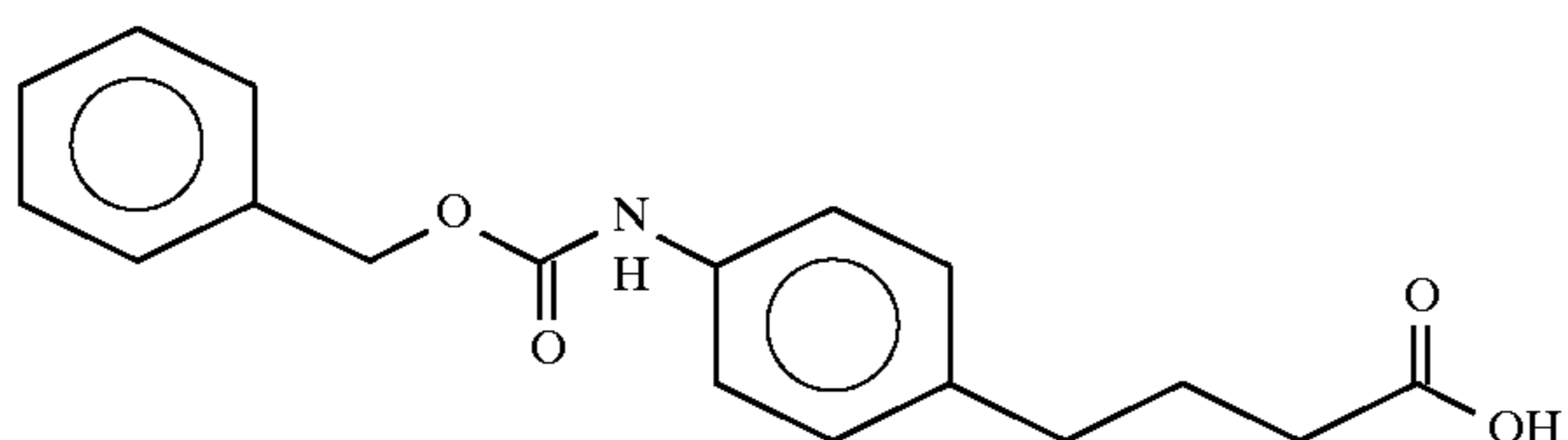
4-(4-benzyloxycarbonylamino)phenylbutyric acid
