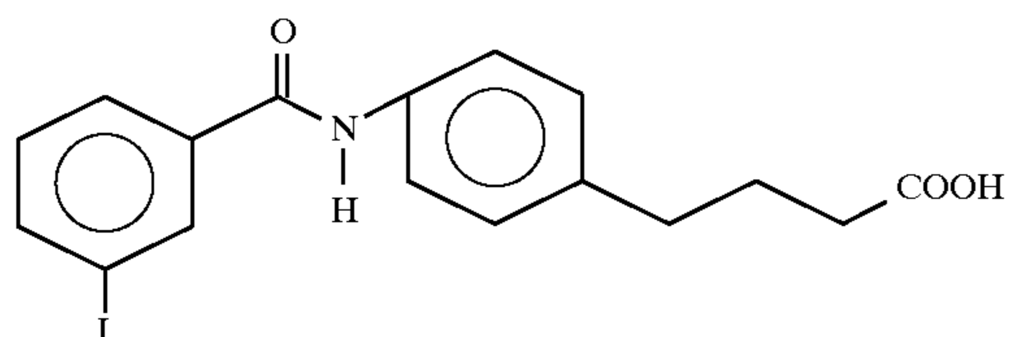
4-{N-[4-(3-iodobenzoyl)aminophenyl]}butyric acid
