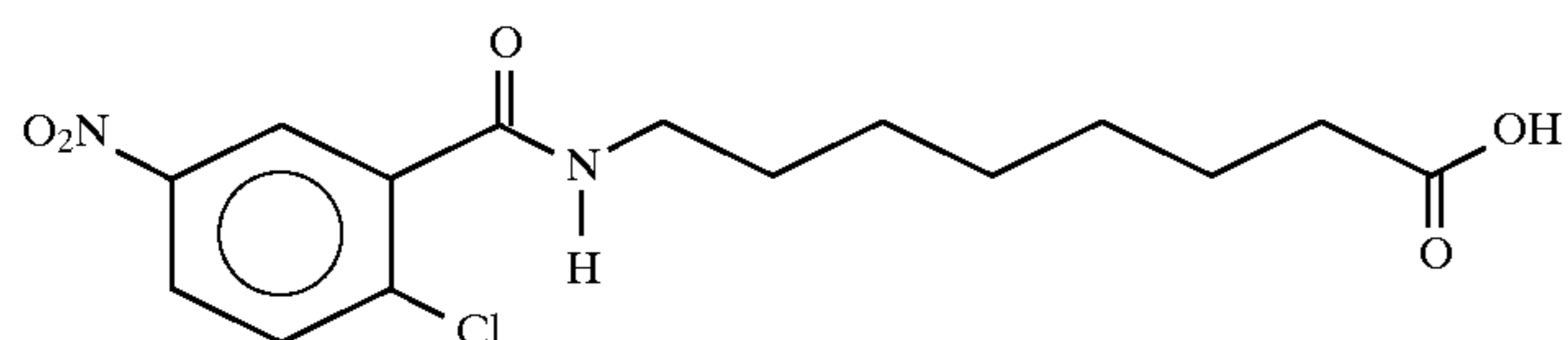
8-(2-chloro-5-nitrobenzoyl)aminocaproic acid
