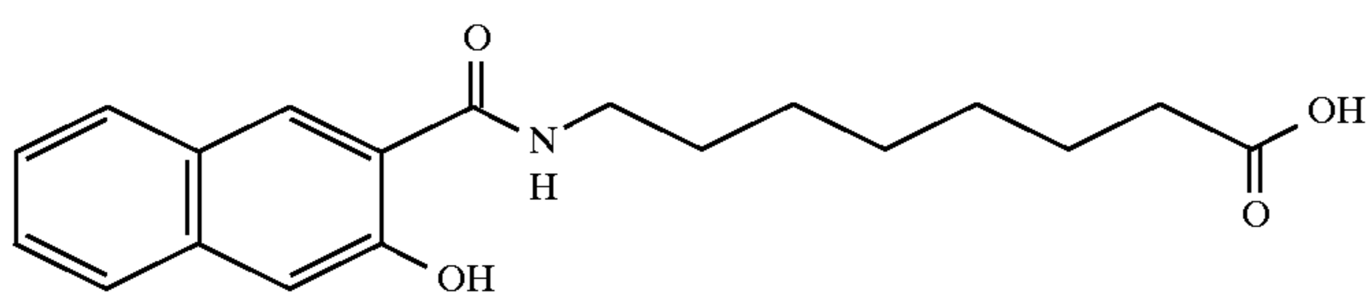
8-(3-hydroxy-2-naphthoyl)aminocaproic acid
