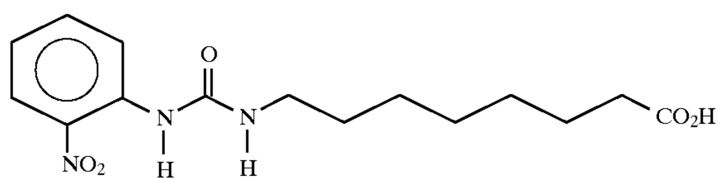
N-2-nitrophenyl-N'-(8-octanoic acid) urea
