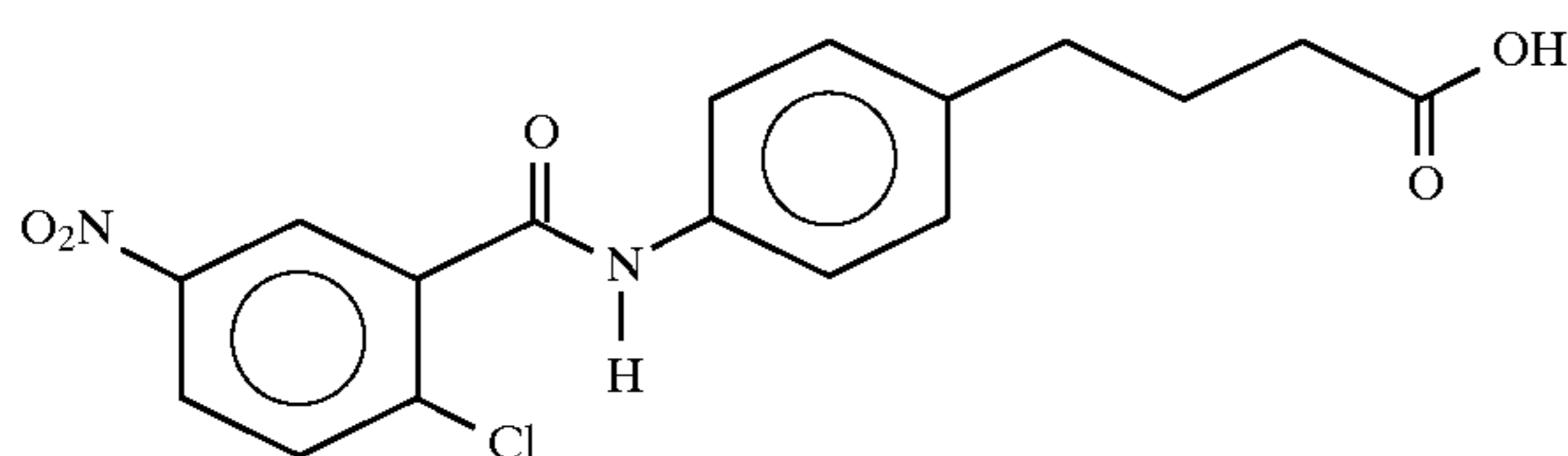
4-(4-(2-chloro-5-nitrobenzoyl)aminophenyl)butyric acid
