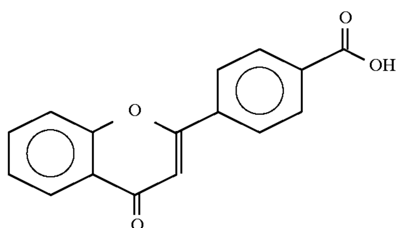
4'-flavonic acid
