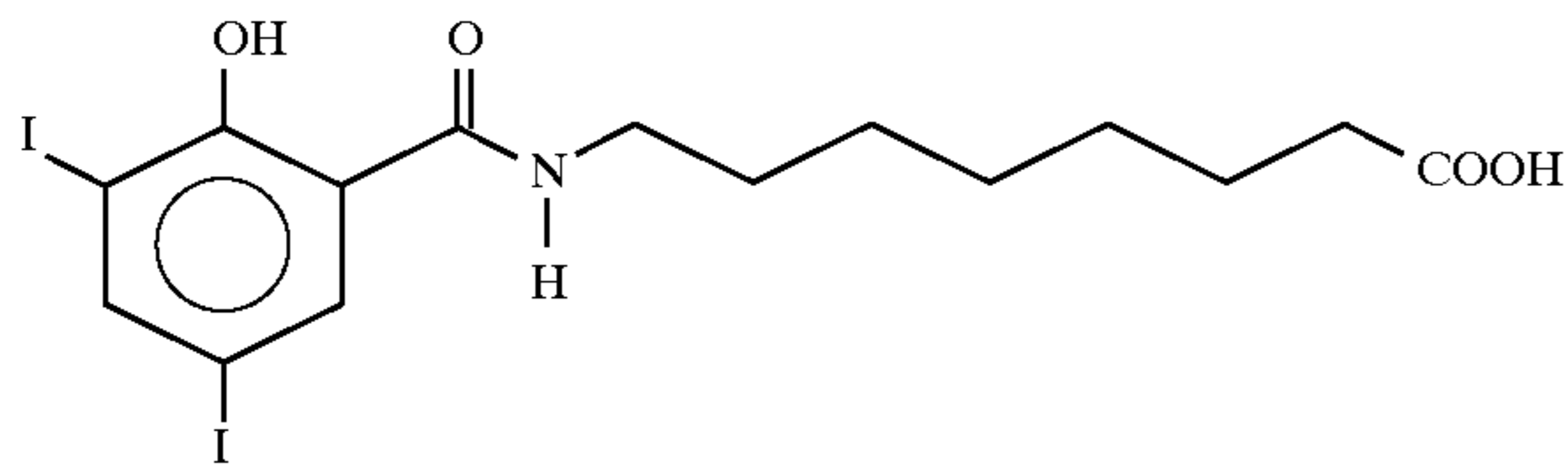
8-(N-(2-hydroxy-3,5-diiodobenzoyl)aminocaprylic acid
