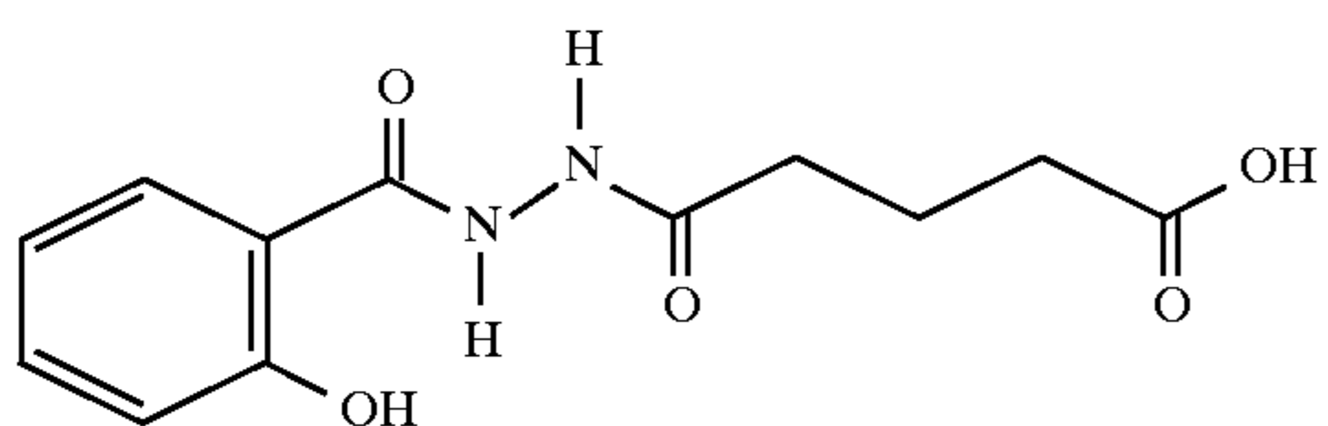
1-salicyloyl-2-glutaryl hydrazide
