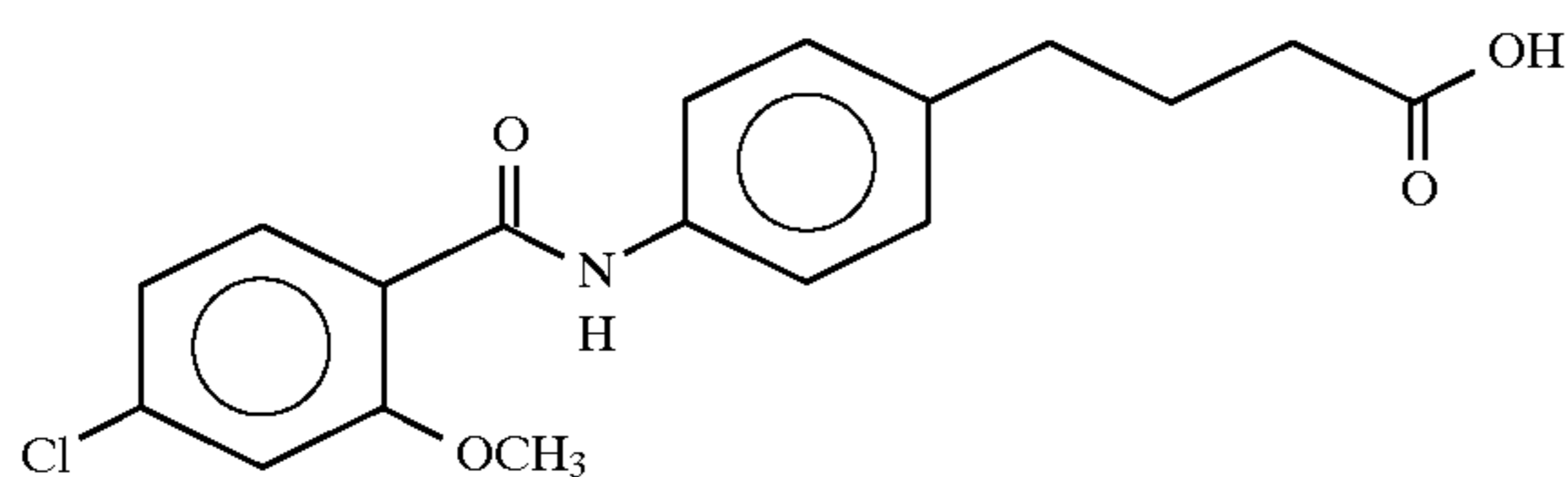
4-(4-(4-chloro-o-anisoyl)aminophenyl)butyric acid
