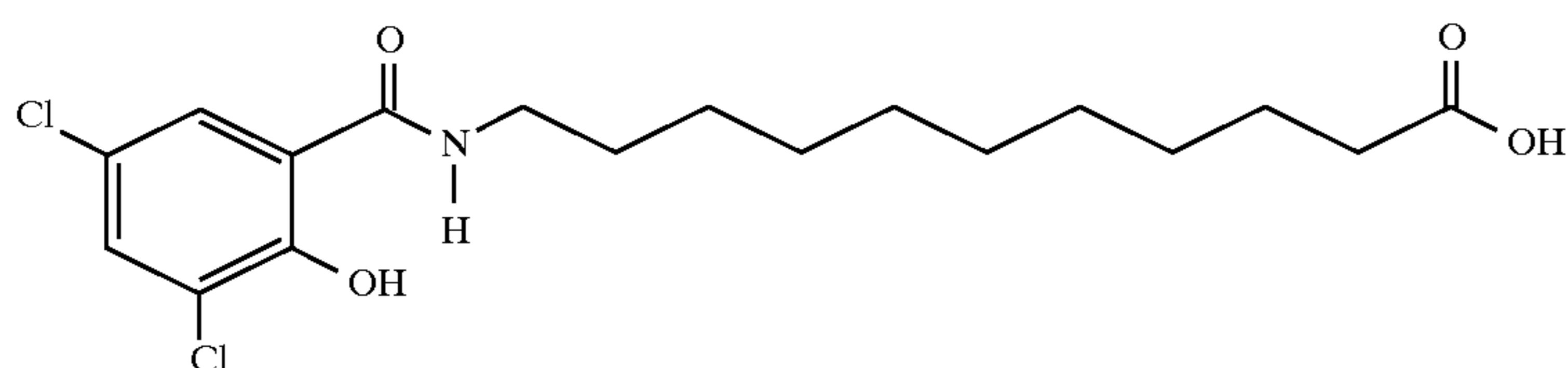
11-N-(3,5-dichloro-2-hydroxybenzoyl)aminoundecanoic acid
