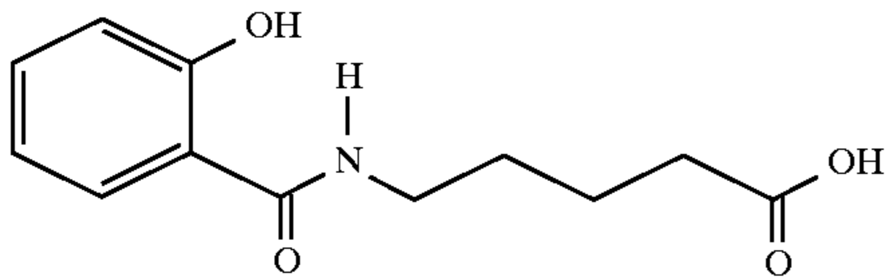
5-(N-salicyloylamino)valeric acid
