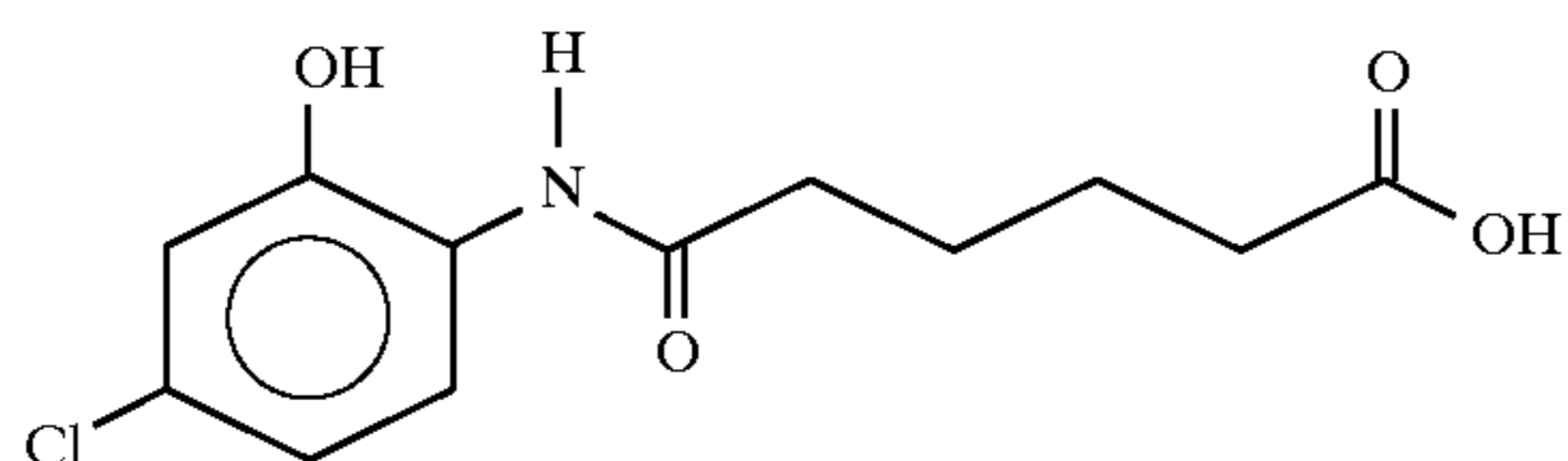
5-(4-chloro-2-hydroxyanilino)valeric acid
