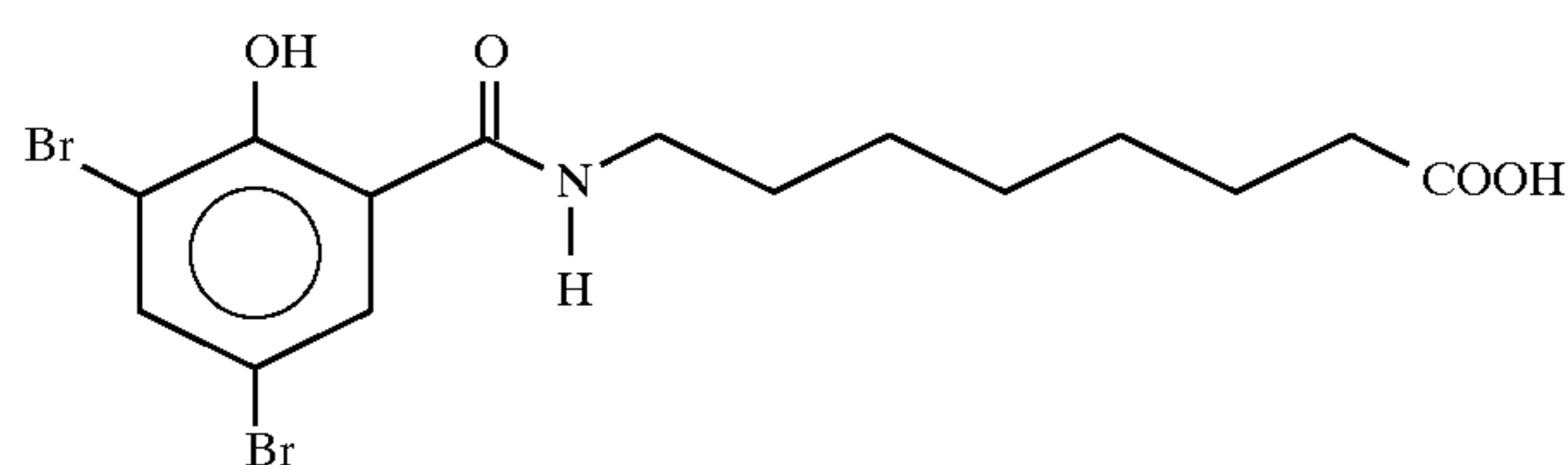
8-[N-(2-hydroxy-3,5-dibromobenzoyl)]aminocaprylic acid
