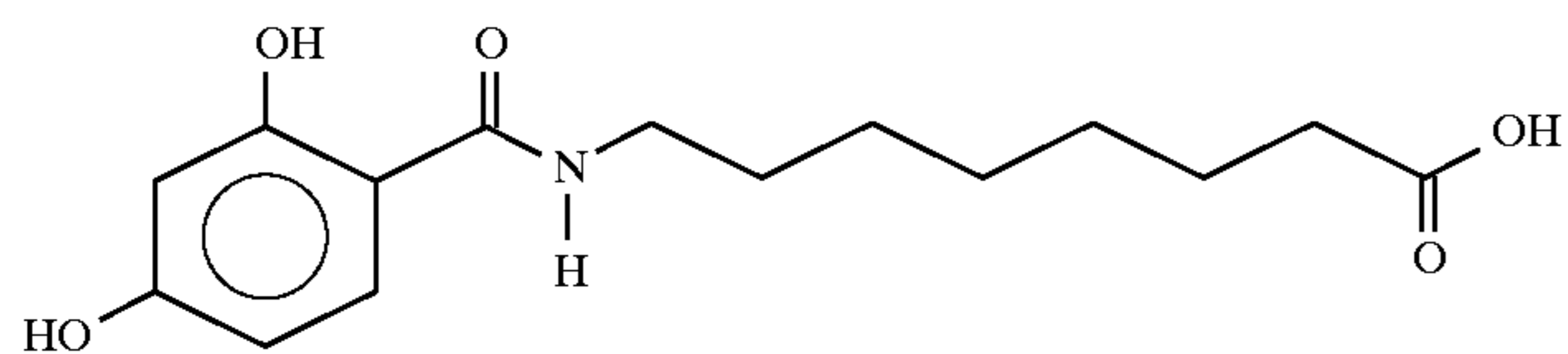
8-(N-2,4-Dihydroxybenzoyl)aminocaprylic acid
