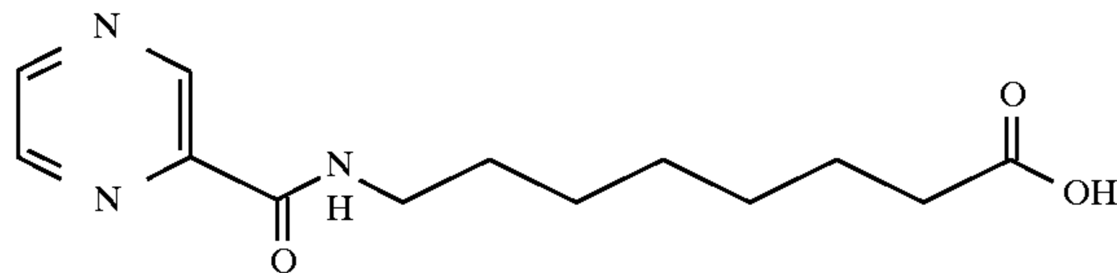
8-(2-pyrazinecarbonyl)aminocaprylic acid
