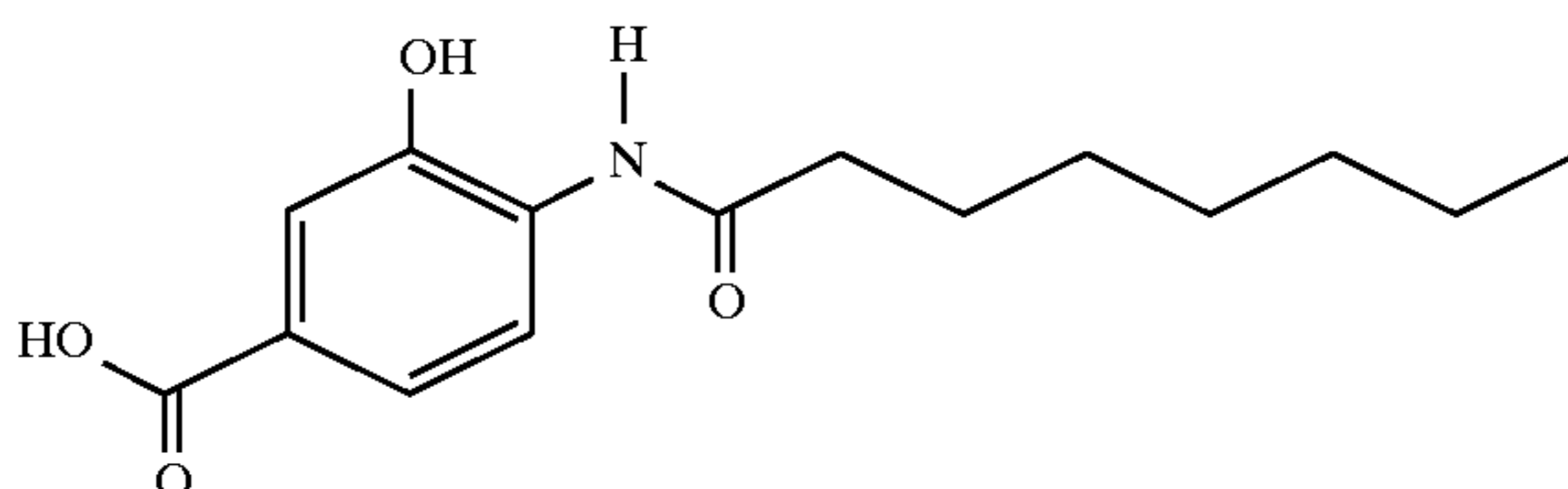
4-octanoylamino-3-hydroxybenzoic acid
