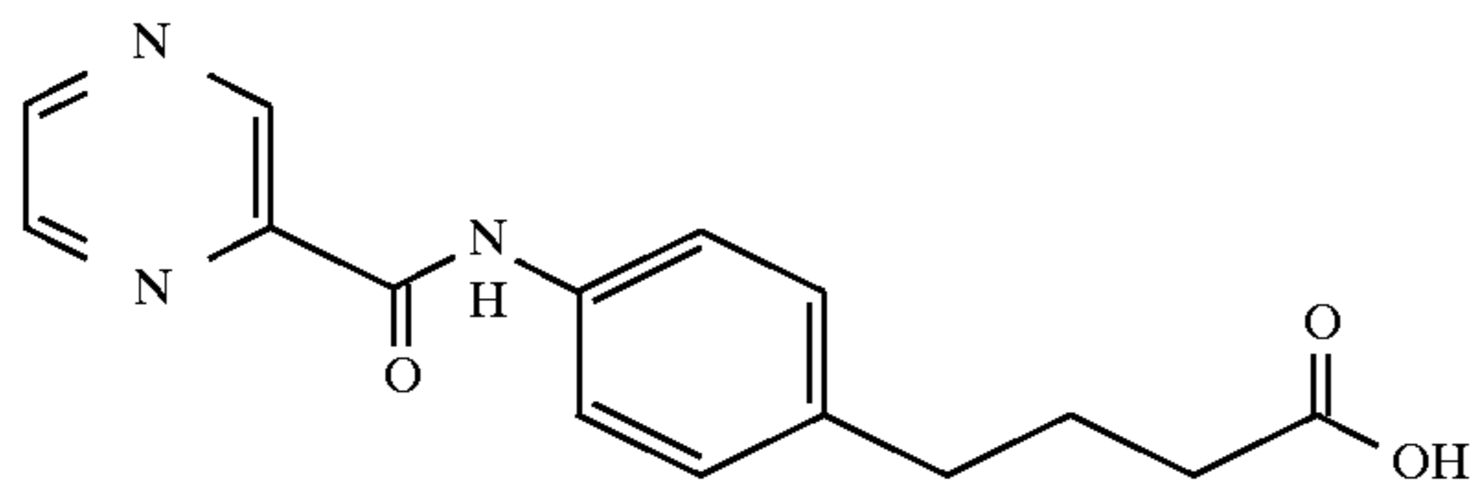
4-(4-(2-pyrazinecarbonyl)aminophenyl)butyric acid
