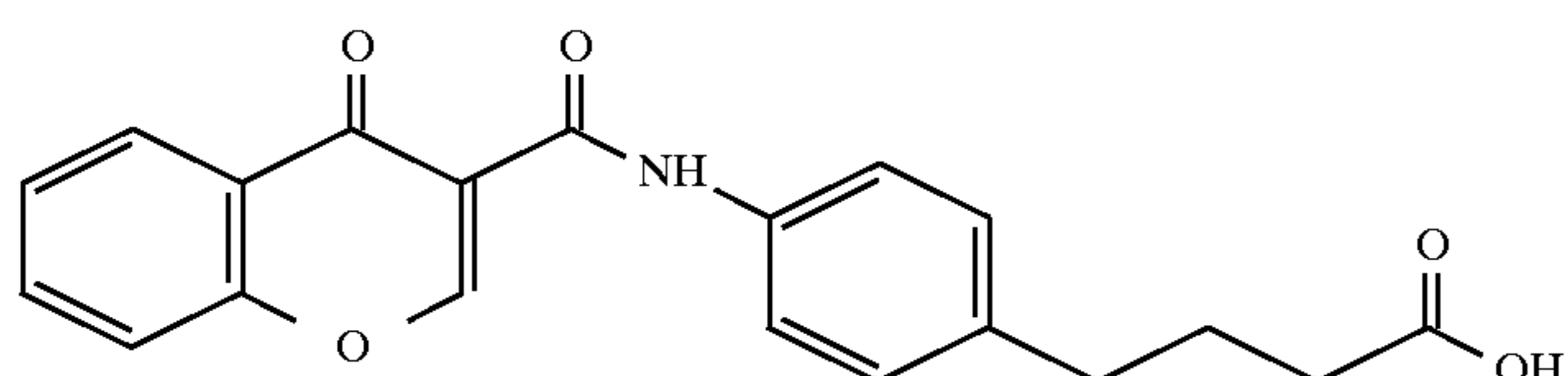
4-(4-chromone-3-carbonyl)aminophenylbutyric acid
