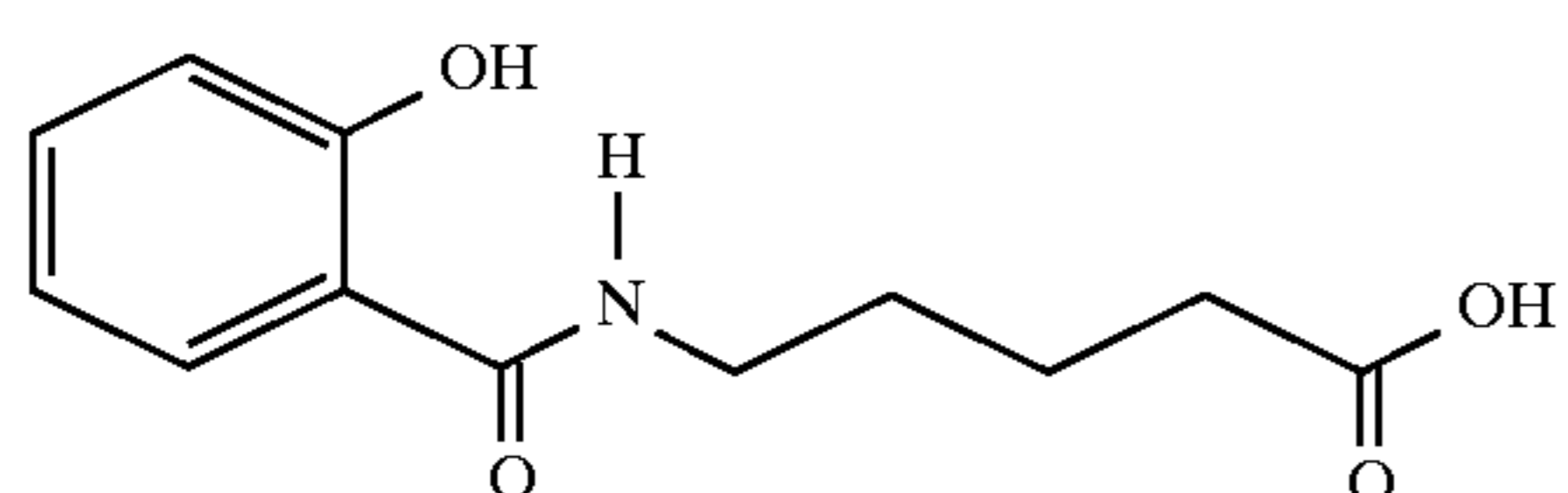
5-(N-salicyloylamino)valeric acid
