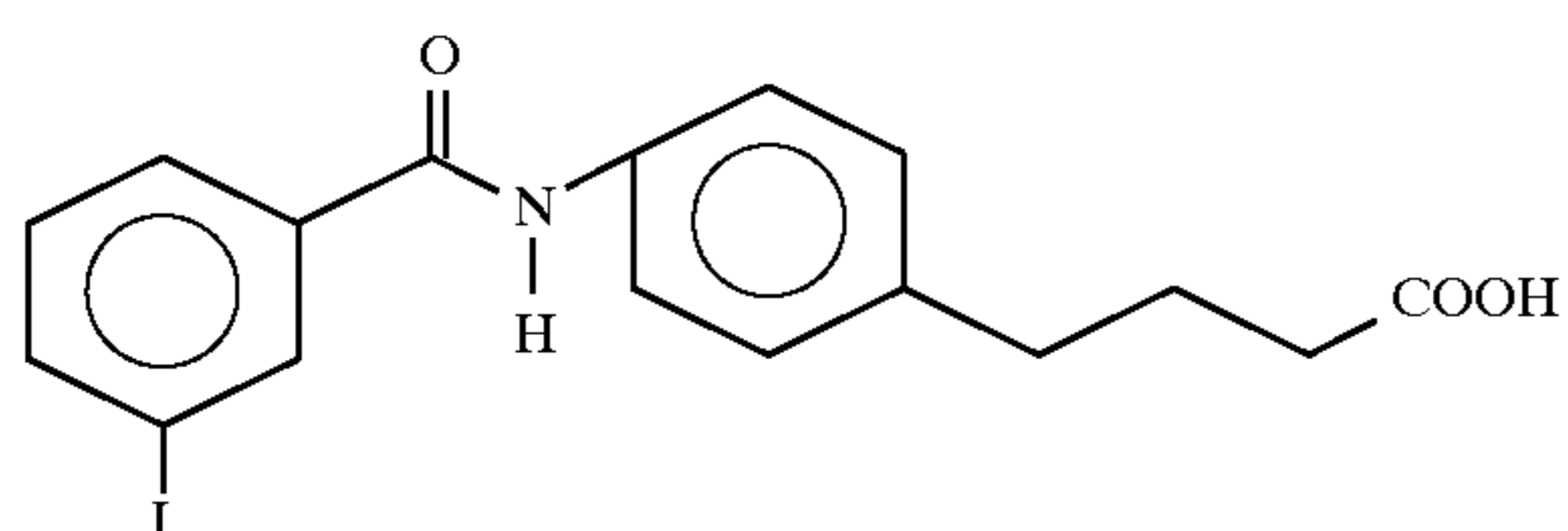
4-{N-[4-(3-iodobenzoyl)aminophenyl]}butyric acid
