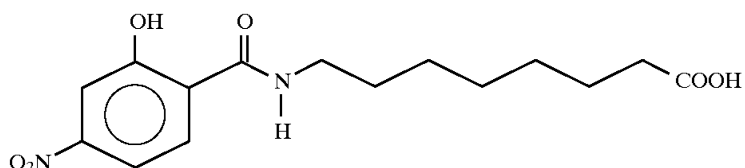
8-(N-2-hydroxy-4-nitrobenzoyl)aminocaproic acid
