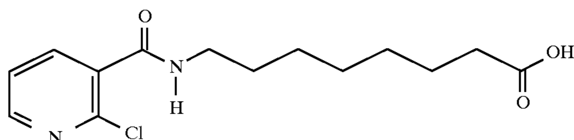
8-(2-chloronicotinoyl)aminocaproic acid
