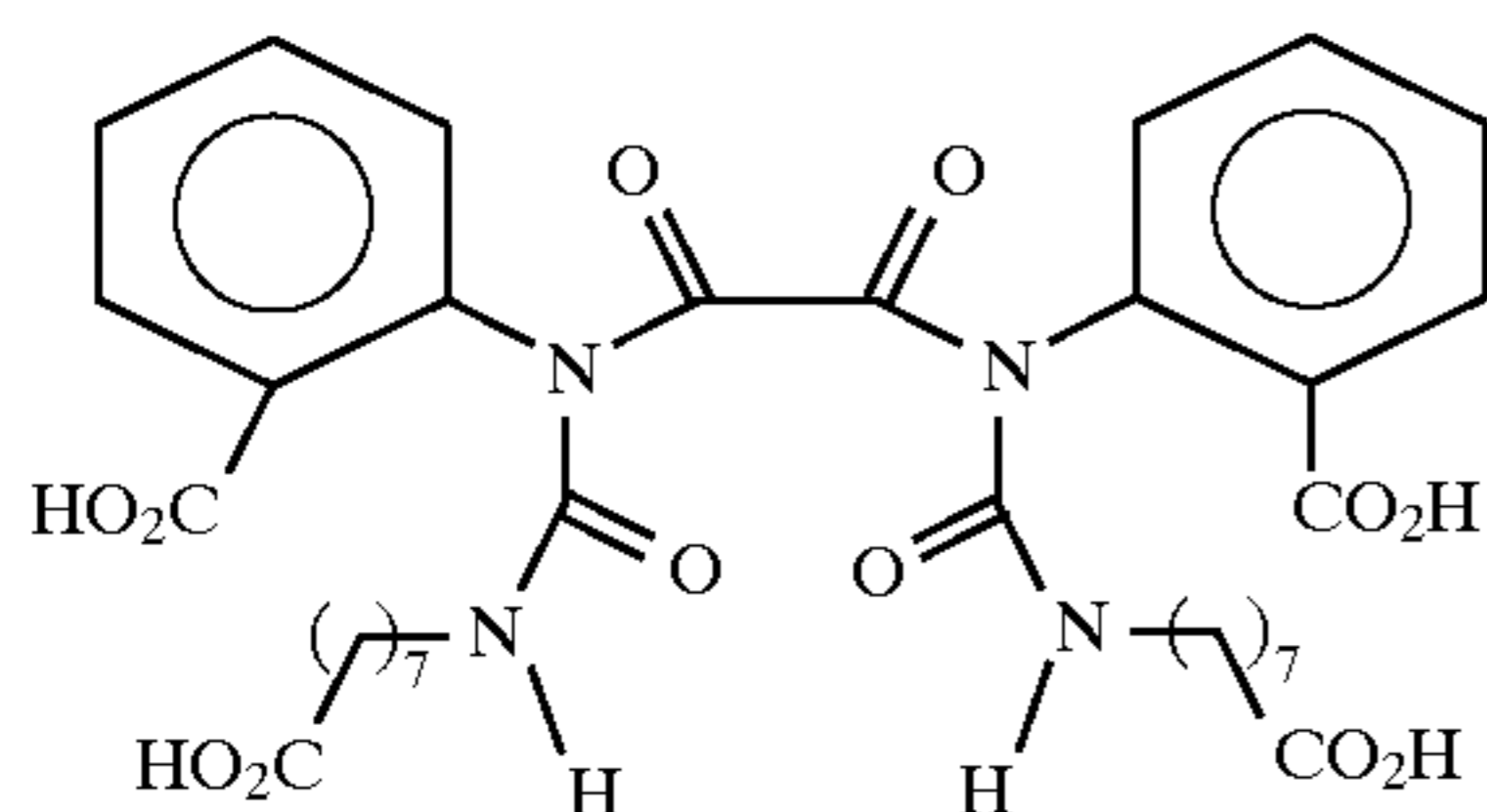
Bis(N-2carboxylphenyl-N-(N'-8-octanoic acid)ureal)oxalyl diamide
