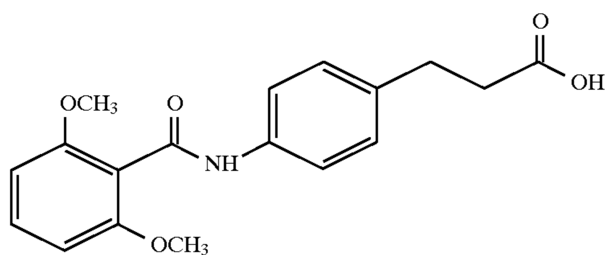
3-(4-(2,6-dimethoxybenzoyl)aminophenyl)propionic acid
