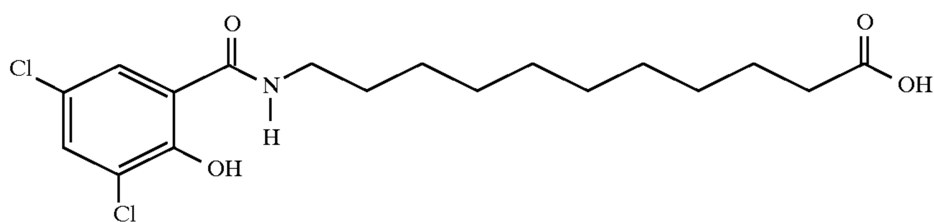
11-N-(3,5-dichloro-2-hydroxybenzoyl)aminoundecanoic acid
