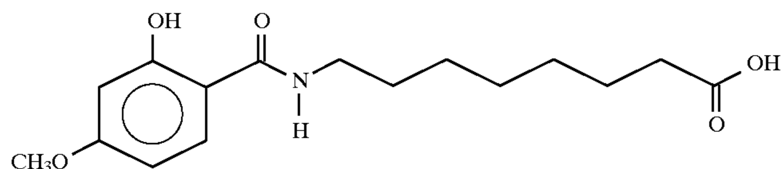
8-(N-2-Hydroxy-4-methoxybenzoyl)aminocaprylic acid
