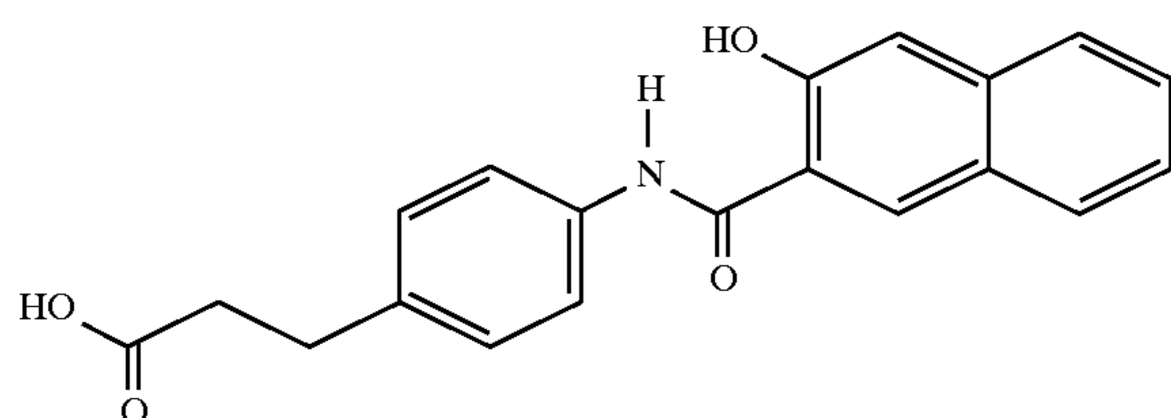
4-(4-(N-(3-hydroxy-2-naphthoyl)aminophenyl)propanoic acid
