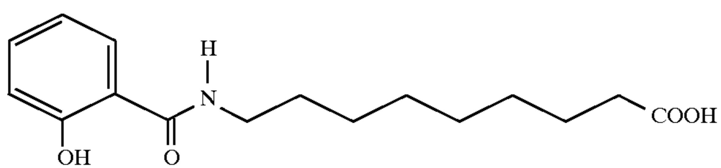
9-Salicyloylaminononanic acid
