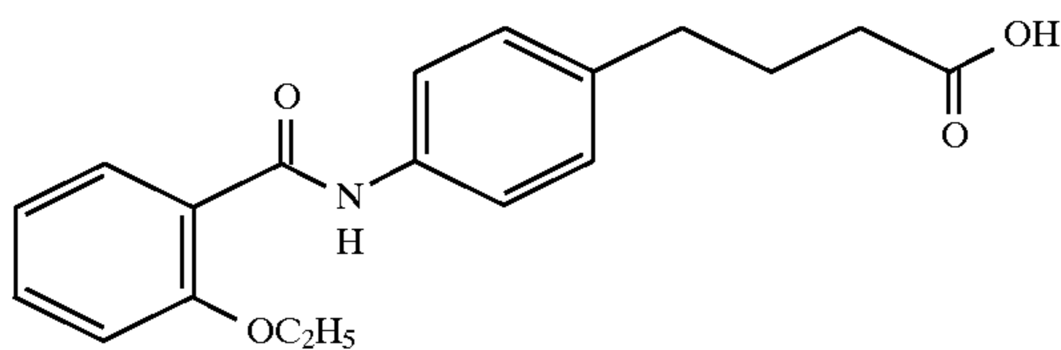
4-(4-(2-ethoxybenzoyl)aminophenyl)butyric acid
