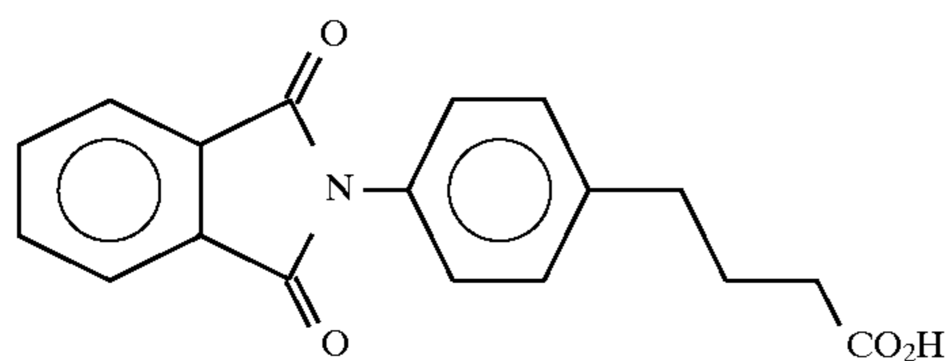
4-(4-phthalimidophenyl)butanoic acid
