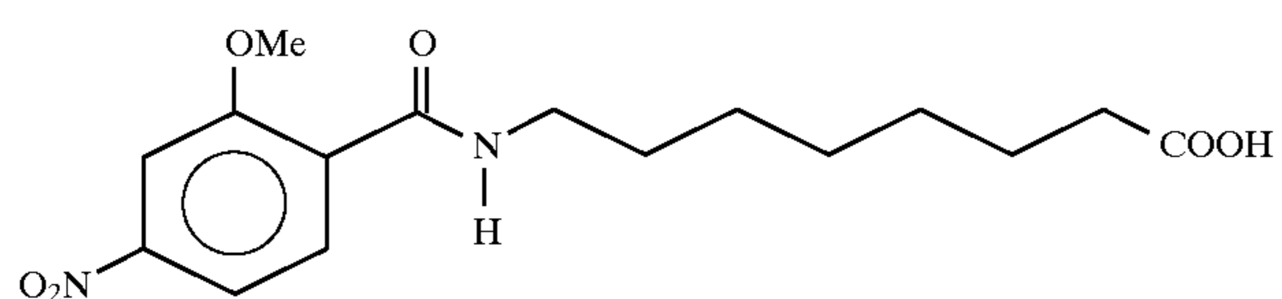
8-N-(4-methoxy-3-nitrobenzoyl)aminocaprylic acid
