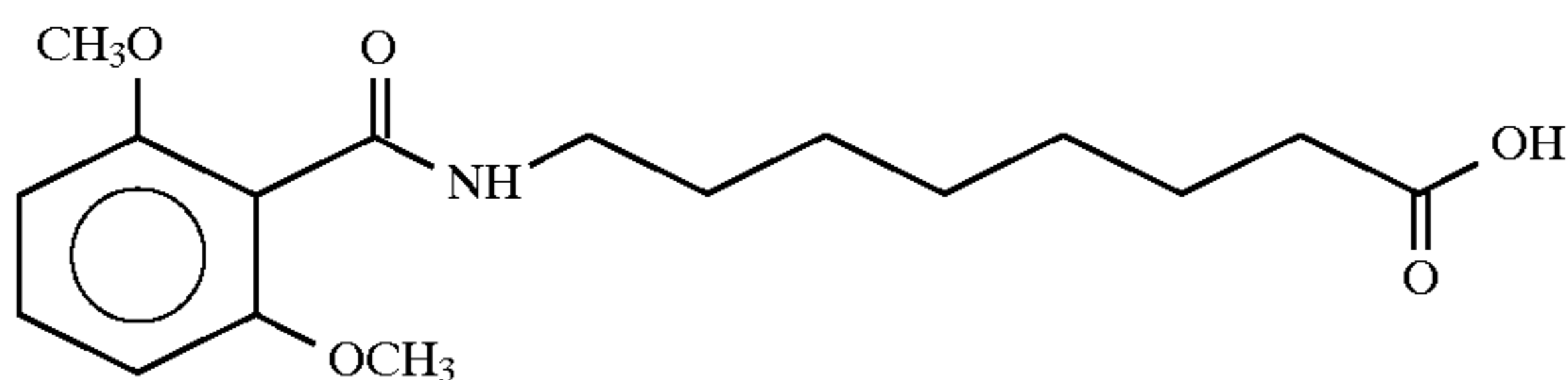
8-(N-2-6-Dimethoxybenzoyl)aminocaprylic acid
