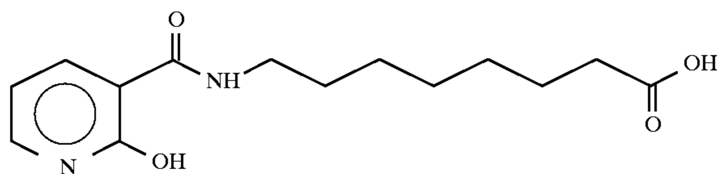
8-(2-Hydroxynicotinoyl)aminocaprylic acid
