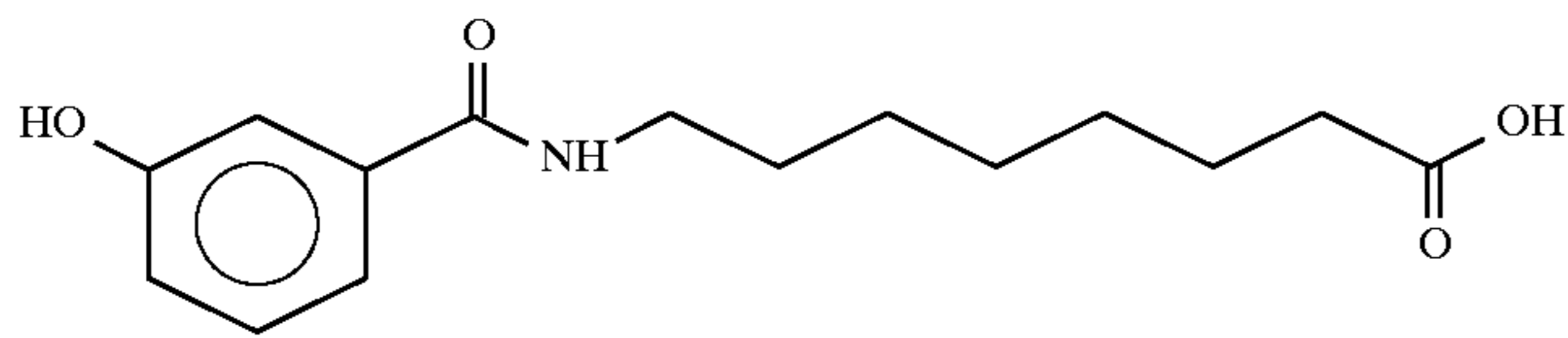
8-(3-Hydroxybenzoyl)aminocaprylic acid
