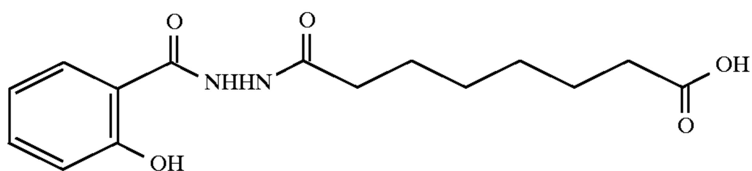
1-salicyloyl-2-suberyl hydrazide
