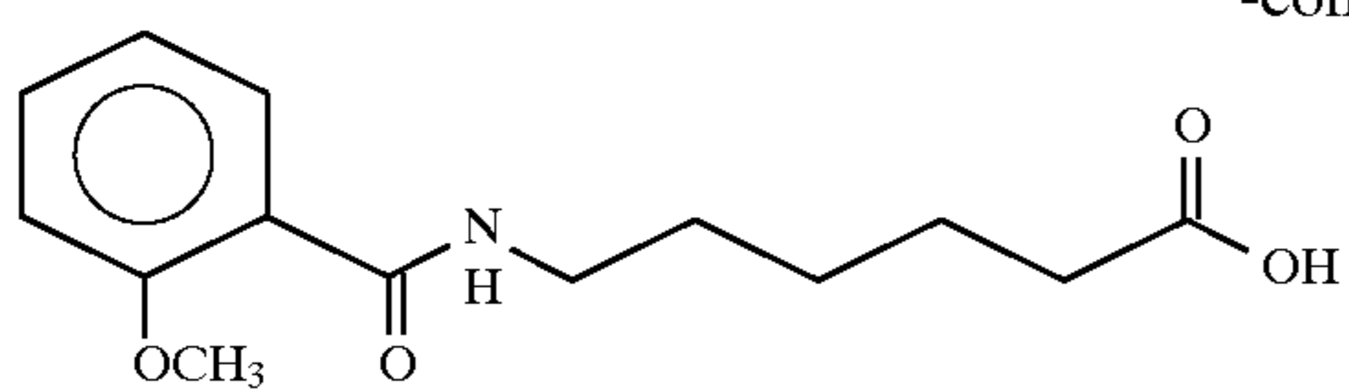
6-(anisoyl)aminocaproic acid
