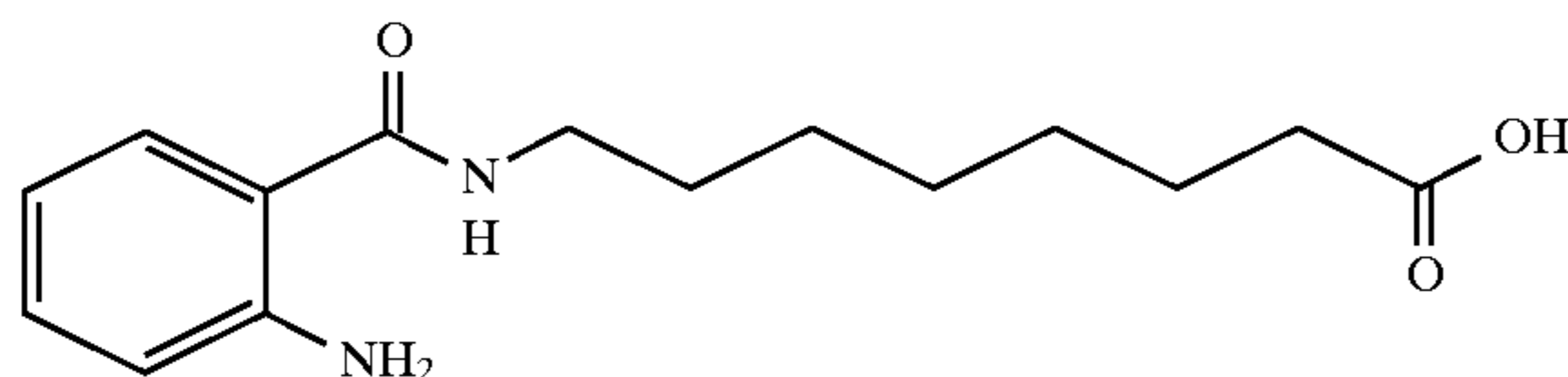
8(2-aminobenzoylamino)caprylic acid
