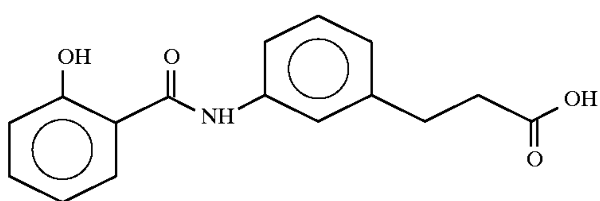
3-(3-(salicyloyl)aminophenyl)propionic acid
