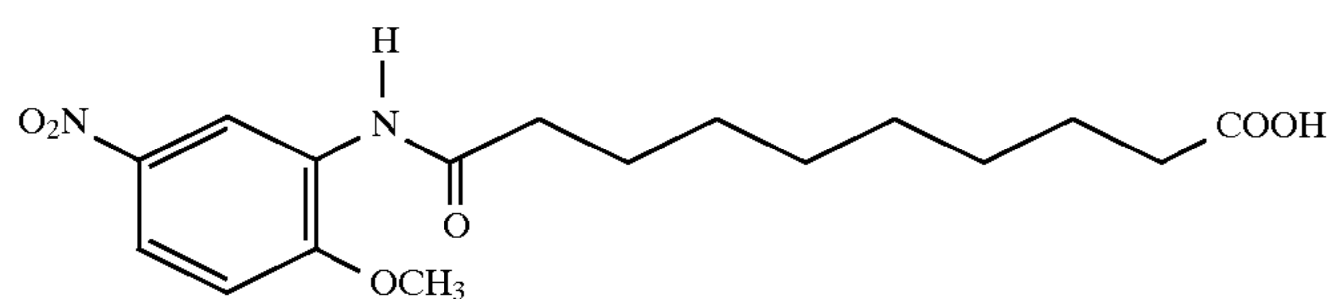
N-(2-methoxy-5-nitrophenyl) sebecoyl amide acid
