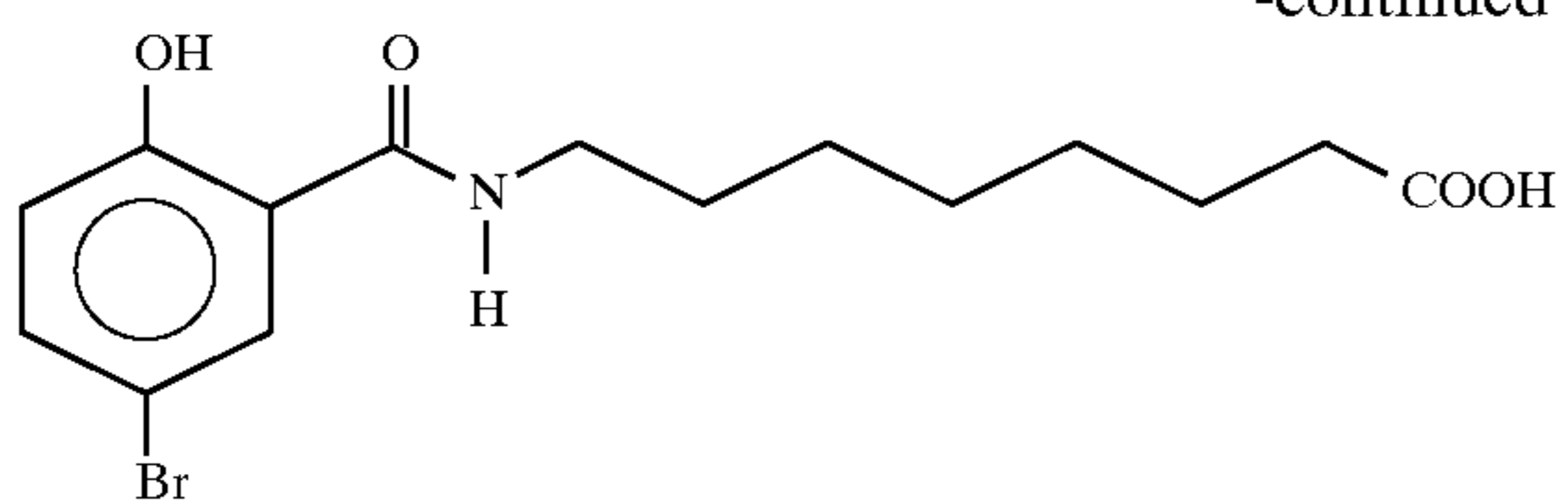
8-(N-(2-hydroxy-5-bromobenzoyl)aminocaprylic acid
