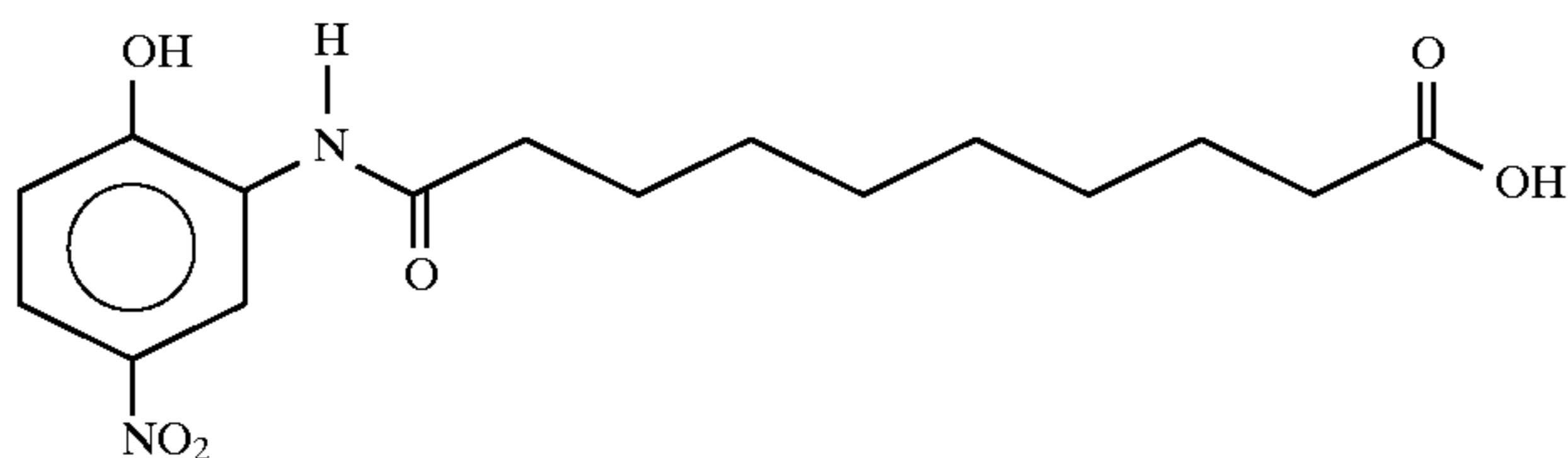
N-10-(2-hydroxy-5-nitroanilino)decanoic acid
