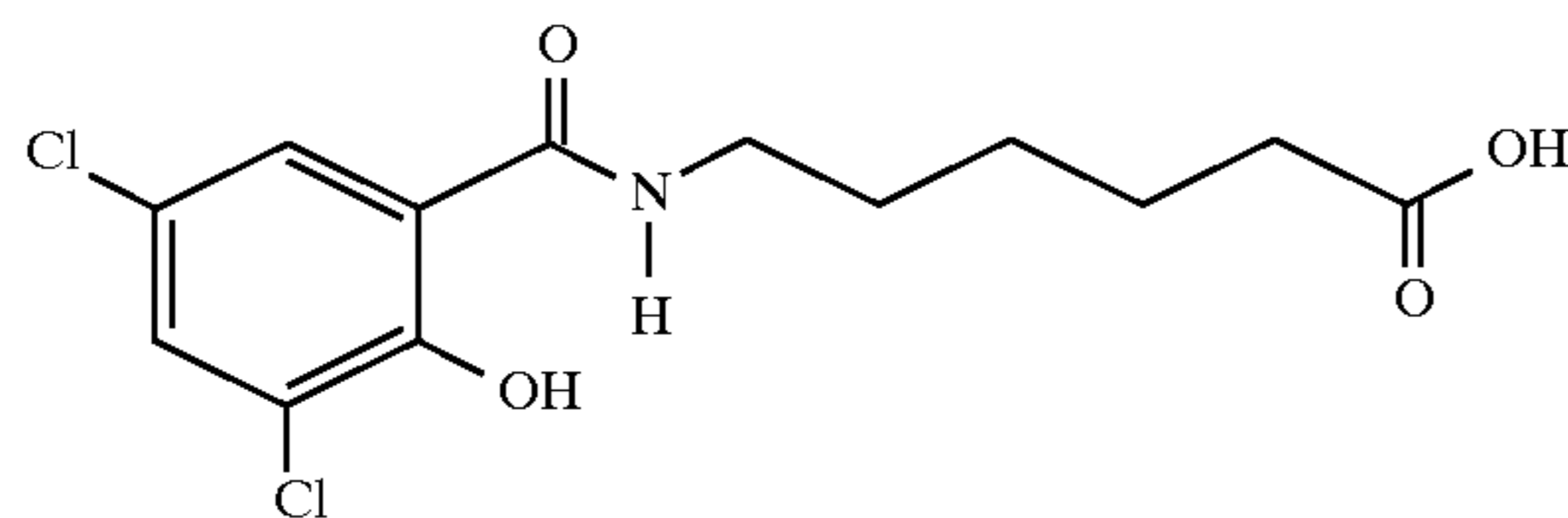
6-N-(3,5-dichloro-2-hydroxybenzoyl)aminocaproic acid
