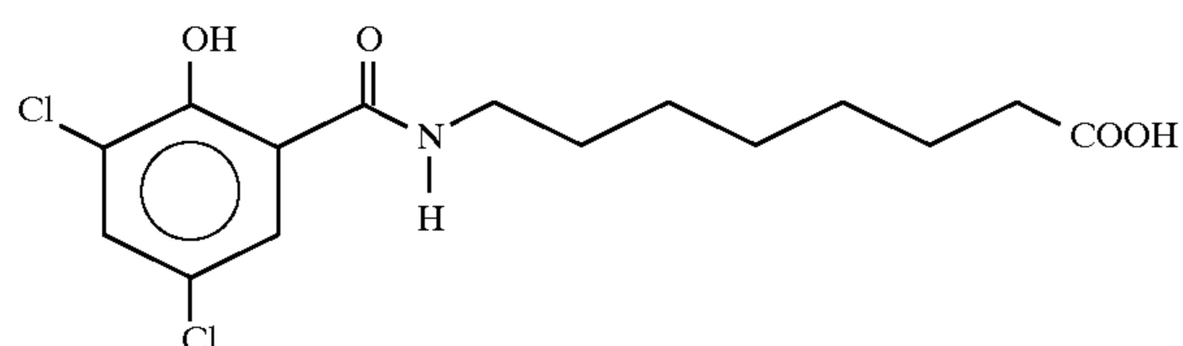
8-[N-(2-hydroxy-3,5-dichlorobenzoyl)]aminocaprylic acid
