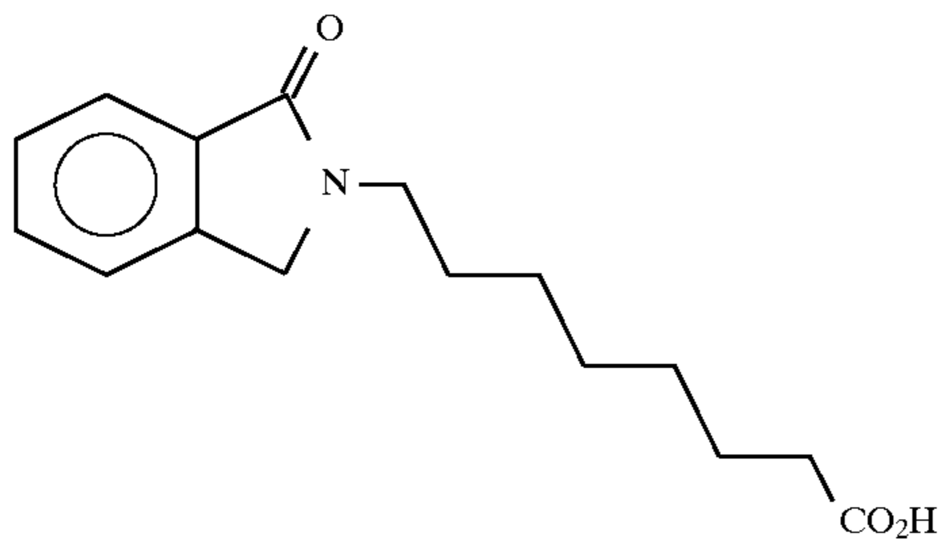
8-(2-(1,2-dihydroisoindole-1-one))octanoic acid
