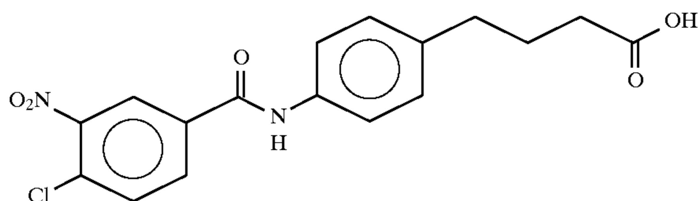
4-(4-(4-chloro-3-nitrobenzoyl)aminophenyl)butyric acid
