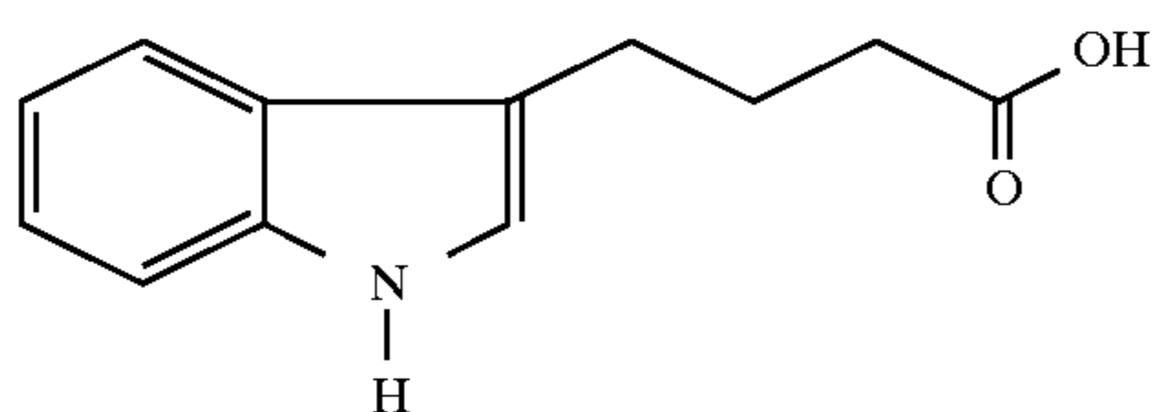
3-Indolebutyric acid
