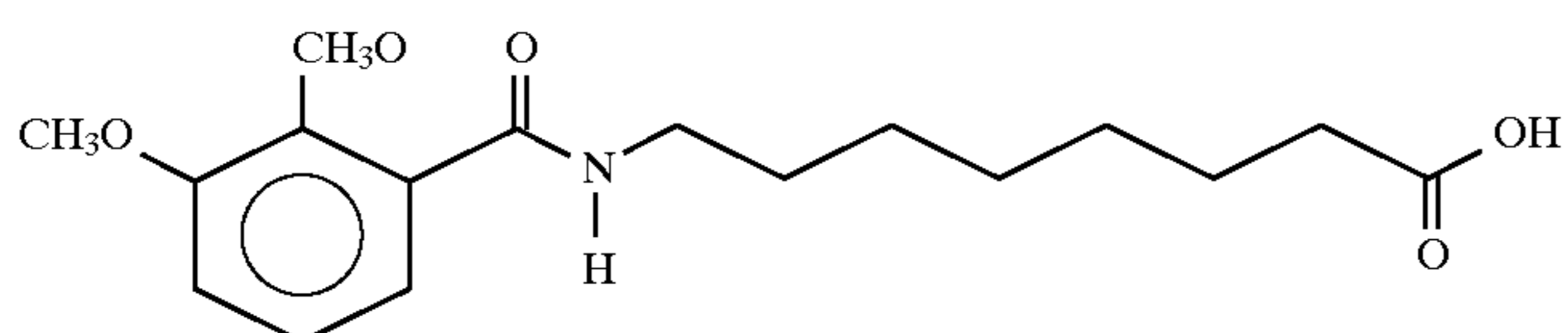
8-(N-2,3-Dimethoxybenzoyl)aminocaprylic acid
