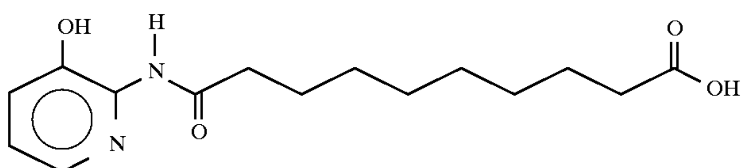
9-[2-(3-hydroxy)pyridylaminocarbonyl]nonanoic acid
