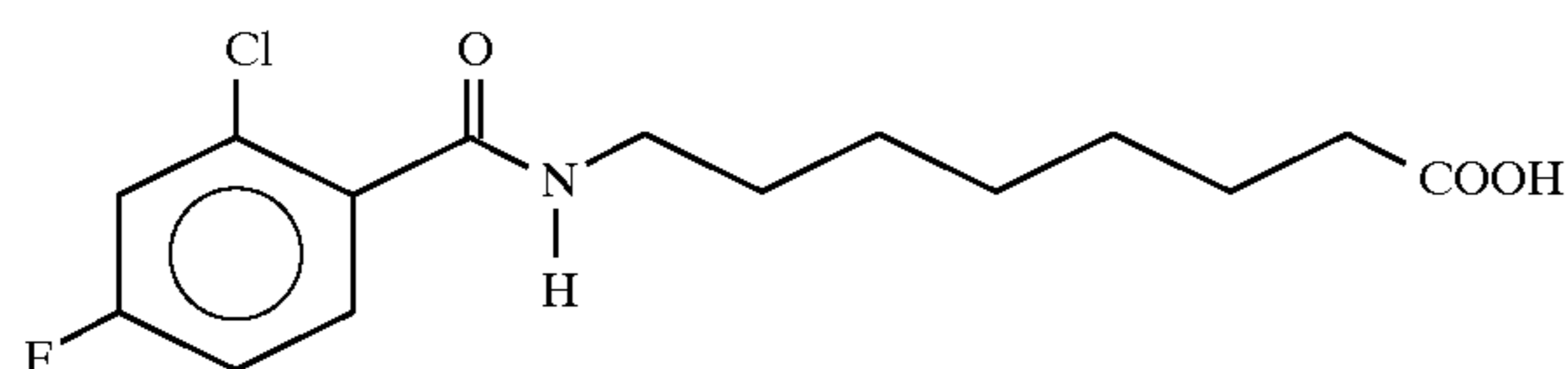
8-(N-(2-chloro-4-fluorobenzoyl)aminocaprylic acid
