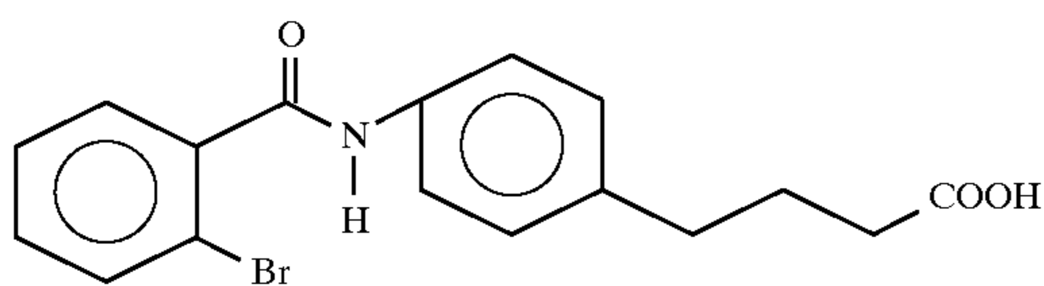
4{4-[N-2-bromobenzoyl] aminophenyl} butyric acid
