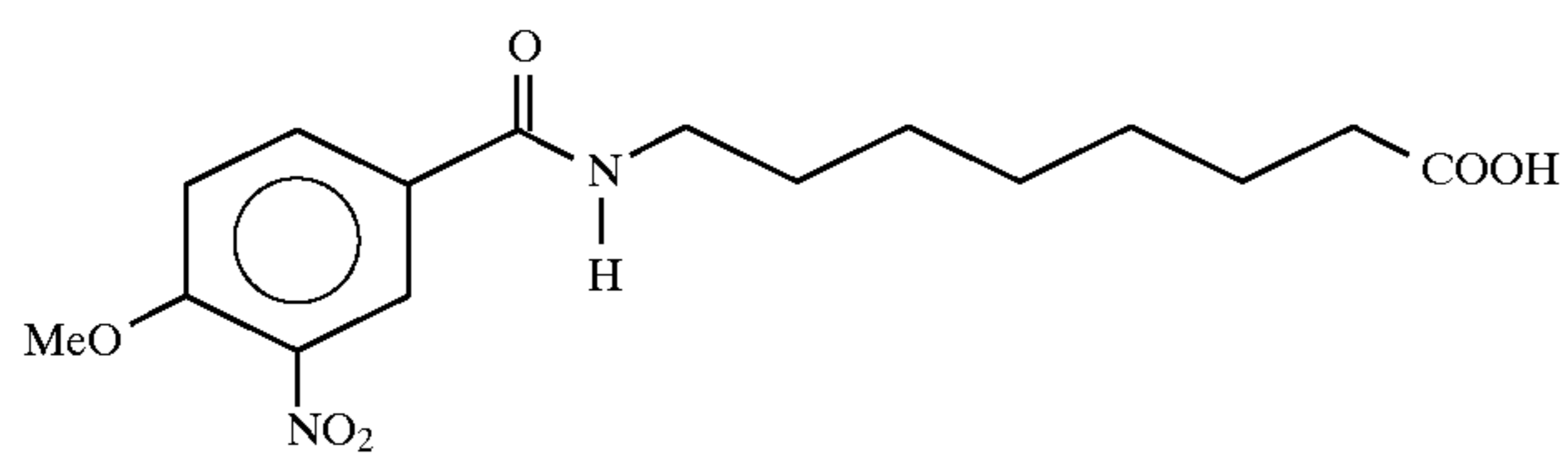
8-N-(4-methoxy-3-nitrobenzoyl)aminocaprylic acid
