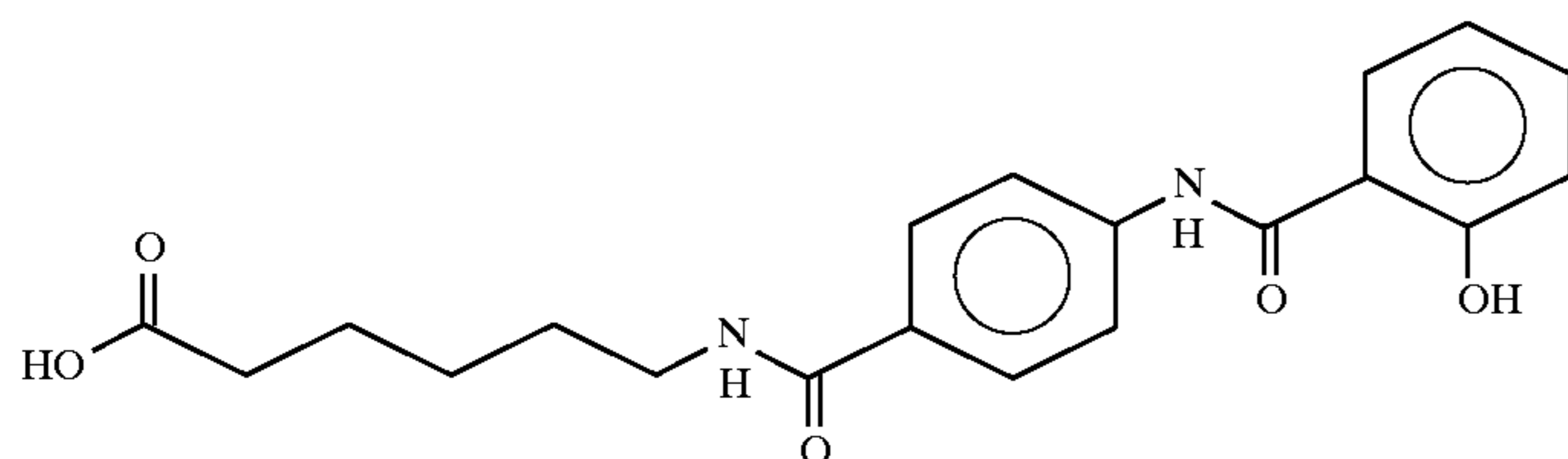
N-(4-salicyloylamino)-6-caproic acid
