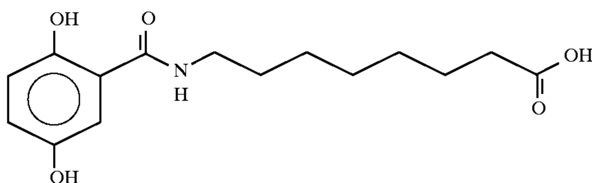
8-(N-2,5-Dihydroxybenzoyl)aminocaprylic acid
