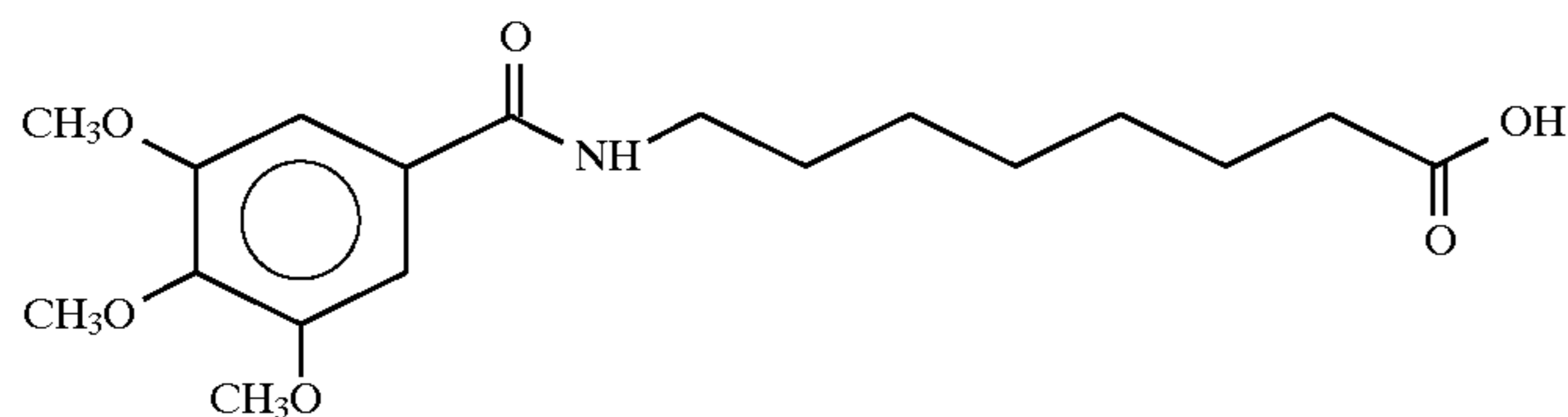
8-(3,4,5-Trimethoxybenzoyl)aminocaprylic acid
