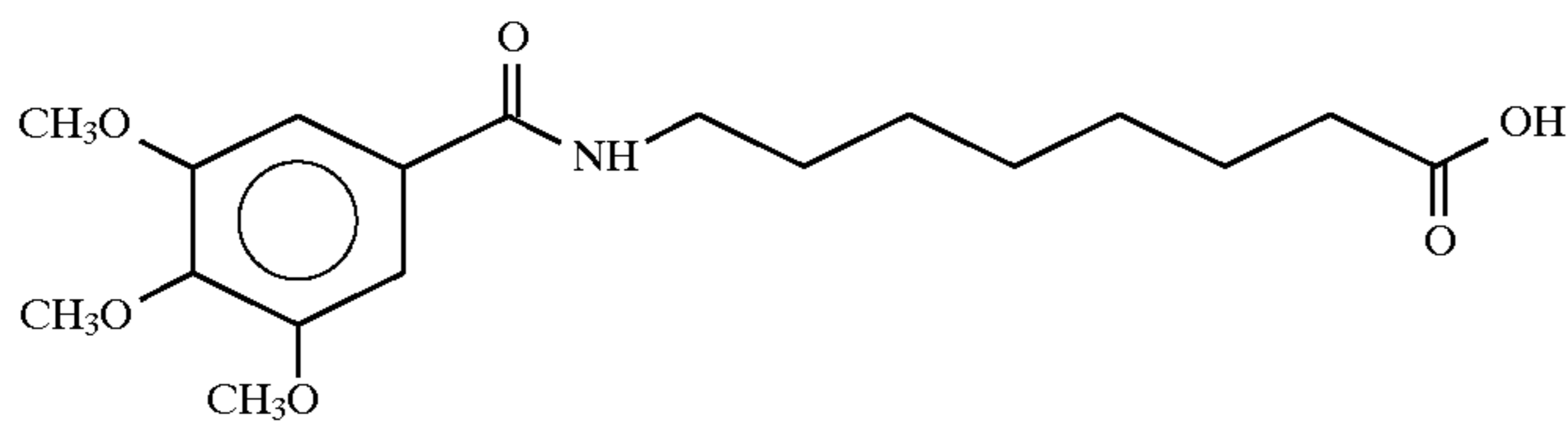
8-(3,4,5-Trimethoxybenzoyl)aminocaprylic acid
