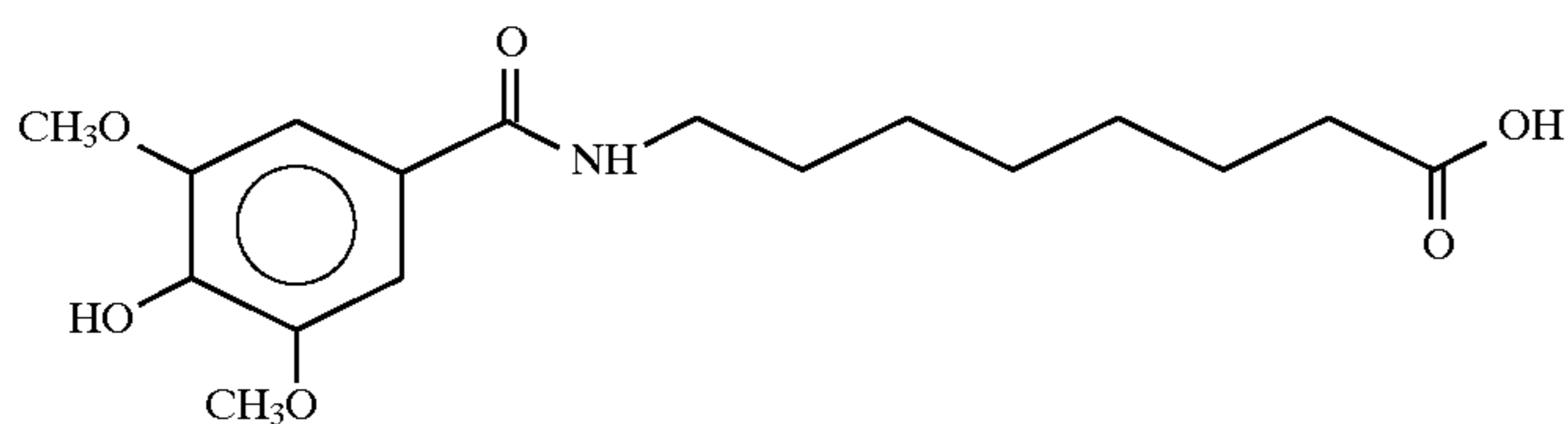
8-(N-3,5 Dimethoxy 4-hydroxybenzoyl)aminocaprylic acid
