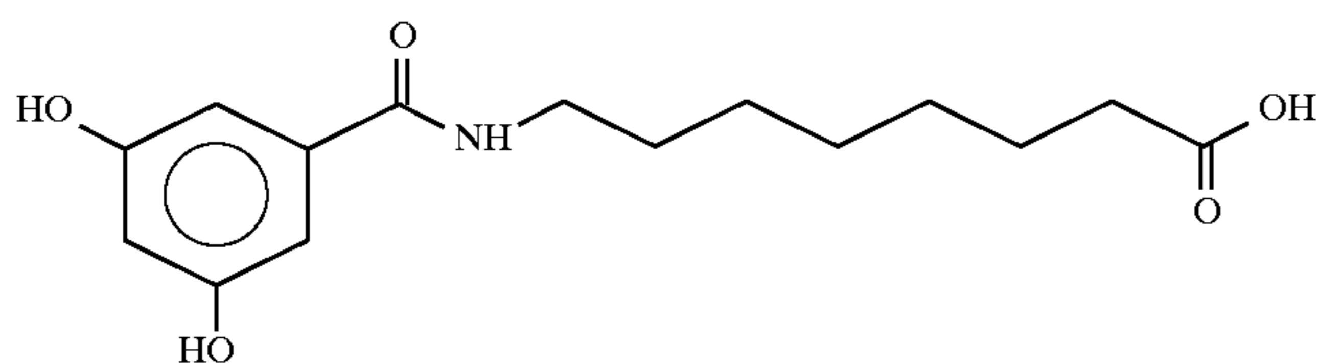
8-(N-3,5 Dihydroxybenzoyl)aminocaprylic acid
