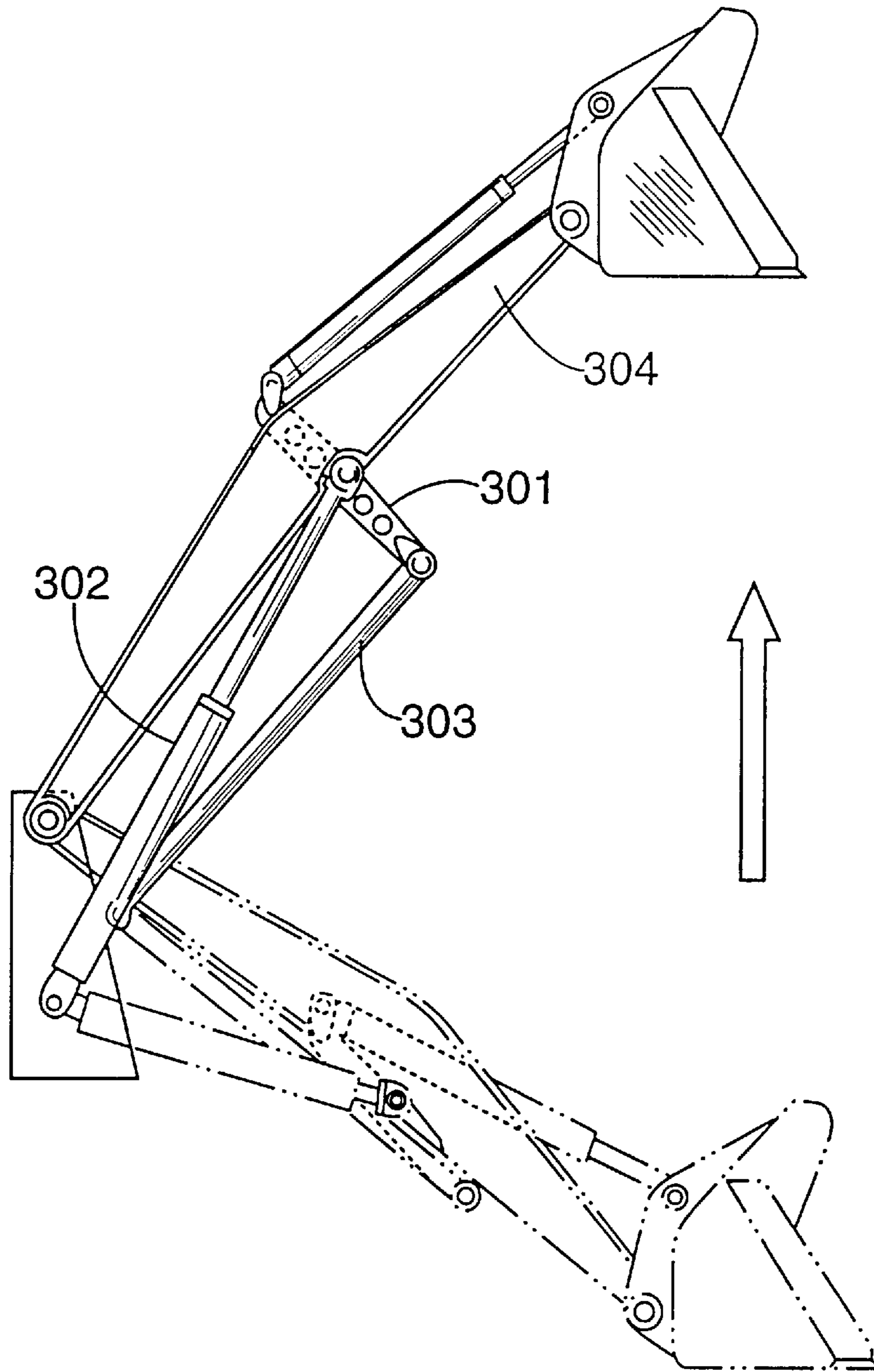
FIG. 1 PRIOR ART
