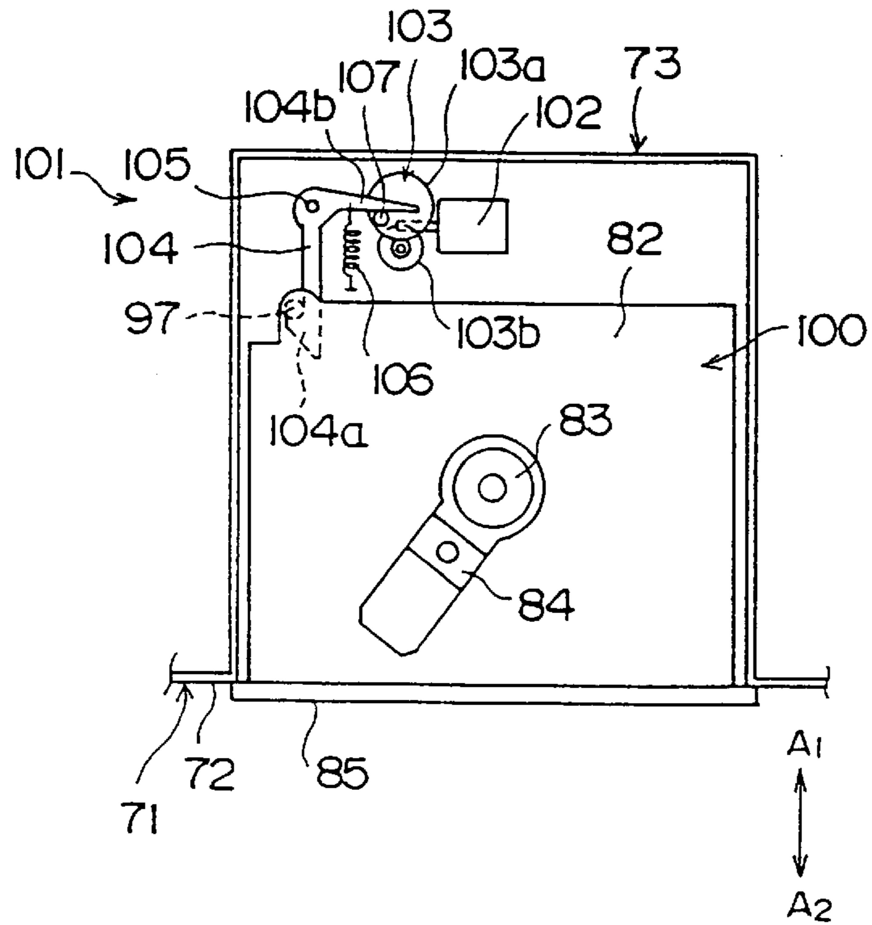
FIG. 2 (PRIOR ART)
