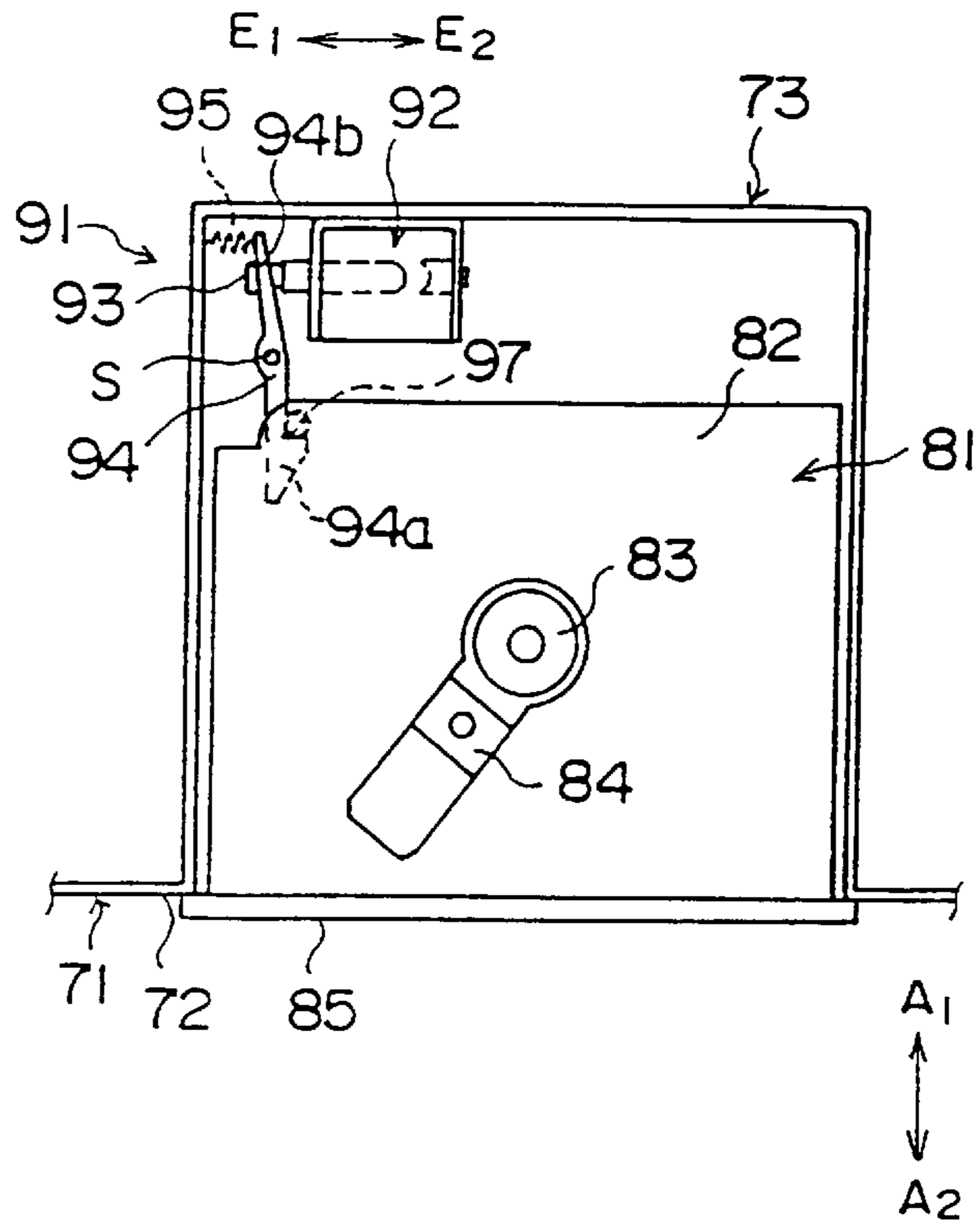
FIG. 1 (PRIOR ART)
