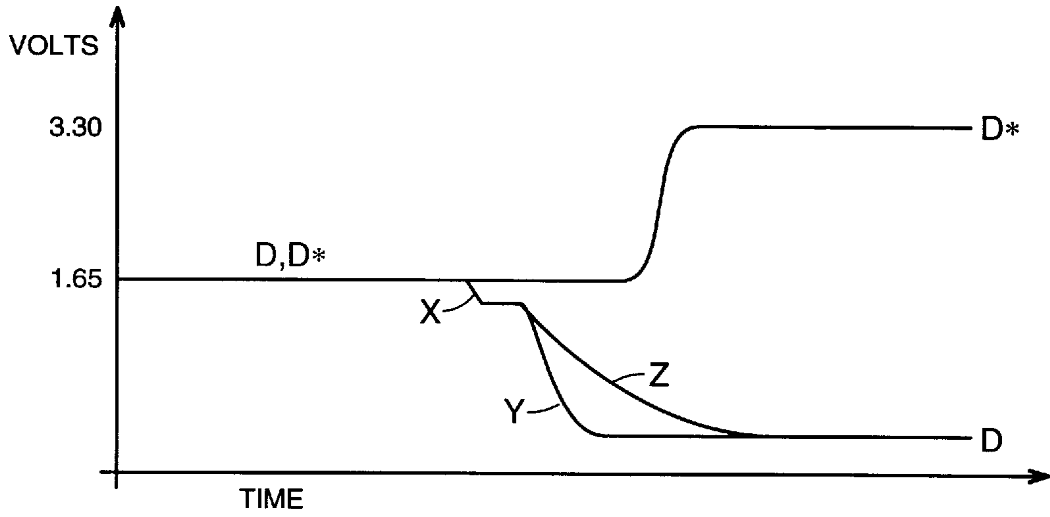
FIG. 2 (PRIOR ART)
