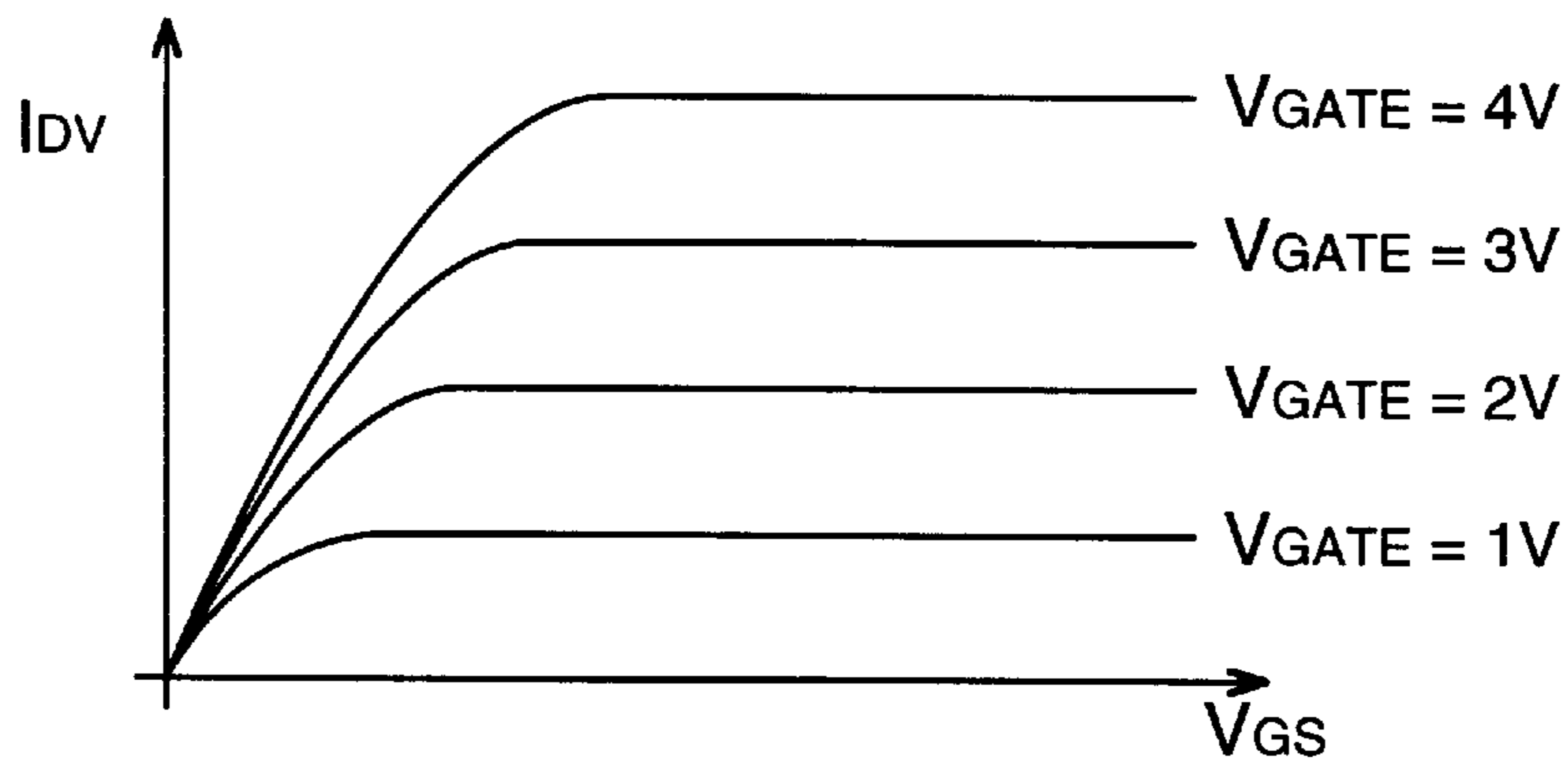
FIG. 3 (PRIOR ART)
