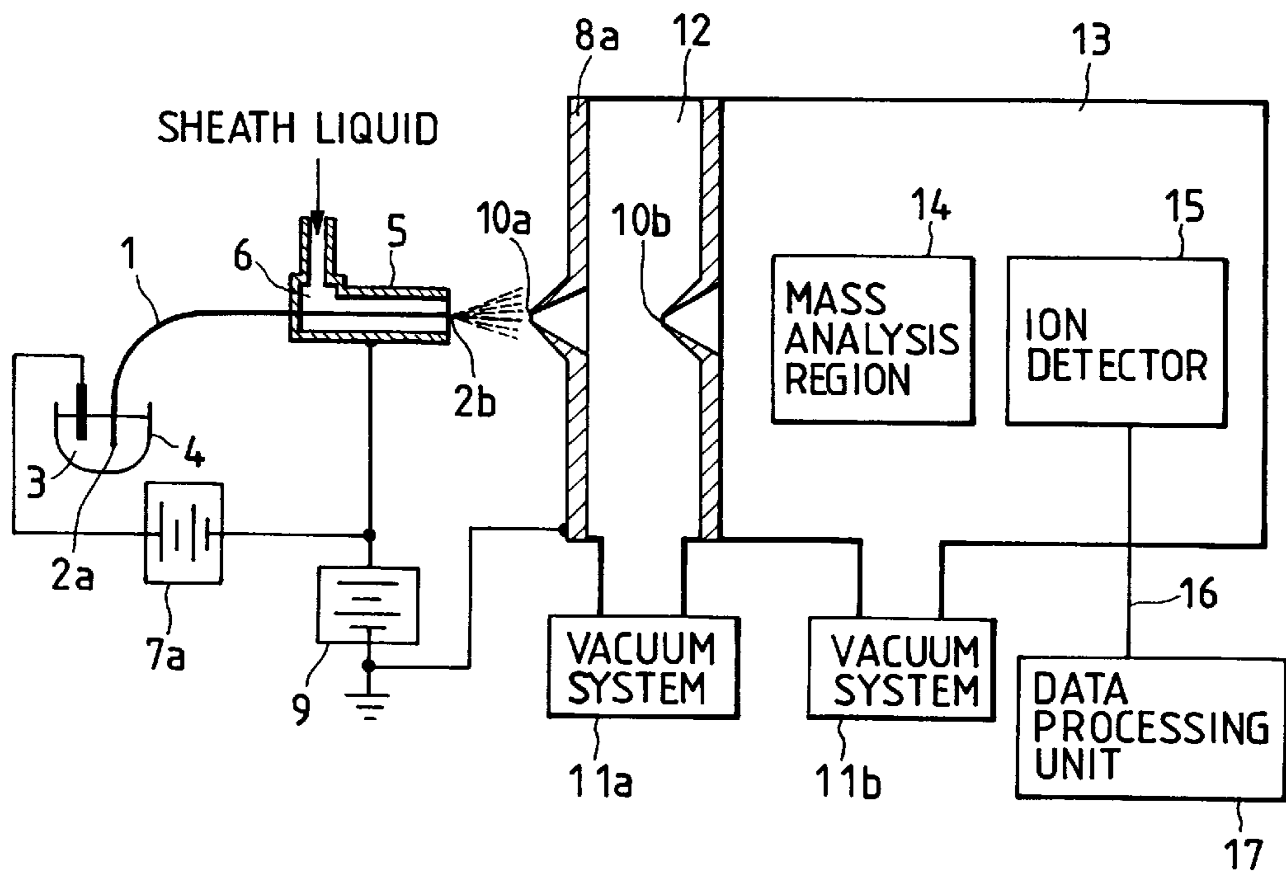
FIG. 13 (PRIOR ART)
