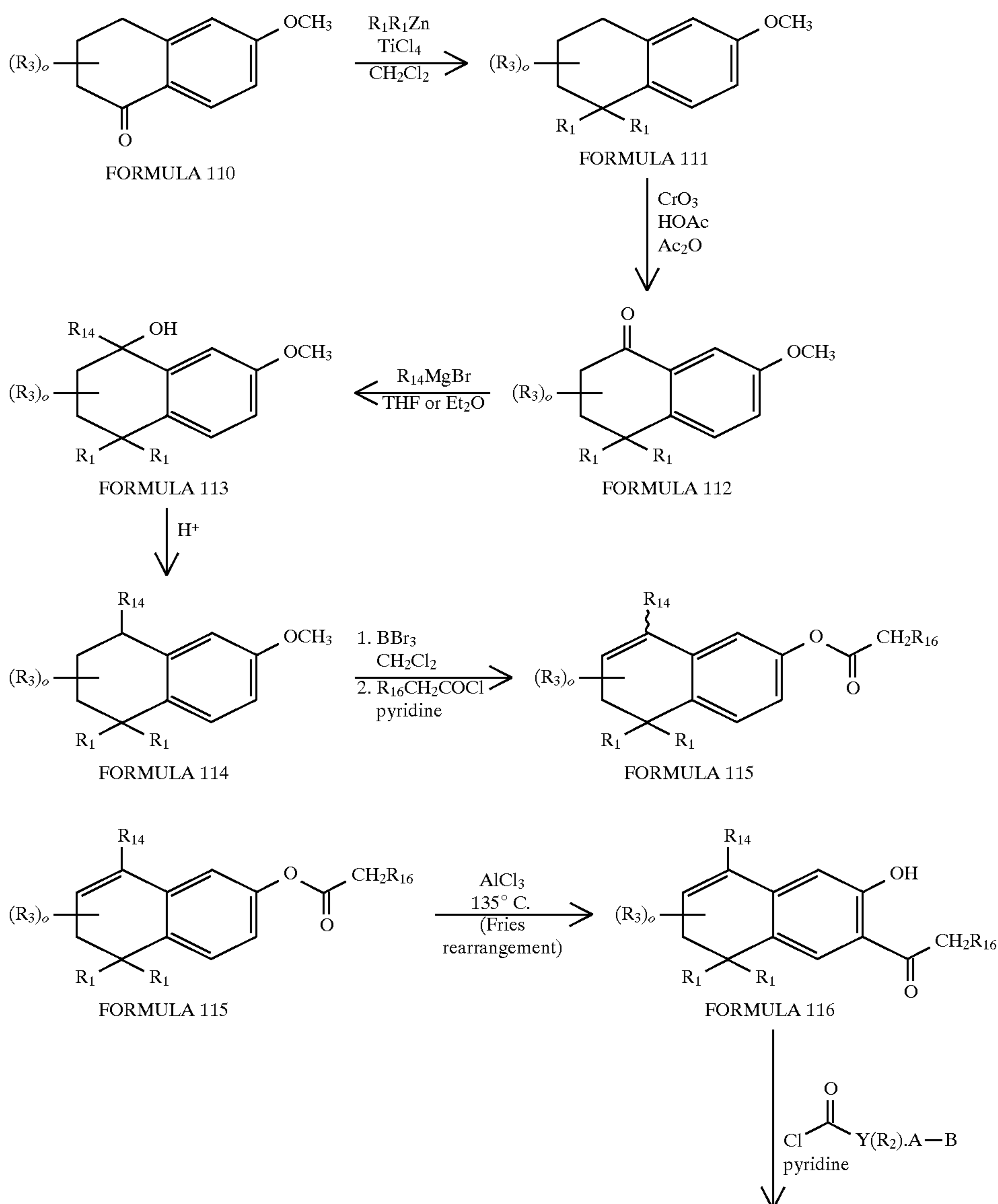
Reaction Scheme 102
