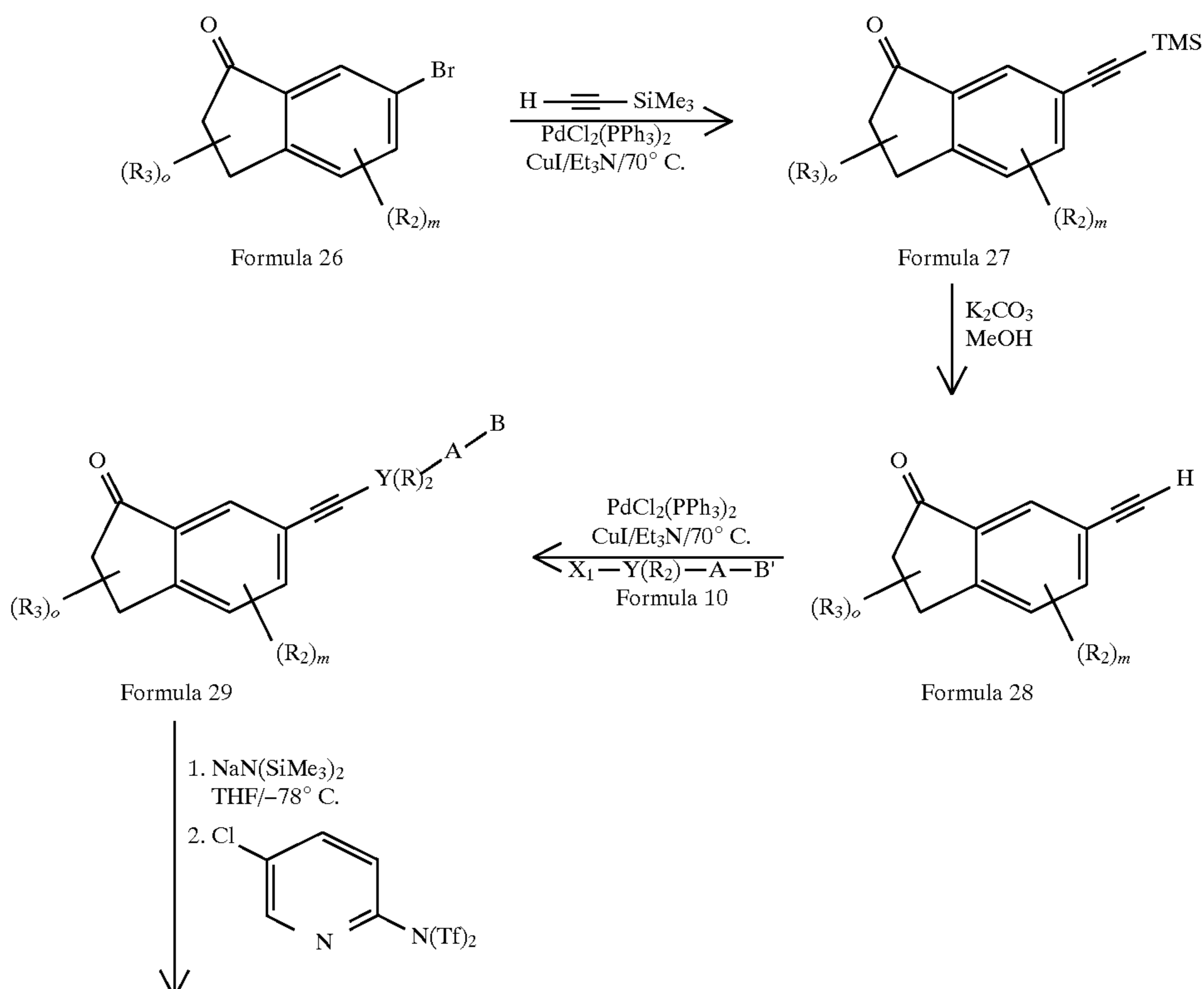
Reaction Scheme 3
