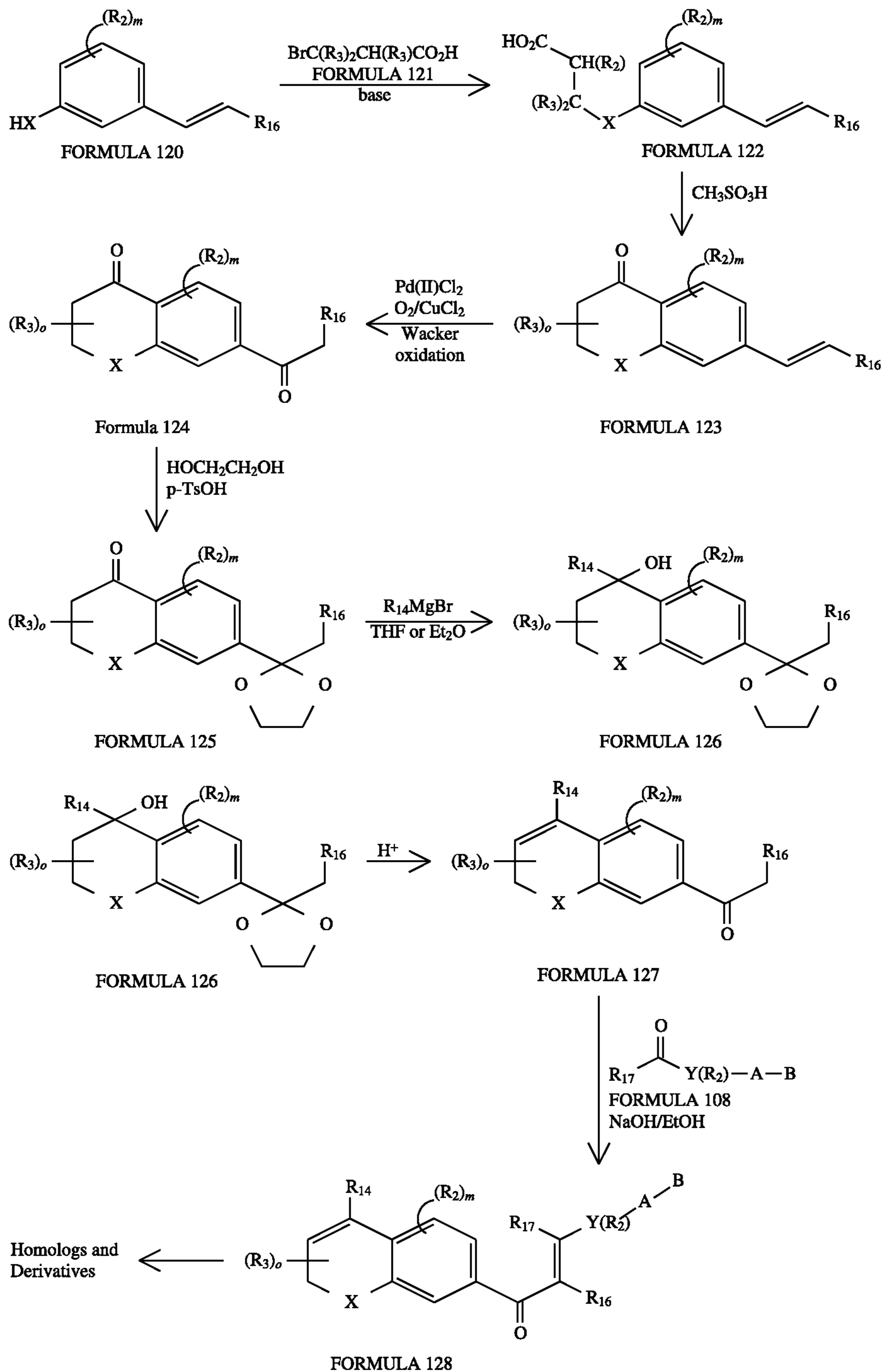
Reaction Scheme 103
