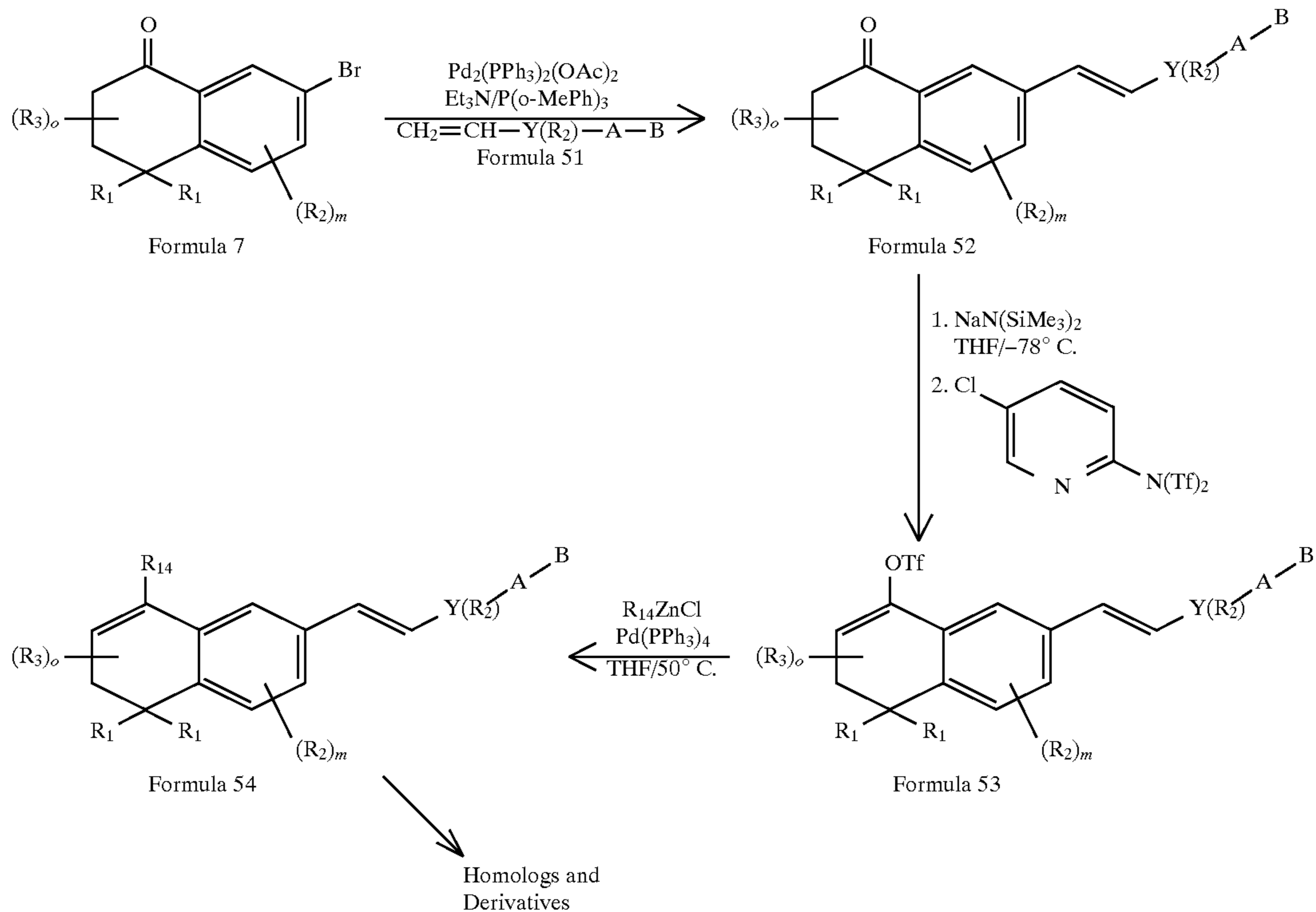
Reaction Scheme 8
