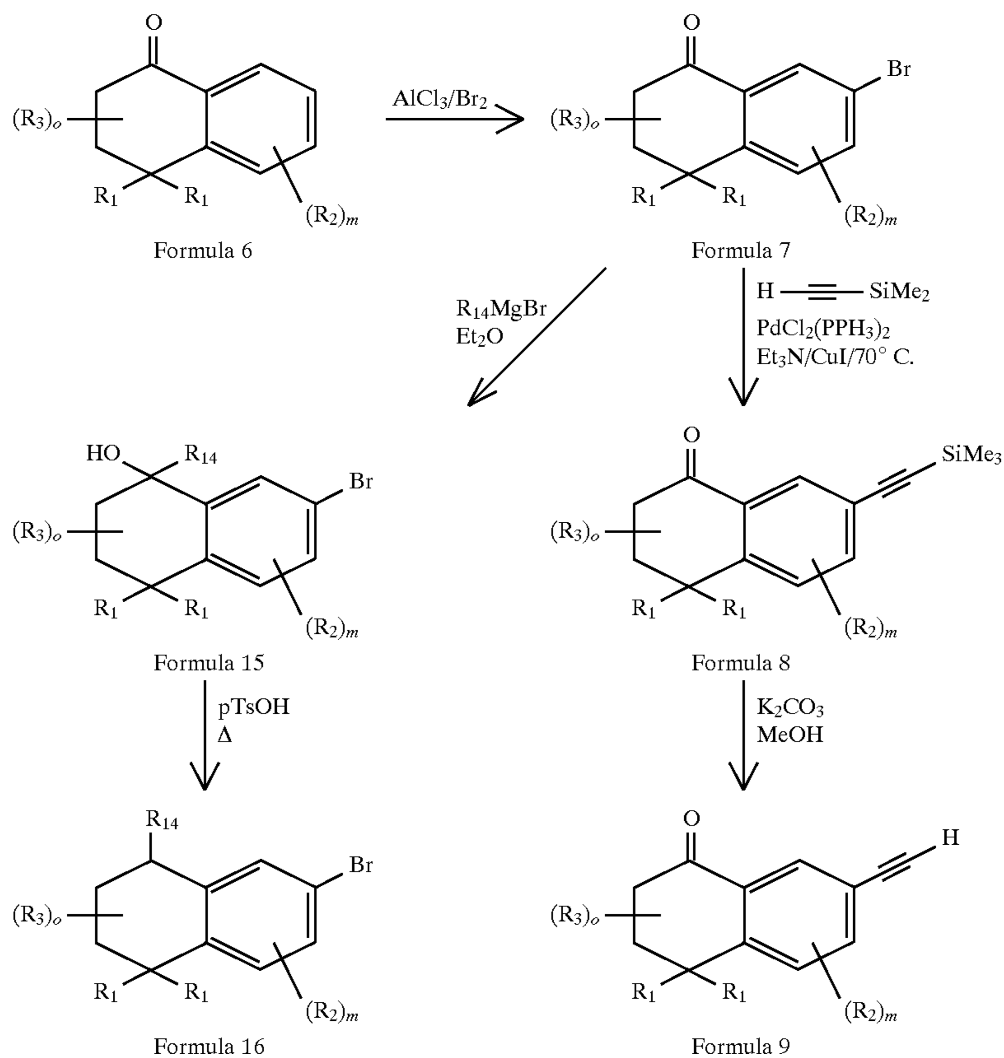
Reaction Scheme 1
