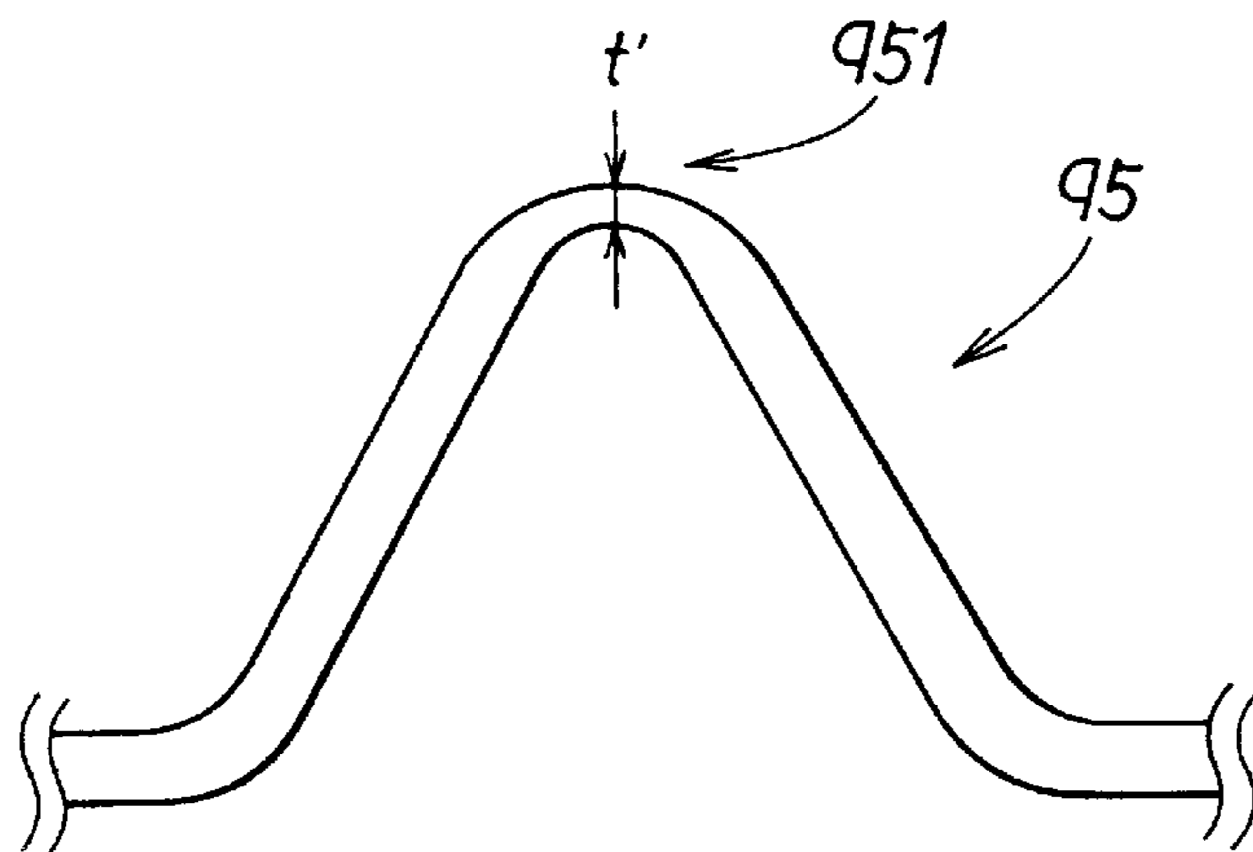
FIG. 32 RELATED ART
