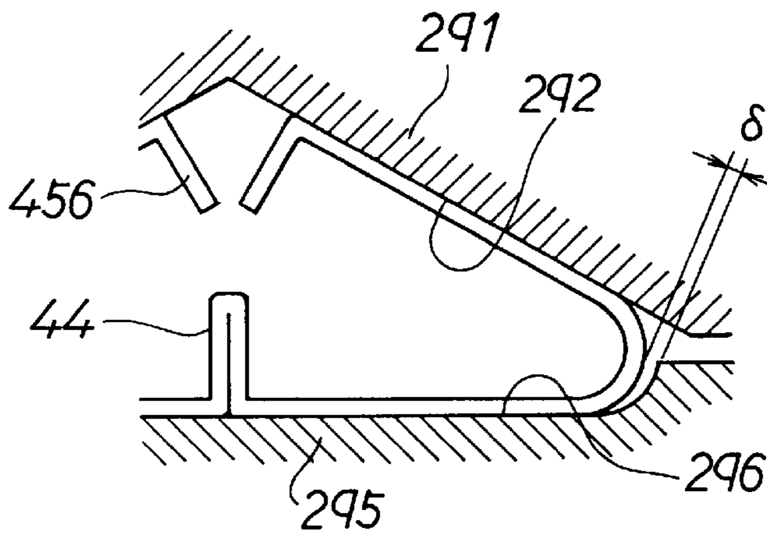
FIG. 30 RELATED ART
