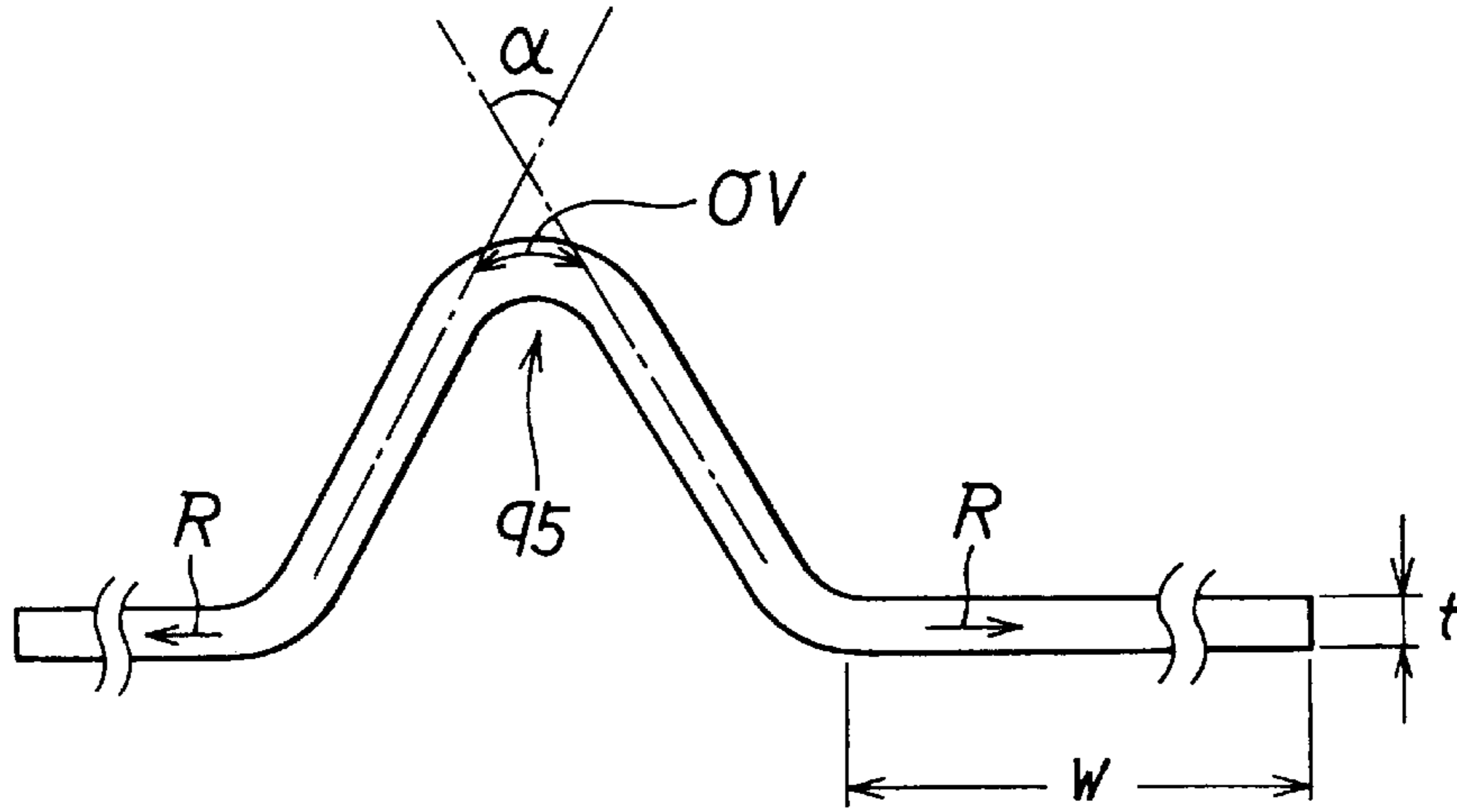
FIG. 32 RELATED ART
