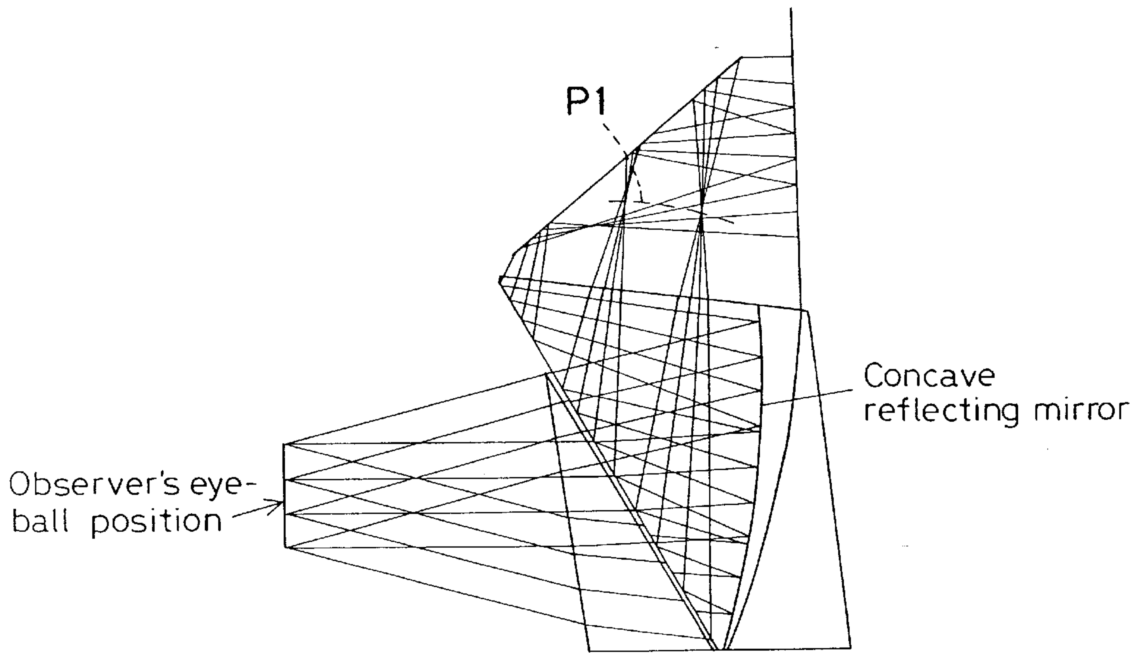
FIG. 19 (b) (PRIOR ART)
