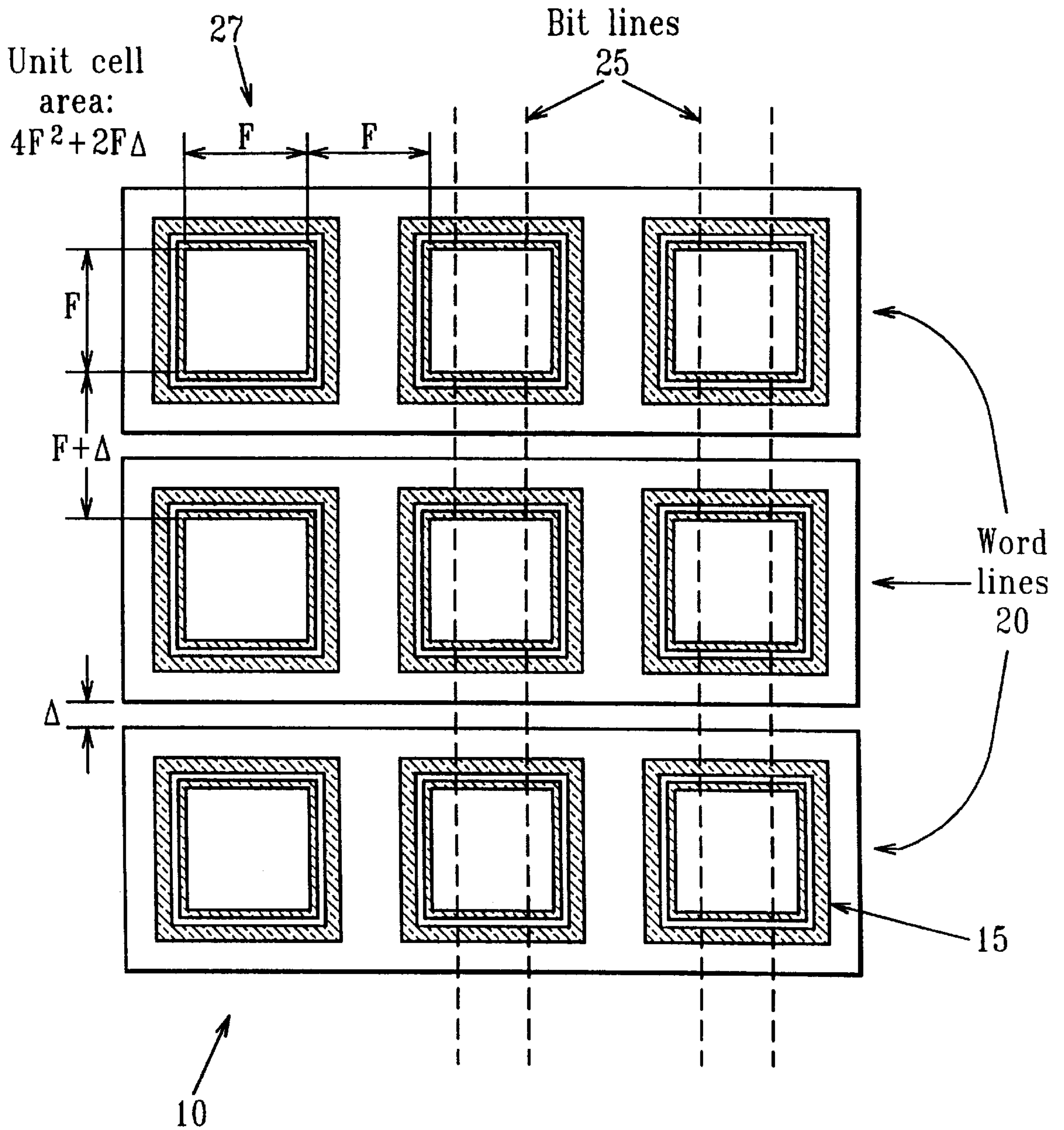
FIG. 1 (PRIOR ART)
