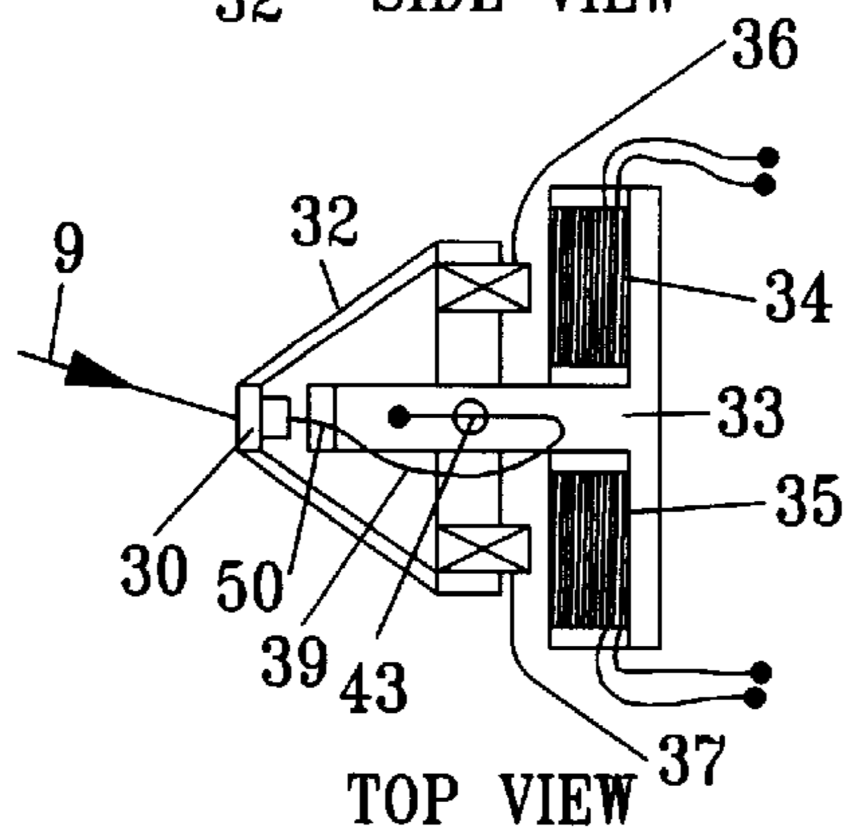
SCAN BEAM: MIRROR NEAR ZERO DEFLECTION
