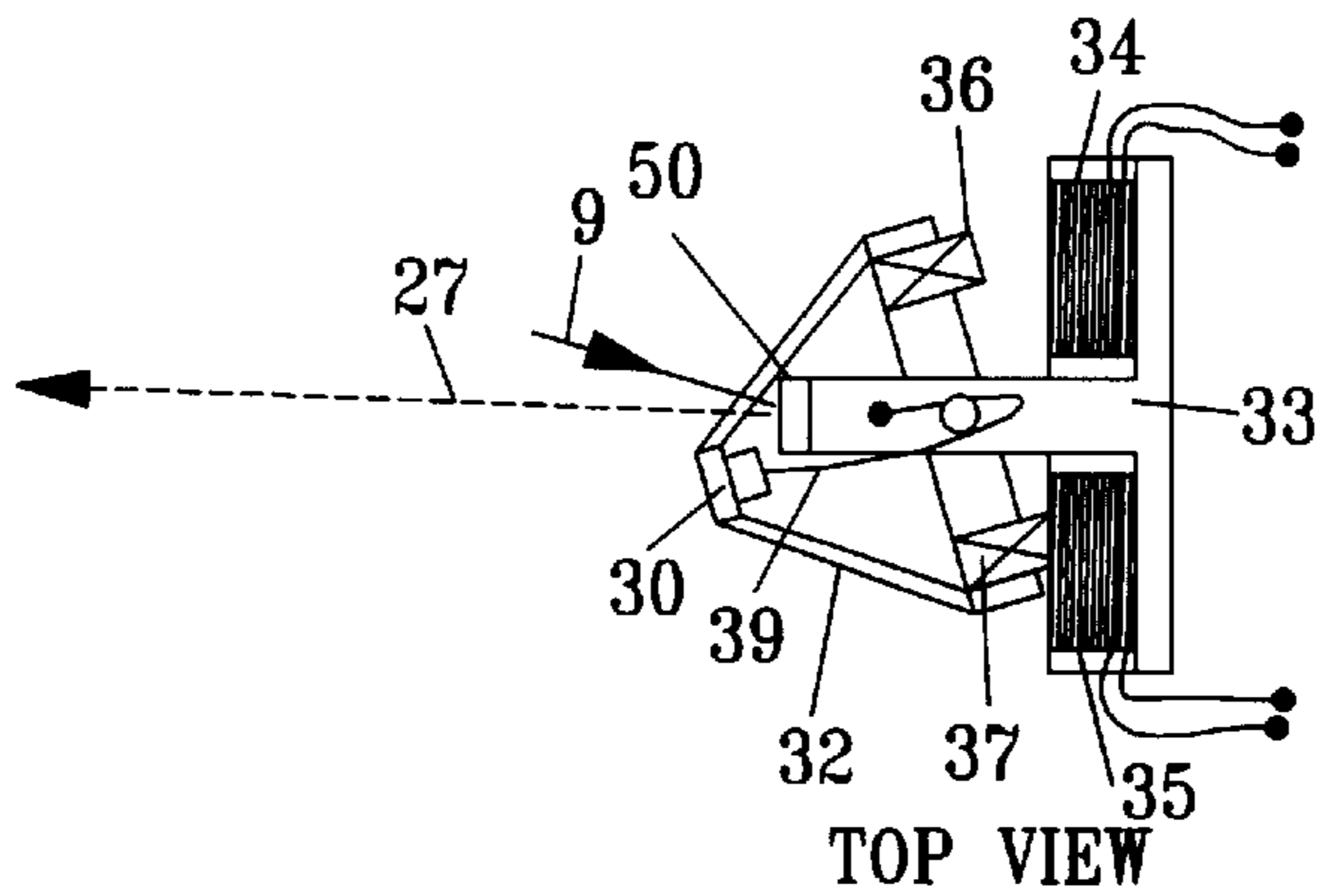
POINTER BEAM: MIRROR AT END OF DEFLECTION
