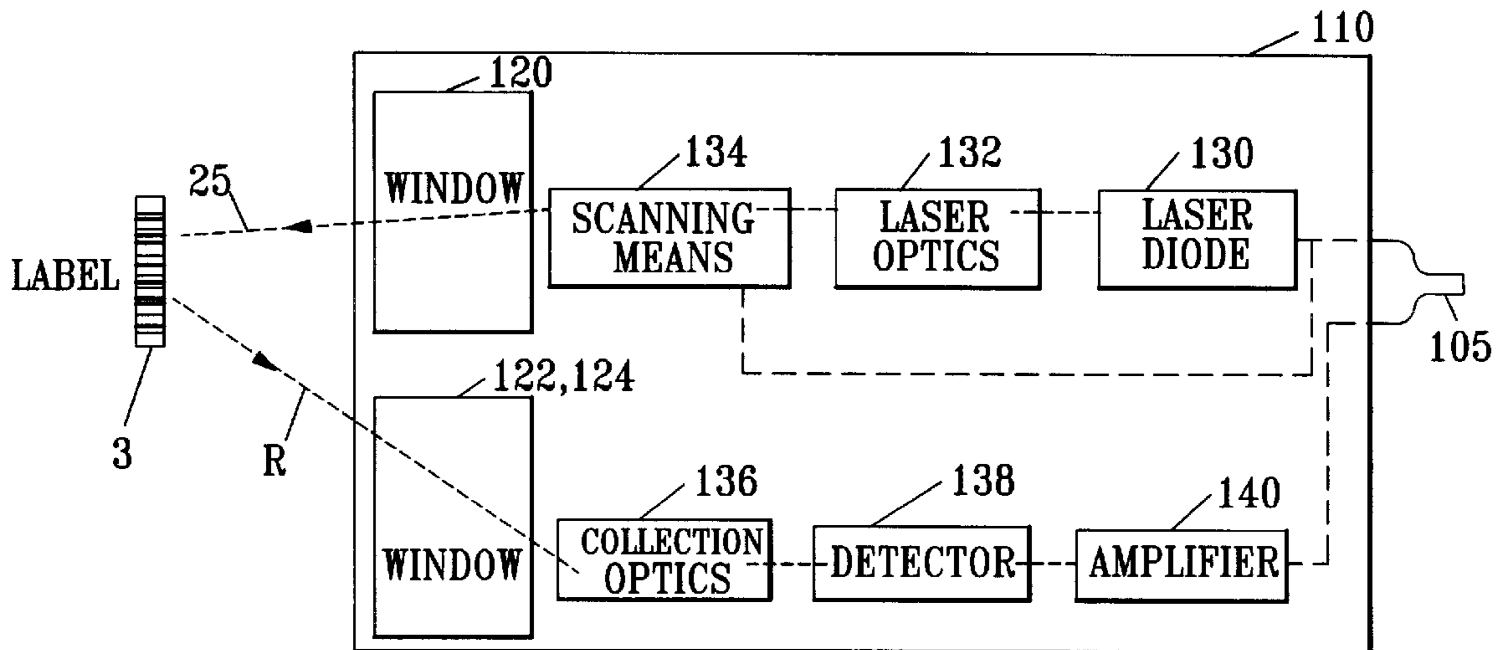
DIRECT COLLECTION BLOCK DIAGRAM OF THE STYLUS MOUNTED LABEL READER
